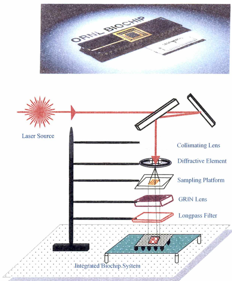
Figure 2.1 Schematic diagram of a biochip concept. Light from a 6.4 mW, He-Ne laser (632.8 nm) was transmitted through a laser band pass filter, a collimating lens, a 4 x 4 optical diffractive element and focused onto sample spots situated directly above the phototransistor detection elements. The 4x4 sensing array is comprised of 16 individual photodiodes arranged in a square with 900- \mu\text{m} edges and 1-mm center-to-center spacing between them. A GRIN lens, and a 650 \pm 10 nm band pass filter was situated between the detector elements and the sample substrate to isolate the fluorescence of interest. The photocurrent of each sensing element of the amplifier/ phototransistor microchip was transmitted to a digital voltmeter linked to a multimeter for data recording.
