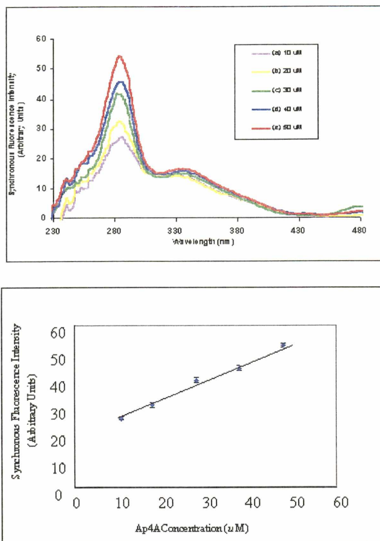
Figure 3.6 The quantitative ability of the SL technique to measure fluorescence intensity associated with increased AMP production at constant Fhit protein concentration and increasing concentrations of Ap 4 A (10-50 μM) are illustrated.
