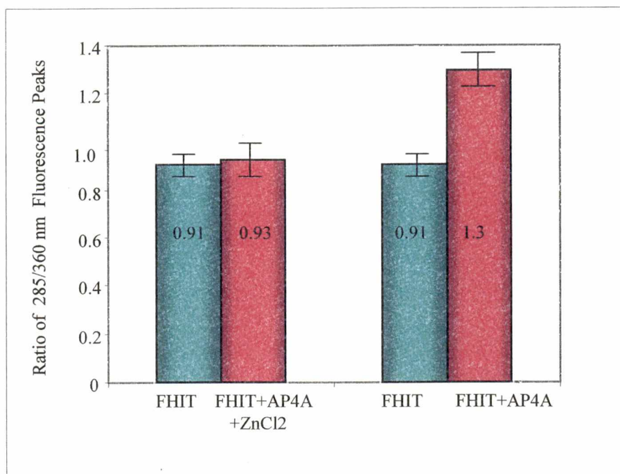
Figure 3.7 Inhibitory effects of \text{ZnCl}_2 (100 \mu\text{l} ) on hydrolysis activity of Fhit protein is demonstrated. Fluorescence intensity of the 285 nm peak did not increase relative to the intensity of the second peak in presence of \text{ZnCl}_2 . This alteration in the fluorescence profile was expected if Fhit protein had maintained its hydrolysis activity in the presence of \text{Zn}^{2+} .
