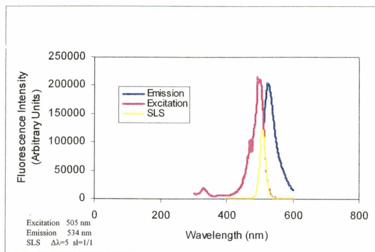
(a) Rhodamine 123 spectra
