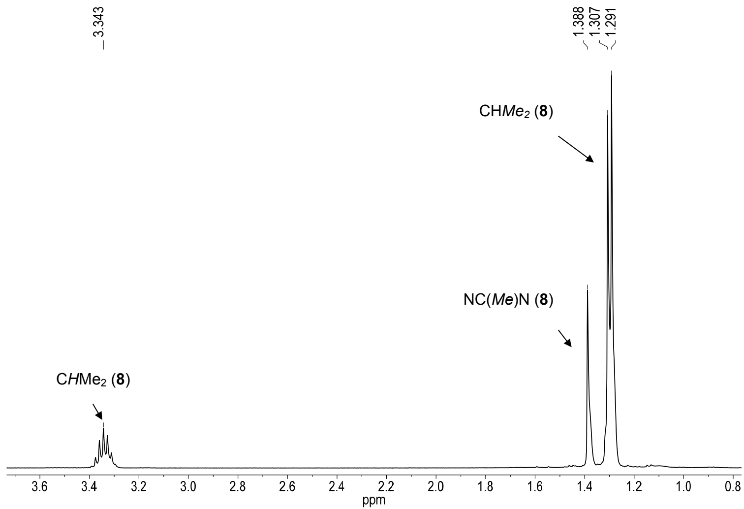
Figure 2.4. ^1\text{H} NMR spectrum of 8 in benzene- d_6 .
