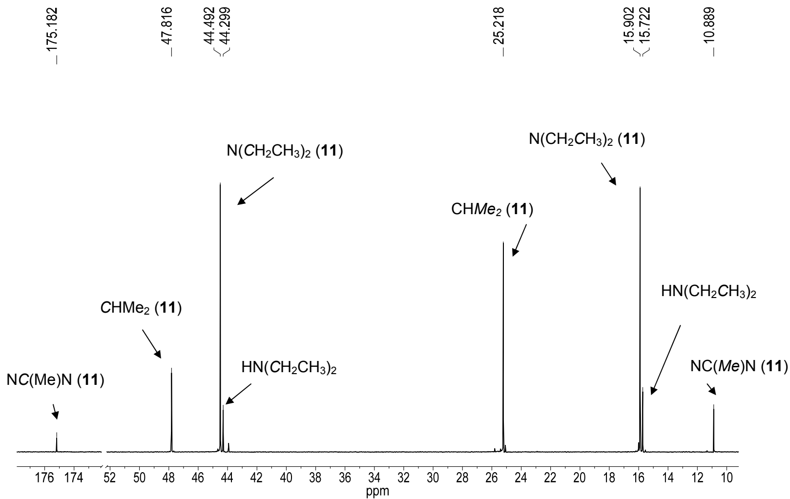
Figure 2.12. ^{13}\text{C}\{^1\text{H}\} NMR spectrum of 11 in benzene- d_6 .
