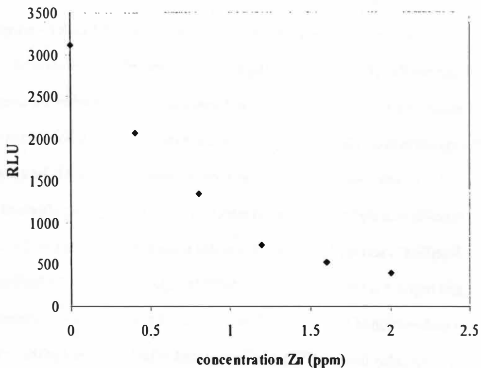
Figure 4.7: Relative light units (RLU) vs. concentration Zn (ppm) for PM6 exposed to \text{Zn}^{2+} showing a power curve relationship between concentration and response.
