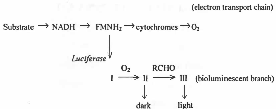
Figure 2.1: Electron transport chain joined with bioluminescent system (Hastings and Nealson, 1977).
