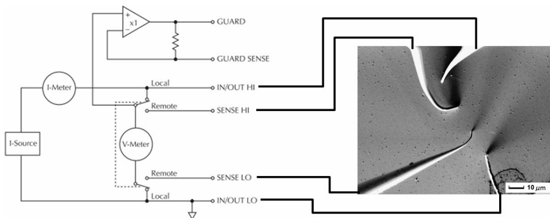
Figure 2-6: Circuit diagram of 4-probe STM transport measurement.
