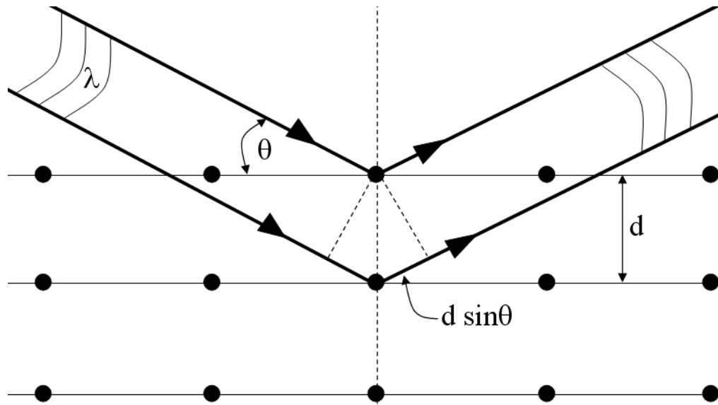
Figure 2-10: Bragg diffraction at sample surface.
