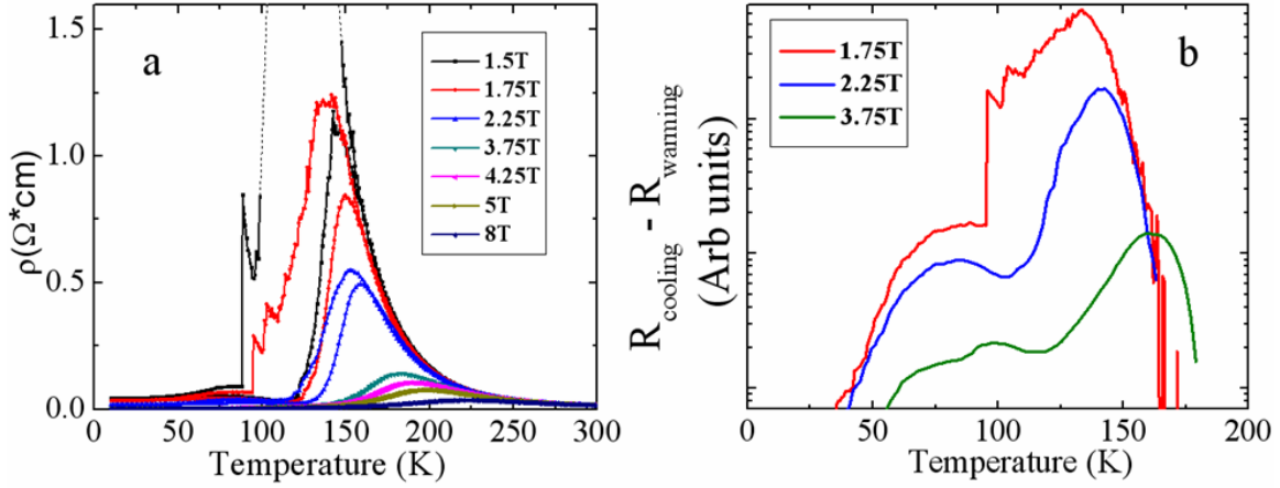
Figure 3-4: 1\ \mu\text{m} wire transport. Transport and magnetic properties of 70 nm \text{La}_{0.325}\text{Pr}_{0.3}\text{Ca}_{0.375}\text{MnO}_3 wire with \langle r_A \rangle of 1.339 Å on lattice matched SrLaGaO4 on heating and cooling. (a) Comparison of temperature dependence of resistivity in 1\ \mu\text{m} wire under various fields. The wire shows a weak reemergent, low temperature peak in \rho . (b) Differences in resistance (log) between warming and cooling curves.
