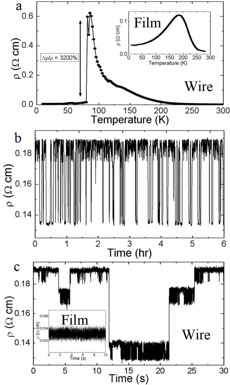
Figure 3-8: Transport measurements for 10 \mu\text{m} wire. (a) Temperature dependent resistivity plot for a 10 \mu\text{m} LPCMO wire under 0.5 \mu\text{A} constant current ( inset : Temperature vs resistivity plot of the same sample in a thin film form.) (b) Long scale, low sample frequency resistivity vs. time plot for wire held at 83 K. (c) Wire's resistivity vs. time plot at the transition temperature taken at 45 kHz ( inset : Films resistivity vs. time plot under the same conditions.)
