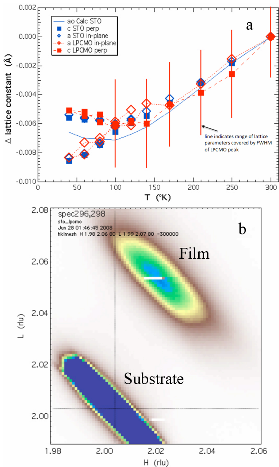
Figure 4-1: LPCMO on STO change in lattice parameters across temperature. (a) Shift in lattice parameters across temperature. (b) H-L mesh scan in reciprocal space for LPCMO on STO taken at 60 K.
