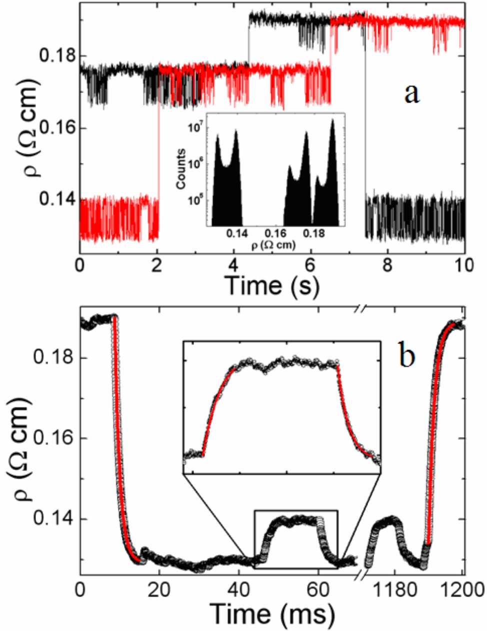
Figure 3-12: High frequency transport data on 10 μm wire held at MIT. (a) Comparison of 10 seconds worth of data taken 1 hour after the critical temperature was reached (black) and 6 hours after the critical temperature was reached (red) (inset: histogram of all data points taken over a 7 hour period.) (b) Examples of transition behaviors for both large and small fluctuations. Red lines indicate inverse exponential fits.
