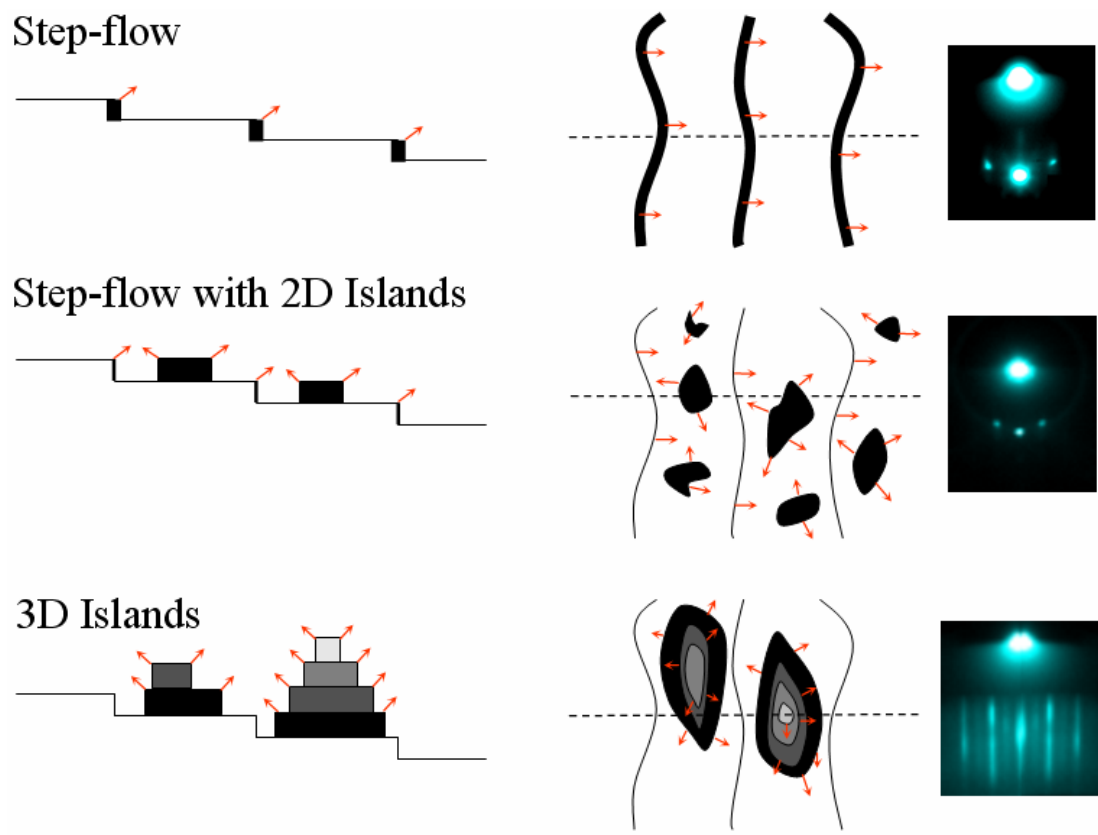
Figure 2-3: Examples of 3 growth modes and their RHEED signatures. Left column shows side view taken at dotted line in middle column. Red arrows indicate direction of growth. Right column shows typical RHEED images for each growth mode.
