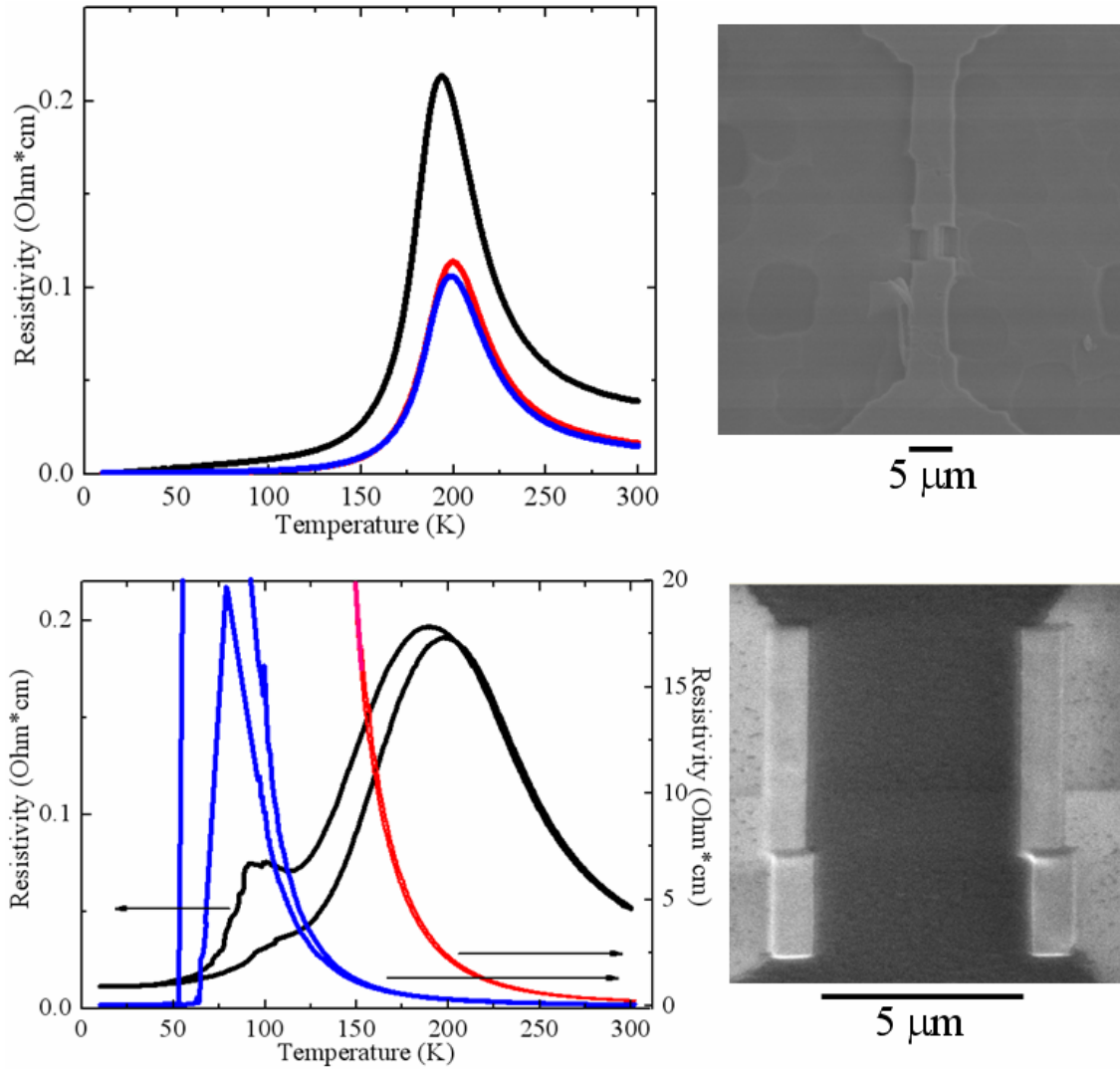
Figure 2-15: Effects of FIB etching on transport. Top: LPCMO on SLGO 5 \mu\text{m} wire (black), wire etched with FIB to 1 \mu\text{m} (red), 1 \mu\text{m} FIB etched wire after anneal (blue). Bottom: LPCMO on LAO 5 \mu\text{m} wire (black), wire edges smoothed with FIB (red), smoothed wire after anneal (blue). SEM images show wires after FIB treatment.
