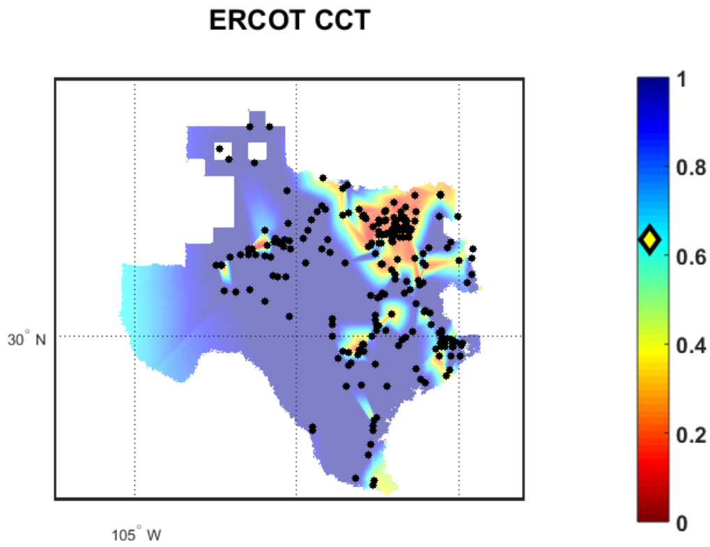
Fig. 73. 50% renewables CCT map.
