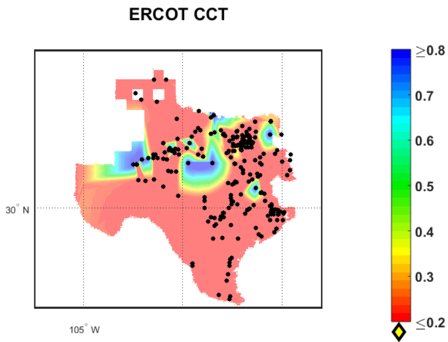
Fig. 76. 54.2% renewable CCT map.
