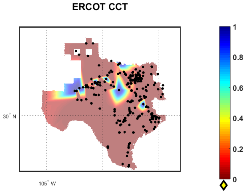
Fig. 74. 55% renewables CCT map.
