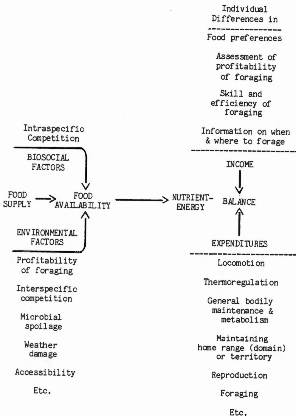
Fig. 4:3. Factors governing nutrient-energy balance, income, and expenditure.
