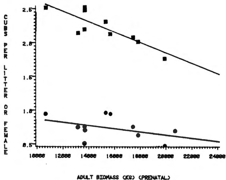
Fig. 8:3. Cub litter size and cubs per adult female regressed on adult biomass prenataally. The lower correlation for cubs per adult female reflects impacts on it by variation in whelping rate which were unrelated to adult biomass. Because whelping rate ( \#L/AdF ) averaged about 33%, mean number of cubs per adult female ( \#C/AdF ) was about 33% as high as litter size ( \#C/L ).
