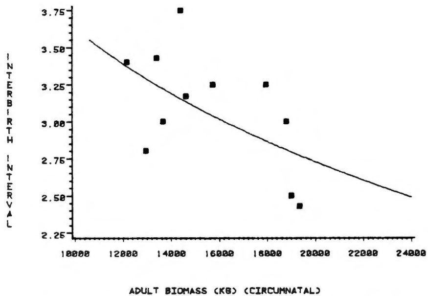
Fig. 8:6. Interbirth interval regressed on adult biomass circumnatally.
