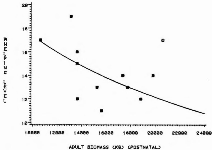
Fig. 8:4. Whelping level regressed on adult biomass postnatally.
