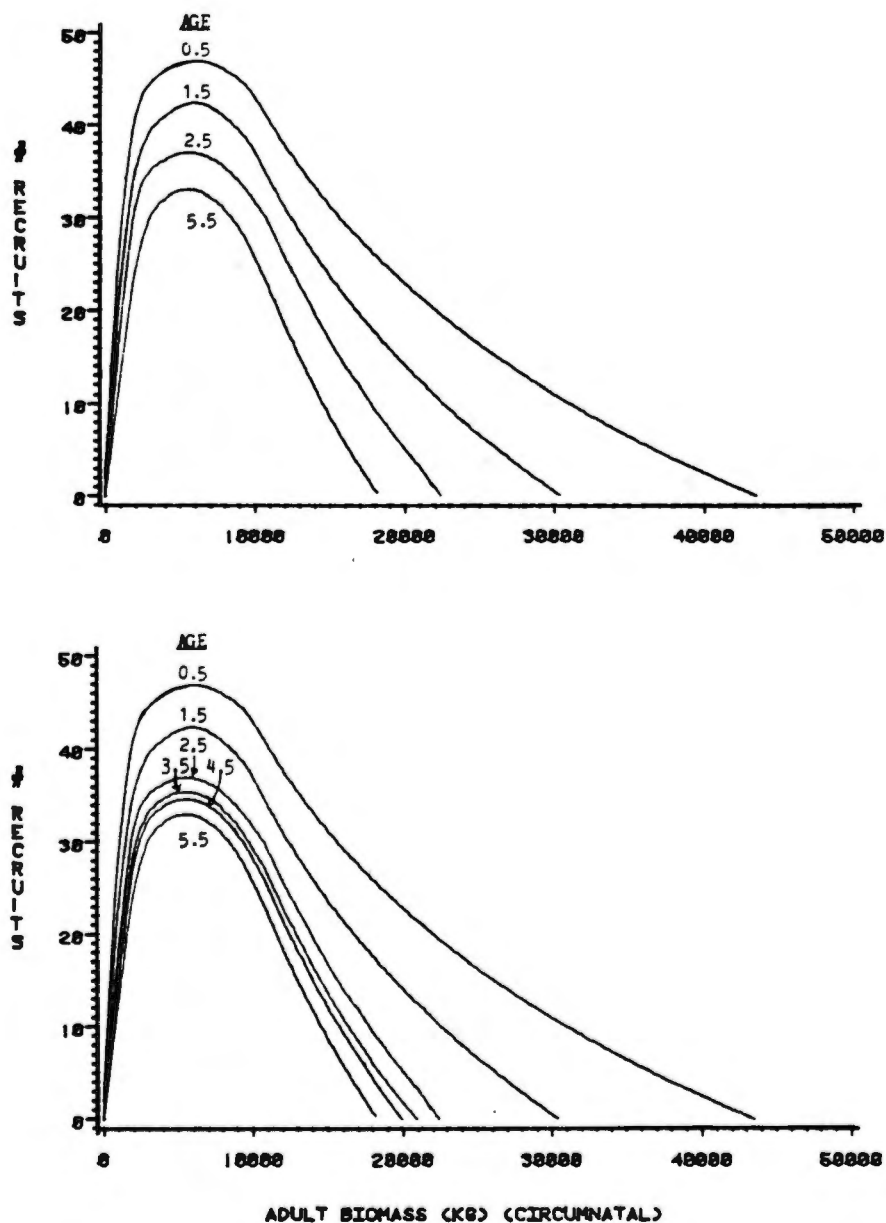
Fig. 8:14. Cohort sizes at ages 0.5-5.5 years regressed on adult biomass circumnataally. Values were extrapolated above and below the range for which data are available. (a) Cohort sizes at ages 0.5-2.5, 5.5. (Compare to Fig. 8:8). (b) Cohort sizes at ages 0.5-5.5, with interpolated values for ages 3.5 and 4.5. The plot for age 0.5 is based on the modification to assure that it has the same X-intercept as cub litter size (see text and Fig. 8:13).
