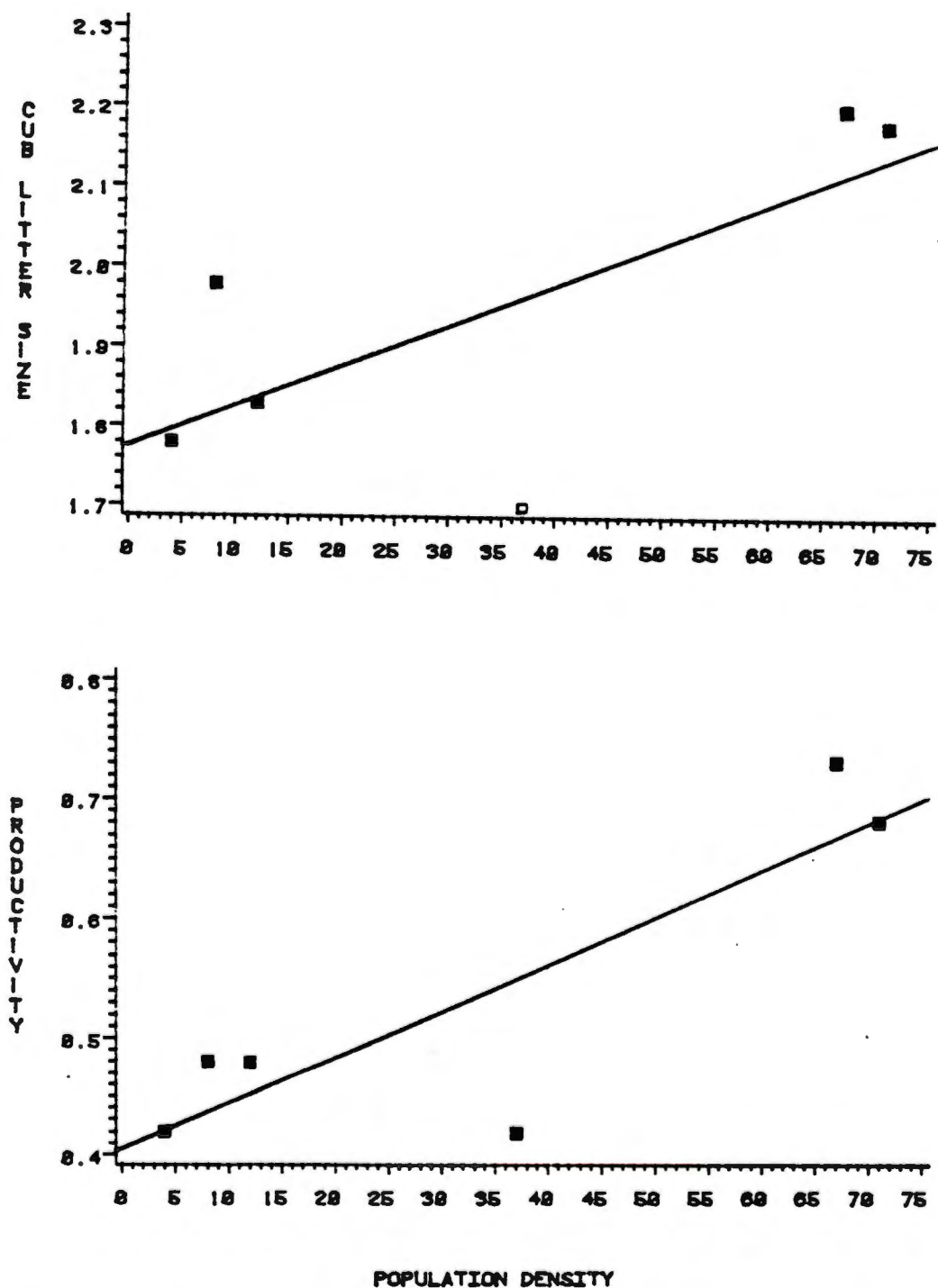
Fig. 5:2. Reproductive parameters regressed on population density in each of 6 North American grizzly populations. (■ inland, □ coastal). (Data from Tables 3:1 and 4:1; see Table 5:2 for r and P :1t).
