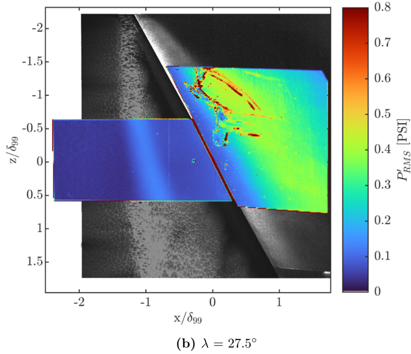
Figure 3.4: P'_{RMS} contours superimposed onto oil flow visualization images for both swept ramps.
