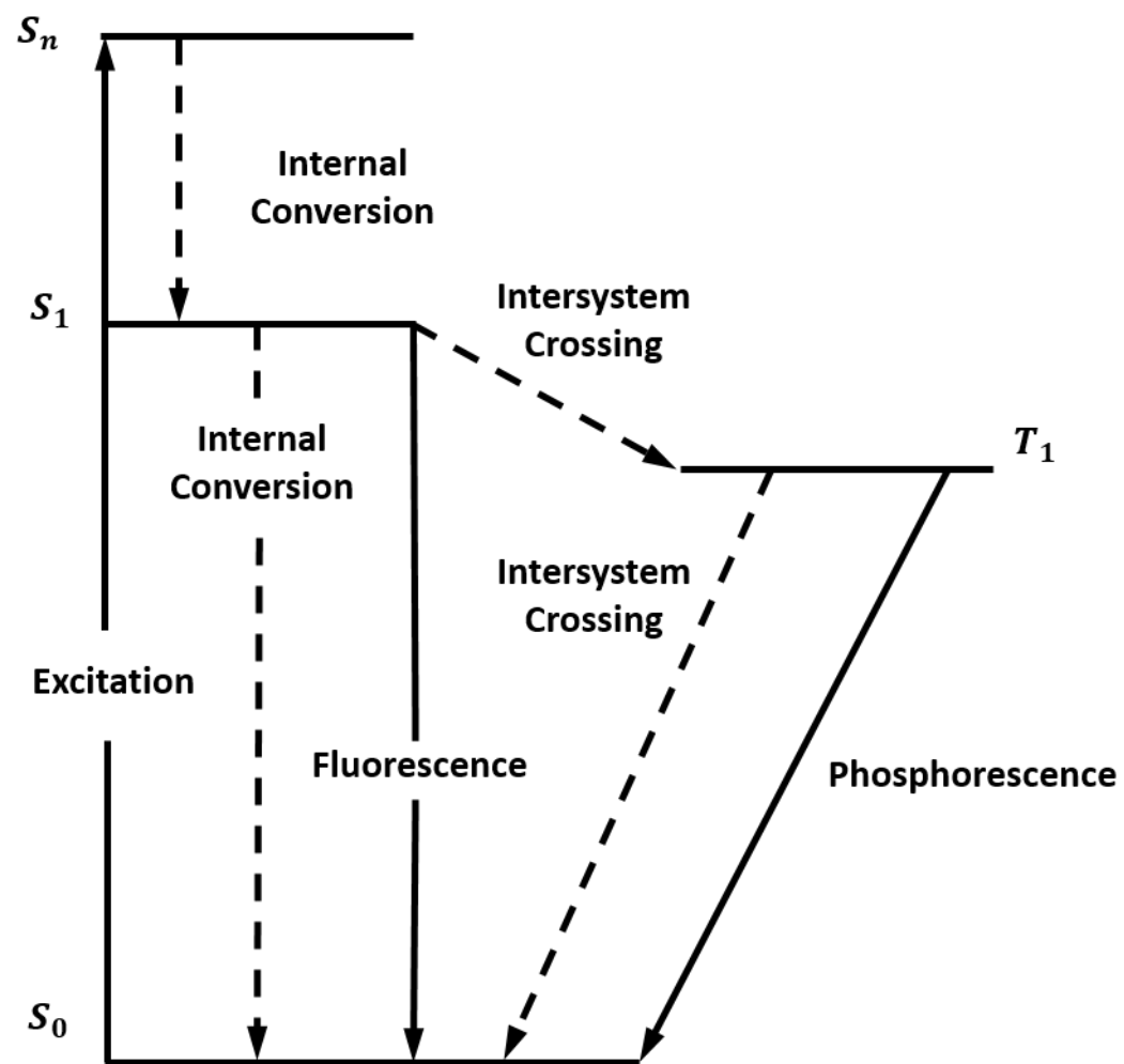
Figure 2.6: Possible energy state paths for excited luminescent molecules to return to the ground state. Adapted from Kavandi [27]
