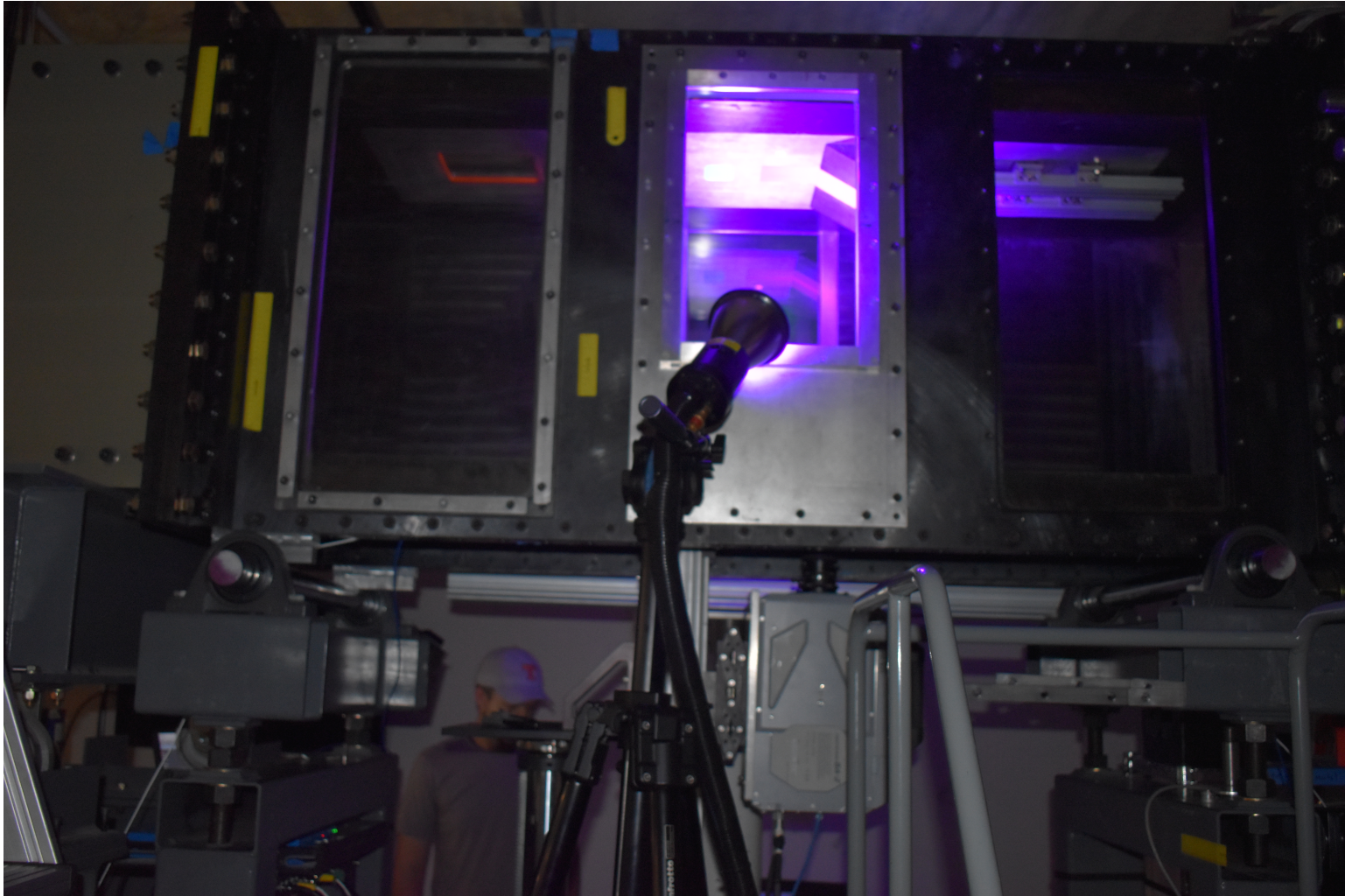
Figure 2.7: Photograph of the experimental setup for the compression ramp PSP campaign.
