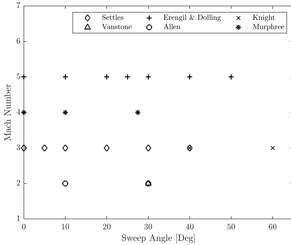
Figure 1.2: Parameter space for existing swept ramp turbulent SBLI research. The asterisk shaped markers denote the present experiment.
