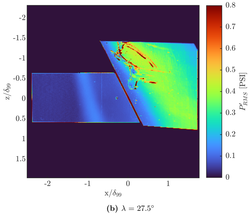
Figure 3.3: P'_{RMS} (pressure fluctuation) contours obtained over 2400 frames from the steady-state conditions run for both swept ramps.
