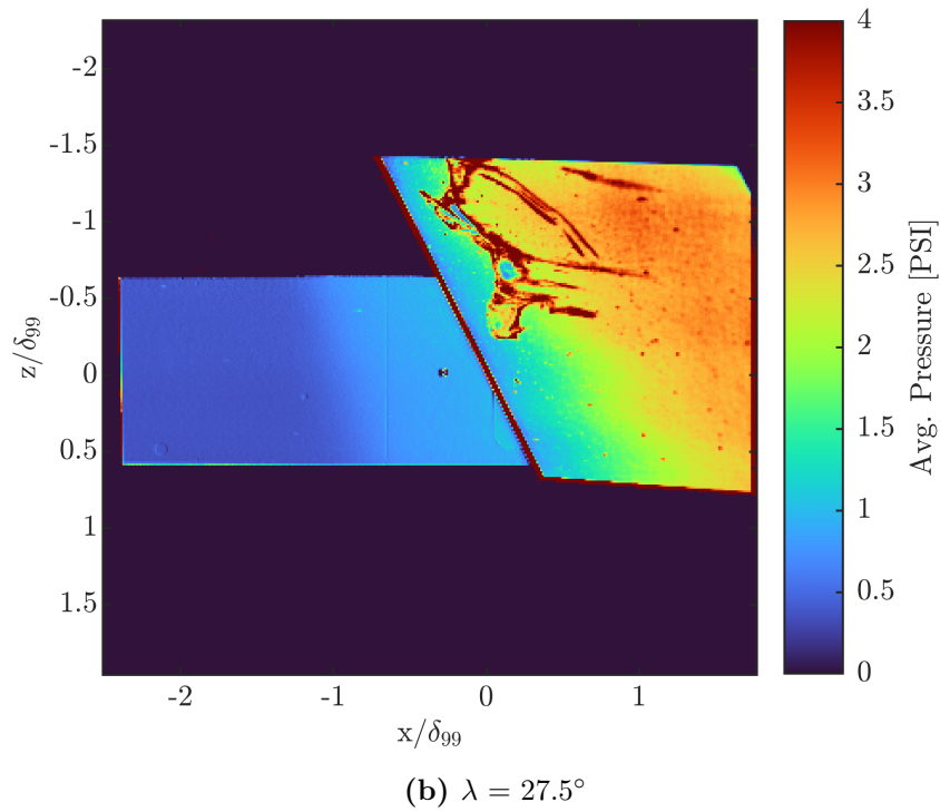
Figure 3.2: Average surface pressure distribution obtained over 2400 frames from the steady-state conditions run for both swept ramps.
