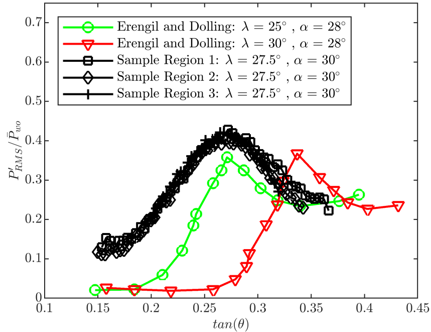
(b) Normalized pressure fluctuations from the three sample locations compared to prior results of Erenkil and Dolling [12]
