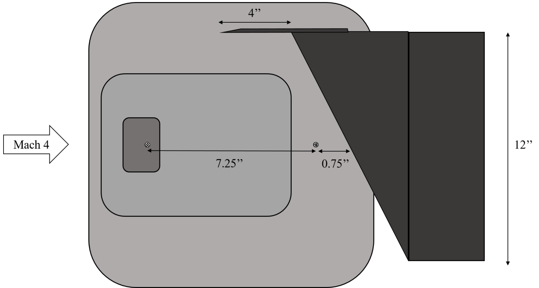
Figure 2.4: Schematic of the floor plate, ramp, and Kulite locations.
