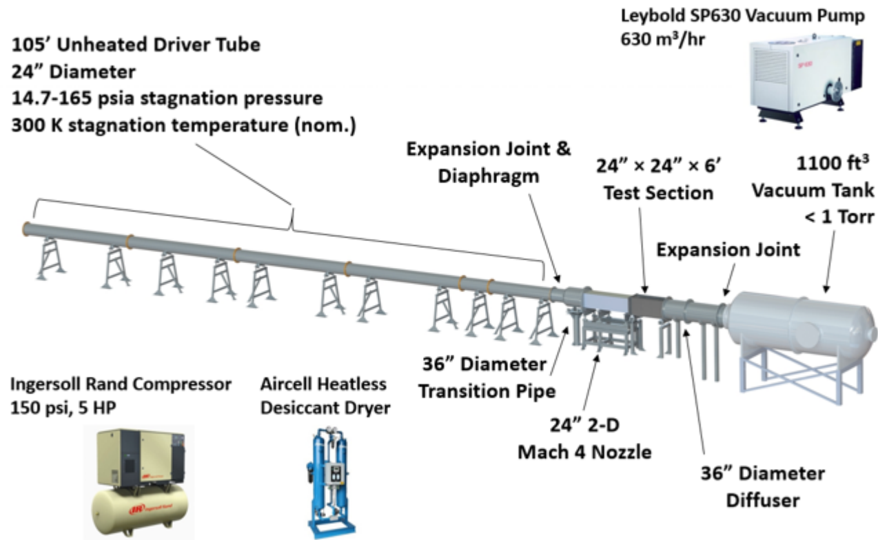
Figure 2.1: Schematic of the UTSI Mach 4 Ludwieg Tube and ancillary equipment [33]
