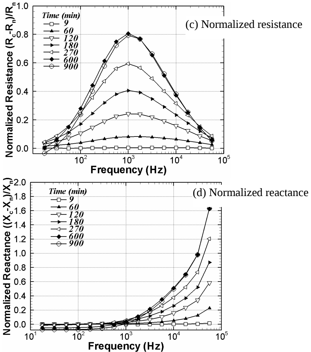
Figure 4.4: Continued. Representative surface plots of normalized resistance (a) and reactance (b) attach scans of PPEACs on a 250 \mu\text{m} diameter ITO electrode as a function of frequency and time following a confluent inoculation density. The surfaces consist of approximately 300 frequency spectrum scans that were sampled at three minute time intervals. Plots (c) and (d) show normalized resistance and reactance, respectively for PPEACs' attachment at t = 9 min, 60 min, 120 min, 180 min, 270 min, 600 min, and 900 min. (c) The normalized resistance as a function of frequency shows a monotonic increase with time up to approximately 600 minutes at which point saturation occurs. (d) The corresponding normalized reactance also shows an increase with time during the cellular attachment phase.
