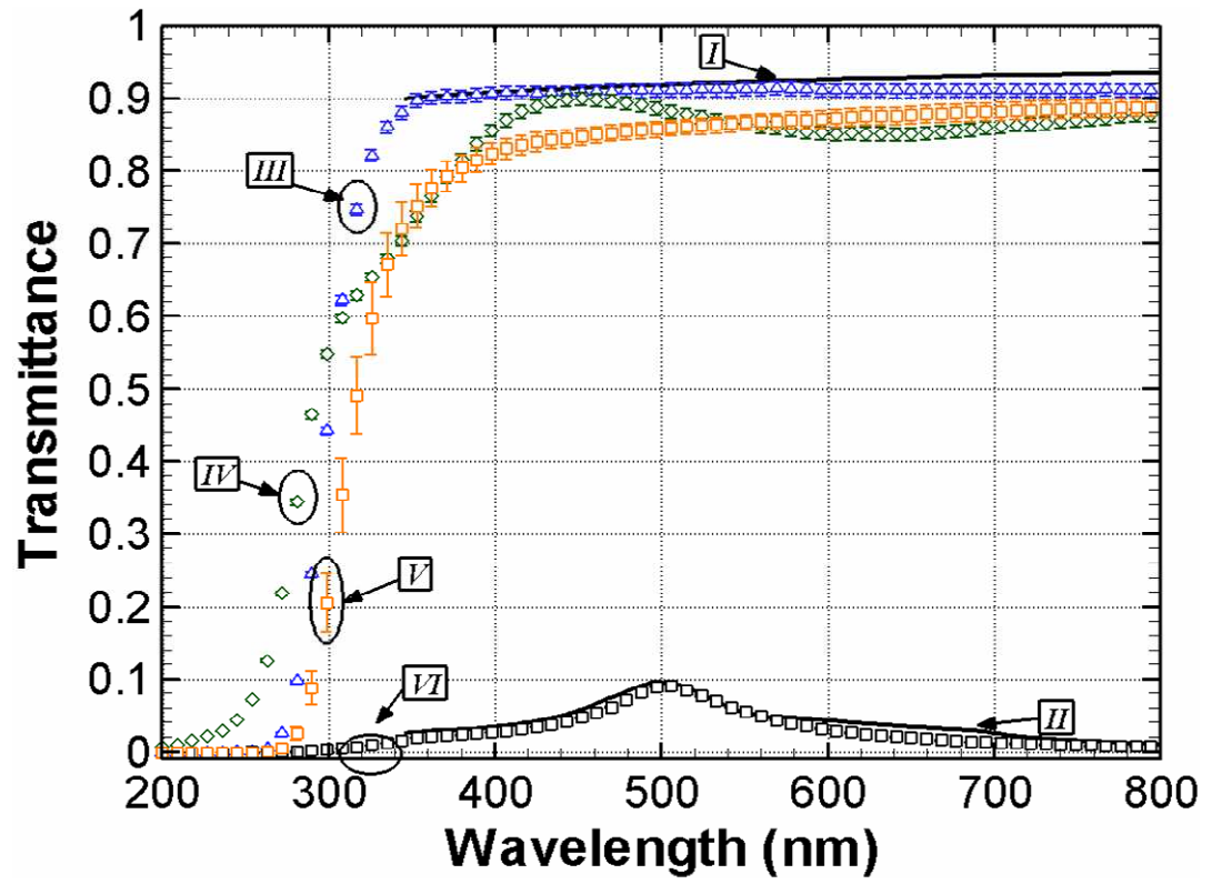
Figure 3.5: Normal transmittance, calculated for bare slideglass (I) and Au (47.5 nm)/Ti (2.5 nm)-coated slideglass (II), and measured for bare slideglass (III), 100-nm ITO-coated slideglass (IV), 500-nm ITO-coated slideglass (V), and Au/Ti-coated slideglass (VI).
