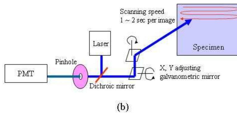
Figure 1.1: Principle of Confocal Microscopy using a pinhole as a spatial filter (a), and a schematic illustration of galvanometric scanning to conform to a full-field image (b).
