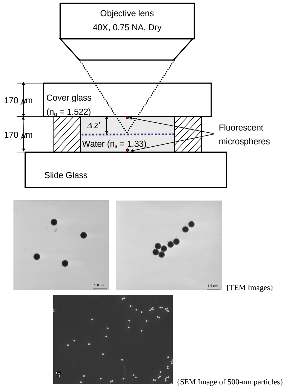
Figure 1.11: Schematic of a test specimen for measuring both symmetric and asymmetric PSFs in the OSSM using 500±16 nm nominal diameter nanoparticles.
