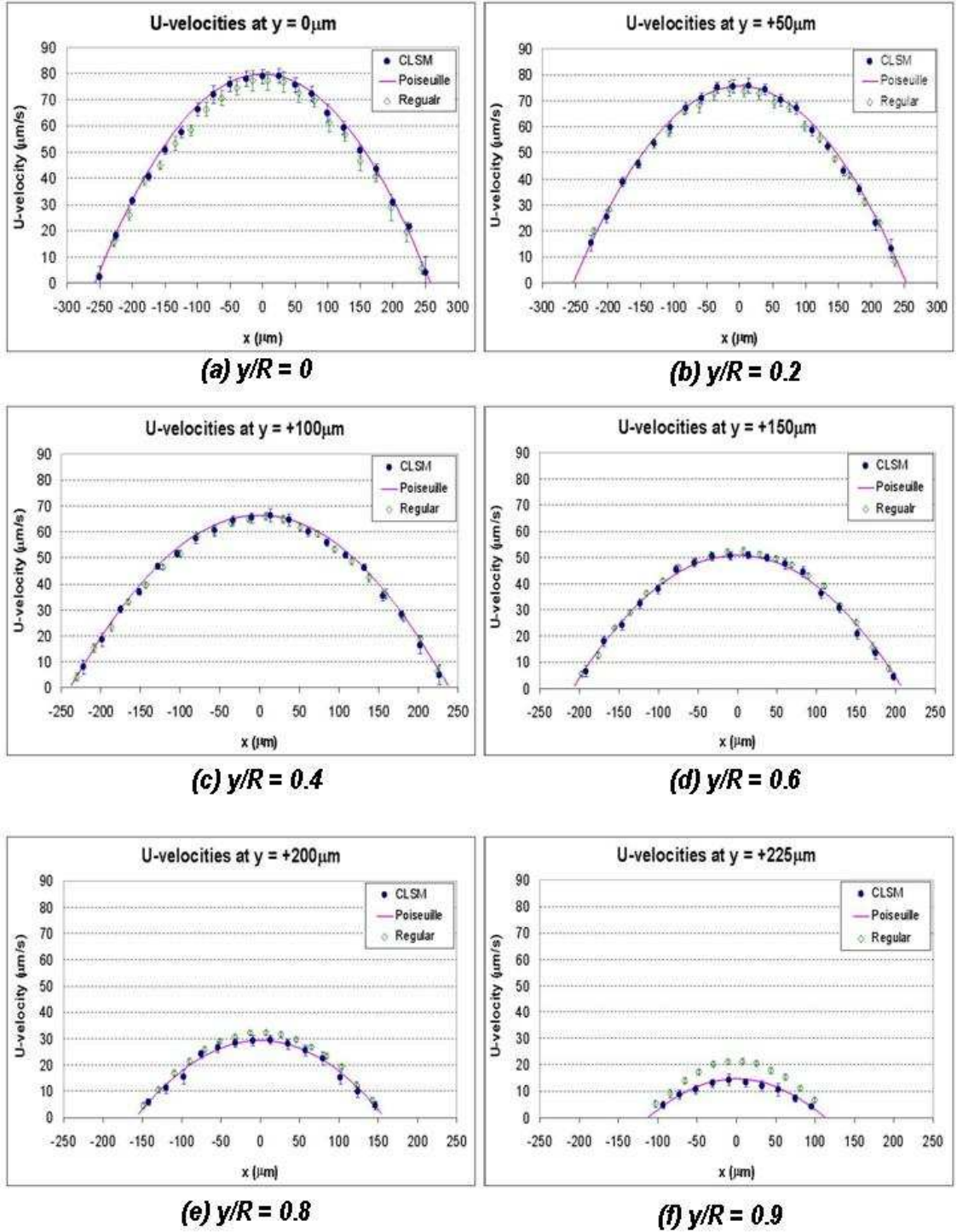
Figure 1.7: Comparison of the velocity profiles measured by the CLSM micro-PIV and by the conventional micro-PIV at different y-planes of the 516-μm ID microtube.
