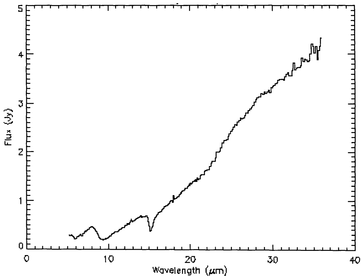
Figure 1. A sample of a Class I spectrum. Notice the strong CO 2 ice feature at 15.2μm, the broad amorphous silicate feature around 9.7μm, and the smaller H 2 O and CH 3 OH features at 6.0 and 6.8μm, respectively.
