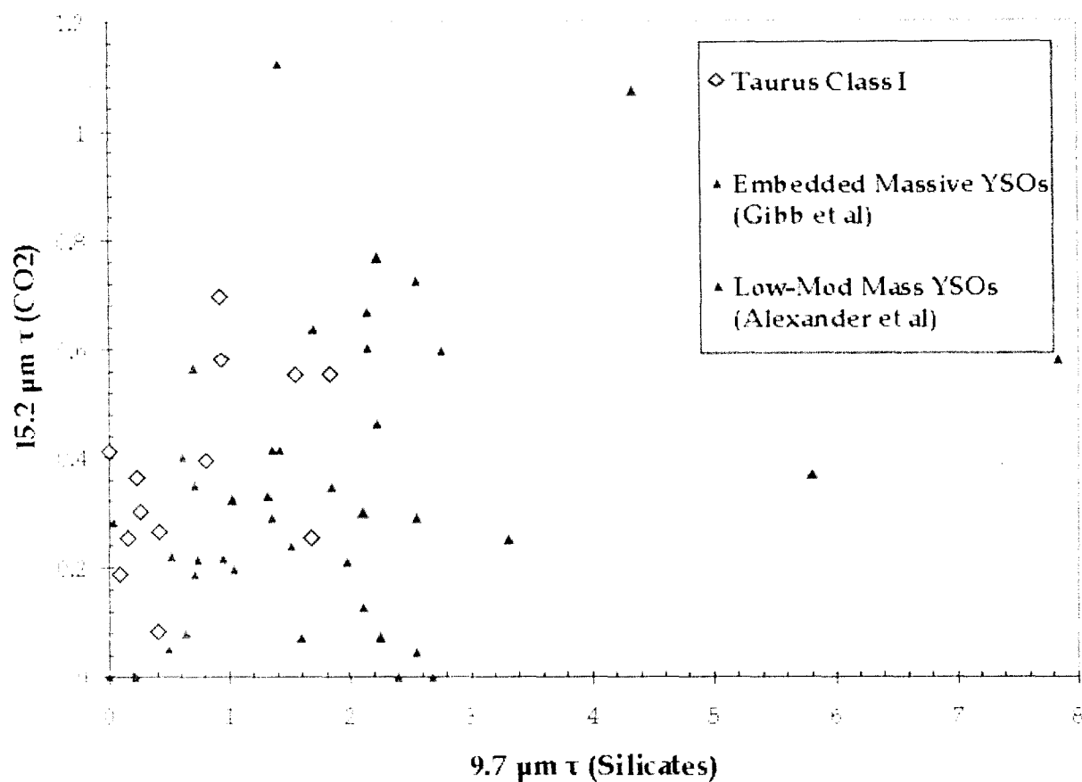
Figure 4. A plot of 9.7 \mu\text{m} silicate optical depth versus 15.2 \mu\text{m} CO 2 ice optical depth. Notice the lack of correlation in any of the studies.
