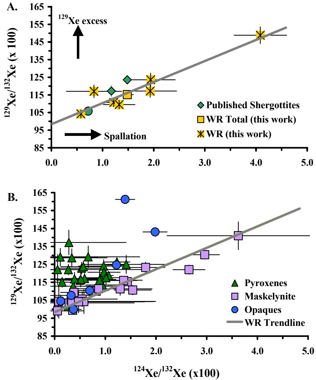
Figure III- 3. ^{129}\text{Xe}/^{132}\text{Xe} ratio versus ^{124}\text{Xe}/^{132}\text{Xe} ratio plot of published whole rock data (Ott, 1988; Terribilini, 2000). The whole rock observed in this experiment defines a trend line that is illustrated in both plots (A and B). In plot B, the pyroxene-dominate separates reflect a low ^{124}\text{Xe}/^{132}\text{Xe} ratio due to the lack of target elements for spallation. The opaque-dominate separates show a steep, positive correlation between spallation and excess ^{129}\text{Xe}/^{132}\text{Xe} representing a concentration of atmospheric xenon in the opaque grains. The maskelynite correlation illustrates that maskelynite grains define the whole rock trend.
