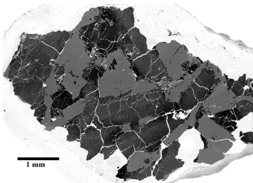
Figure III- 2. Inverted backscatter image of a thick section of Shergotty meteorite showing large pyroxene crystals separated by grey lathes of maskelynite.
