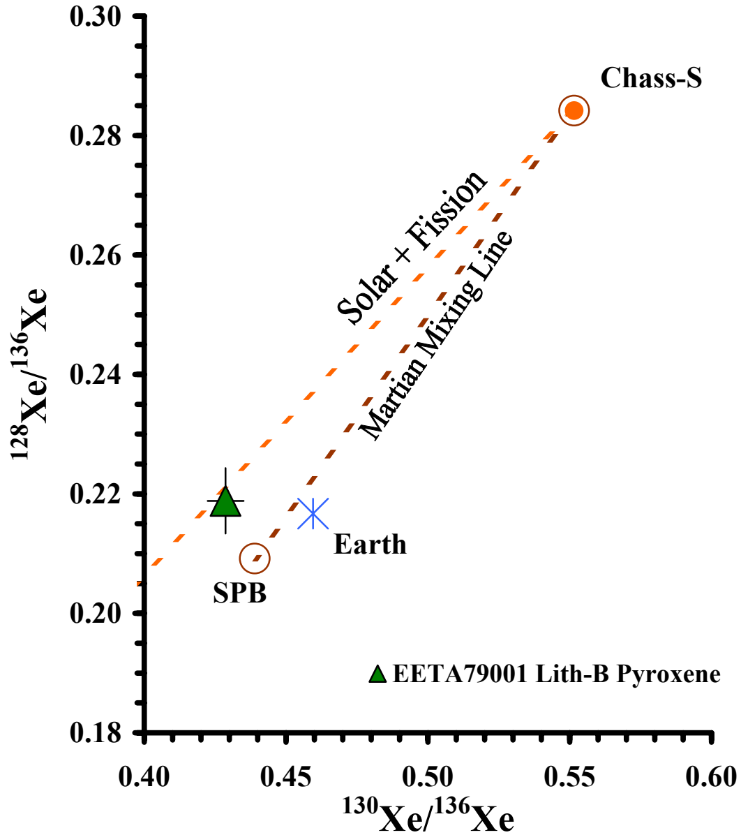
Figure IV-3. ^{128}\text{Xe}/^{136}\text{Xe} versus ^{130}\text{Xe}/^{136}\text{Xe} graph of the average of spallation corrected pyroxene data. The interior component defined by the pyroxene-dominant separates lie on the line illustrating the addition of fission-xenon to solar xenon, as measured in Chassigny. Also drawn is the mixing line between Martian interior and Martian atmosphere. The location of the pyroxene data illustrates that the interior component is a product of solar with a fission contribution and is of Martian origin.
