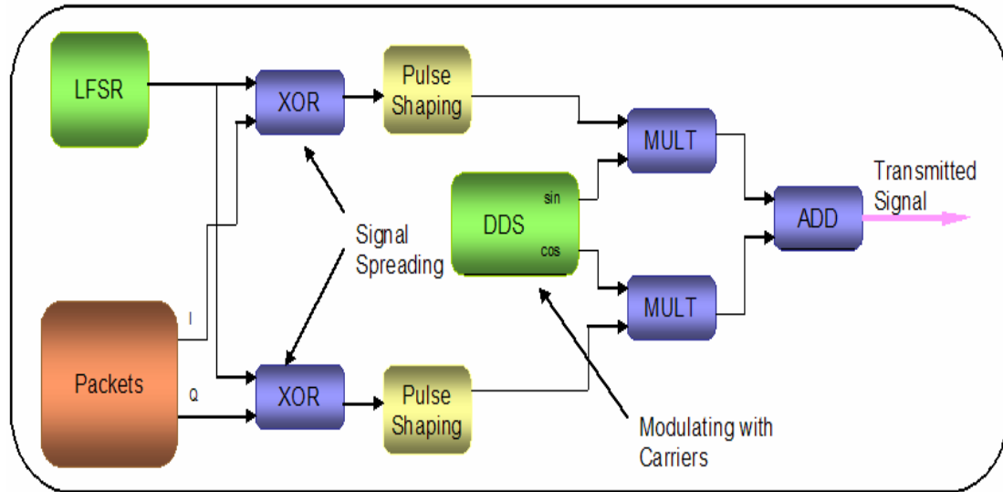
Figure 3.10: QPSK Transmitter
