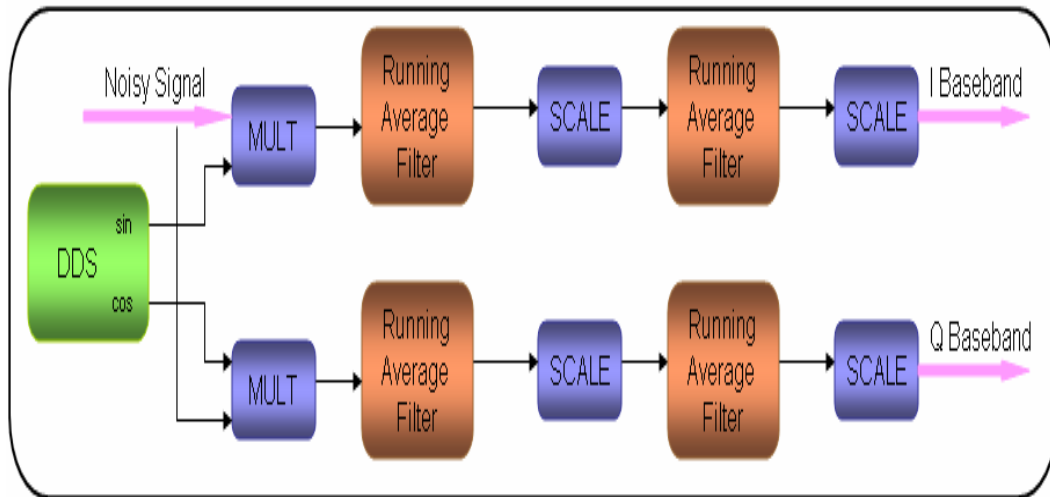
Figure 3.34: Digital Down Conversion Block
