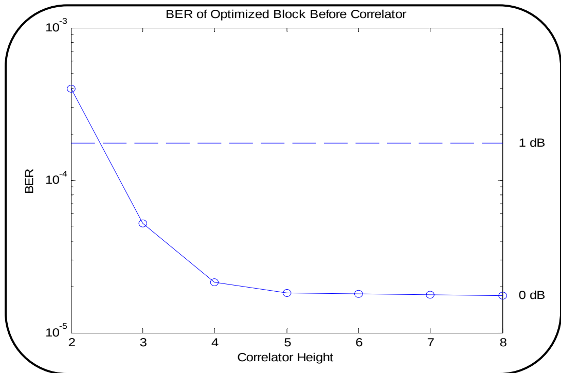
Figure 6.5: BER versus Correlator Datapath Height
