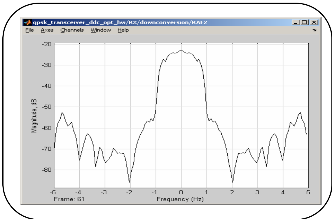
Figure 3.43: Magnitude Response of Signal after Filter 2
