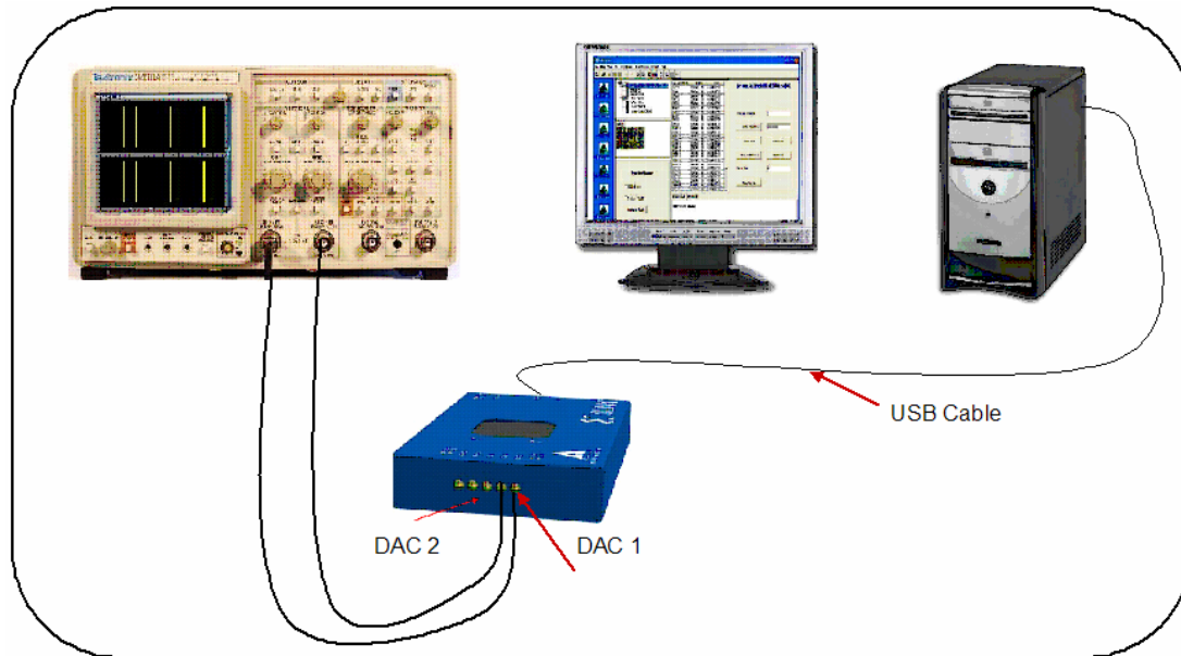
Figure 5.12: Overall Hardware Setup
