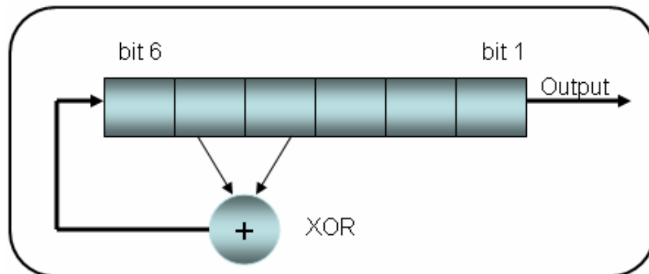
Figure 3.16: 63-Length PN Generator
