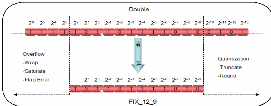
Figure 4.3: Quantization and Overflow Example
