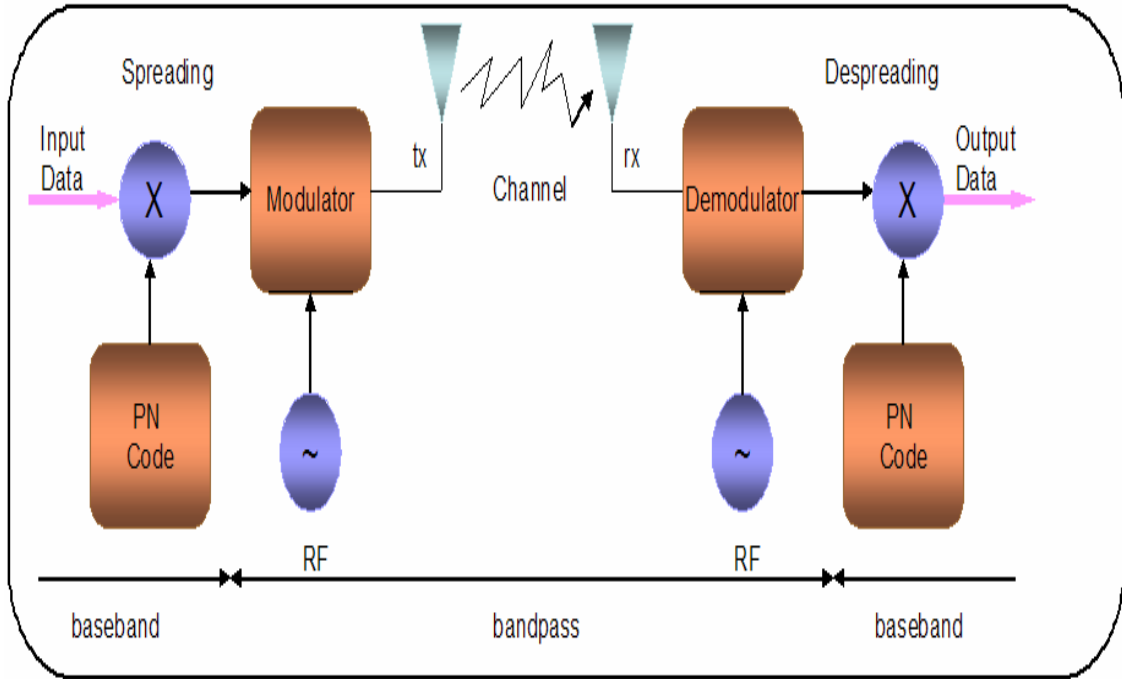
Figure 3.1: Spread Spectrum Model
