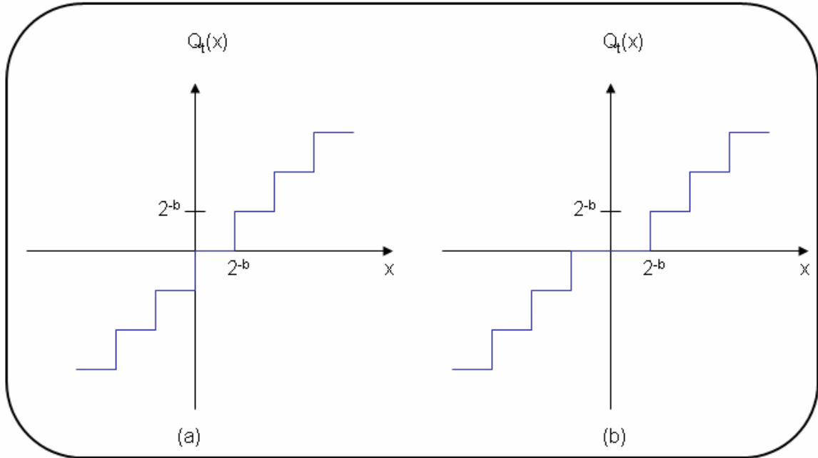
Figure 6. 8: Effects of Quantization for (a) two's complement representaion and (b) sign-magnitude representation
