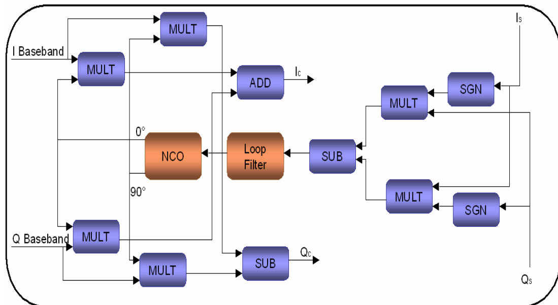
Figure 3.47: Costas Loop
