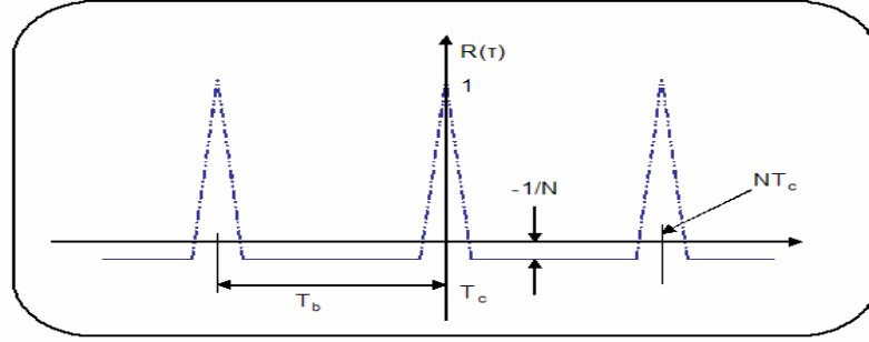
Figure 3.7: Autocorrelation of PN Code
