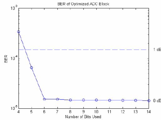
Figure 2. BER versus ADC resolution
