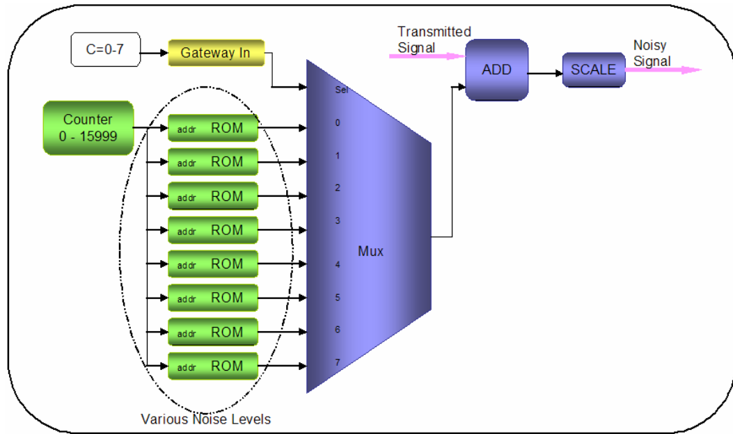
Figure 3.32: Design for Implementing Various Noise Levels
