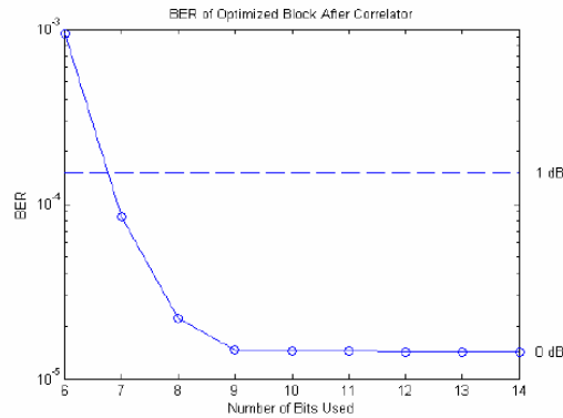
Figure 6. BER versus correlator datapath size
