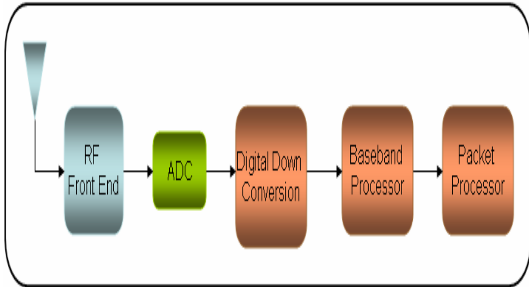
Figure 3.33: QPSK Receiver
