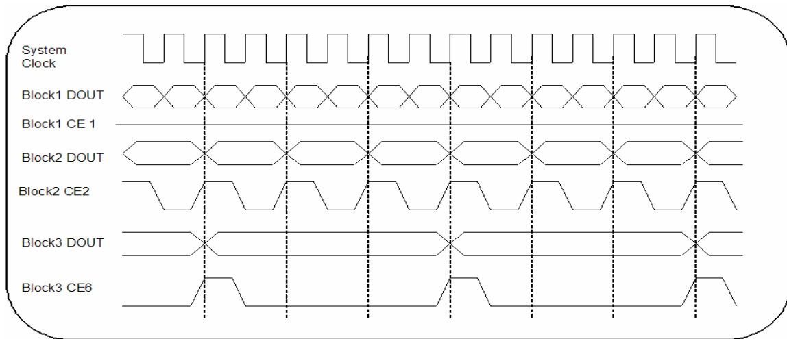
Figure 4.6: Clock Enable Behavior Example
