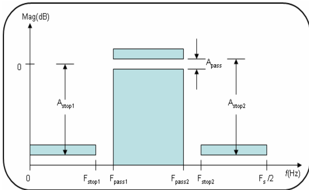
Figure 3.24: Bandpass Filter Specifications
