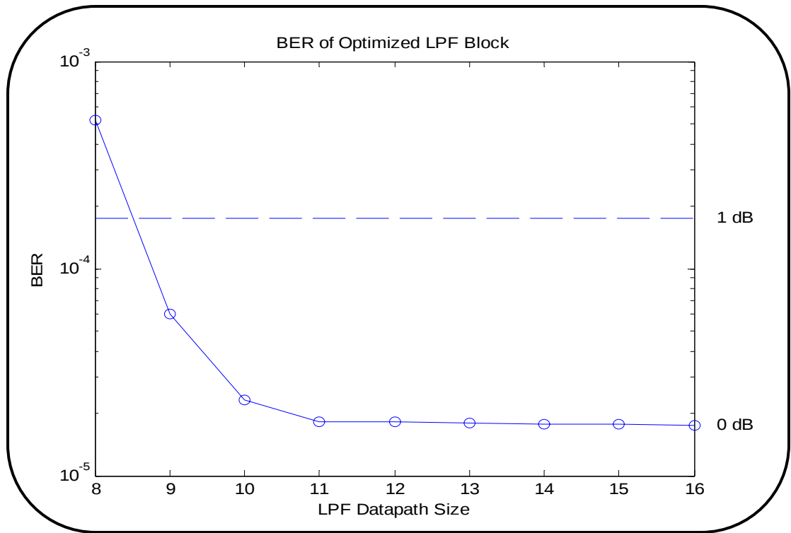
Figure 6.4: BER versus LPF Datapath Size
