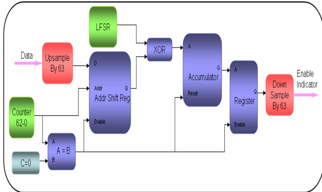
Figure 3.63: DDW Block within the Packet Processor
