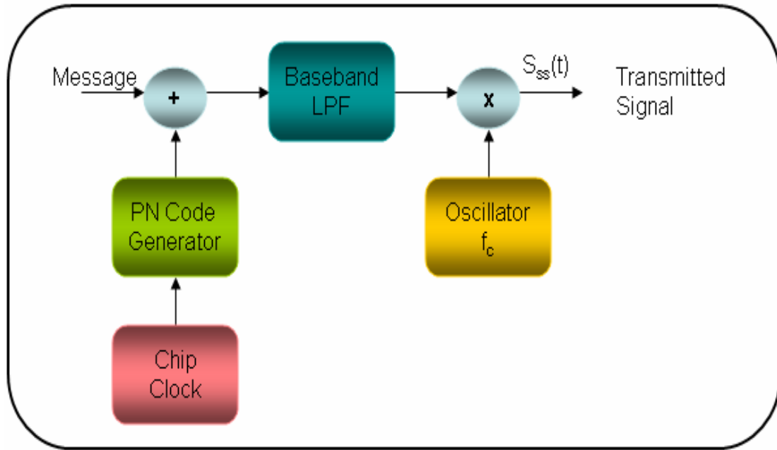
Figure 3.4: Design of Transmitter
