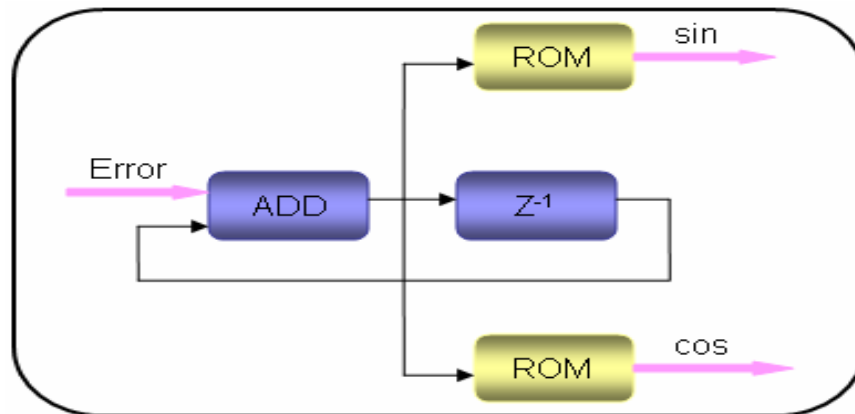
Figure 3.48: NCO
