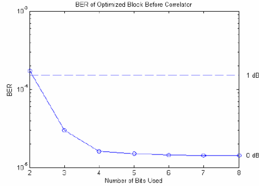
Figure 5. BER versus correlator height
