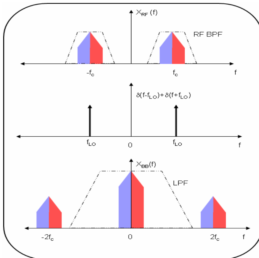
Figure 3.35: Frequency Domain Analysis for Down Conversion
