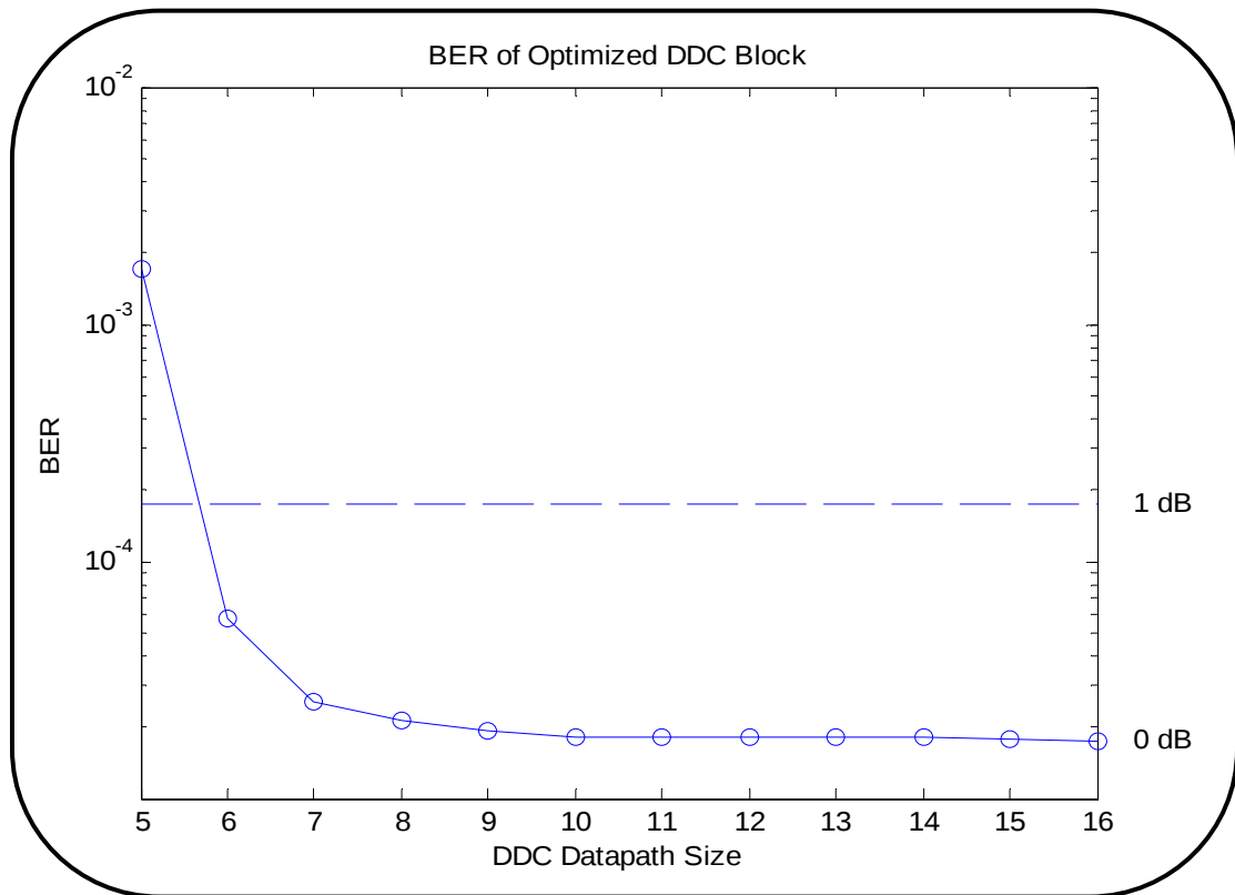
Figure 6.3: BER versus DDC Datapath Size
