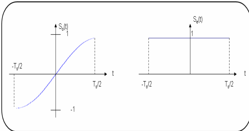
Figure 3.20: S_o and S_e Pulse Shape
