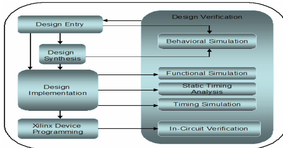
Figure 5.8: System Generator Based Design Flow
