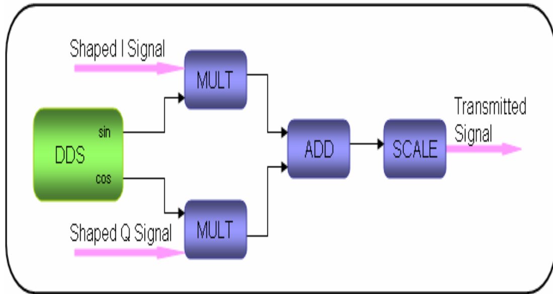
Figure 3.22: Modulation
