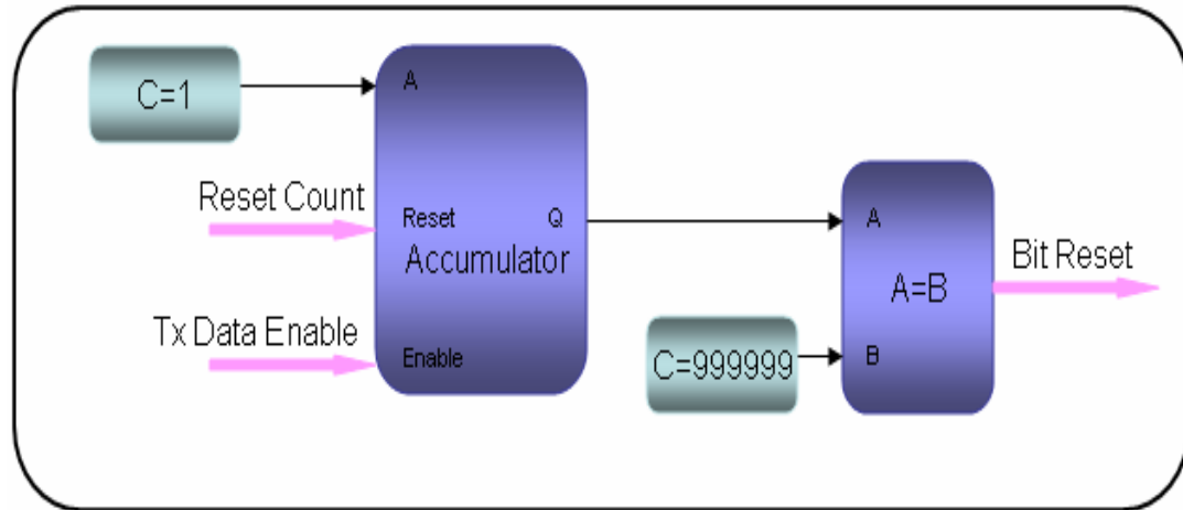
Figure 3.66: Bit Counter
