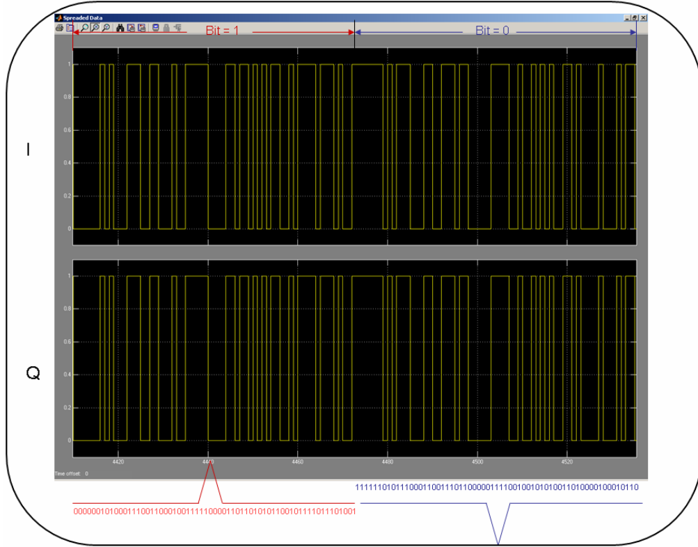
Figure 3.18: Data after Spreading in Simulation (for 2 bits)
