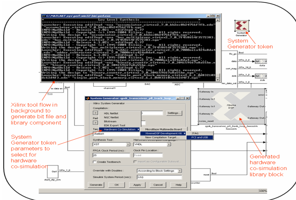
Figure 4.9: HIL Emulation
