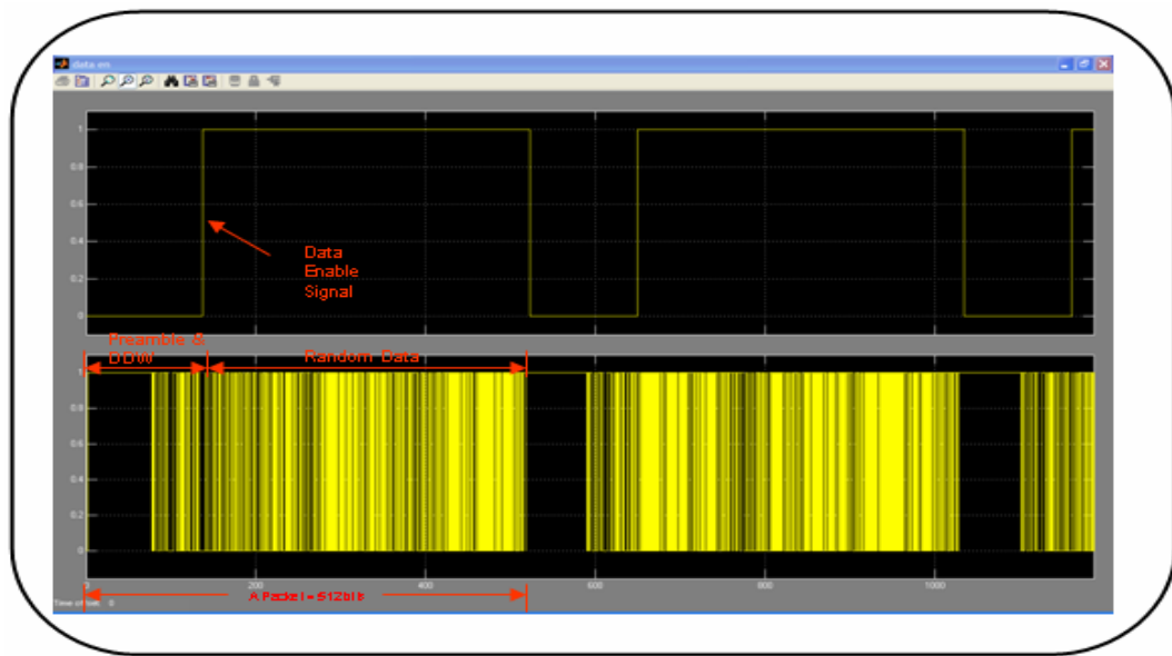
Figure 3.65: Data Enable Signal and Packeted Data
