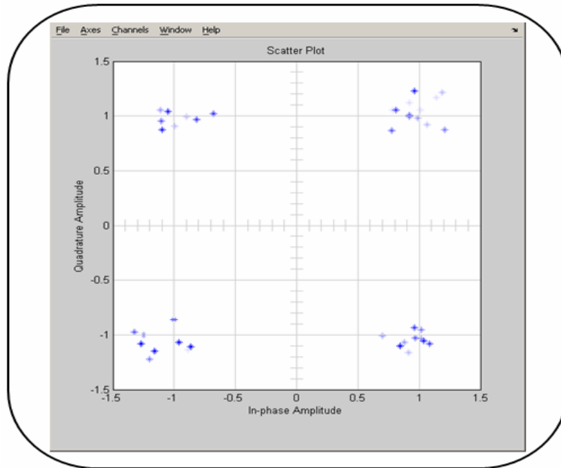
Figure 3.61: QPSK Phase Values
