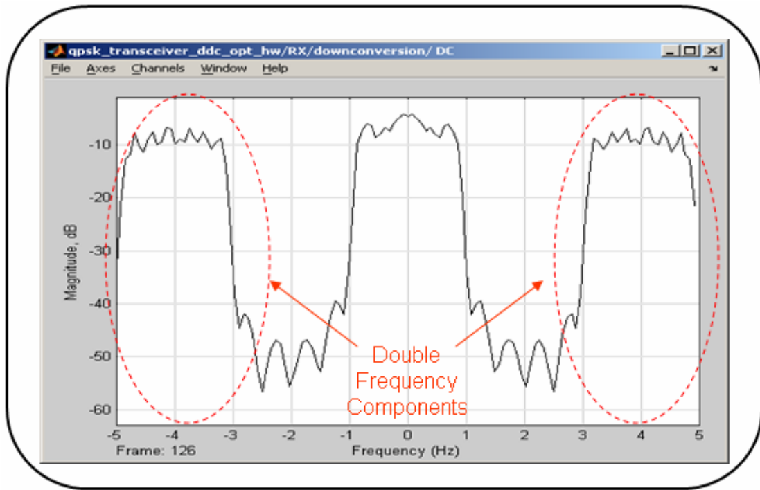
Figure 3 39: Magnitude Response after Down Conversion
