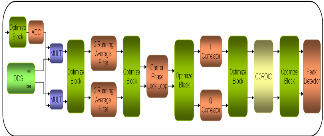
Figure 3.68: Location of Optimization Points in Receiver
