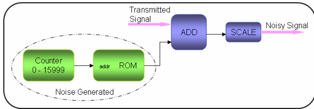
Figure 3.29: Design of Channel
