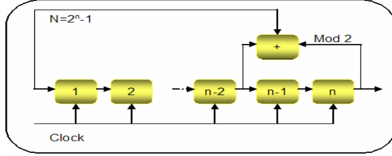
Figure 3.6: PN Generator Model
