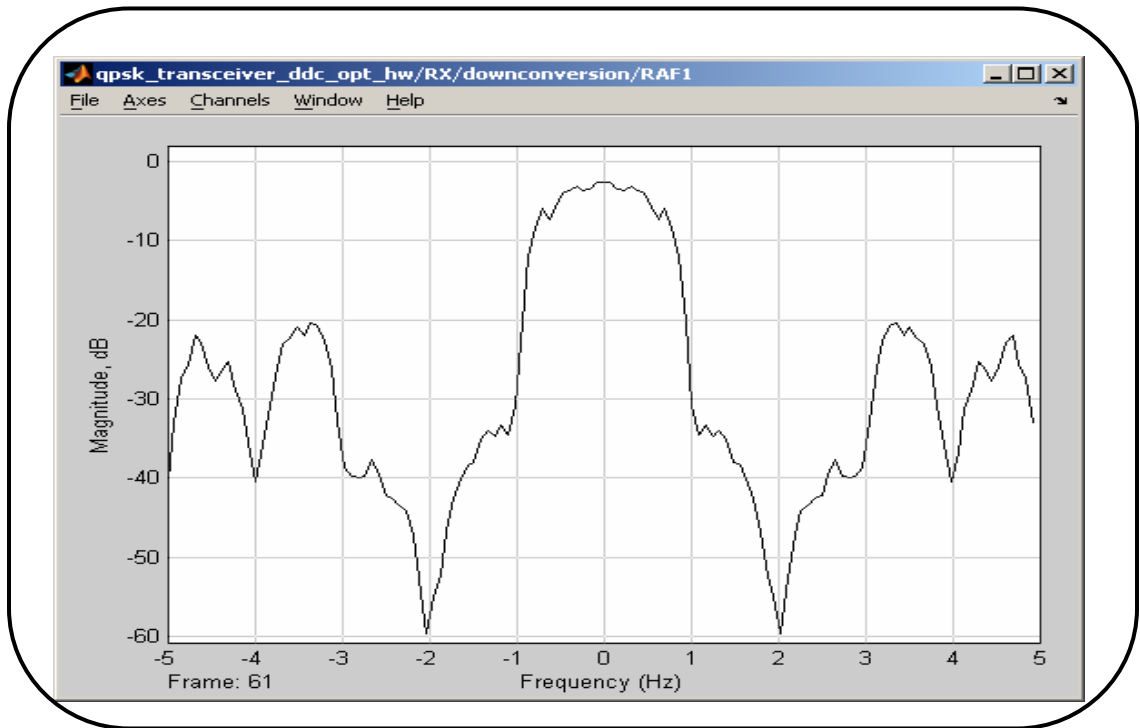
Figure 3.41: Magnitude Response of Signal after Filter 1
