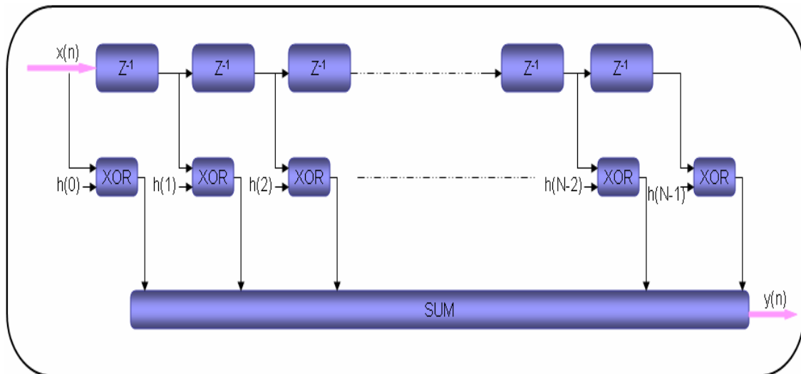
Figure 3.52: FIR Filter
