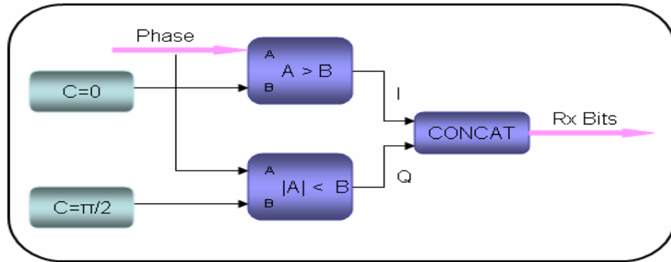
Figure 3.62: Phase Decoder Model
