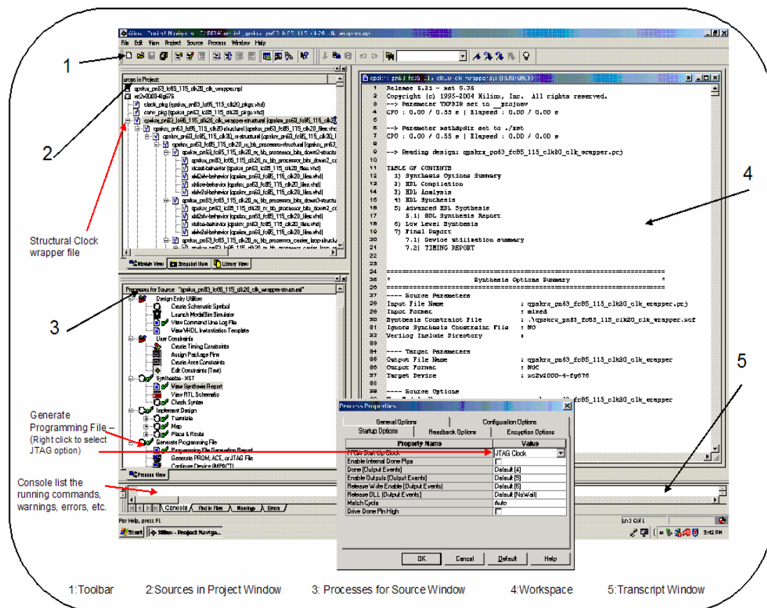
Figure 5.9: Project Navigator Window
