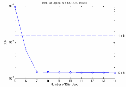
Figure 7. BER versus rec-to-pol datapath size
