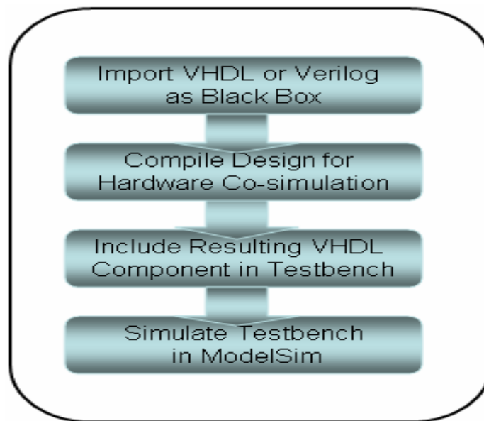
Figure 4.8: Required Steps for HDL Co-simulation through ModelSim
