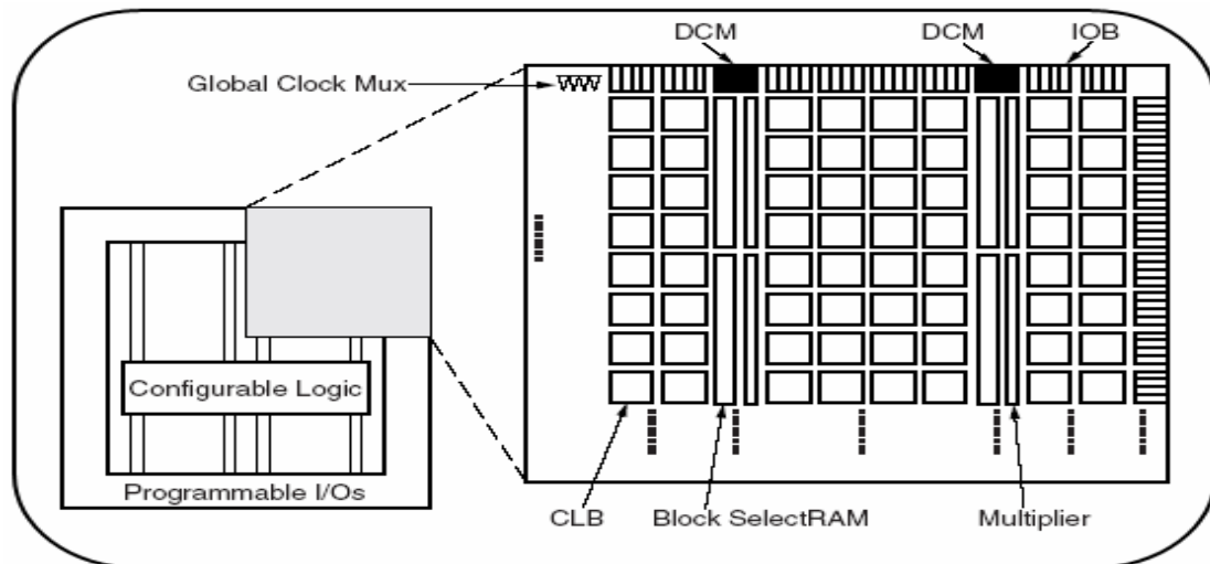
Figure 5.5: Virtex-II Architecture Overview
