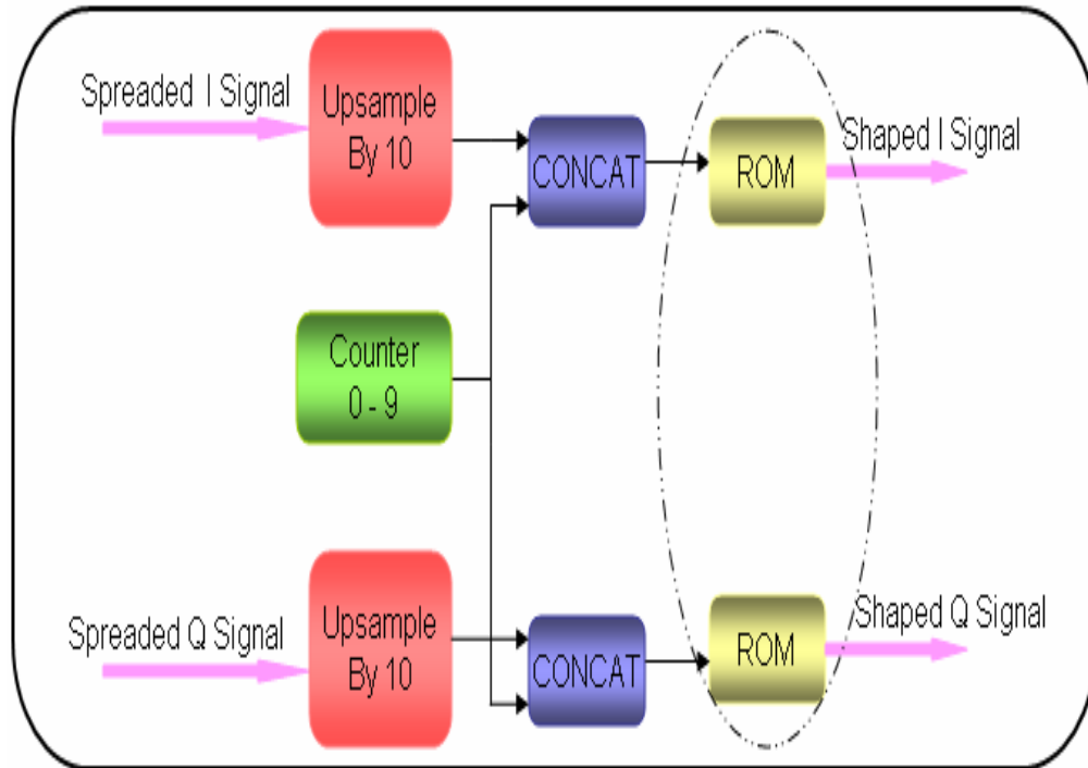
Figure 3.19: Pulse Shaping Model
