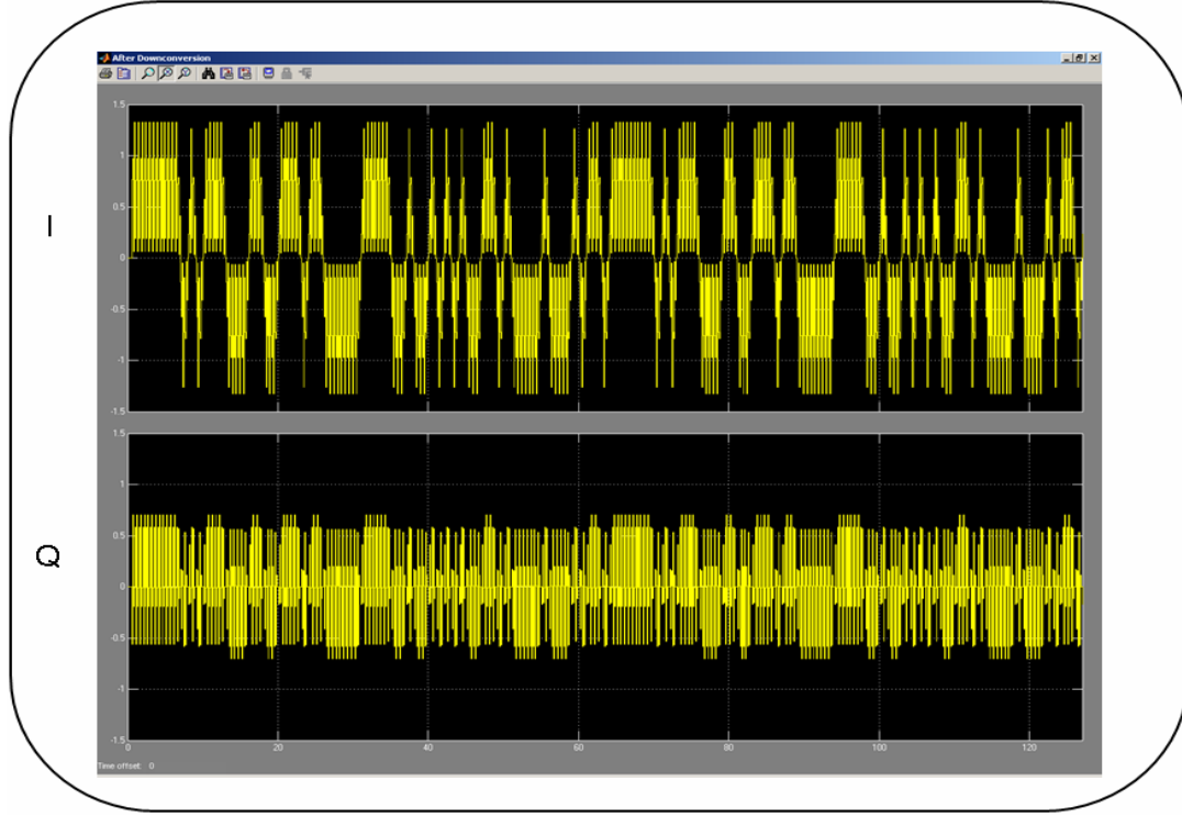
Figure 3.36: Signal after Down Conversion
