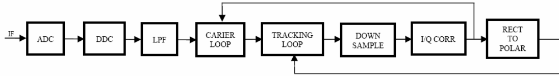
Figure 1. DSSS receiver block diagram
