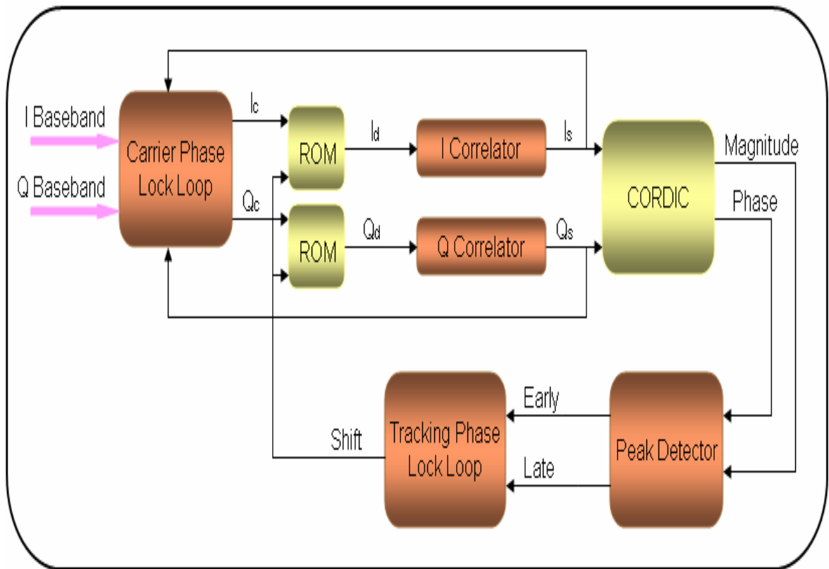
Figure 3.46: Baseband Processor
