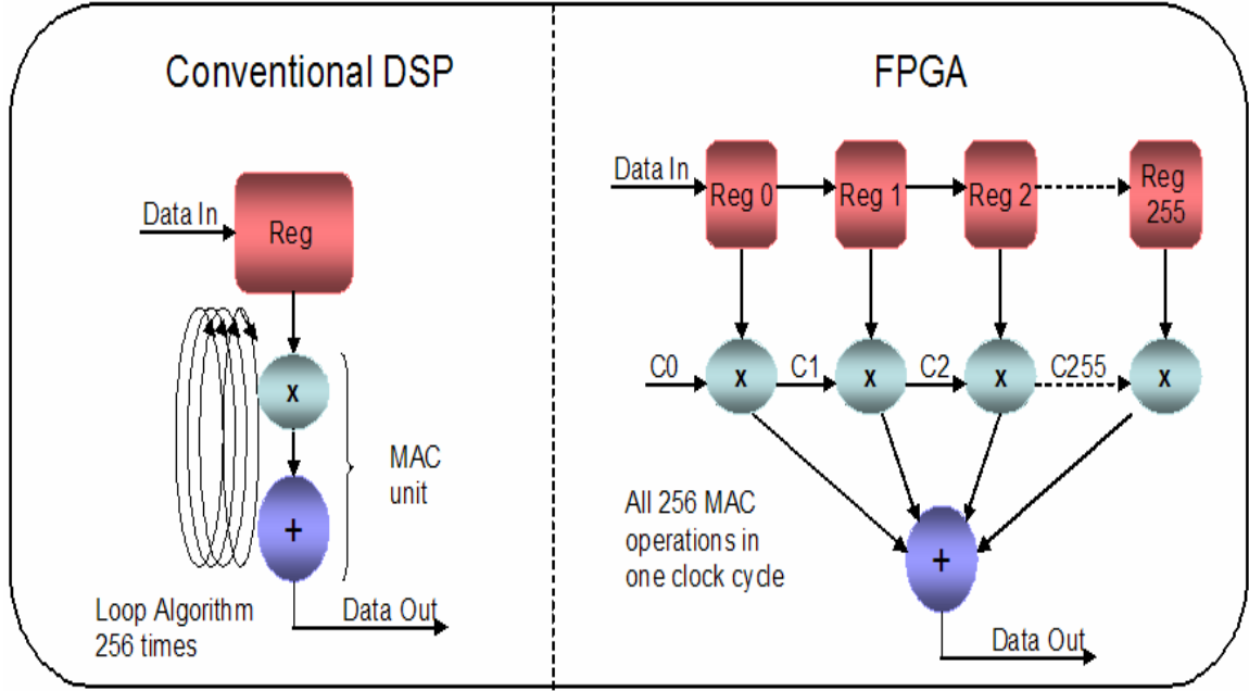
Figure 5.1: Architecture Difference in MACs between DSPs and FPGAs
