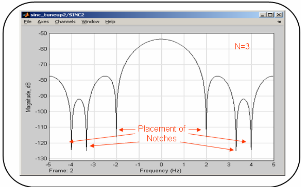
Figure 3.42: Magnitude Response of Filter 1 and 2
