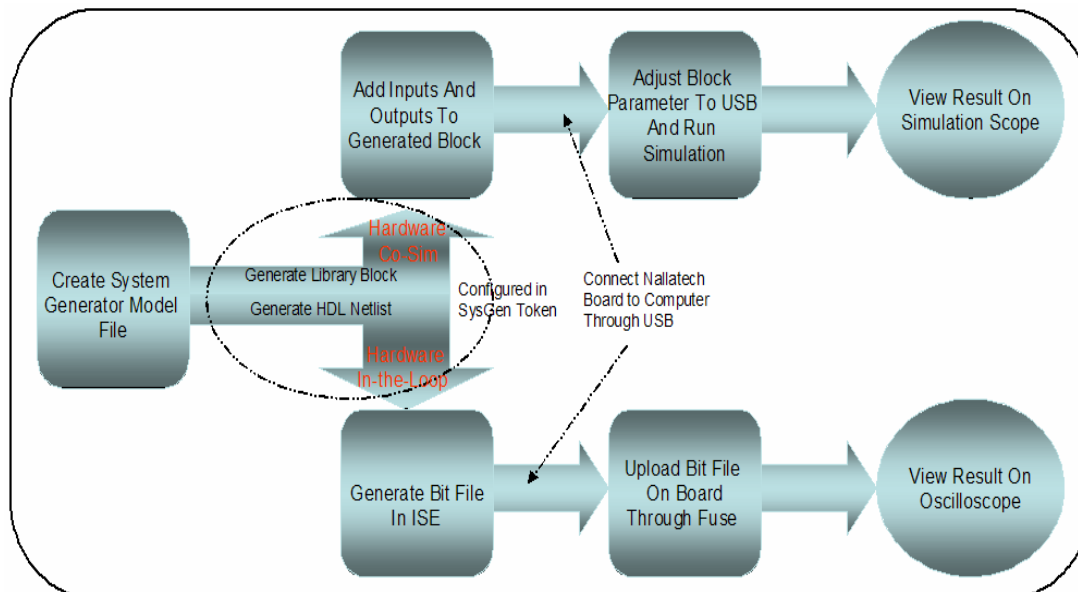
Figure 4.10: Steps for HIL and Hardware Co-Simulation
