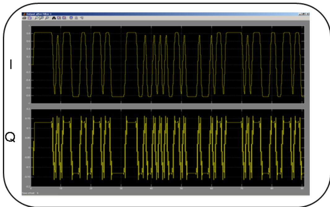
Figure 3.44: Signal after Running Average Filter 1
