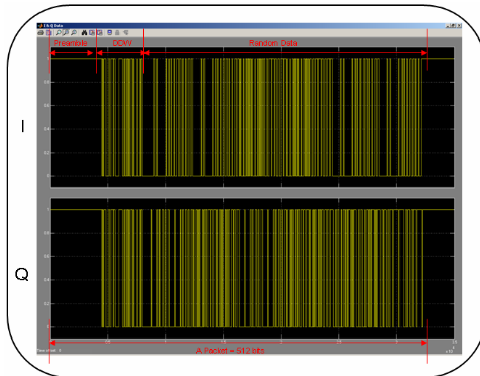
Figure 3.14: I and Q Packets in Simulation
