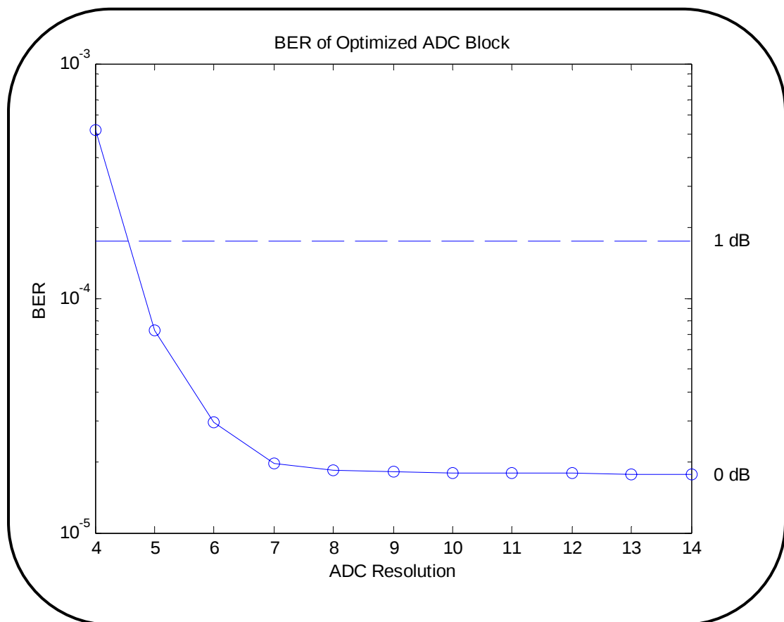
Figure 6.2: BER versus ADC Resolution
