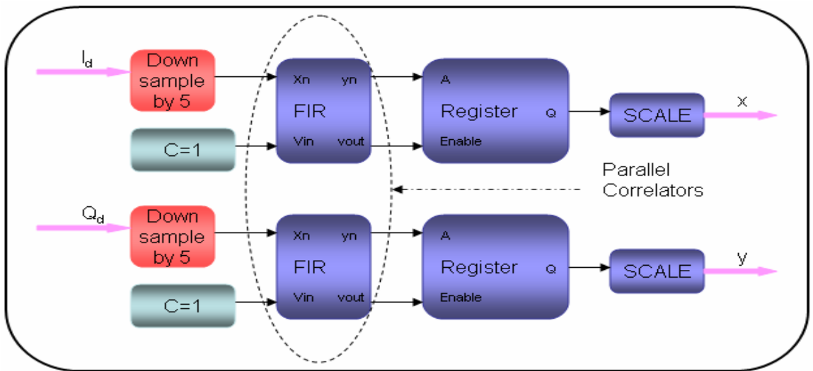
Figure 3.51: Implementation of Parallel Correlators
