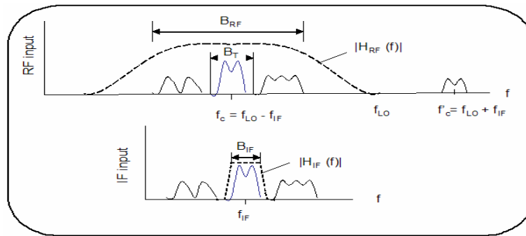
Figure 2.2: Spectral Drawings
