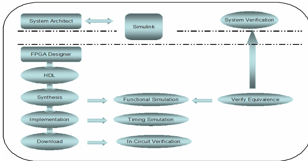
Figure 4.1: Traditional Simulink FPGA Flow
