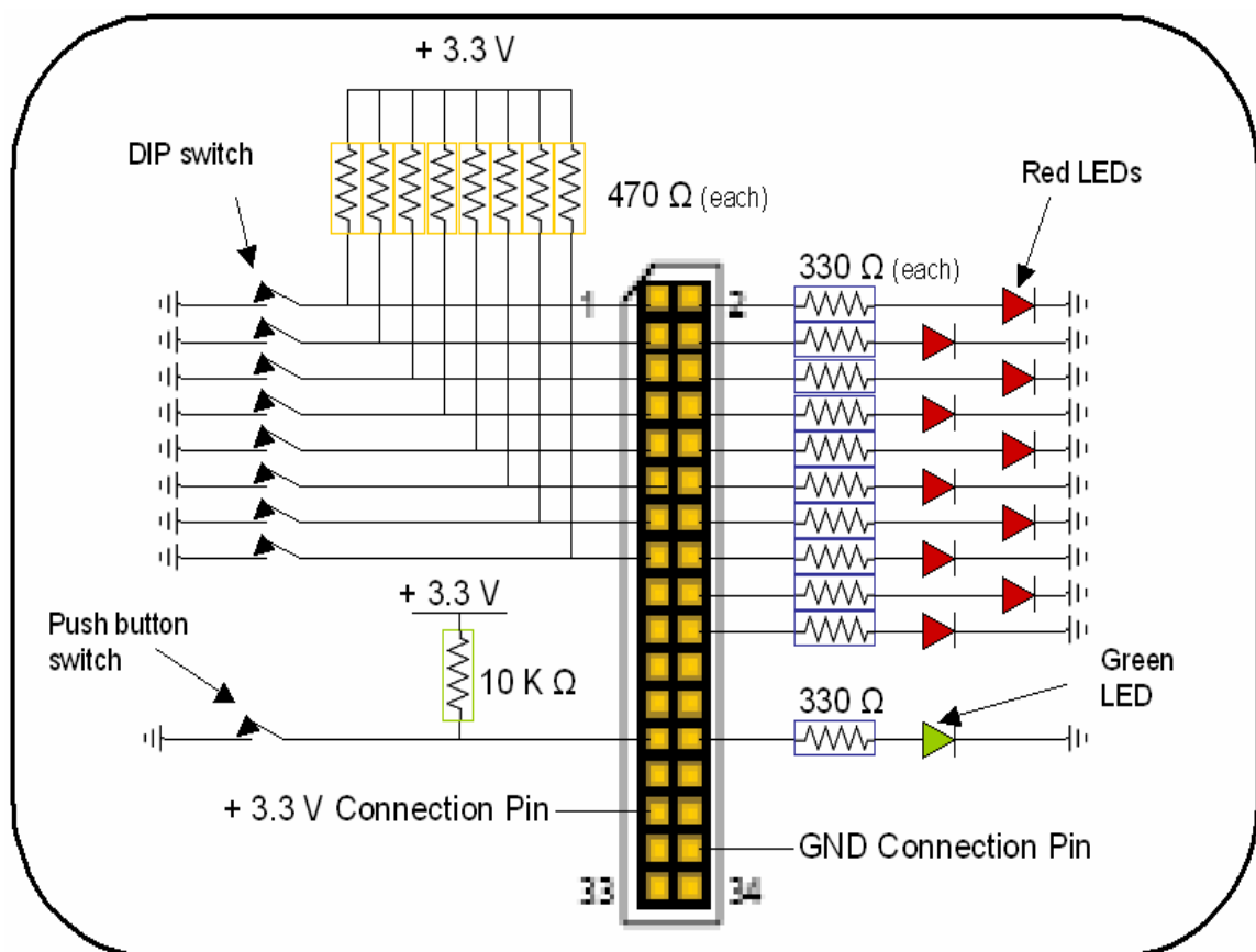
Figure 5.14: Circuit Diagram for BER Board
