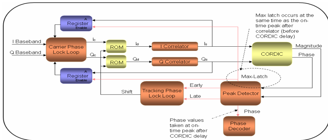
Figure 3.56: Peak Detector Outputs
