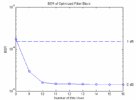
Figure 4. BER versus LPF datapath size
