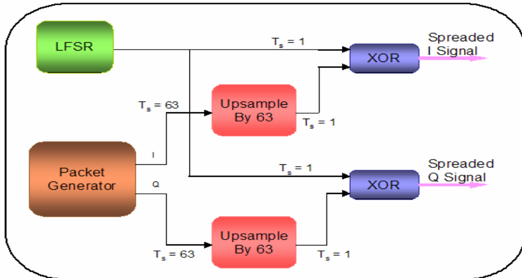
Figure 3.15: Spreading Packets with PN Sequence
