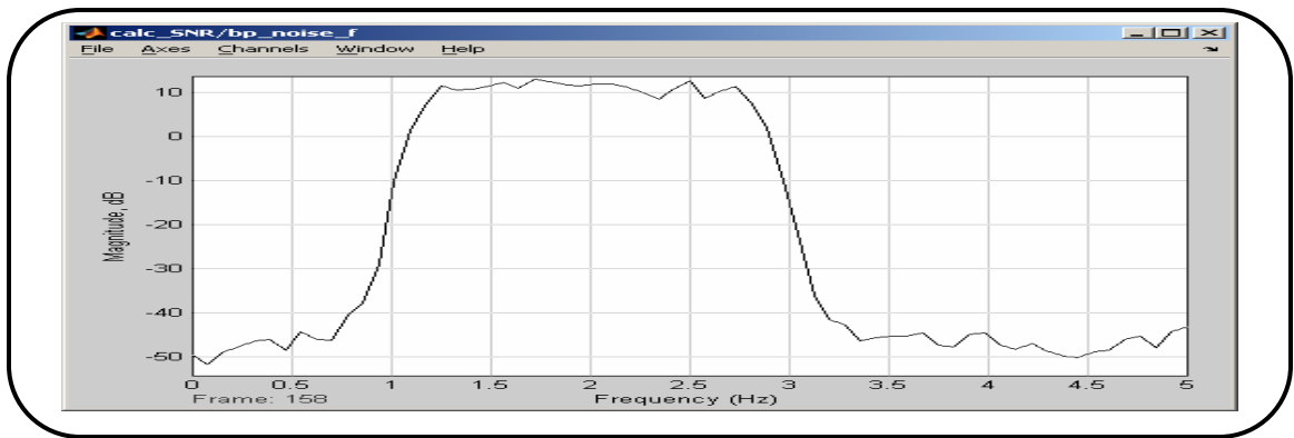
Figure 3.28: Spectrum of Bandpass Noise
