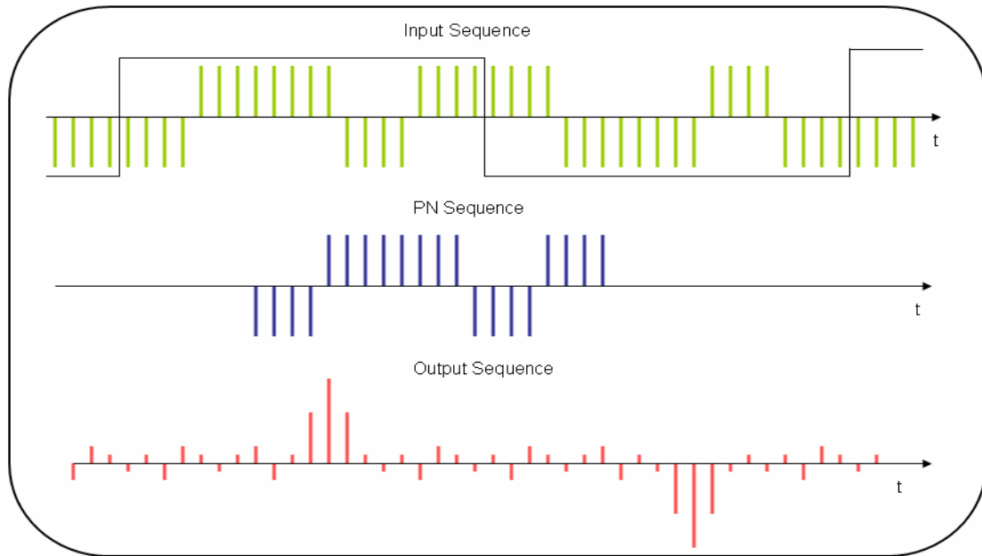
Figure 3.53: Example of Correlator
