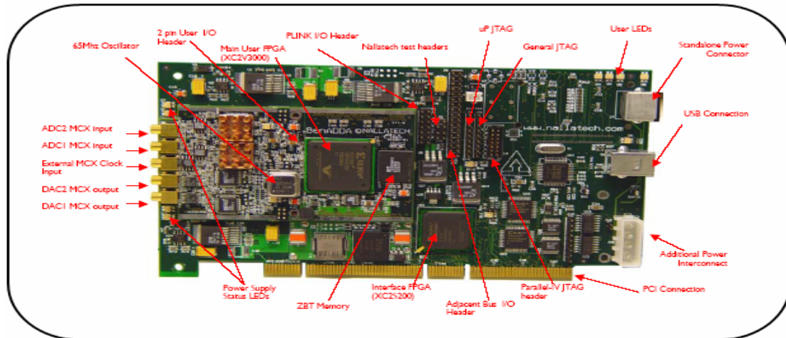
Figure 5.4: Key Features of the Motherboard
