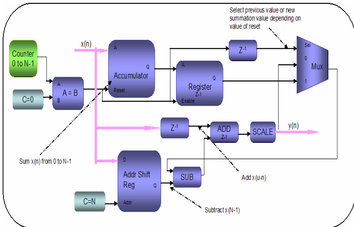
Figure 3.38: Running Average Filter Model
