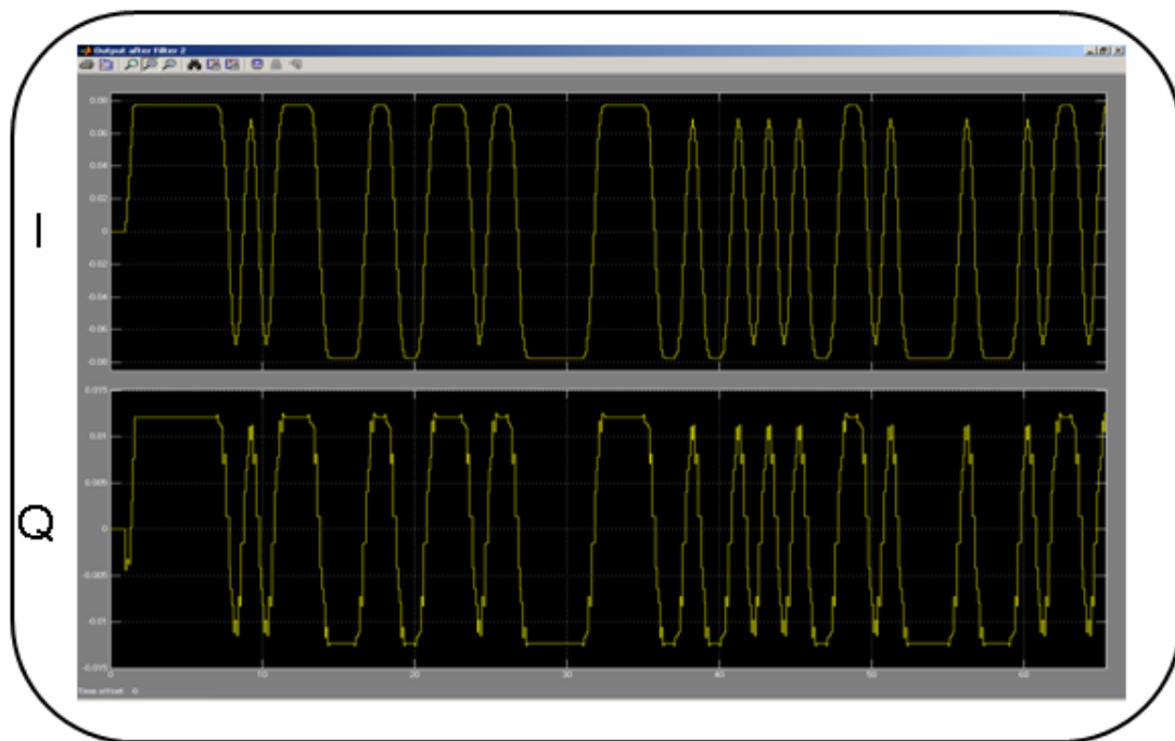
Figure 3.45: Signal after Running Average Filter 2
