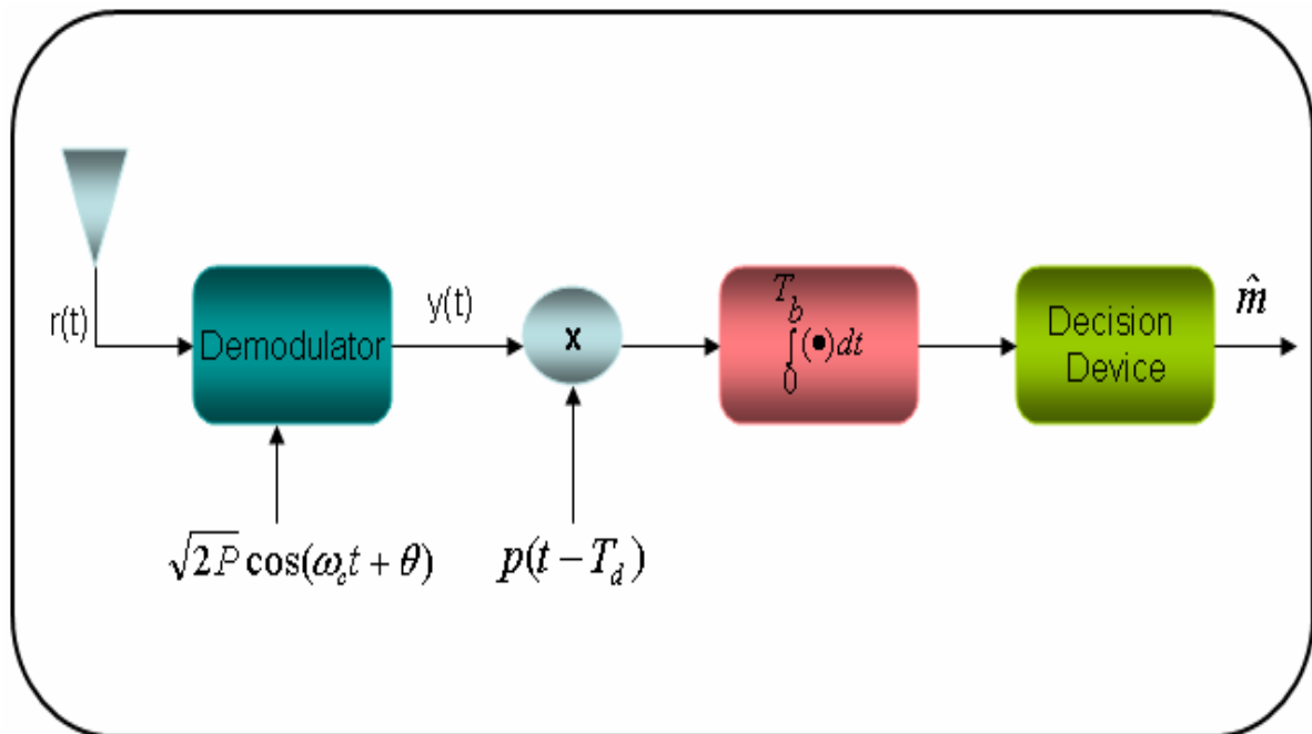
Figure 3.5: Design of Receiver
