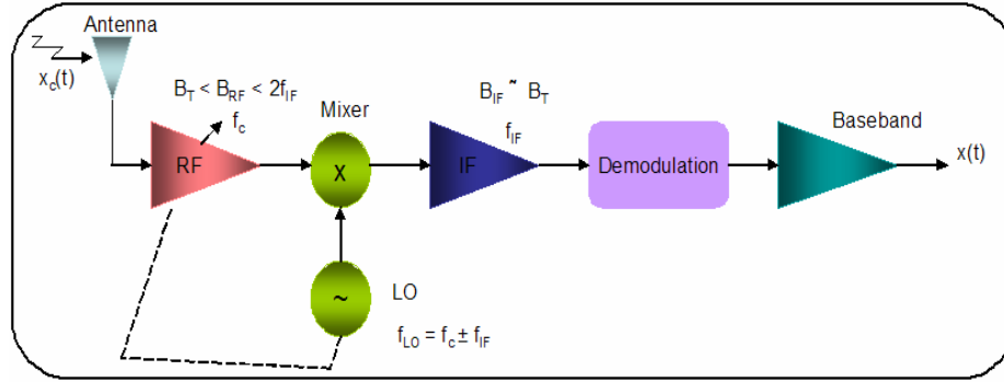
Figure 2.1: Superheterodyne Receiver
