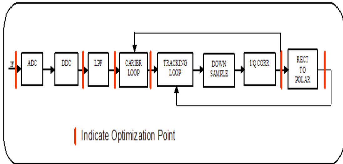
Figure 6.1: Optimization Points in DSSS Receiver
