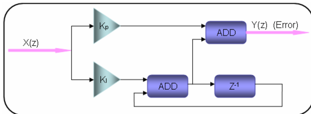
Figure 3.49: Loop Filter
