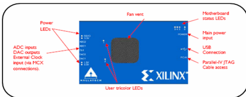
Figure 5.3: Front Case of XtremeDSP Board
