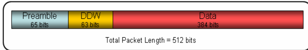
Figure 3.11: Packet Structure
