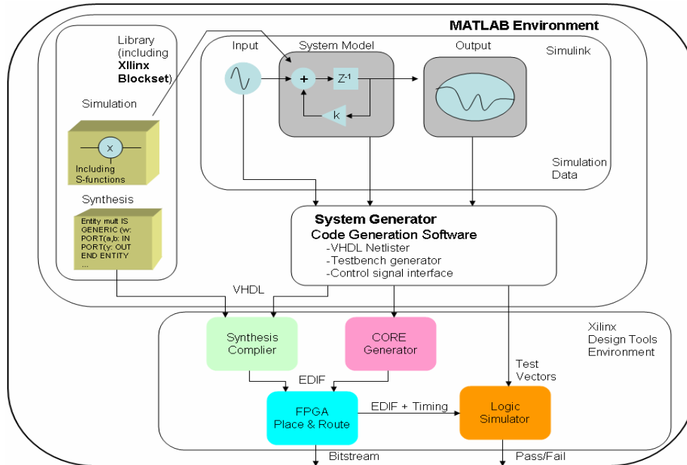
Figure 4.2: System Generator Flow Diagram
