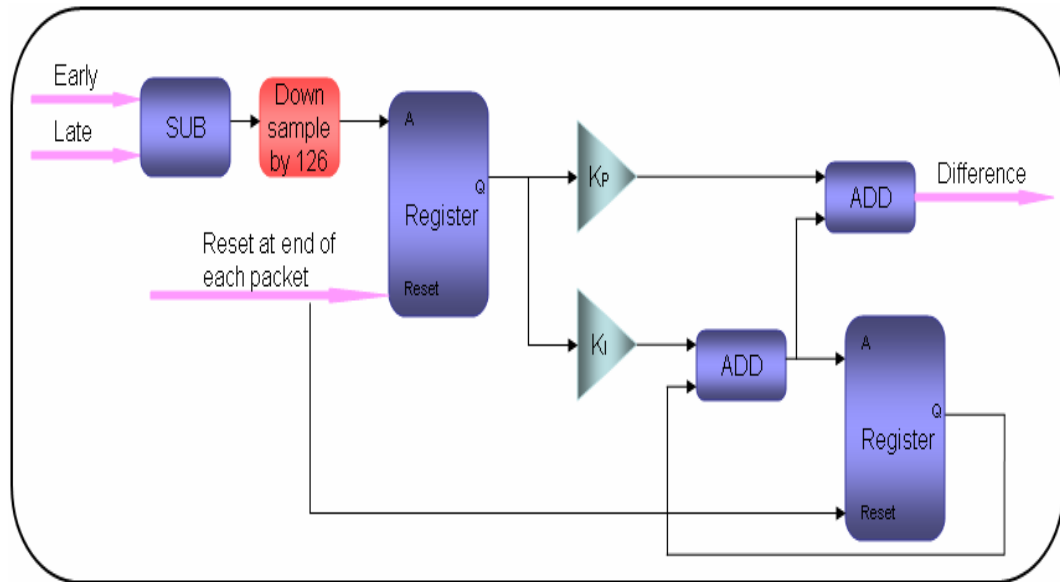
Figure 3.59: Tracking Phase Lock Loop Model
