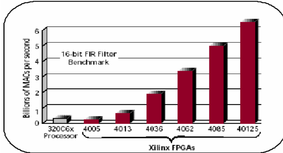
Figure 2.6: Comparison of Performance of Xilinx FPGAs to DSP Processors
