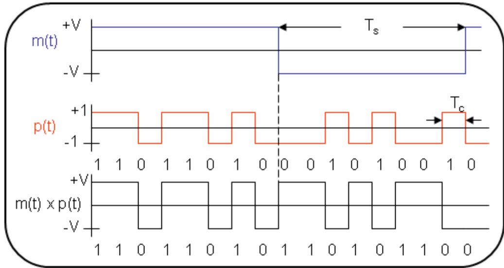
Figure 3.2: Effect of Spreading on Message Stream
