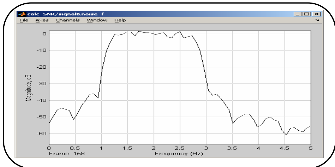
Figure 3.31: Spectrum of the Signal after Noise is Added
