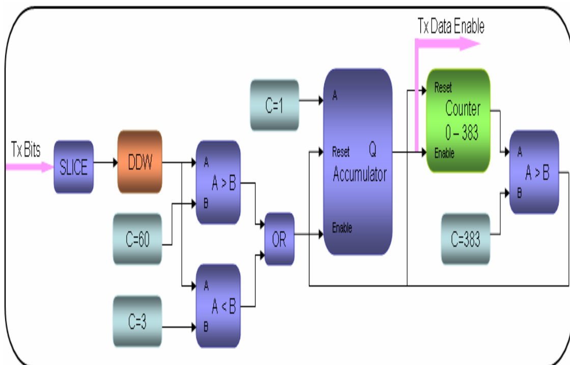
Figure 3.64: Packet Processor
