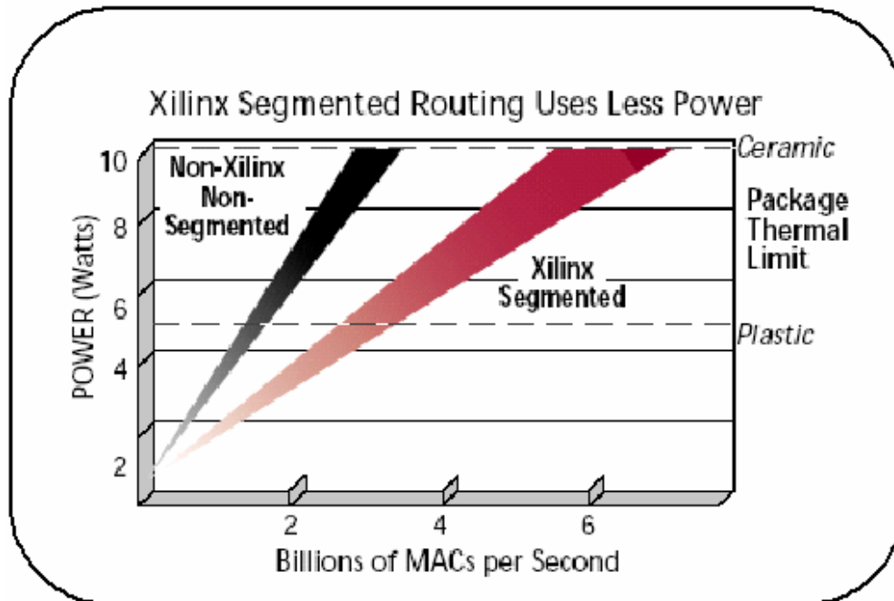
Figure 2.7: Power Consumption of Segmented and Non-Segmented Routing Architecture
