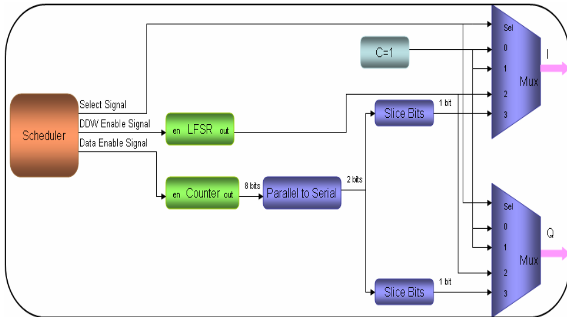
Figure 3.13: I and Q Packets
