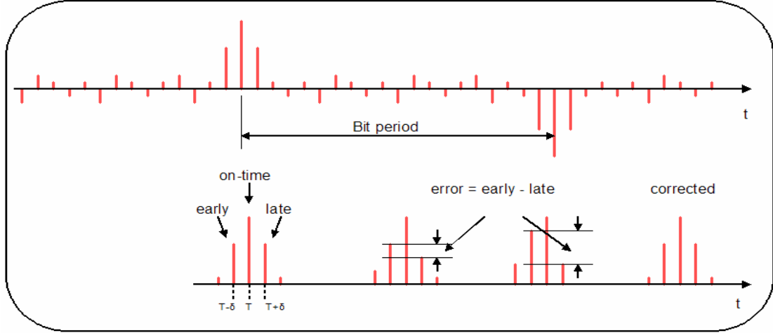
Figure 3.58: Early, Late, and On-time Samples
