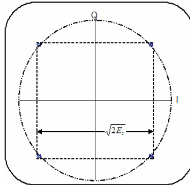
Figure 3.8: QPSK Constellation Diagram
