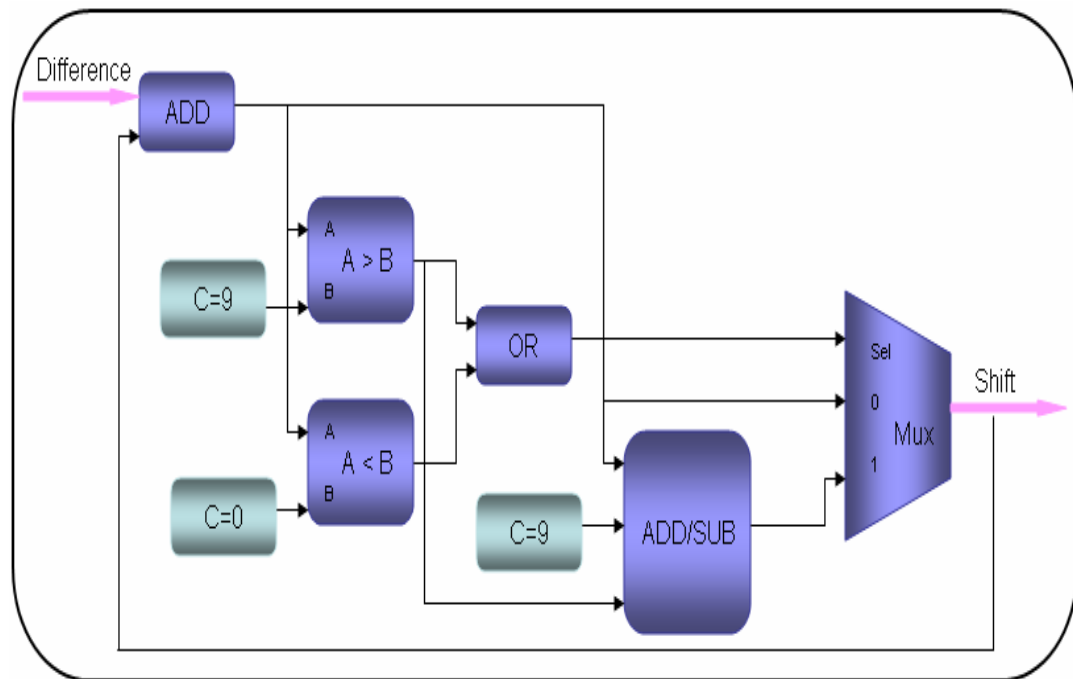
Figure 3.60: Tracking Phase Lock Loop Model (2)
