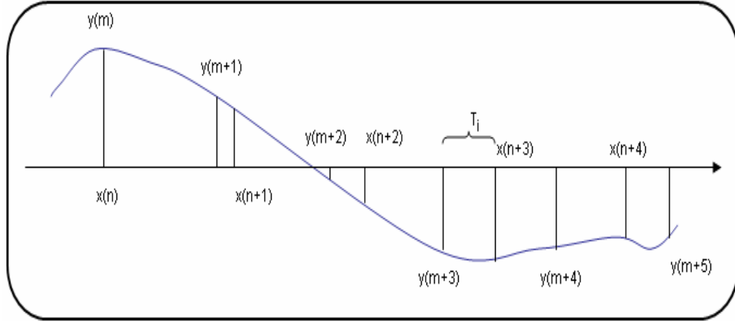
Figure 4.5: Sample Rate Conversion Example
