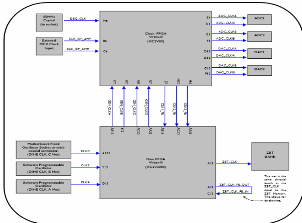
Figure 5.7: Overview of Clock Structure
