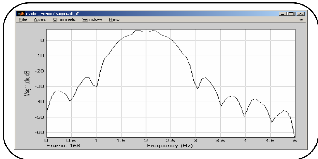
Figure 3.30: Spectrum of Signal before Noise is Added
