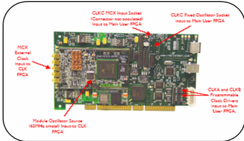
Figure 5.6: Inputs Related to Clock Sources on Hardware
