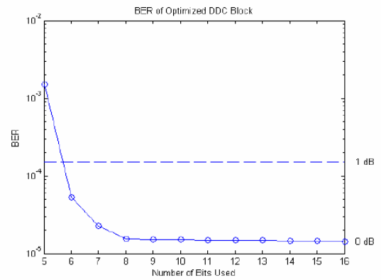
Figure 3. BER versus DDC datapath size
