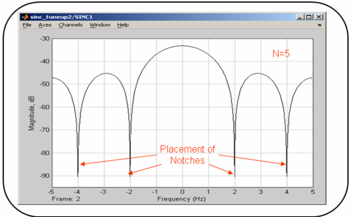
Figure 3.40: Magnitude Response of Filter 1
