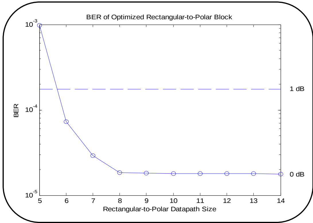
Figure 6.7: BER versus Rectangular-to-Polar Datapath Size
