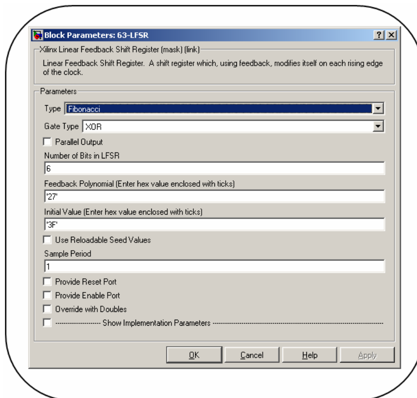
Figure 3.17: Block Parameters for LFSR
