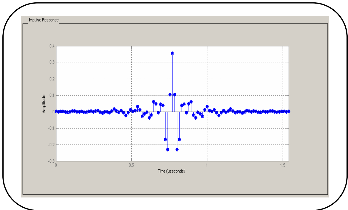
Figure 3.26: Impulse Response of Bandpass Filter
