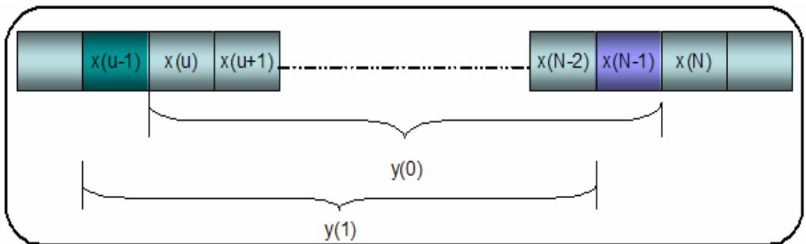
Figure 3.37: Running Average Filter Example
