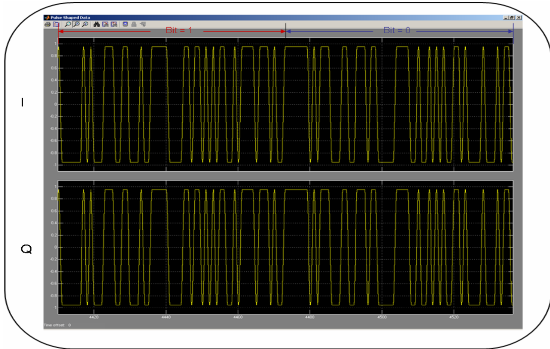
Figure 3.21: Signal Pulse Shaping in Simulation
