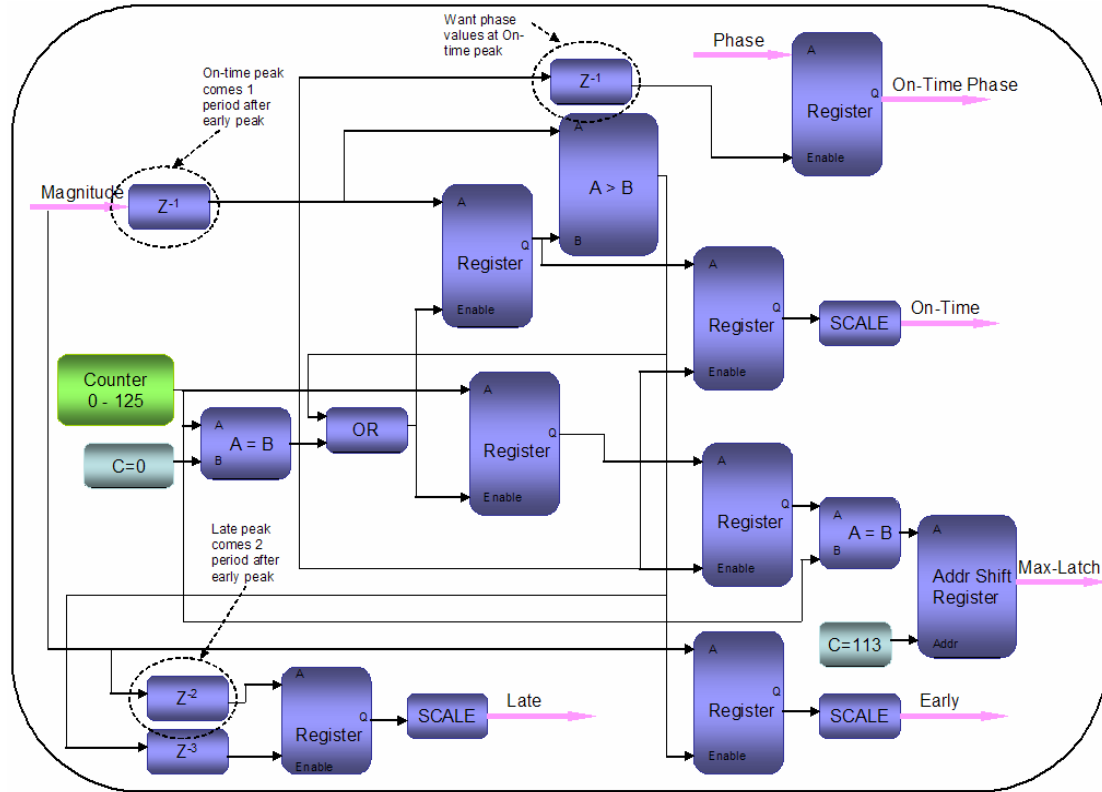
Figure 3.57: Peak Detector Model
