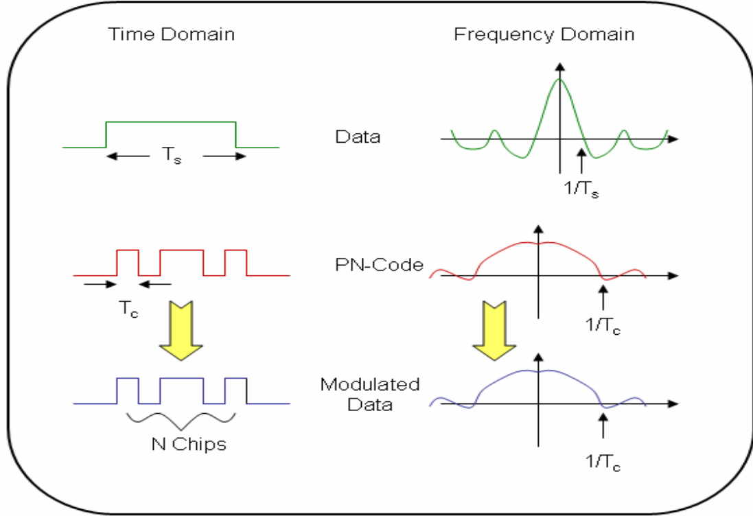
Figure 3.3: Time/Frequency Analysis
