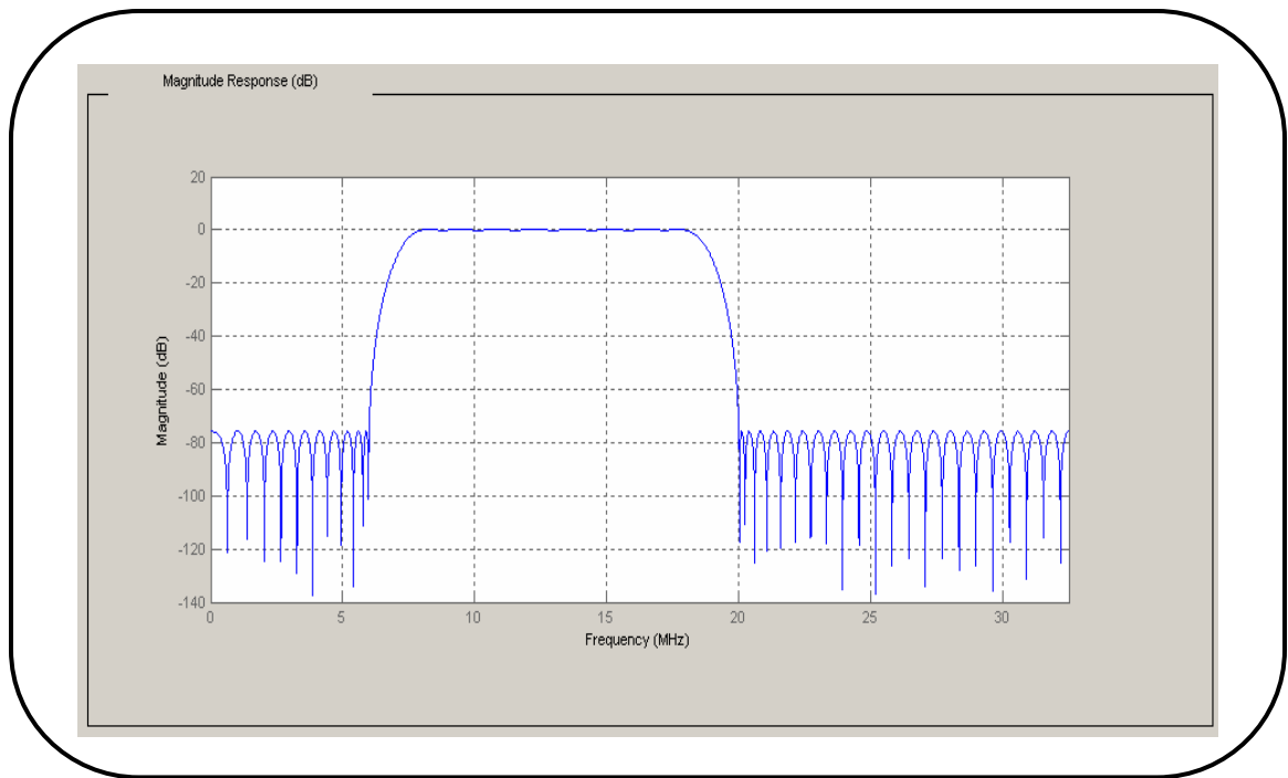
Figure 3.25: Magnitude Response of Bandpass Filter
