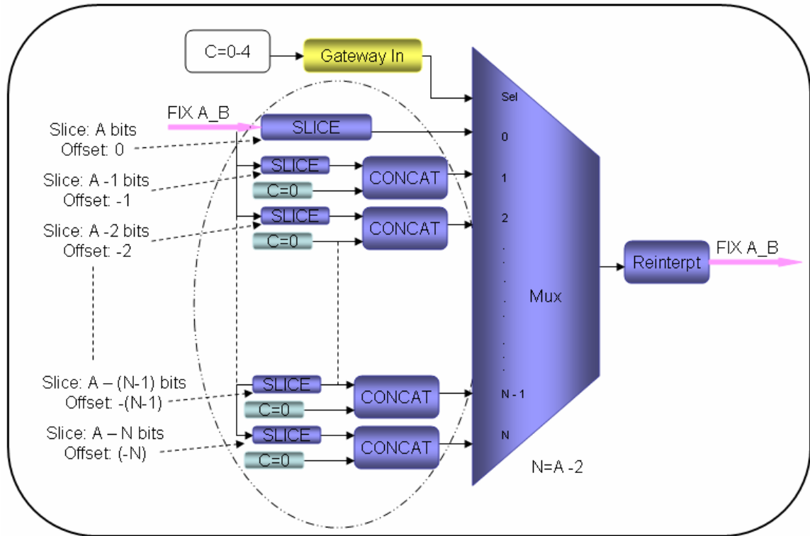
Figure 3.59: Optimization Block
