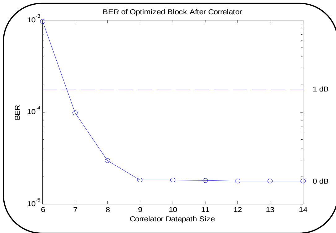
Figure 6.6: BER versus Correlator Datapath Size
