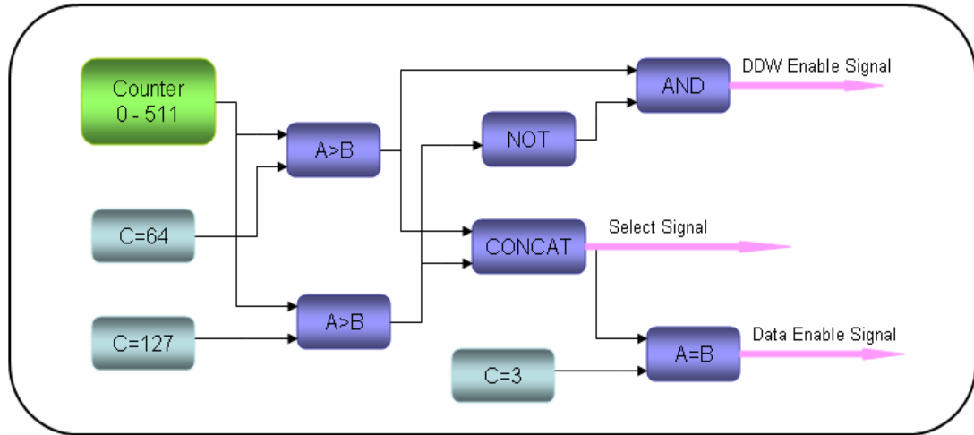
Figure 3.12: Packet Scheduler
