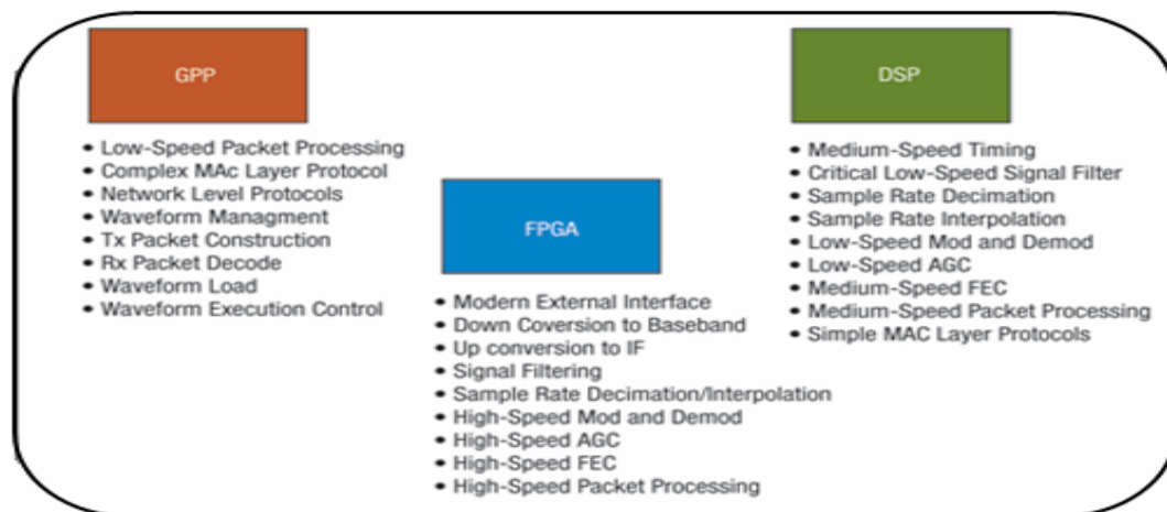
Figure 2.5: Architecture Splitting SDR Functions across GPPs, DSPs, and FPGAs
