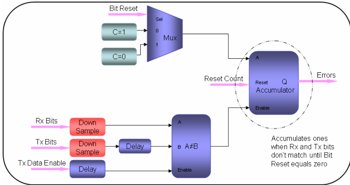
Figure 3.67: Error Counter
