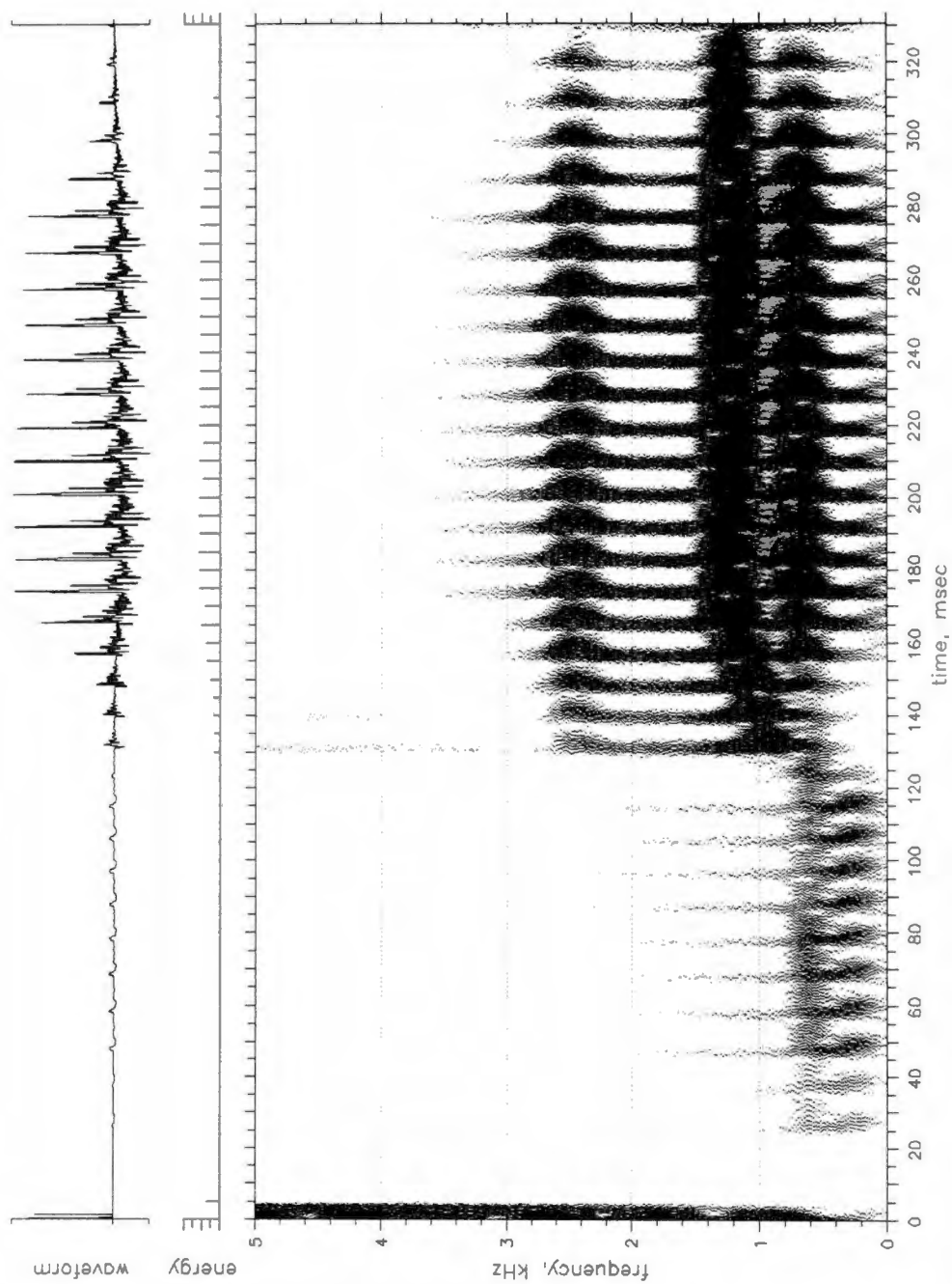
Figure 2. Waveform and spectrogram of the end point stimulus in condition one, continuum number on, having an F2 transition appropriate for /m/ and an /n/-like relative amplitude value.
