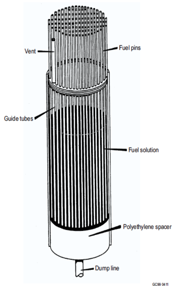
Figure 6. Schematic of the Boiler Tube-Type Tank used for MMT-001 [6]
