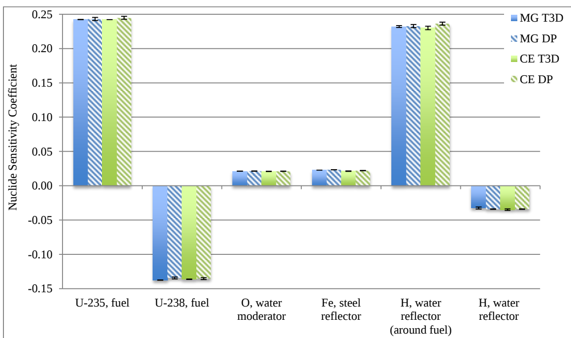
Figure 46. TSUNAMI and Direct Perturbation Sensitivity Comparisons for Representative LCT-042-007 Nuclides
