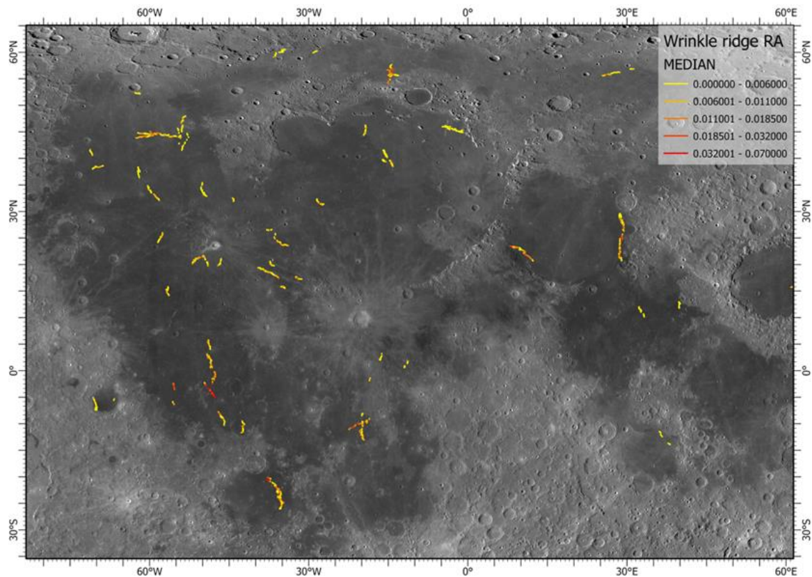
Figure 2.S10. Recently active wrinkle ridges identified in this work colorized by median Diviner rock abundance value. Many of the wrinkle ridges exhibit low rock abundance values, but several ridges in S. Mare Procellarum, Mare Serenitatis, and Mare Frigoris exhibit moderate rock abundance.
