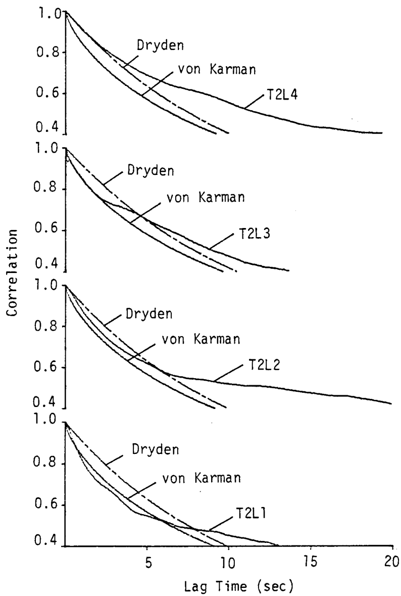
Figure 6.23. Comparison with von Karman and Dryden expressions for the longitudinal correlation (length scale L_4 , T2, Run #8624).
