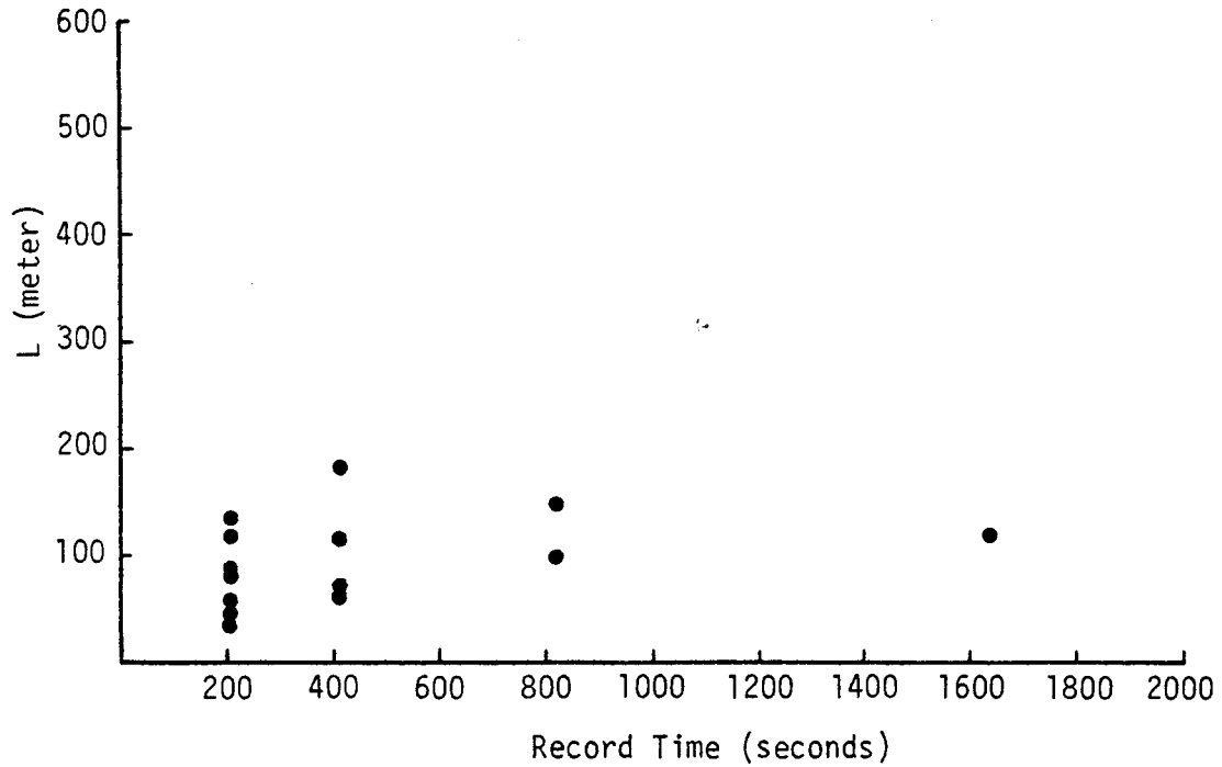
Figure 5.4. The variation of integral length scale with different record times.
