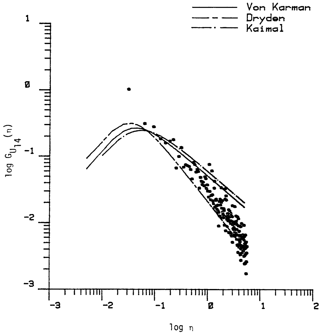
Figure 7.12. Comparison of longitudinal turbulence spectrum with three correlation models. (The length scale is calculated by Method 3, Chapter V, Run #8624).
