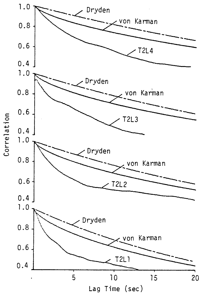
Figure 6.17. Comparison with von Karman and Dryden expressions for the longitudinal correlation (length scale L_1 , T2, Run #8624).
