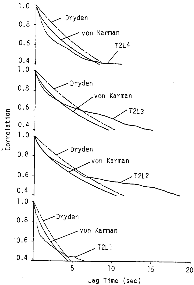
Figure 6.14. Comparison with von Karman and Dryden expressions for the longitudinal correlation (length scale L_1 , T2, Run #8623).
