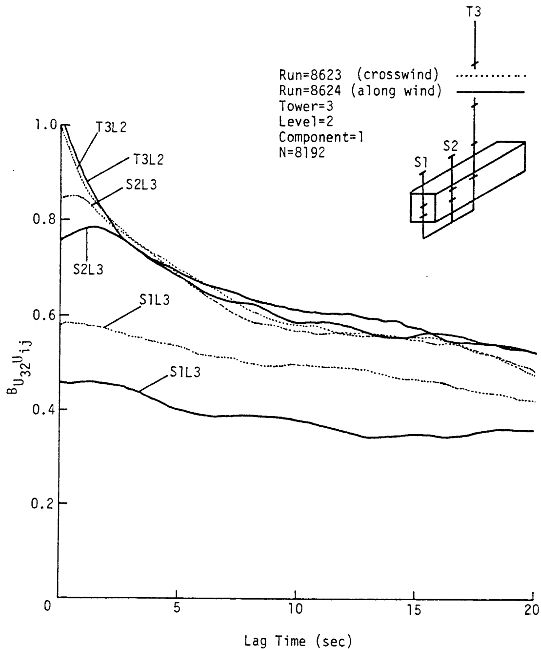
Figure 6.9. Two-point horizontal space-time correlation immediately behind the building and slightly above wake relative to T3L2.
