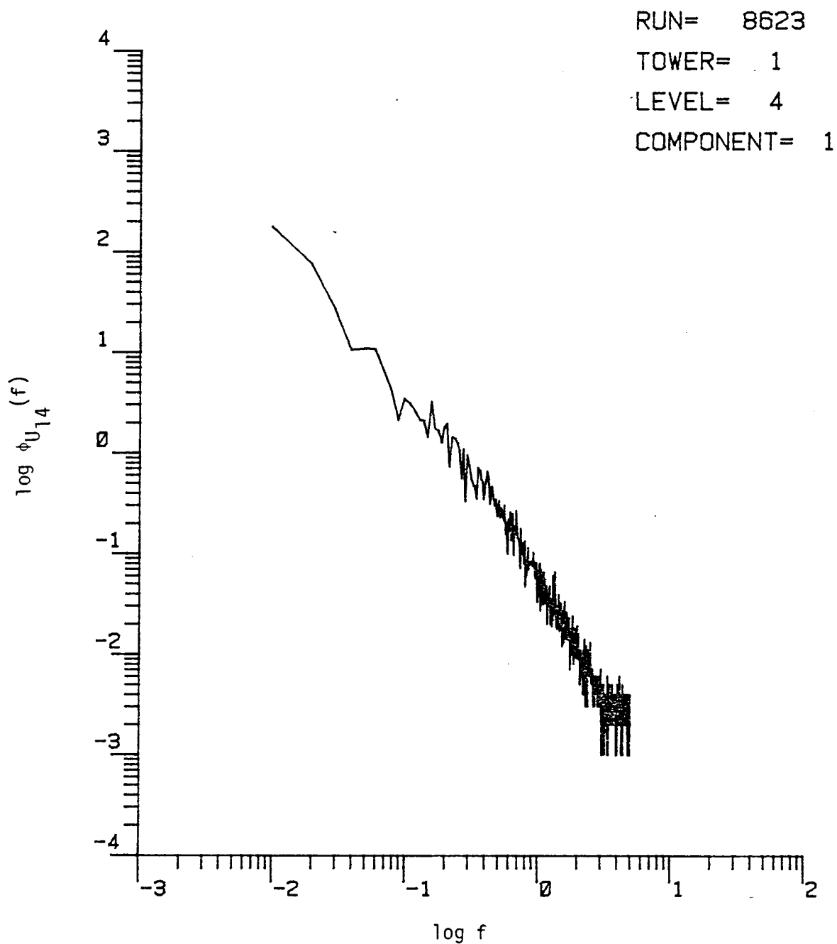
Figure 7.2. Power spectral density function calculated by the FFT method without using a tapering window.
