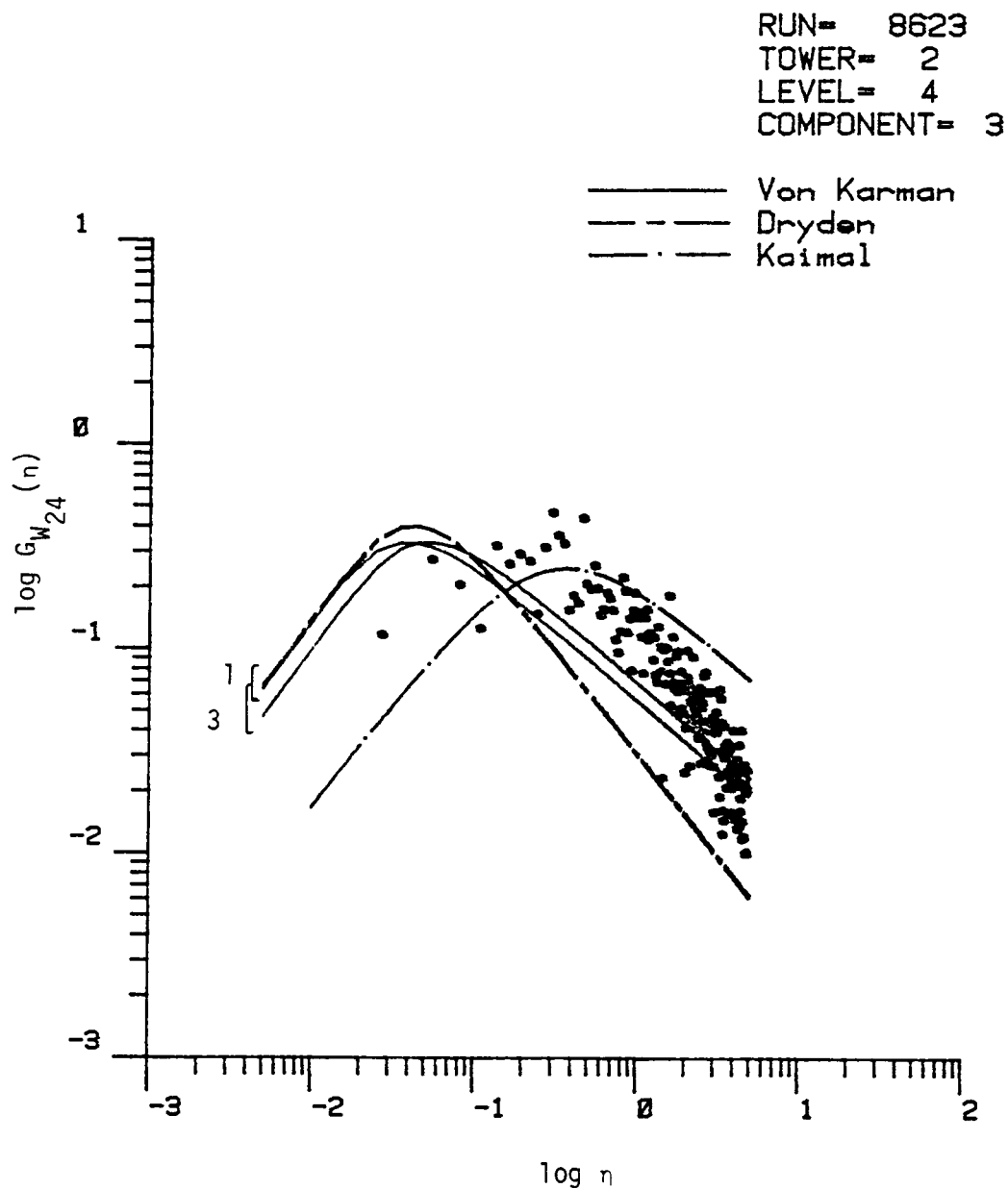
Figure 7.26. Comparison of vertical turbulence spectrum with three correlation models. (The length scale is calculated by Methods 1 and 3, Chapter V, T2, Run #8623).
