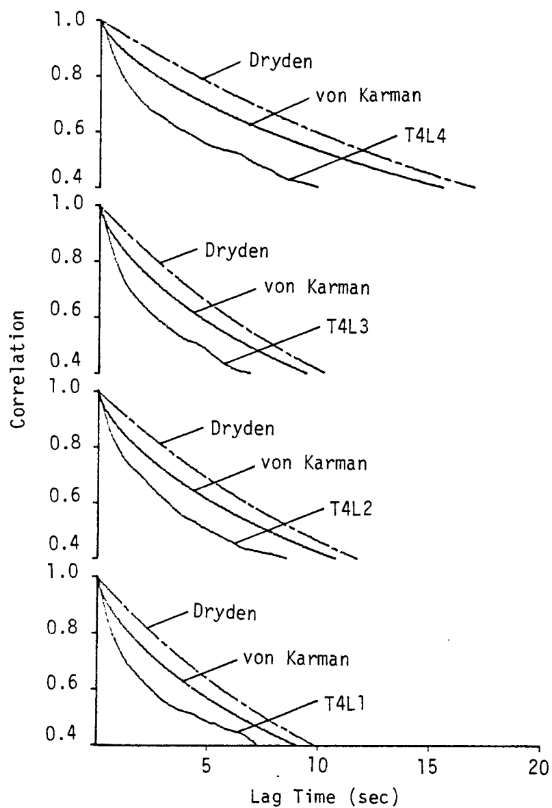
Figure 6.15. Comparison with von Karman and Dryden expressions for the longitudinal correlation (length scale L_1 , T4, Run #8623).
