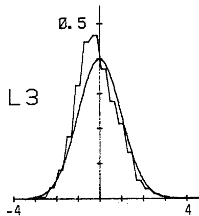
Figure C.4. Probability density function for longitudinal velocity component normalized with \sigma_{w_x} (Run #8623, T4, Component 1).
