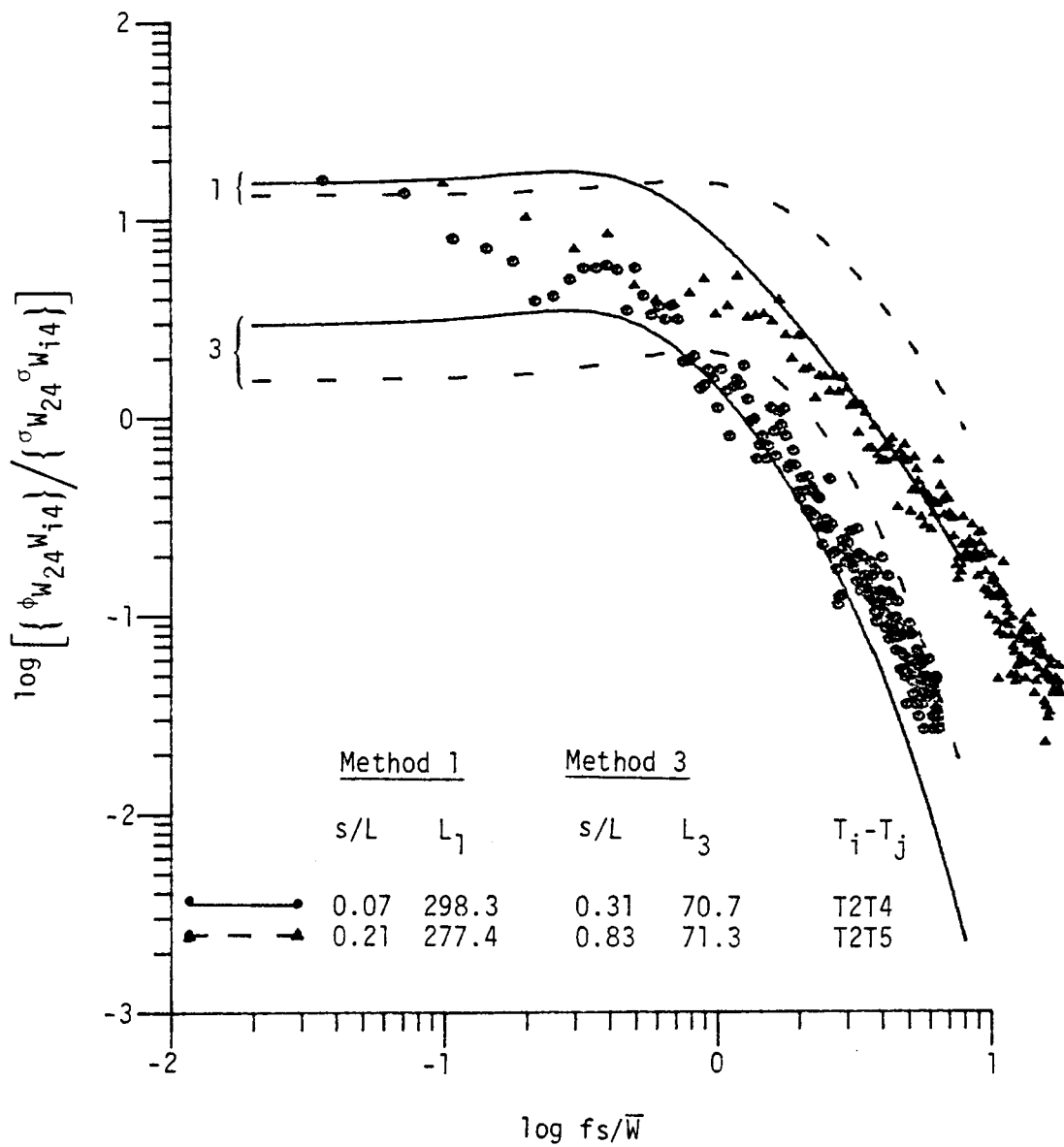
Figure 8.11. Comparison of computed two-point spatial spectra with the theoretical model of HouboIt and Sen (1972) (Run #8624, L4, Component 3).
