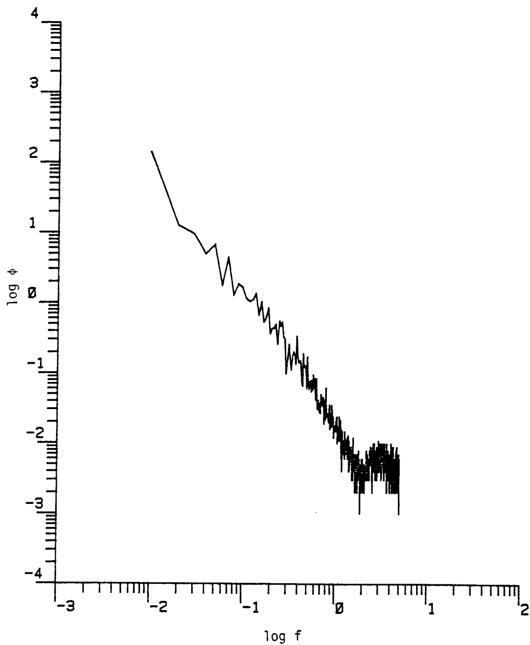
Figure D.42. The longitudinal power spectrum (Run #8624, T3L2, Component 1).
