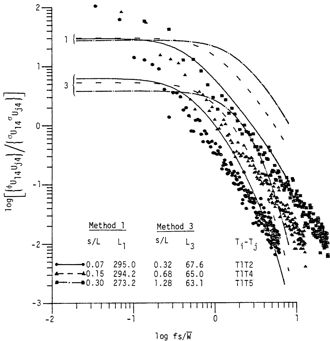
Figure 8.4. Comparison of computed two-point spatial spectra with the theoretical model of Houbolt and Sen (1972) (Run #8624, L4, Component 1).
