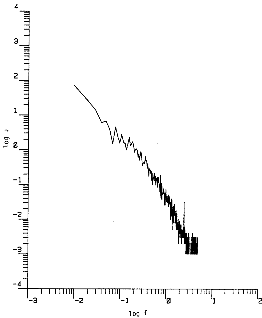
Figure D.21. The longitudinal power spectrum (Run #8623, S1L1, Component 1).
