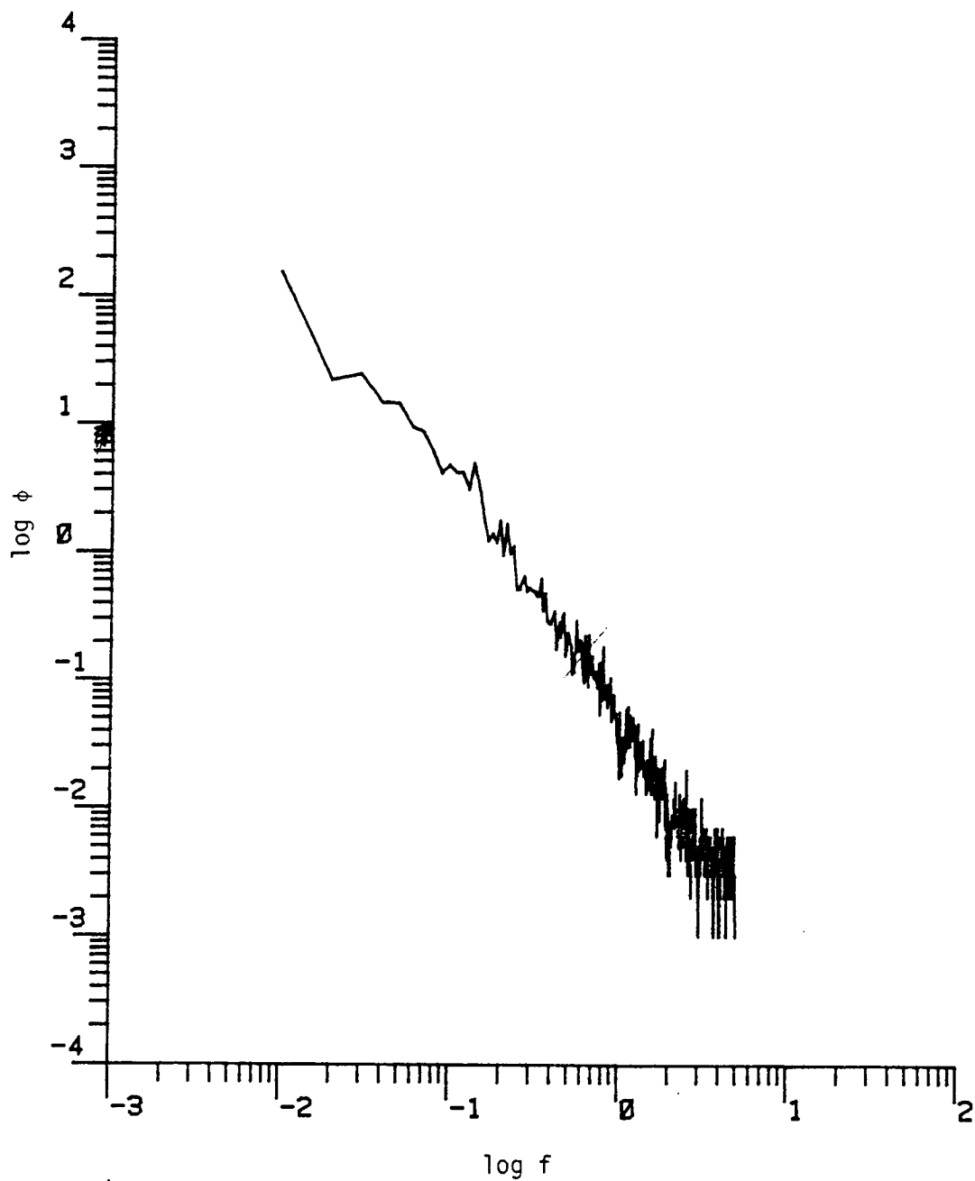
Figure D.64. The longitudinal power spectrum (Run #8624, S4L3, Component 1).
