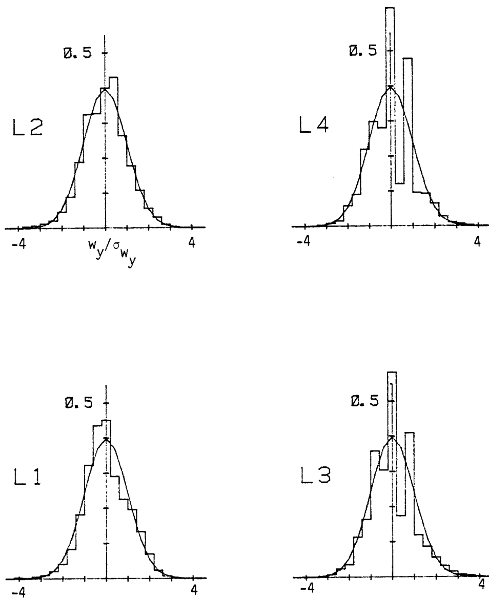
Figure C.31. Probability density function for lateral velocity component normalized with \sigma_{wy} (Run #8624, T4, Component 2).
