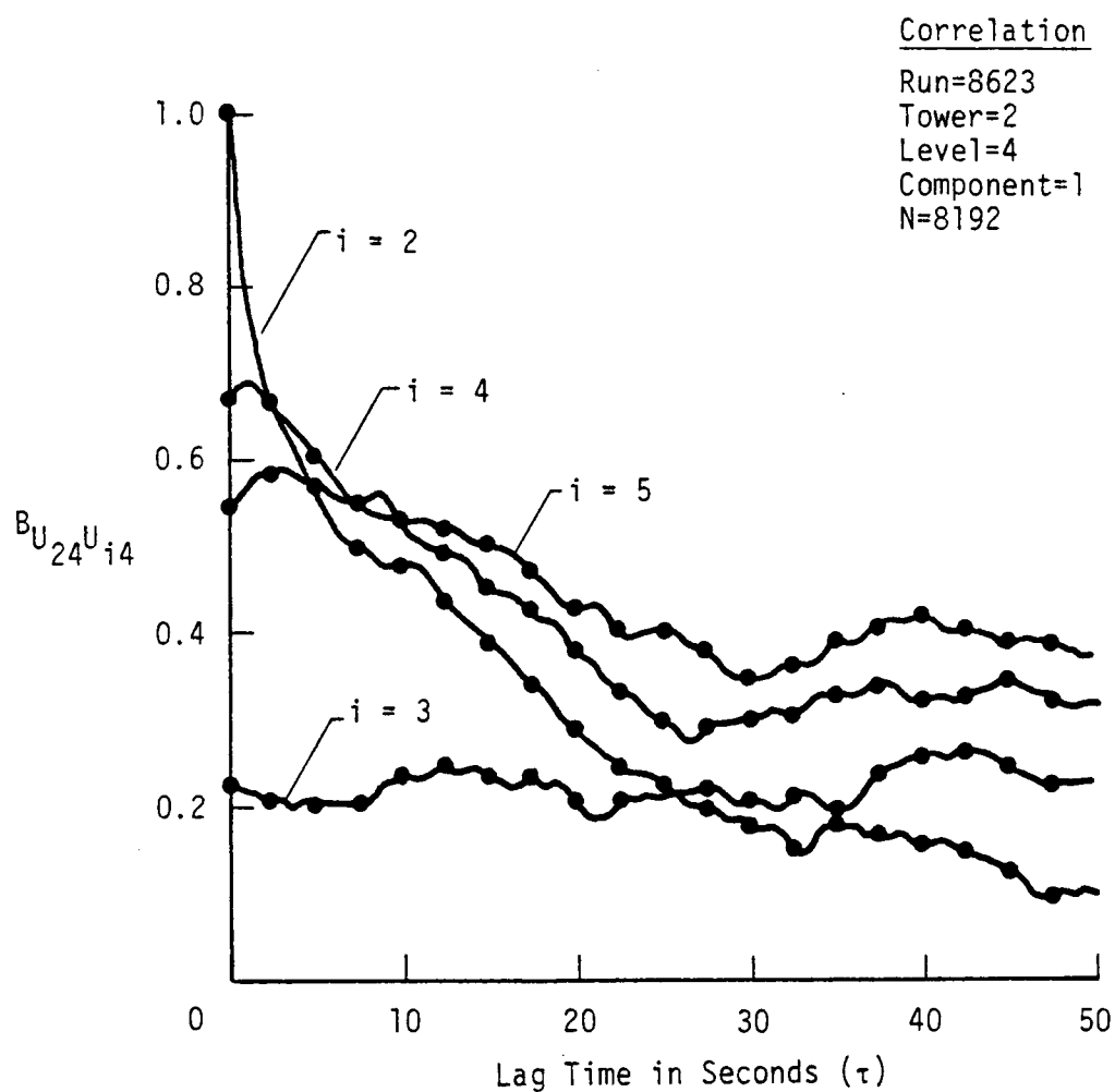
Figure 6.1. Comparison of the correlation coefficient computed by the direct method and by the FFT method (• represents the FFT computed values).
