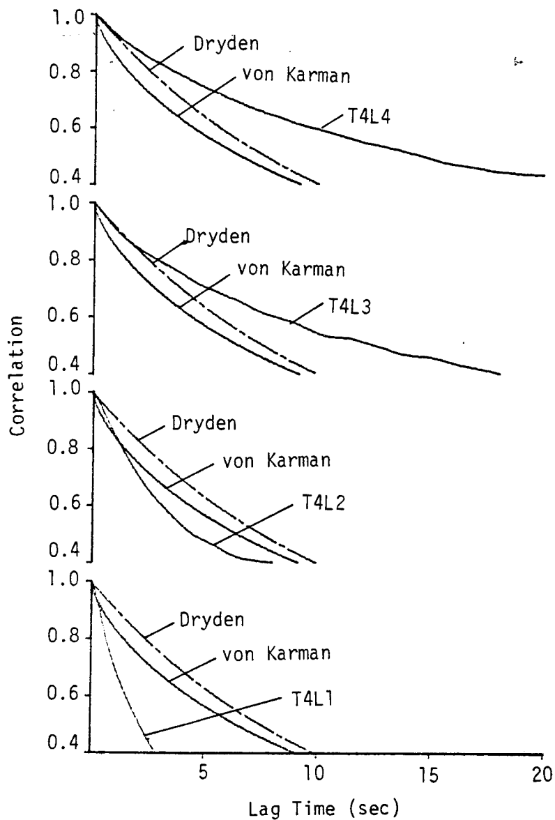
Figure 6.24. Comparison with von Karman and Dryden expressions for the longitudinal correlation (length scale L_4 , T4, Run #8624).
