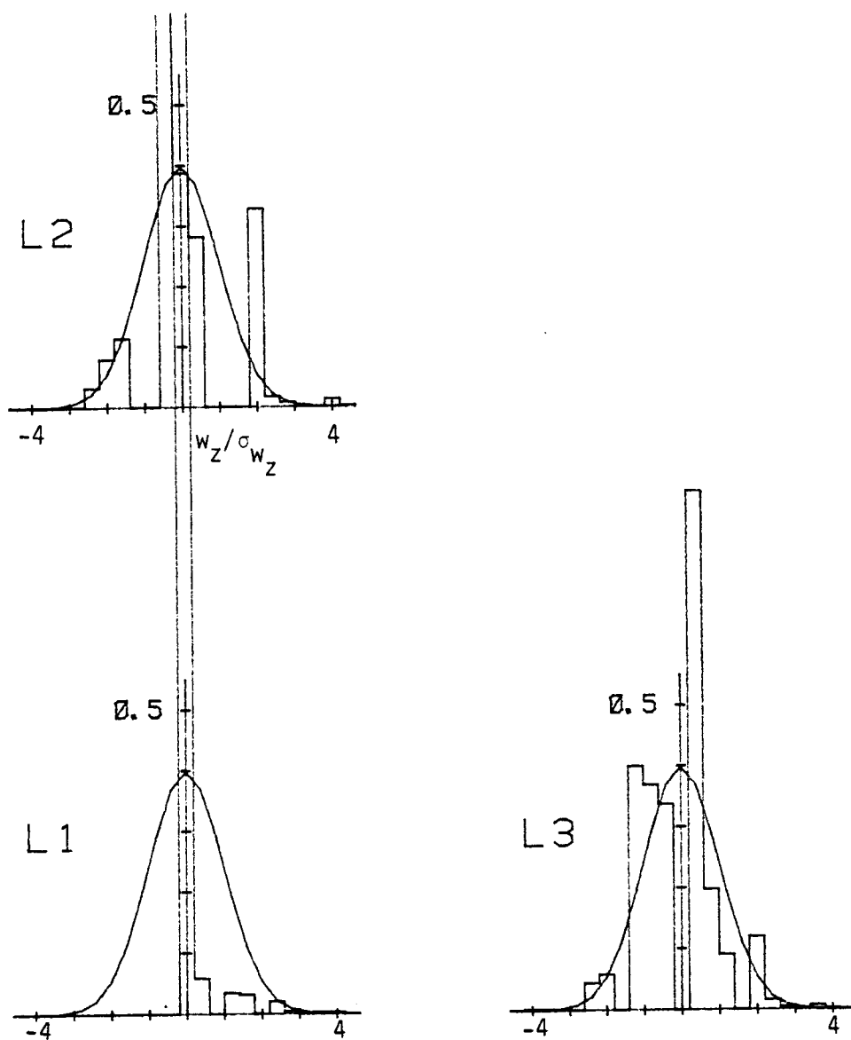
Figure C.42. Probability density function for vertical velocity component normalized with \sigma_{w_z} (Run #8623, S1, Component 3).
