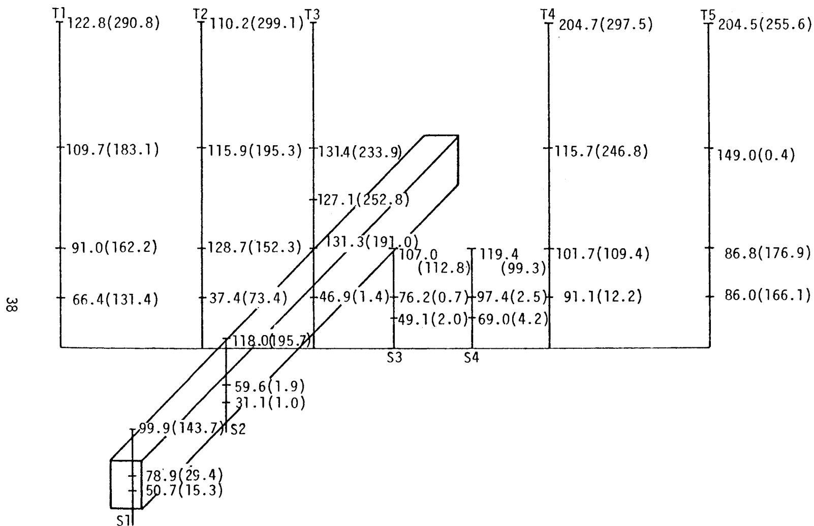
Figure 5.1. Spatial variation of the integral length scale in meters as computed by Method 1. (Component 1: Numbers not in parentheses, Run #8623, crosswind; numbers in parentheses, Run #8624, along wind).
