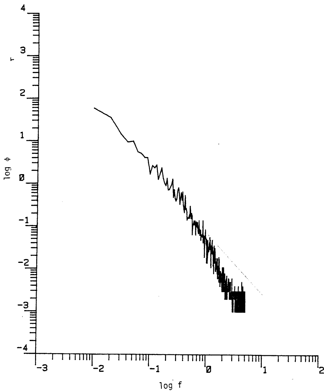
Figure D.24. The longitudinal power spectrum (Run #8623, S2L1, Component 1).
