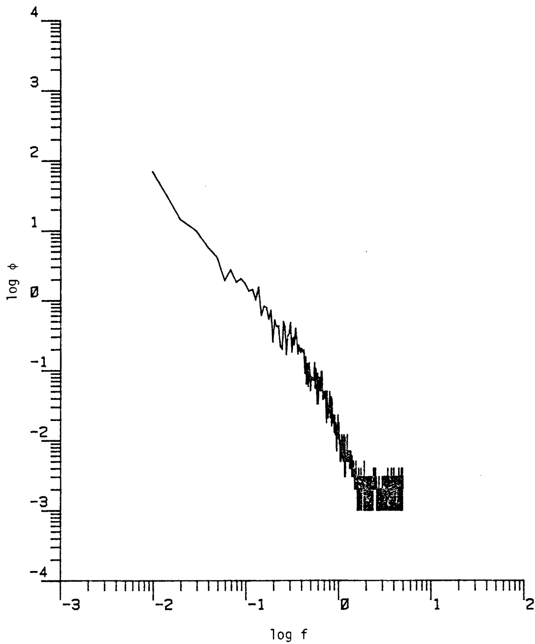
Figure D.37. The longitudinal power spectrum (Run #8624, T2L1, Component 1).
