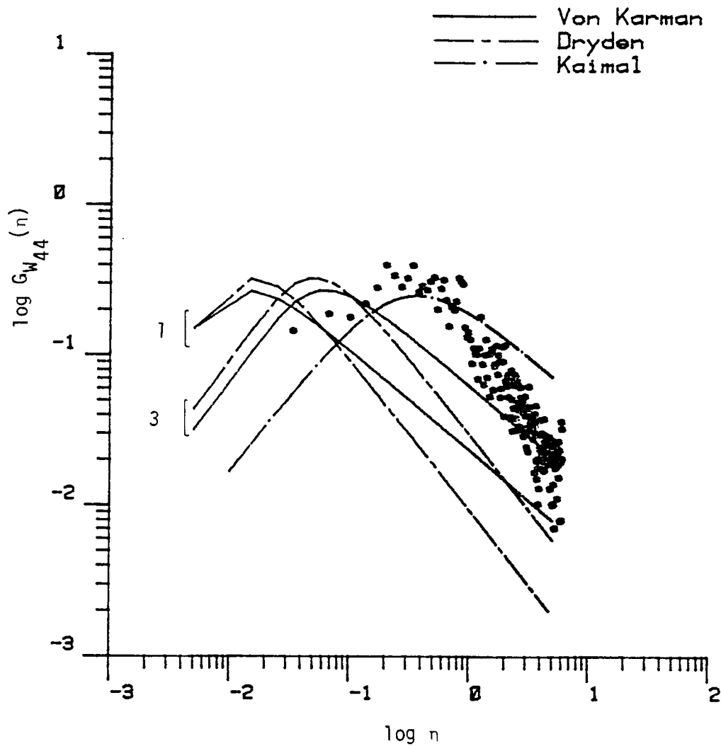
Figure 7.30. Comparison of vertical turbulence spectrum with three correlation models. (The length scale is calculated by Methods 1 and 3, Chapter V, T4, Run #8624).
