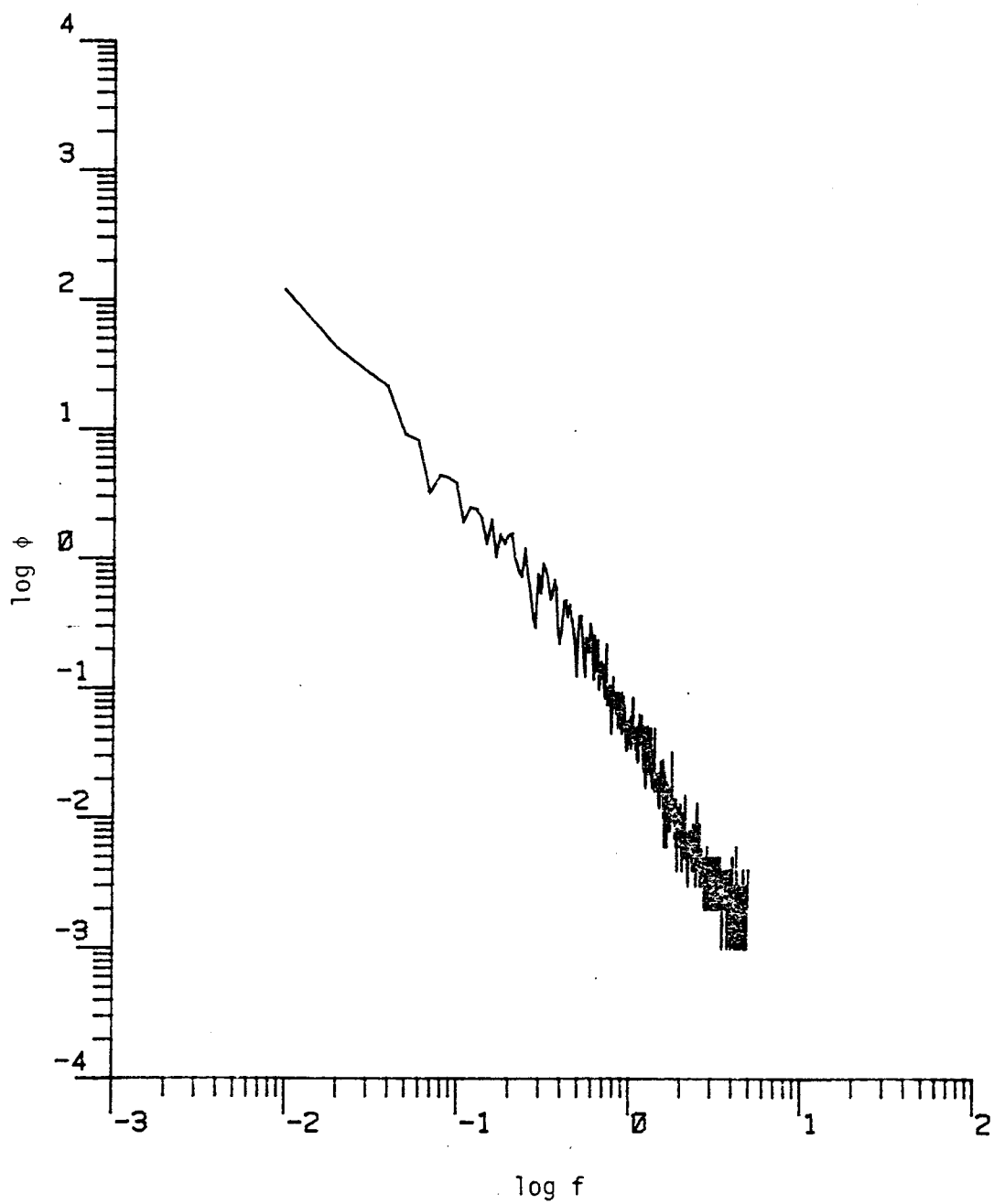
Figure D.1. The longitudinal power spectrum (Run #8623, T1L1, Component 1).
