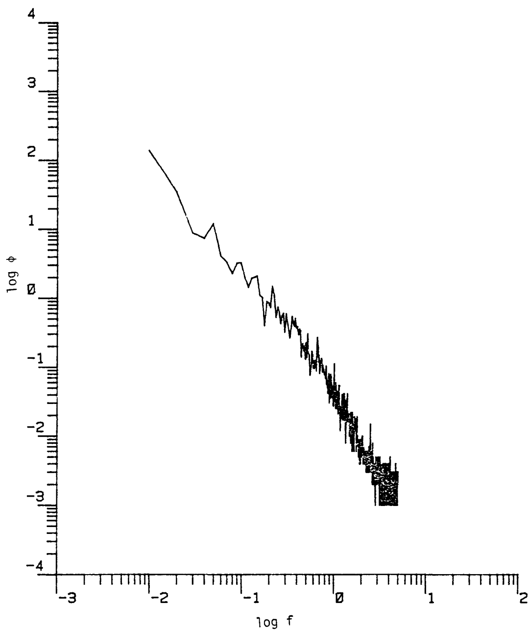
Figure D.17. The longitudinal power spectrum (Run #8623, T5L1, Component 1).
