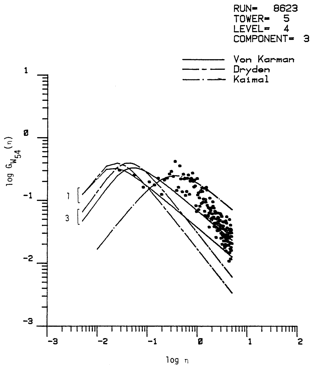
Figure 7.28. Comparison of vertical turbulence spectrum with three correlation models. (The length scale is calculated by Methods 1 and 3, Chapter V, T5, Run #8623).
