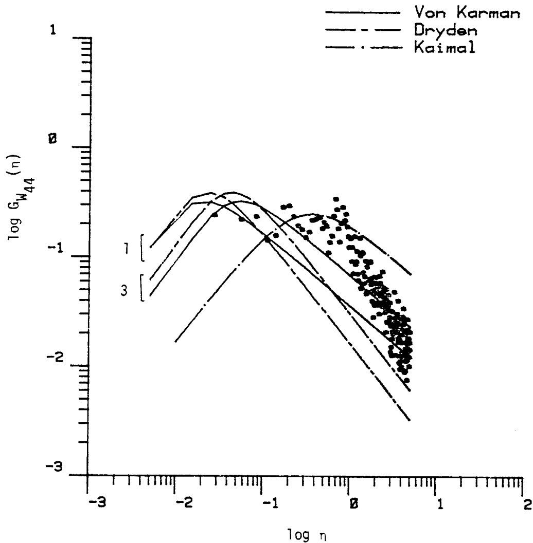
Figure 7.27. Comparison of vertical turbulence spectrum with three correlation models. (The length scale is calculated by Methods 1 and 3, Chapter V, T4, Run #8623).
