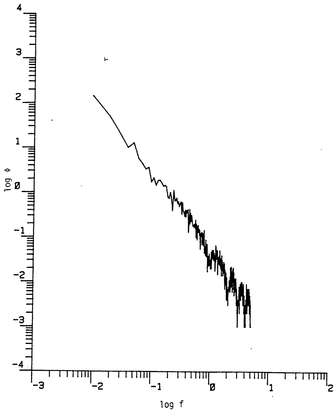
Figure D.32. The longitudinal power spectrum (Run #8623, S4L3, Component 1).
