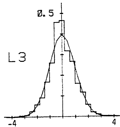
Figure C.36. Probability density function for lateral velocity component normalized with \sigma_{w_y} (Run #8624, S4, Component 2).
