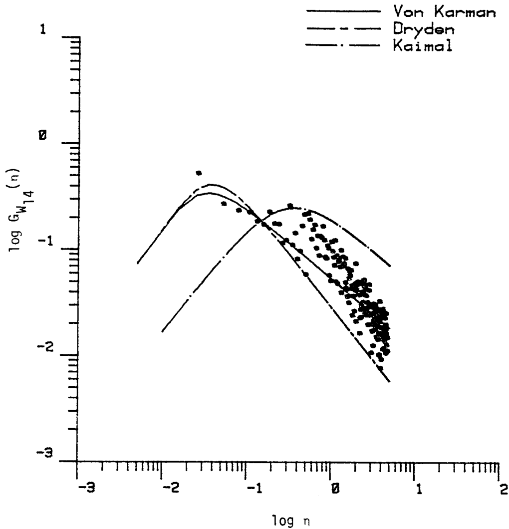
Figure 7.20. Comparison of vertical turbulence spectrum with three correlation models. (The length scale is calculated by Method 1, Chapter V, Run #8623).
