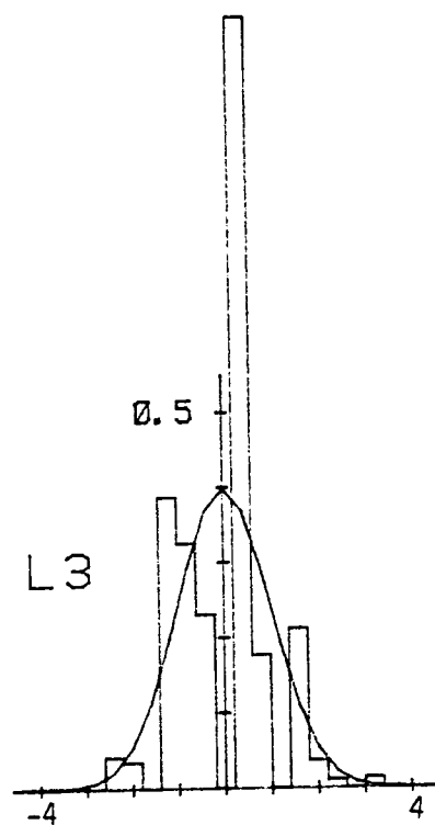
Figure C.51. Probability density function for vertical velocity component normalized with \sigma_{w_z} (Run #8624, S1, Component 3).
