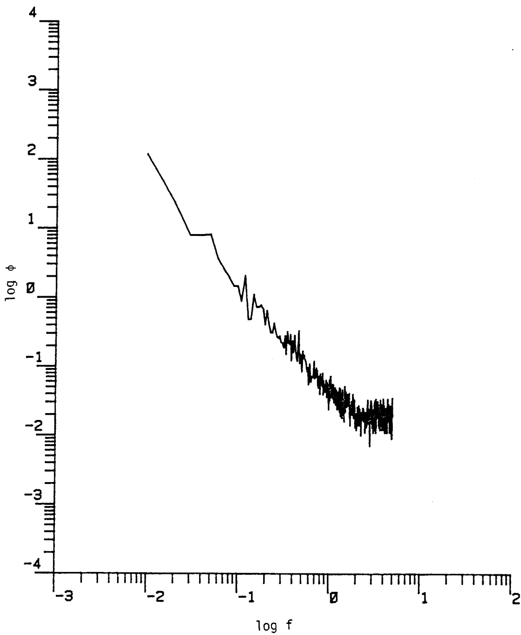
Figure D.55. The longitudinal power spectrum (Run #8624, S1L3, Component 1).
