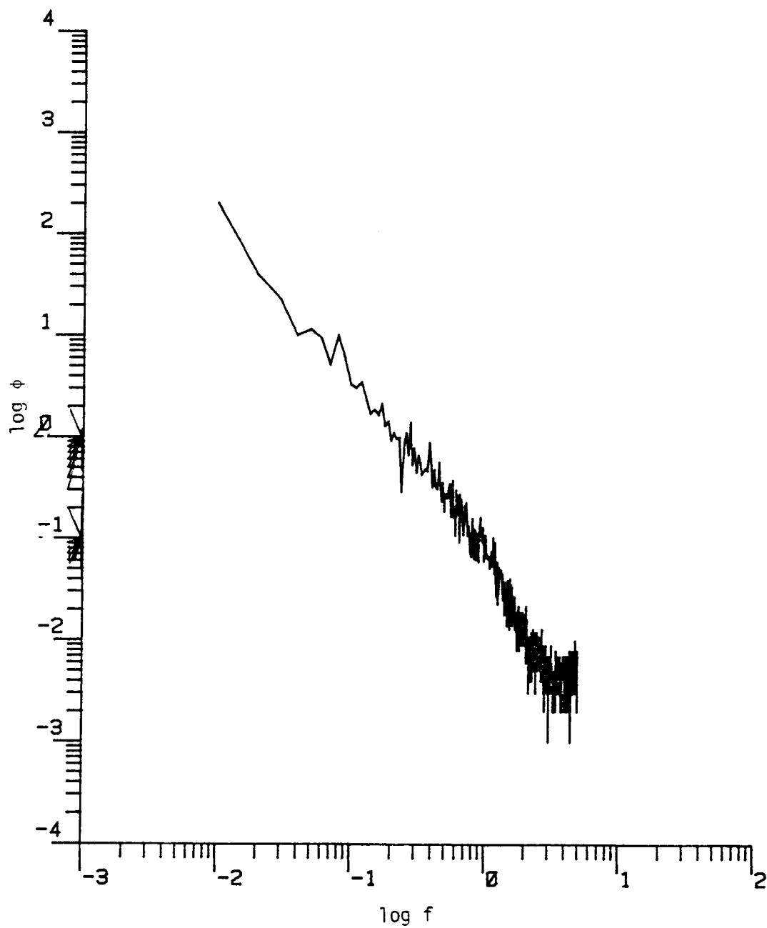
Figure D.14. The longitudinal power spectrum (Run #8623, T4L2, Component 1).
