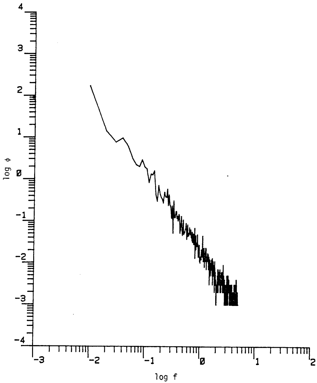
Figure D.58. The longitudinal power spectrum (Run #8624, S2L3, Component 1).
