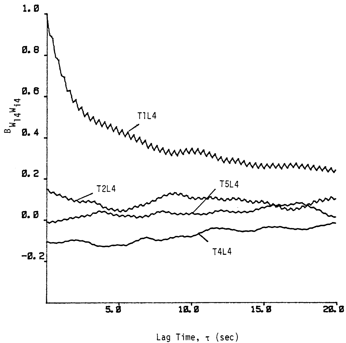
Figure E.5. Two-point horizontal space-time correlation relative to T1L4.
