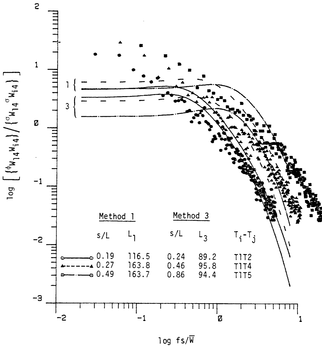
Figure 8.7. Comparison of computed two-point spatial spectra with the theoretical model of Houbolt and Sen (1972) (Run #8623, L4, Component 3).
