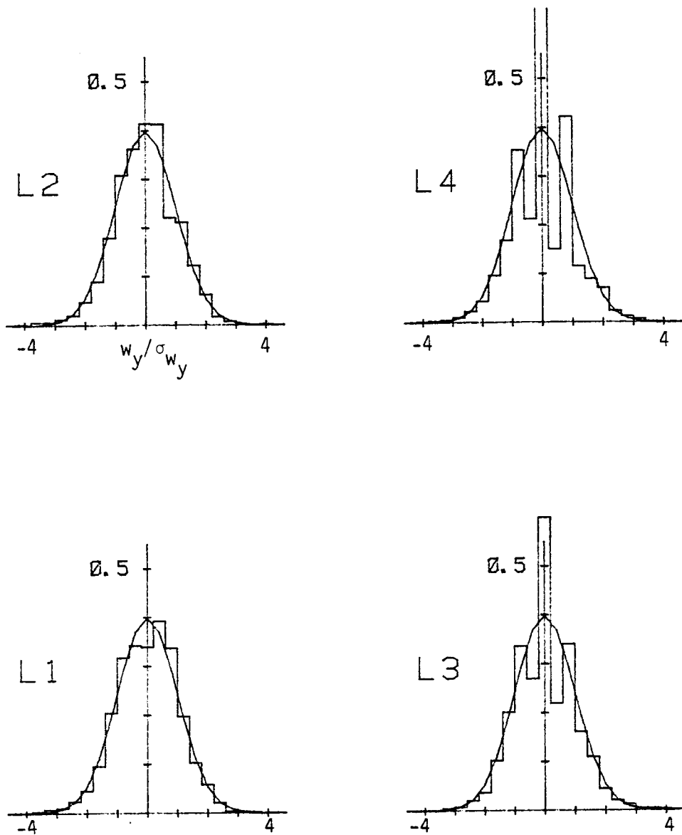
Figure C.29. Probability density function for lateral velocity component normalized with \sigma_{w_y} (Run #8624, T2, Component 2).
