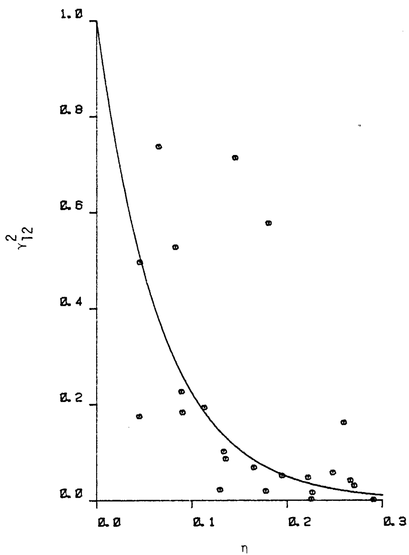
Figure 8.13. The lateral coherence \gamma_{12}^2 for the longitudinal velocity component at the 3-m level.
