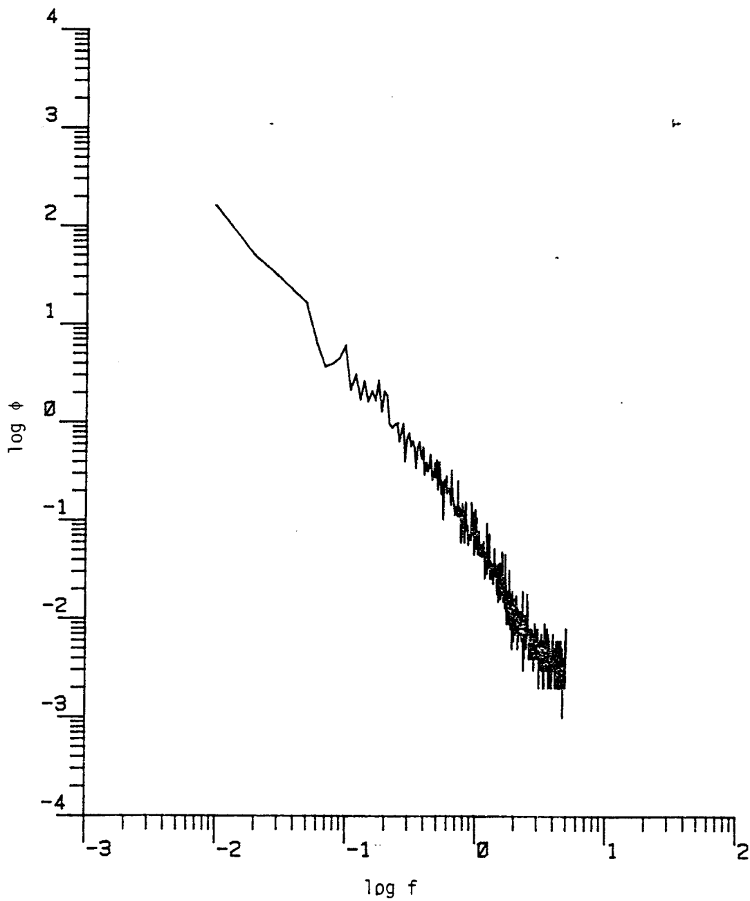
Figure D.2. The longitudinal power spectrum (Run #8623, T1L2, Component 1).
