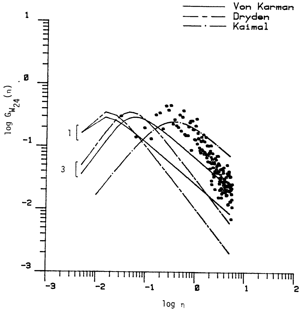
Figure 7.29. Comparison of vertical turbulence spectrum with three correlation models. (The length scale is calculated by Methods 1 and 3, Chapter V, T2, Run #8624).
