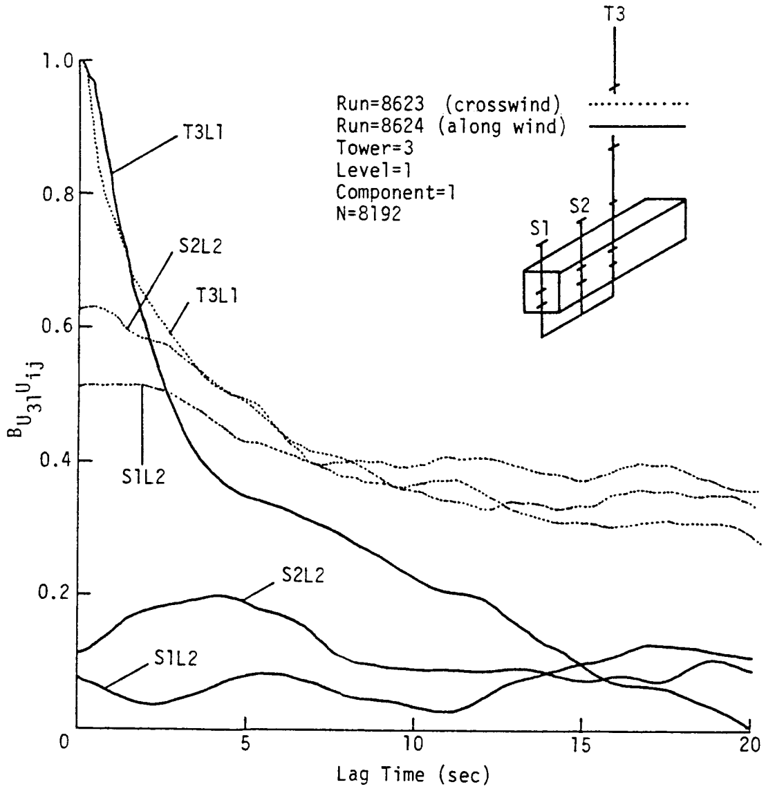
Figure 6.10. Two-point horizontal space-time correlation immediately behind the building and in the wake region relative to T3L1.
