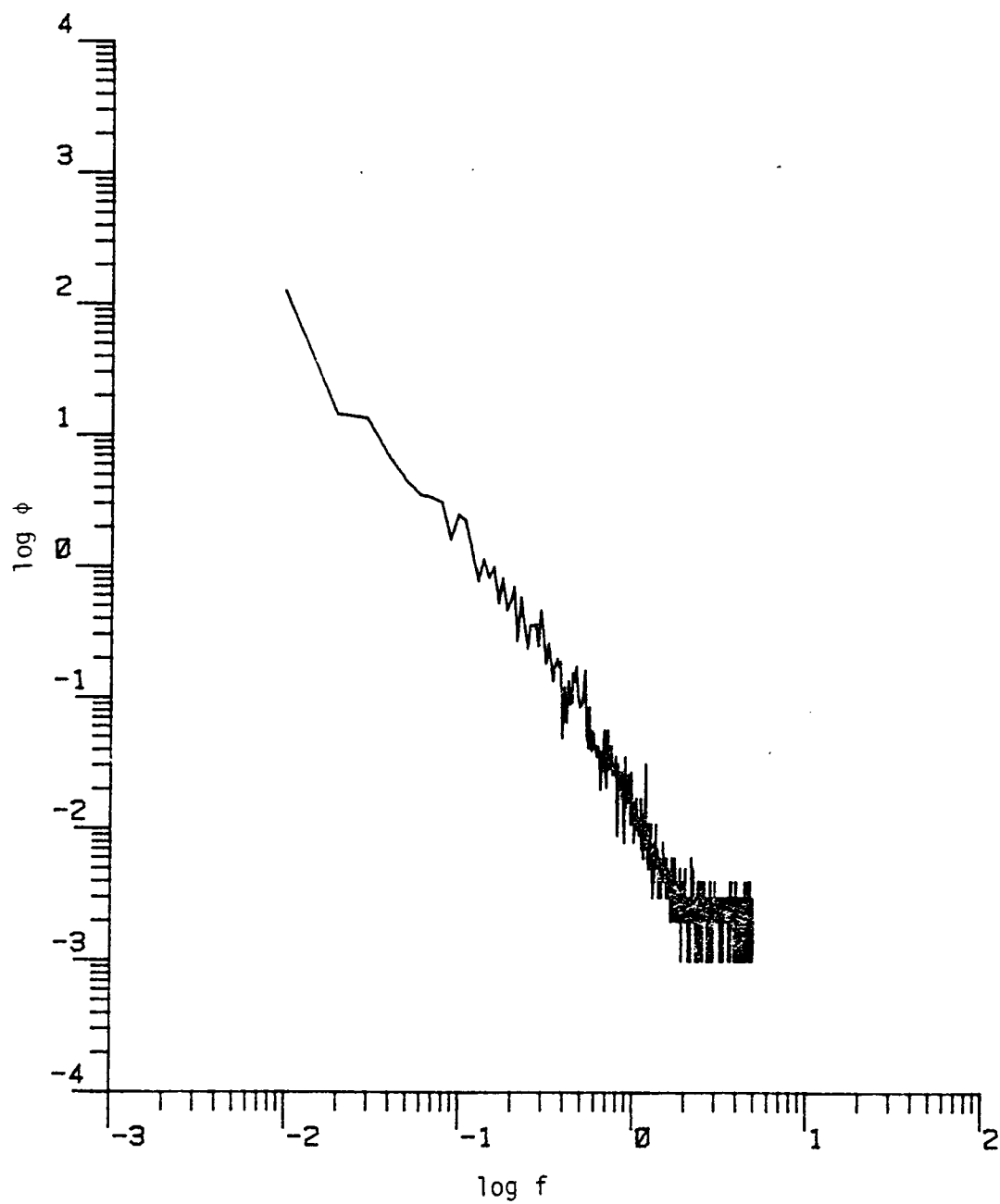
Figure D.34. The longitudinal power spectrum (Run #8624, T1L2, Component 1).
