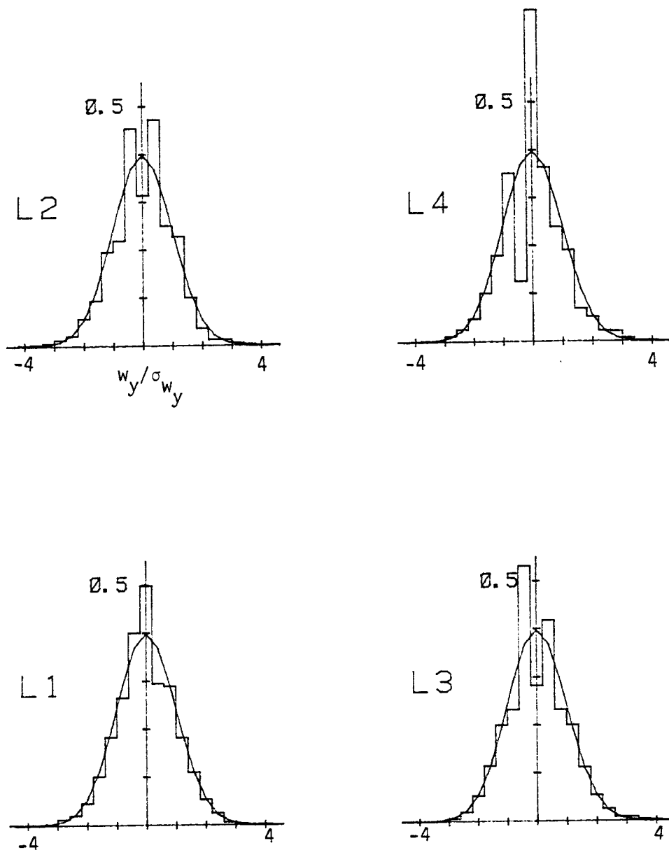
Figure C.22. Probability density function for lateral velocity component normalized with \sigma_{w_y} (Run #8623, T4, Component 2).
