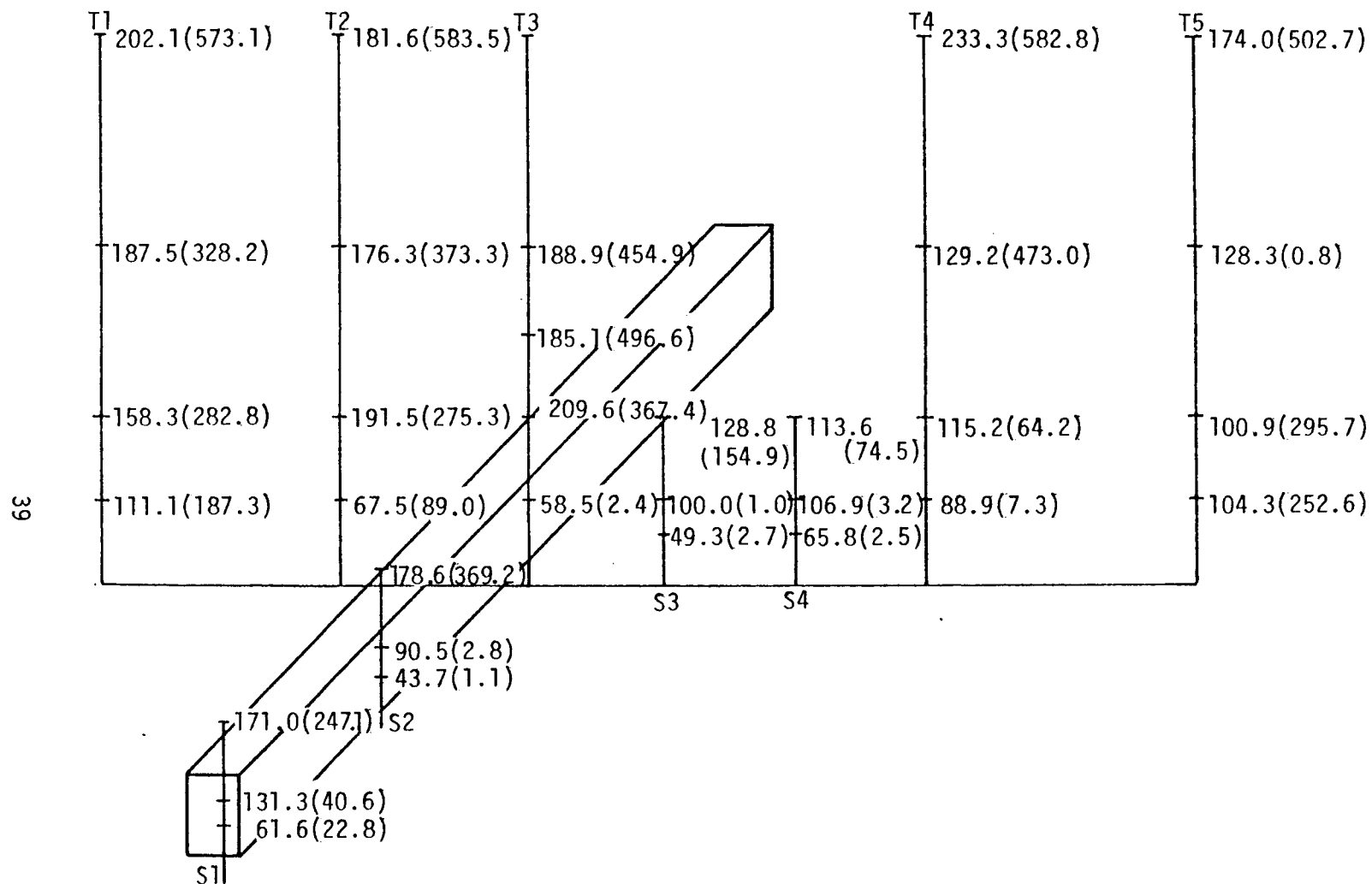
Figure 5.2. Spatial variation of the integral length scale in meters as computed by Method 2, Equation 5.2. (Component 1: Numbers not in parentheses, Run #8623, crosswind; numbers in parentheses, Run #8624, along wind).
