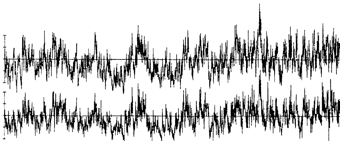
Figure B.4. Time history of turbulent fluctuations. (Run #8623, T4, Component 1).
