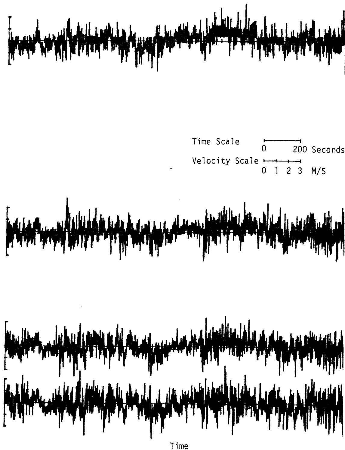
Figure B.38. Time history of turbulent fluctuations. (Run #8624, T2, Component 2).
