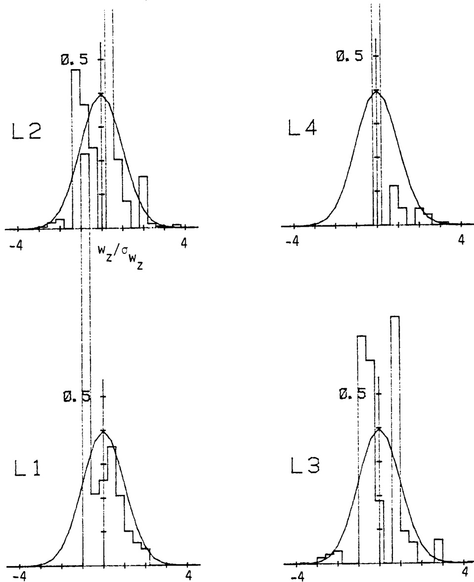
Figure C.48. Probability density function for vertical velocity component normalized with \sigma_{w_z} (Run #8624, T3, Component 3).
