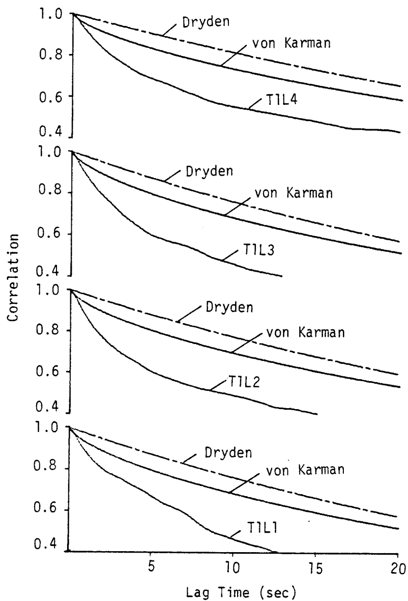
Figure 6.16. Comparison with von Karman and Dryden expressions for the longitudinal correlation (length scale L_1 , T1, Run #8624).
