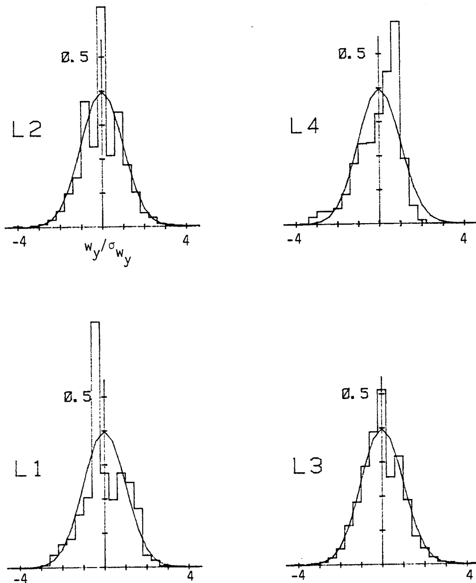
Figure C.30. Probability density function for lateral velocity component normalized with \sigma_{w_y} (Run #8624, T3, Component 2).
