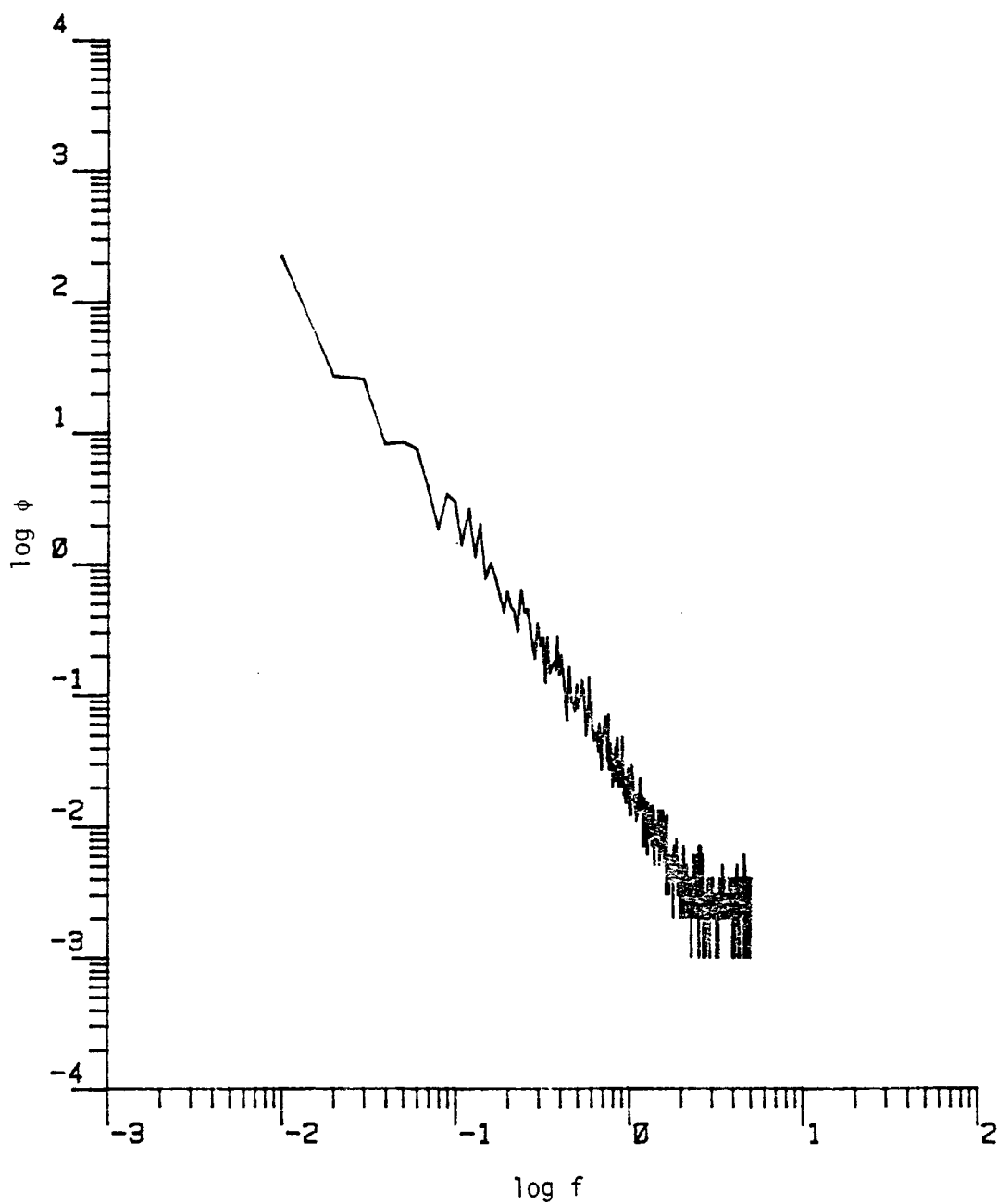
Figure D.40. The longitudinal power spectrum (Run #8624, T2L4, Component 1).
