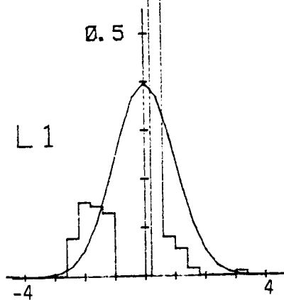
Figure C.51. Probability density function for vertical velocity component normalized with \sigma_{w_z} (Run #8624, S1, Component 3).
