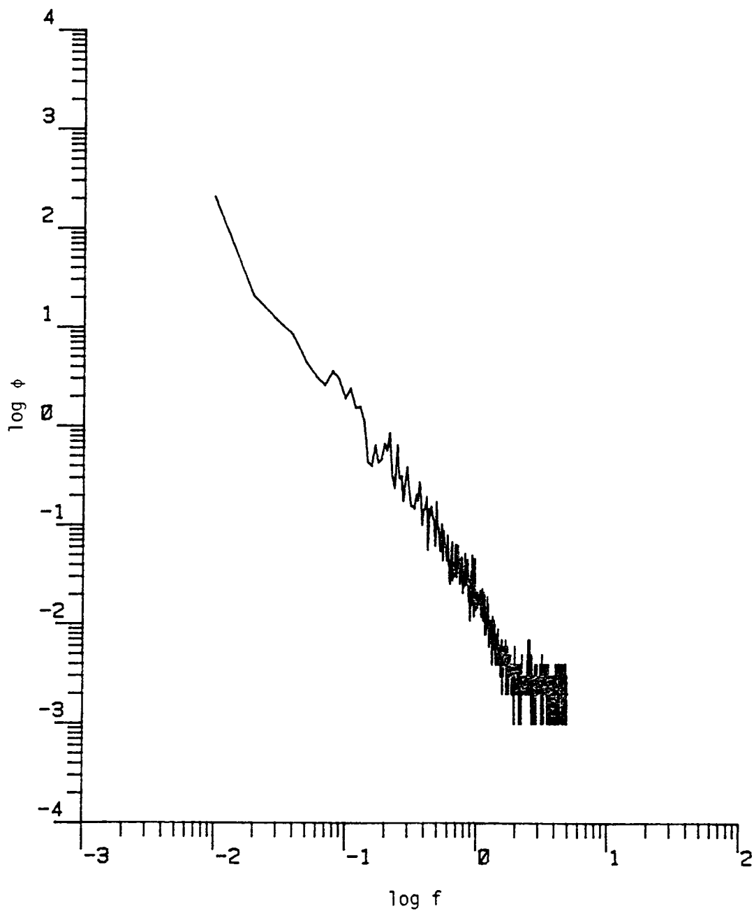
Figure D.50. The longitudinal power spectrum (Run #8624, T5L2, Component 1).
