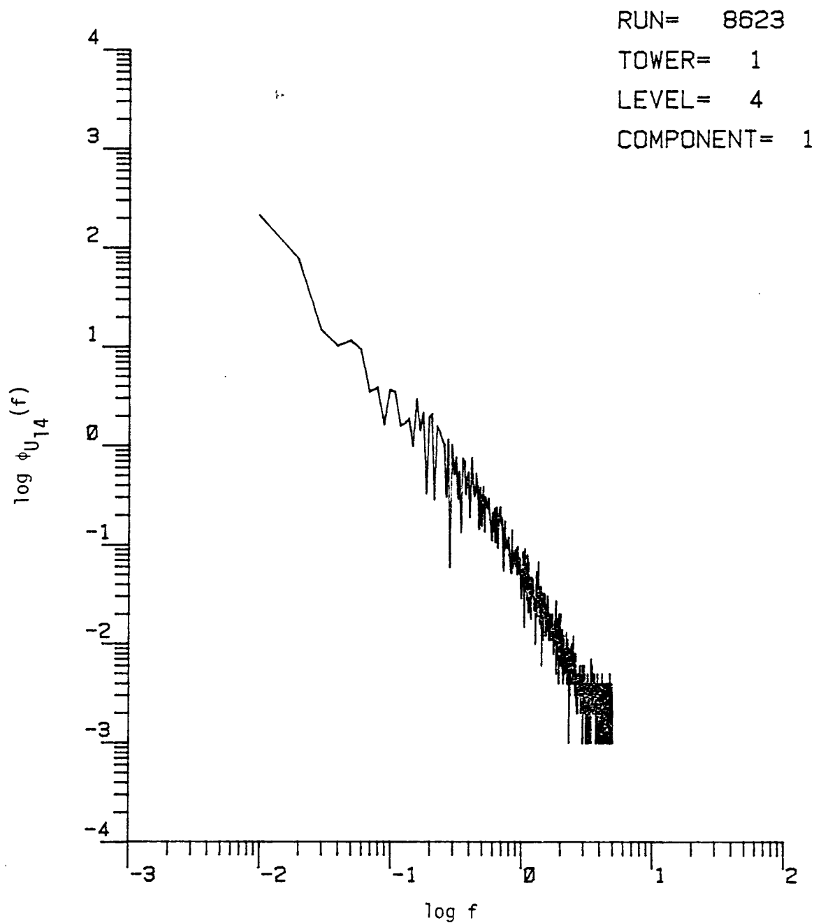
Figure 7.1. Power spectral density function calculated by the standard method (Equation 7.5).
