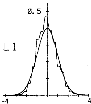
Figure C.7. Probability density function for longitudinal velocity component normalized with \sigma_{w_x} (Run #8623, S2, Component 1).
