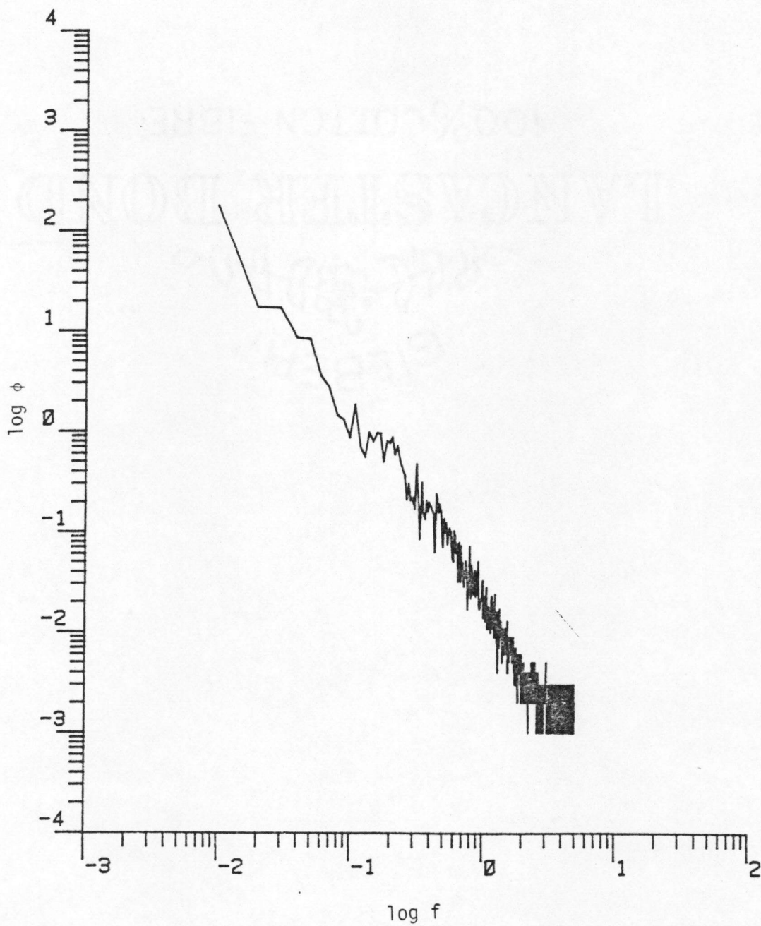
Figure D.43. The longitudinal power spectrum (Run #8624, T3L3, Component 1).
