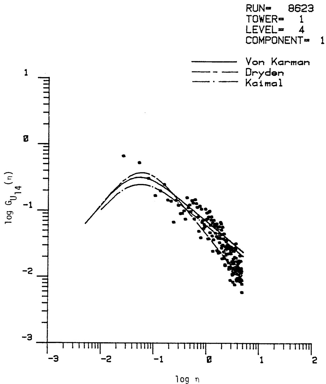
Figure 7.9. Comparison of longitudinal turbulence spectrum with three correlation models. (The length scale is calculated by Method 4, Chapter V, Run #8623).
