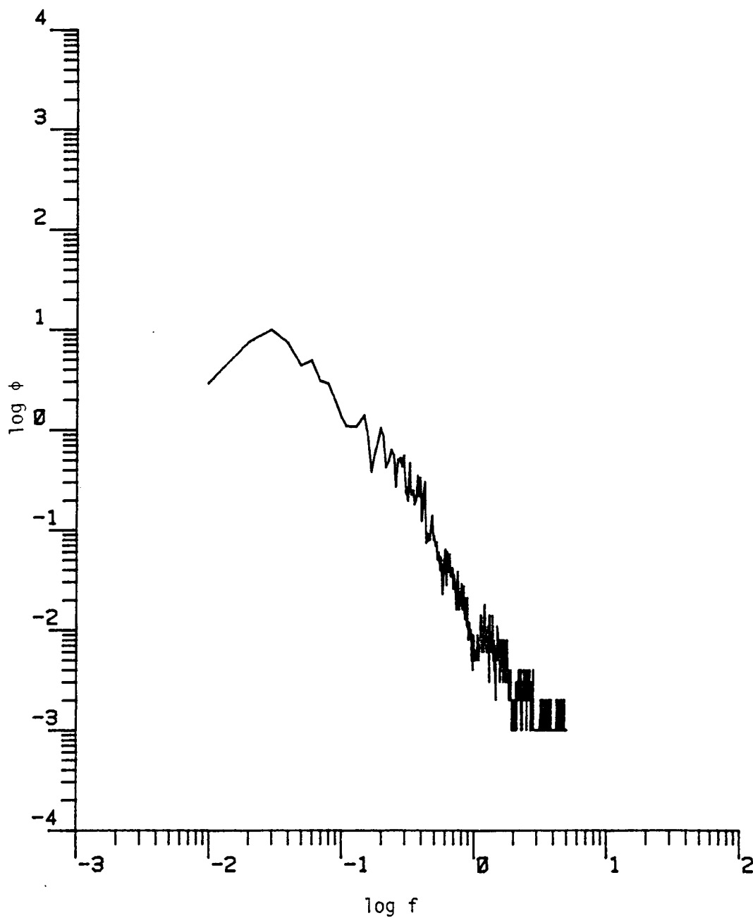
Figure D.57. The longitudinal power spectrum (Run #8624, S2L2, Component 1).
