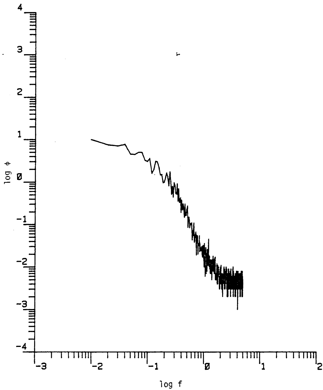
Figure D.59. The longitudinal power spectrum (Run #8624, S3L1, Component 1).
