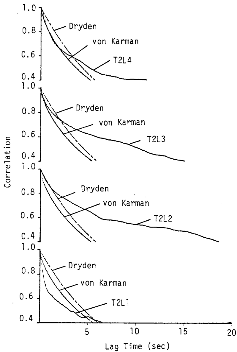
Figure 6.20. Comparison with von Karman and Dryden expressions for the longitudinal correlation (length scale L_4 , T2, Run #8623).
