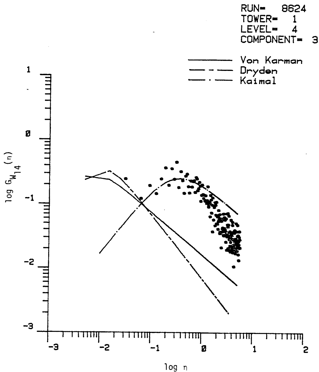
Figure 7.24. Comparison of vertical turbulence spectrum with three correlation models. (The length scale is calculated by Method 2, Chapter V, Run #8624).
