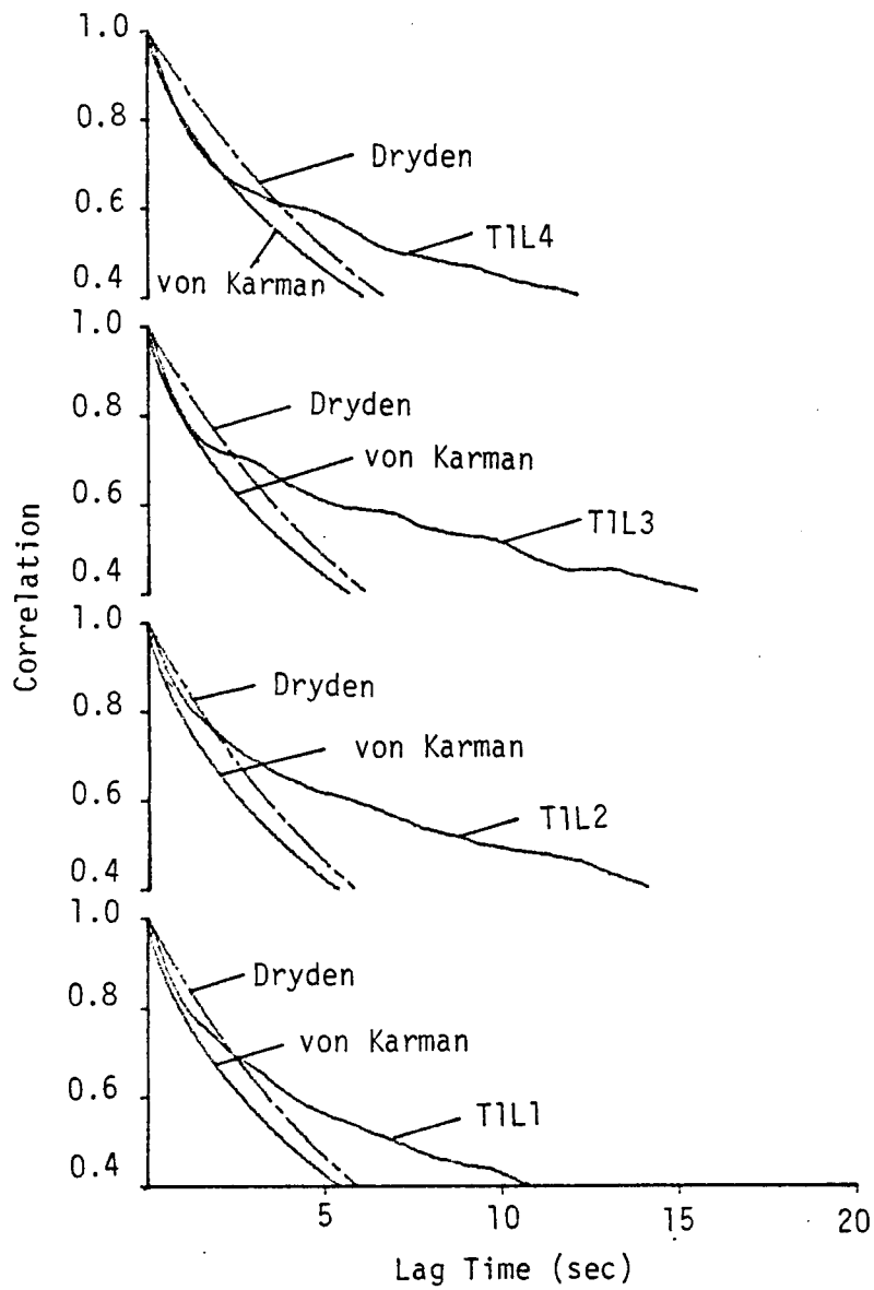
Figure 6.19. Comparison with von Karman and Dryden expressions for the longitudinal correlation (length scale L_4 , T1, Run #8623).
