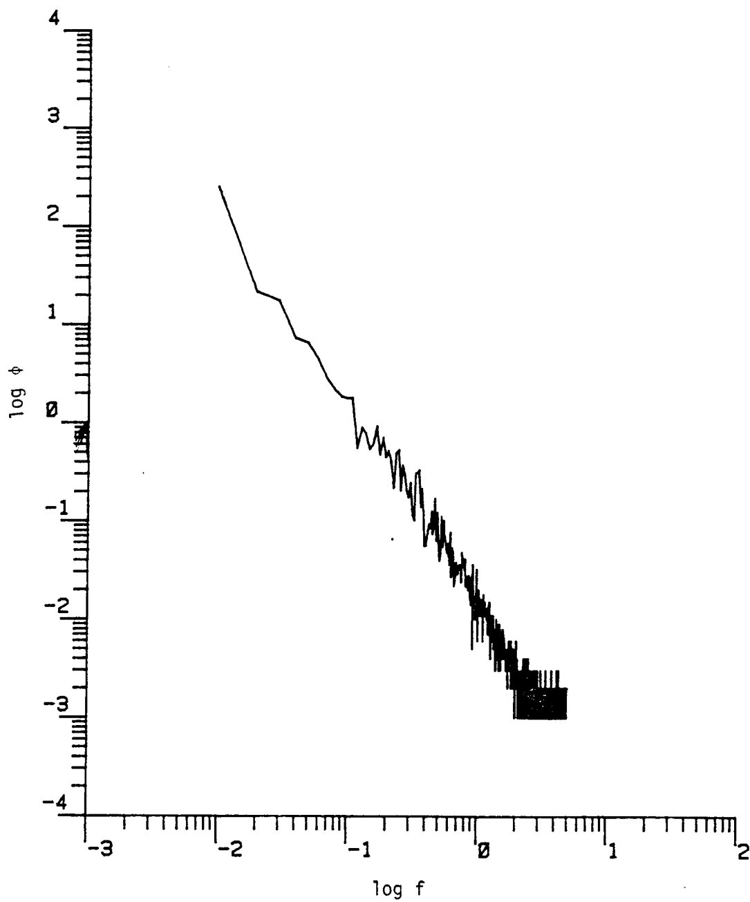
Figure D.47. The longitudinal power spectrum (Run #8624, T4L3, Component 1).
