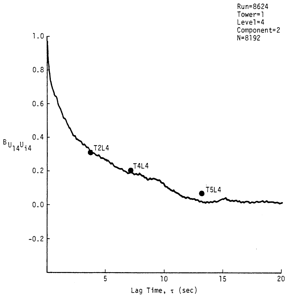
Figure 6.12. Illustration of validity of Taylor's hypothesis (● spatial correlation converted to a time correlation with the relationship \lambda = \bar{W}\tau ).
