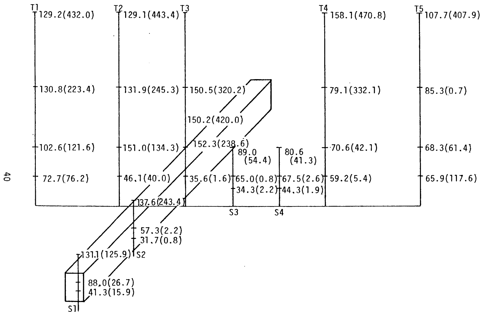
Figure 5.3. Spatial variation of the integral length scale in meters as computed by Method 2, Equation 5.3. (Component 1: Numbers not in parentheses, Run #8623, crosswind; numbers in parentheses, Run #8624, along wind).
