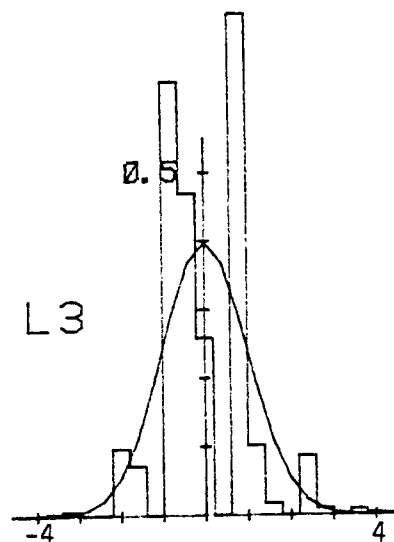
Figure C.53. Probability density function for vertical velocity component normalized with \sigma_{w_z} (Run #8624, S3, Component 3).
