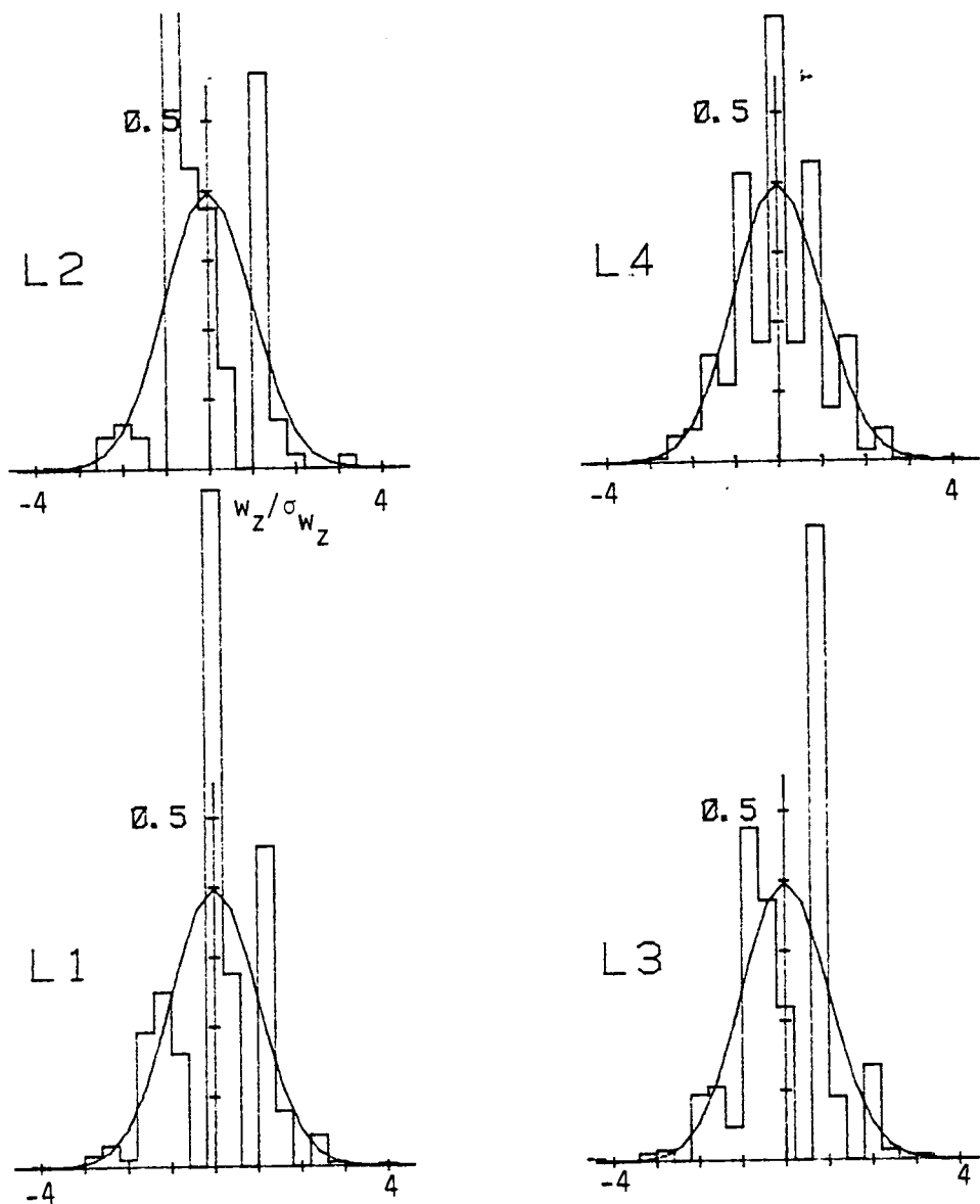
Figure C.38. Probability density function for vertical velocity component normalized with \sigma_{w_z} (Run #8623, T2, Component 3).
