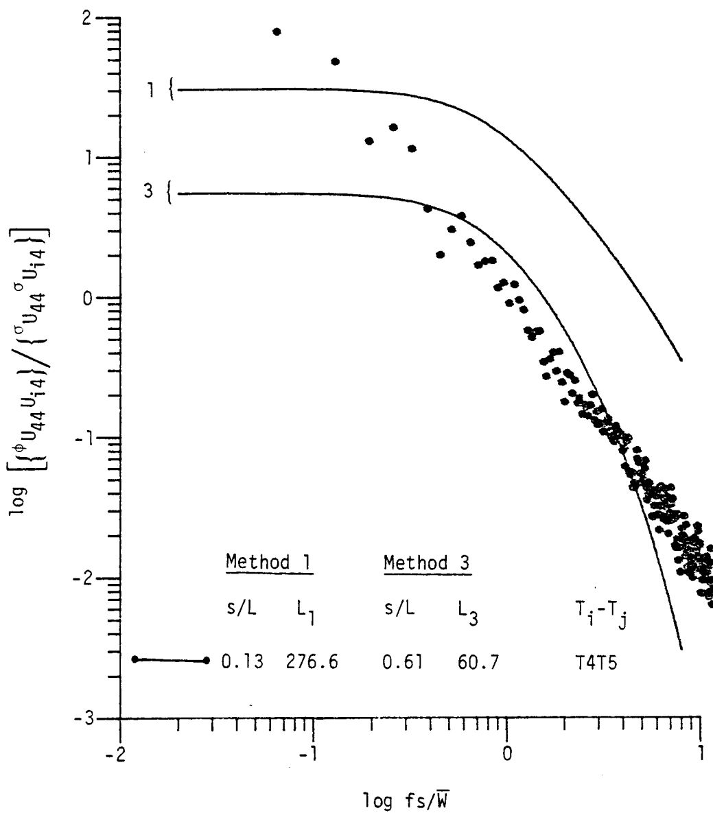
Figure 8.6. Comparison of computed two-point spatial spectra with the theoretical model of Houbolt and Sen (1972) (Run #8624, L4, Component 1).
