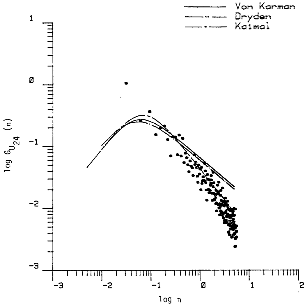
Figure 7.17. Comparison of longitudinal turbulence spectra with three analytical models. (The length scale is calculated by Method 4, T2).
