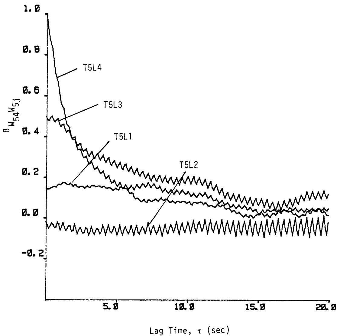
Figure E.4. Two-point vertical space-time correlation relative to T5L4.
