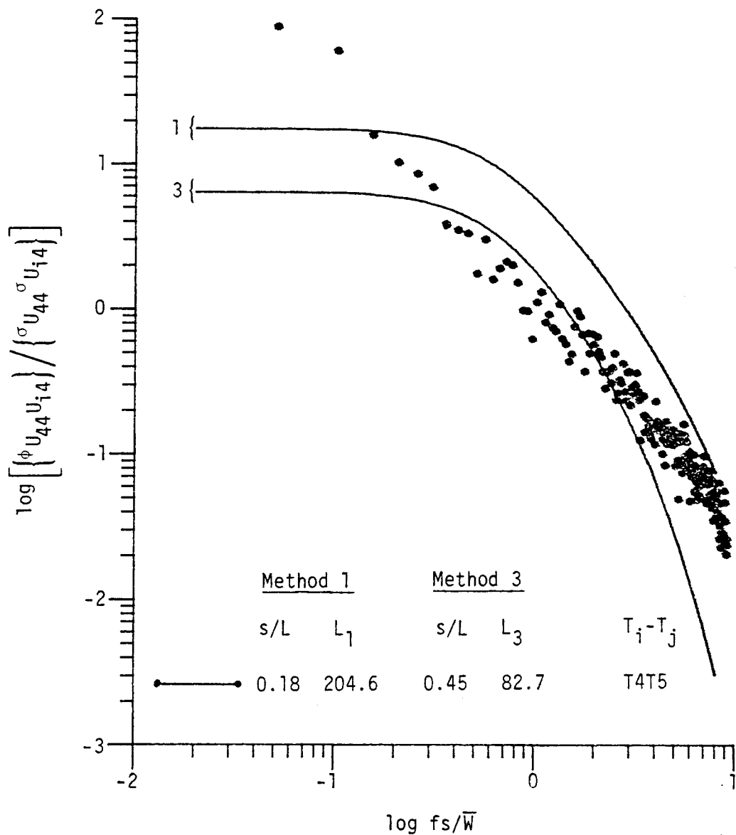
Figure 8.3. Comparison of computed two-point spatial spectra with the theoretical model of Houbolt and Sen (1972) (Run #8623, L4, Component 1).
