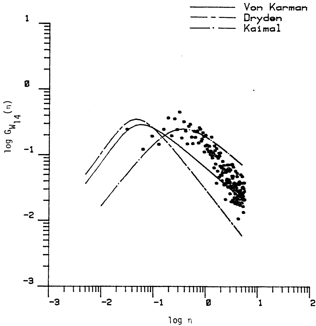
Figure 7.25. Comparison of vertical turbulence spectrum with three correlation models. (The length scale is calculated by Method 3, Chapter V, Run #8624).
