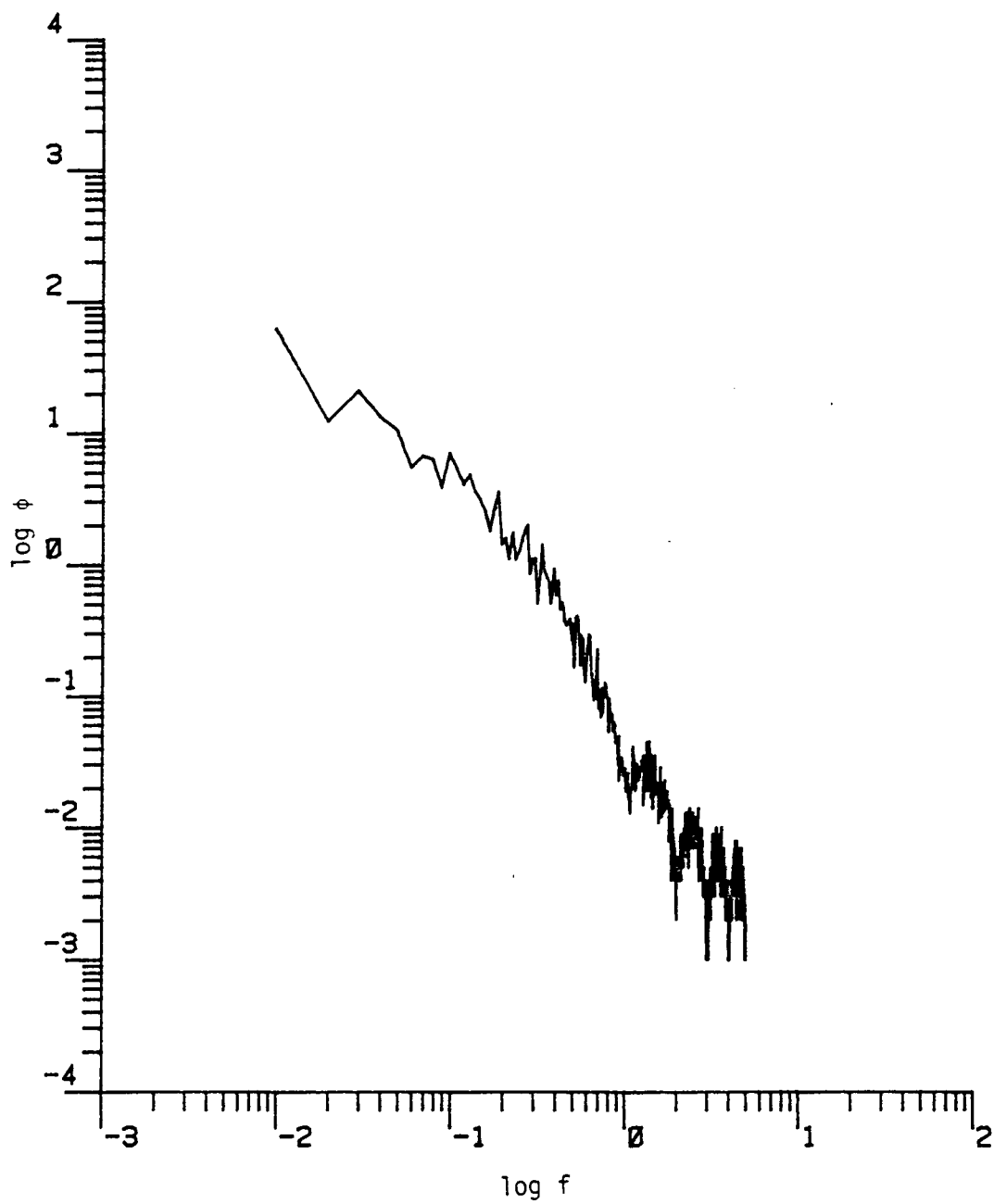
Figure D.62. The longitudinal power spectrum (Run #8624, S4L1, Component 1).
