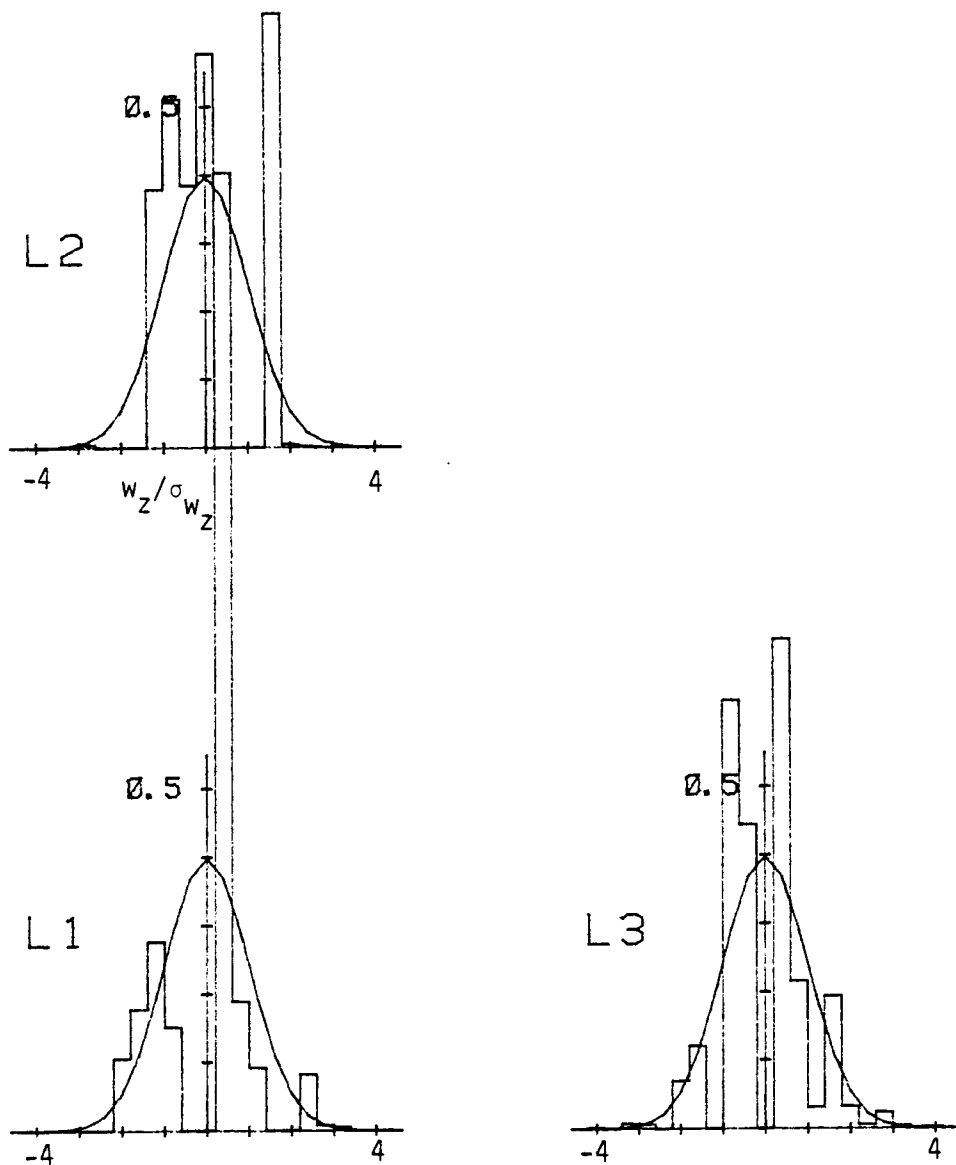
Figure C.52. Probability density function for vertical velocity component normalized with \sigma_{w_z} (Run #8624, S2, Component 3).
