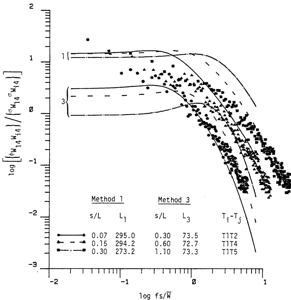
Figure 8.10. Comparison of computed two-point spatial spectra with the theoretical model of Houbolt and Sen (1972) (Run #8624, L4, Component 3).
