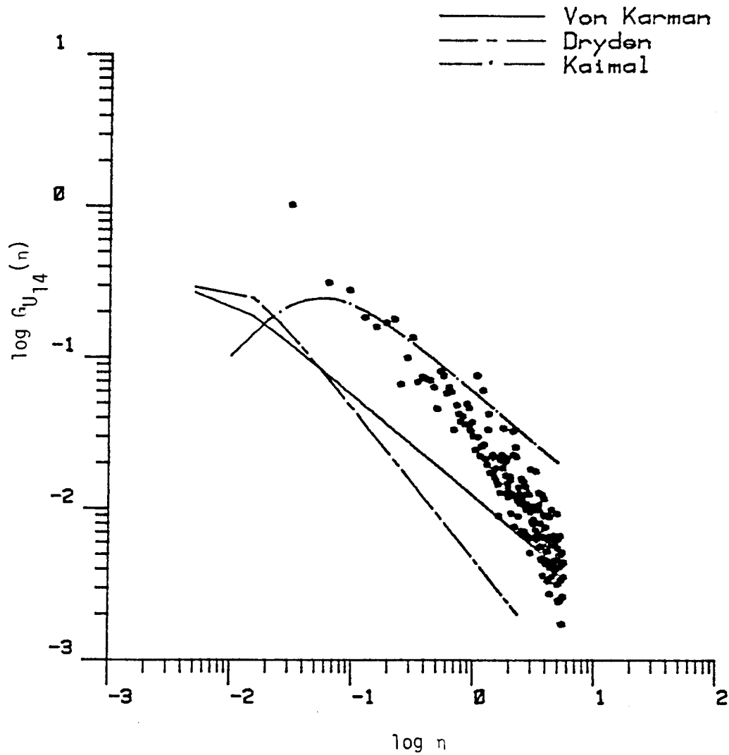
Figure 7.11. Comparison of longitudinal turbulence spectrum with three correlation models. (The length scale is calculated by Method 2, Chapter V, Run #8624).
