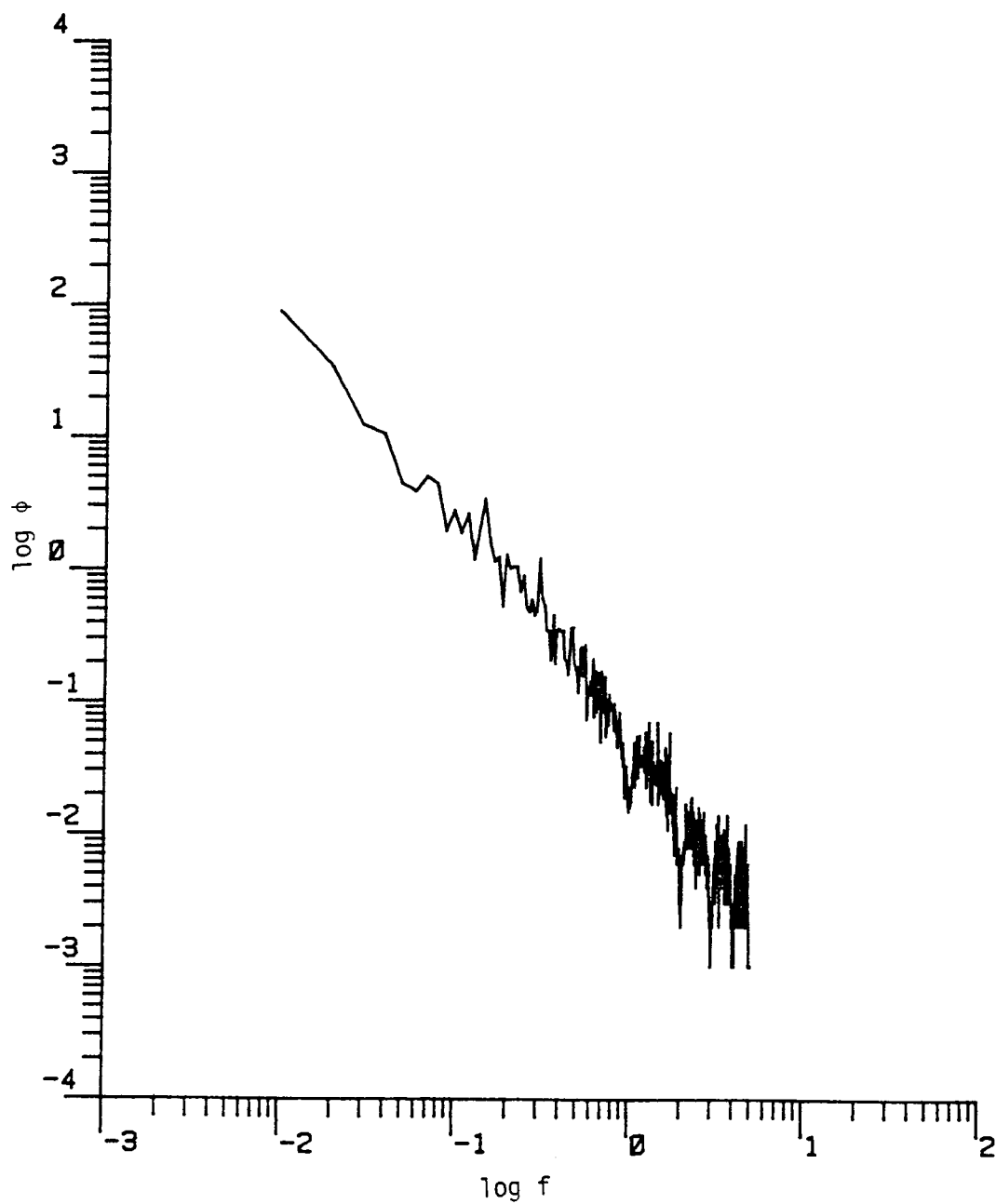
Figure D.30. The longitudinal power spectrum (Run #8623, S4L1, Component 1).
