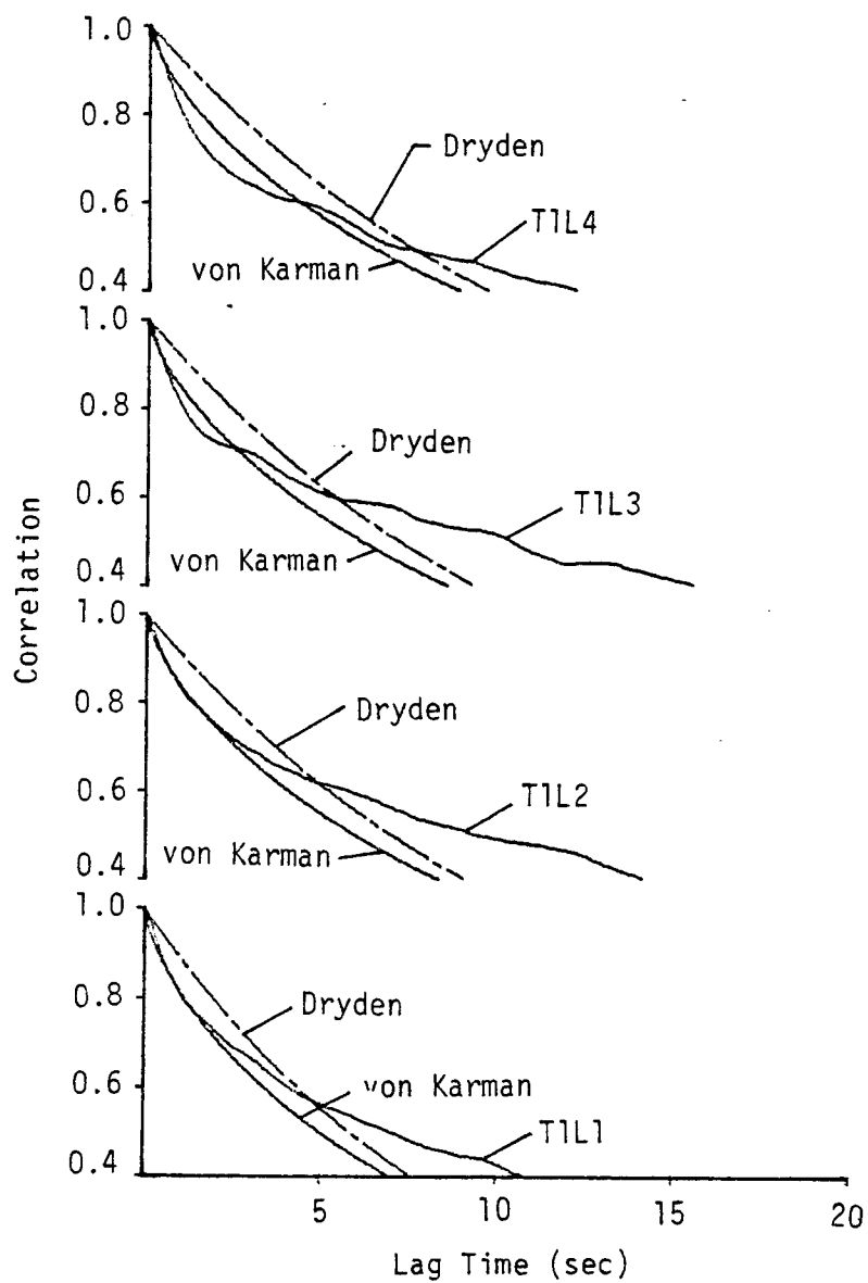
Figure 6.13. Comparison with von Karman and Dryden expressions for the longitudinal correlation (length scale L_1 , T1, Run #8623).
