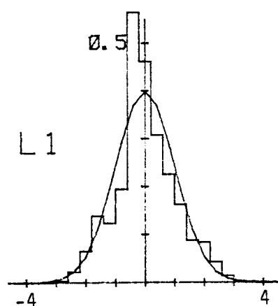
Figure C.15. Probability density function for longitudinal velocity component normalized with \sigma_{w_x} (Run #8624, S1, Component 1).
