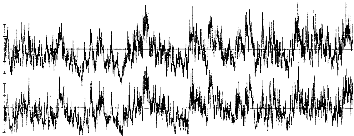
Figure B.1. Time history of turbulent fluctuations. (Run #8623, T1, Component 1).
