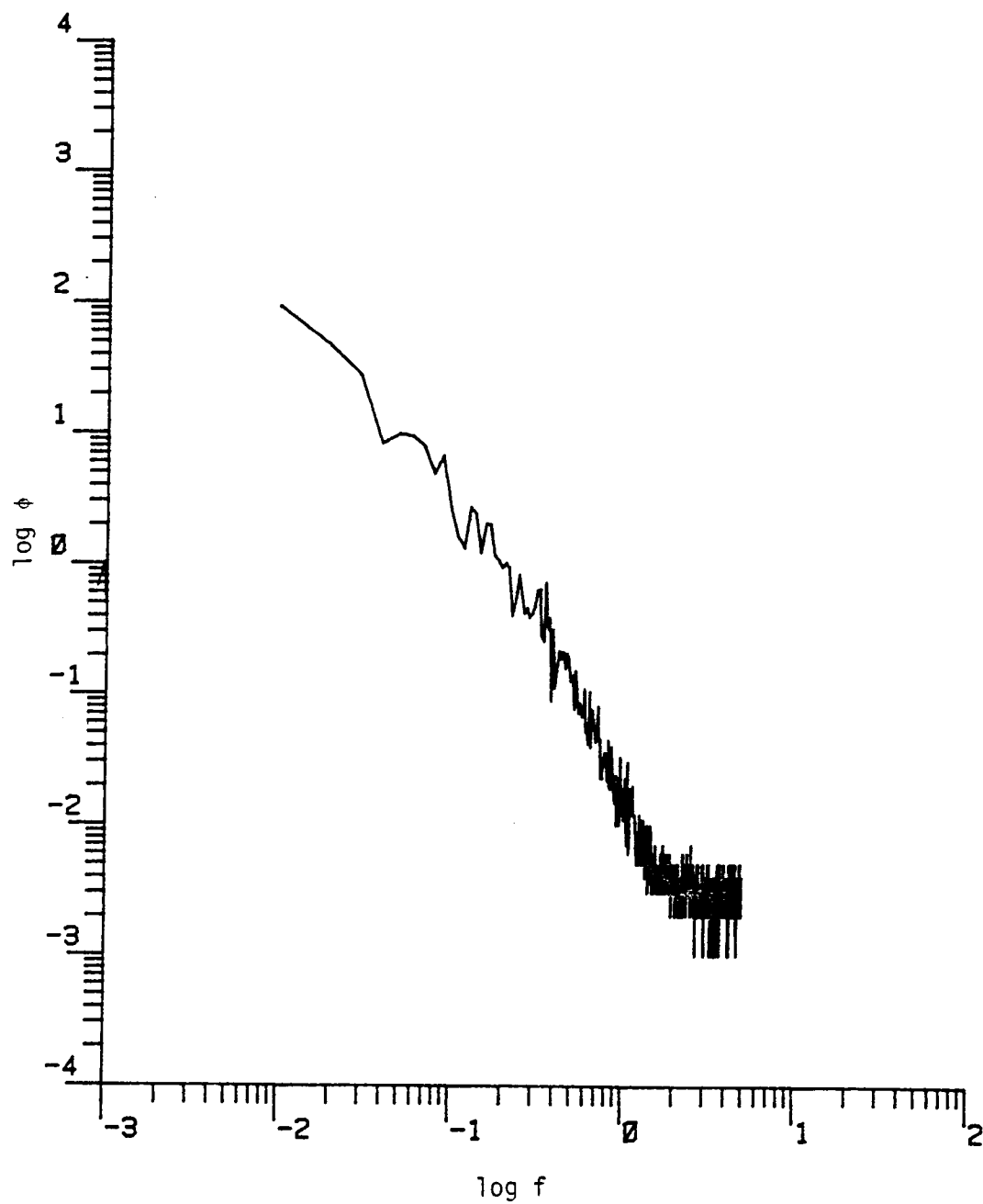
Figure D.53. The longitudinal power spectrum (Run #8624, S1L1, Component 1).
