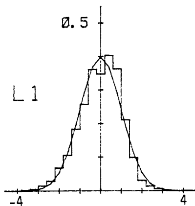
Figure C.21. Probability density function for lateral velocity component normalized with \sigma_{w_y} (Run #8623, T3, Component 2).
