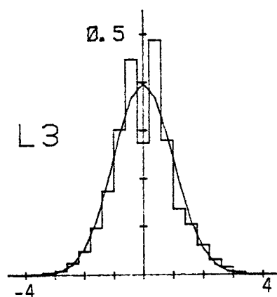
Figure C.34. Probability density function for lateral velocity component normalized with \sigma_{w_y} (Run #8624, S2, Component 2).
