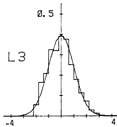
Figure C.12. Probability density function for longitudinal velocity component normalized with \sigma_{w_x} (Run #8624, T3, Component 1).
