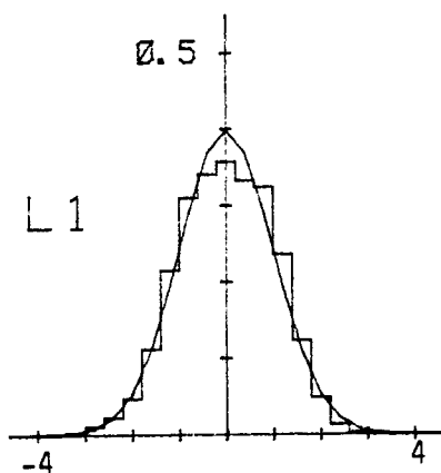
Figure C.20. Probability density function for lateral velocity component normalized with \sigma_{w_y} (Run #8623, T2, Component 2).
