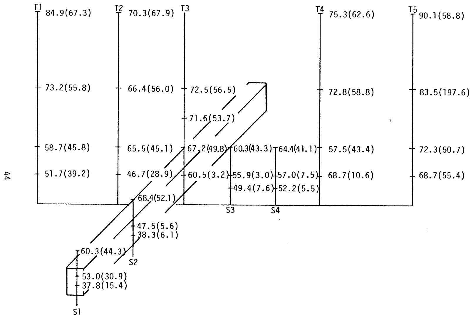
Figure 5.5. Spatial variation of the integral length scale in meters as computed by Method 3, Equation 5.6. (Component 1: Numbers not in parentheses, Run #8623, crosswind; numbers in parentheses, Run #8624, along wind).
