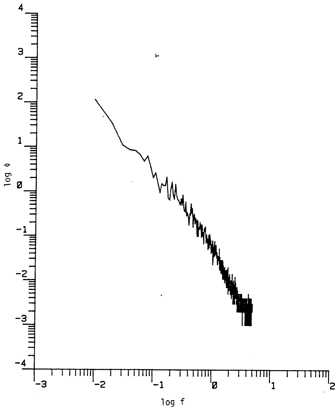
Figure D.13. The longitudinal power spectrum (Run #8623, T4L1, Component 1).
