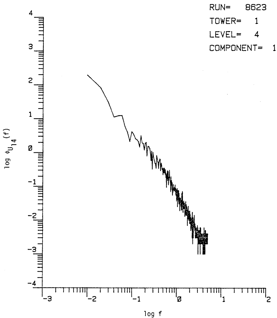
Figure 7.3. Power spectral density function calculated by the FFT method with a cosine tapering window.
