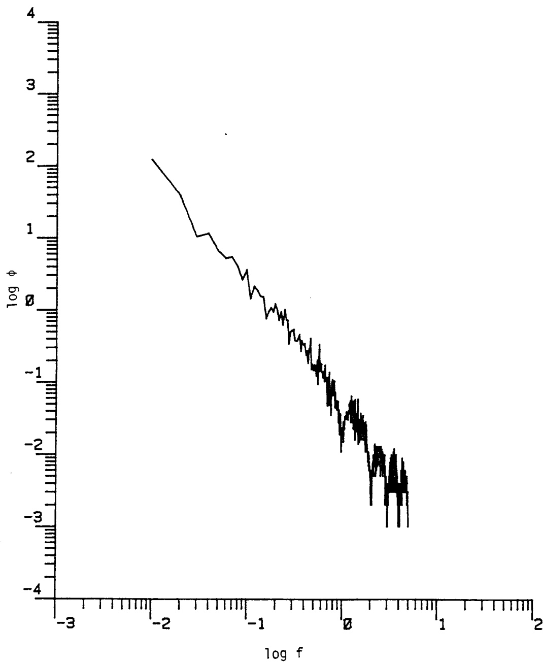
Figure D.31. The longitudinal power spectrum (Run #8623, S4L2, Component 1).
