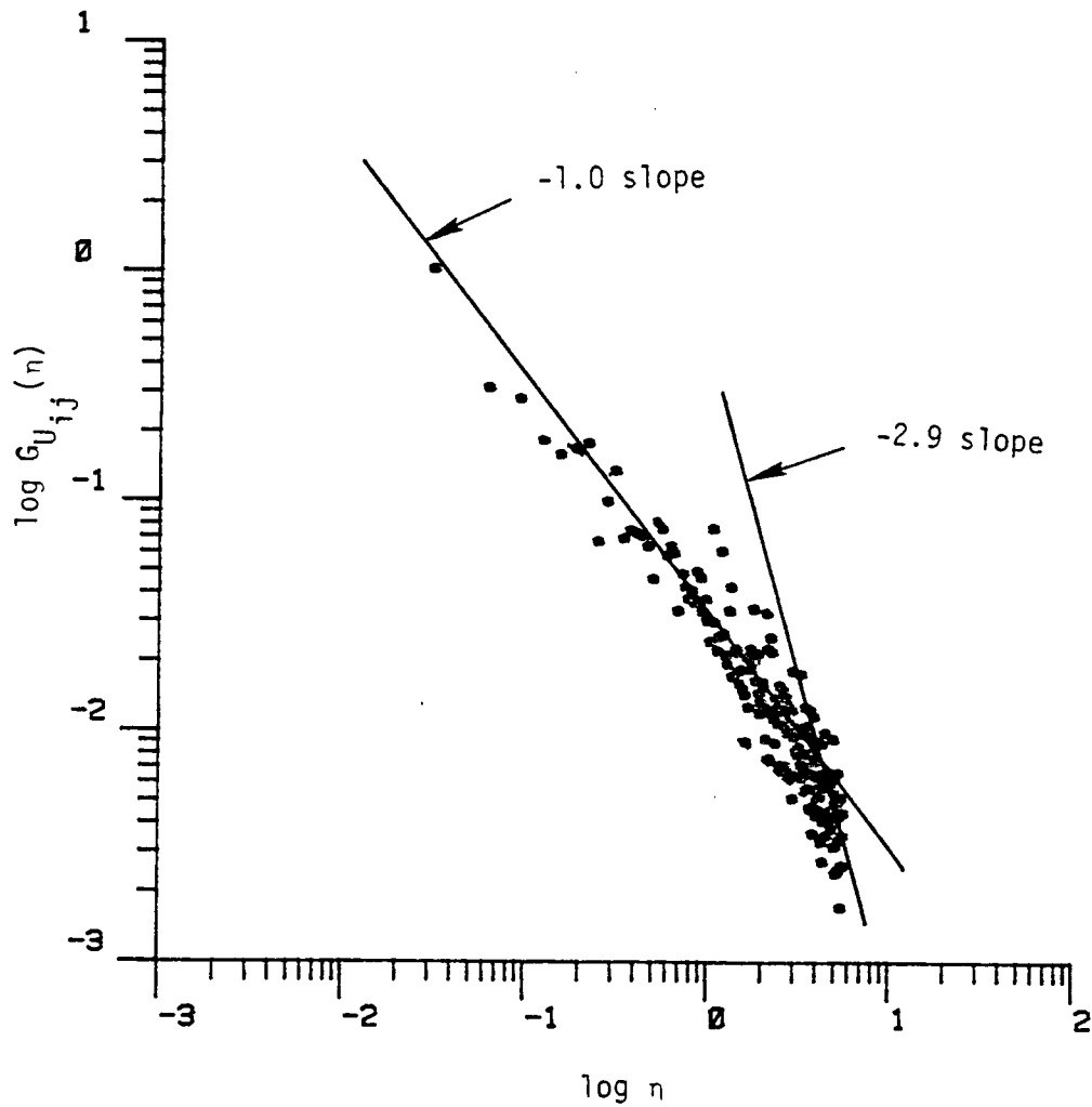
Figure 7.5. Characteristic slope of spectra is -1 at L4 for Run #8624.
