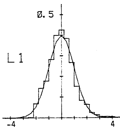
Figure C.14. Probability density function for longitudinal velocity component normalized with \sigma_{w_x} (Run #8624, T5, Component 1).
