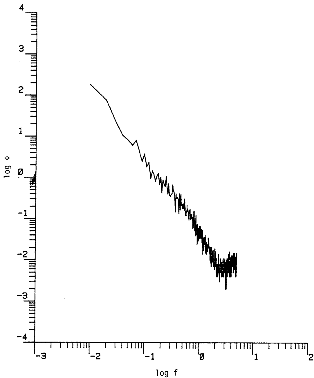
Figure D.10. The longitudinal power spectrum (Run #8623, T3L2, Component 1).
