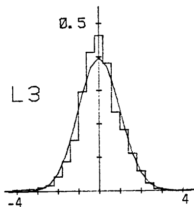
Figure C.18. Probability density function for longitudinal velocity component normalized with \sigma_{w_x} (Run #8624, S4, Component 1).
