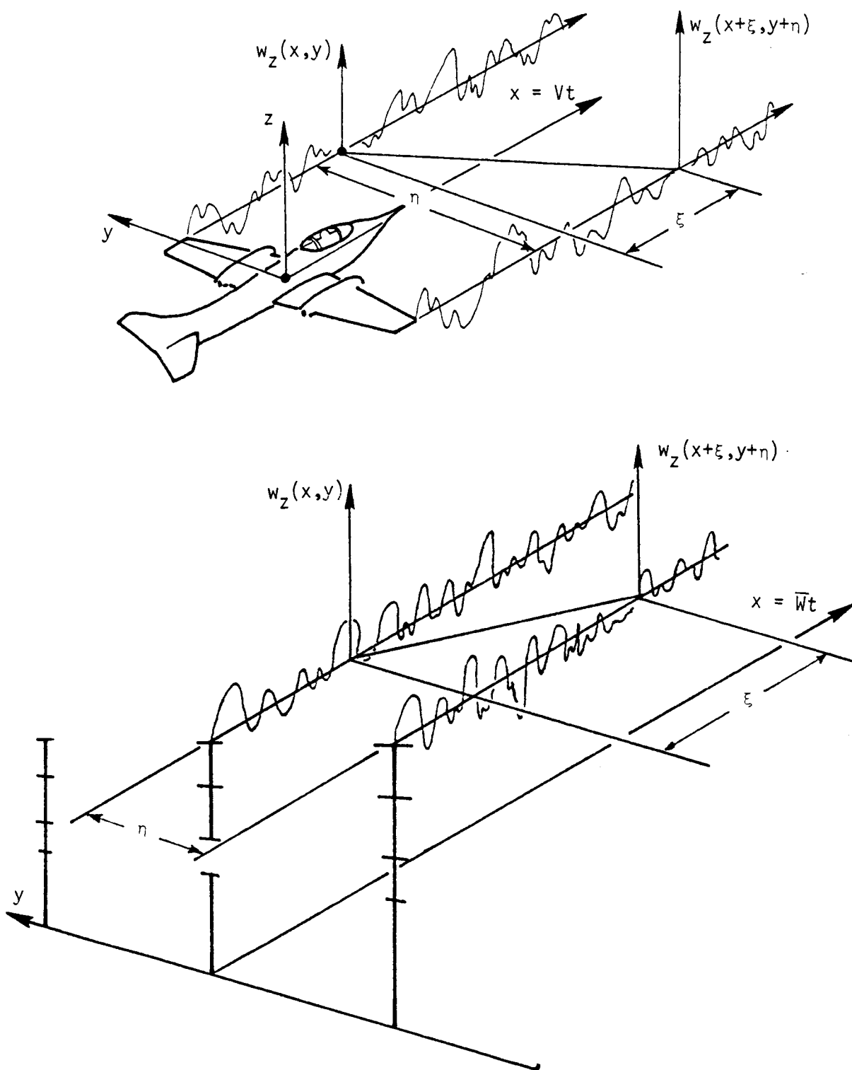
Figure 2.1. Illustration of coordinate system for either the aircraft or the tower array.
