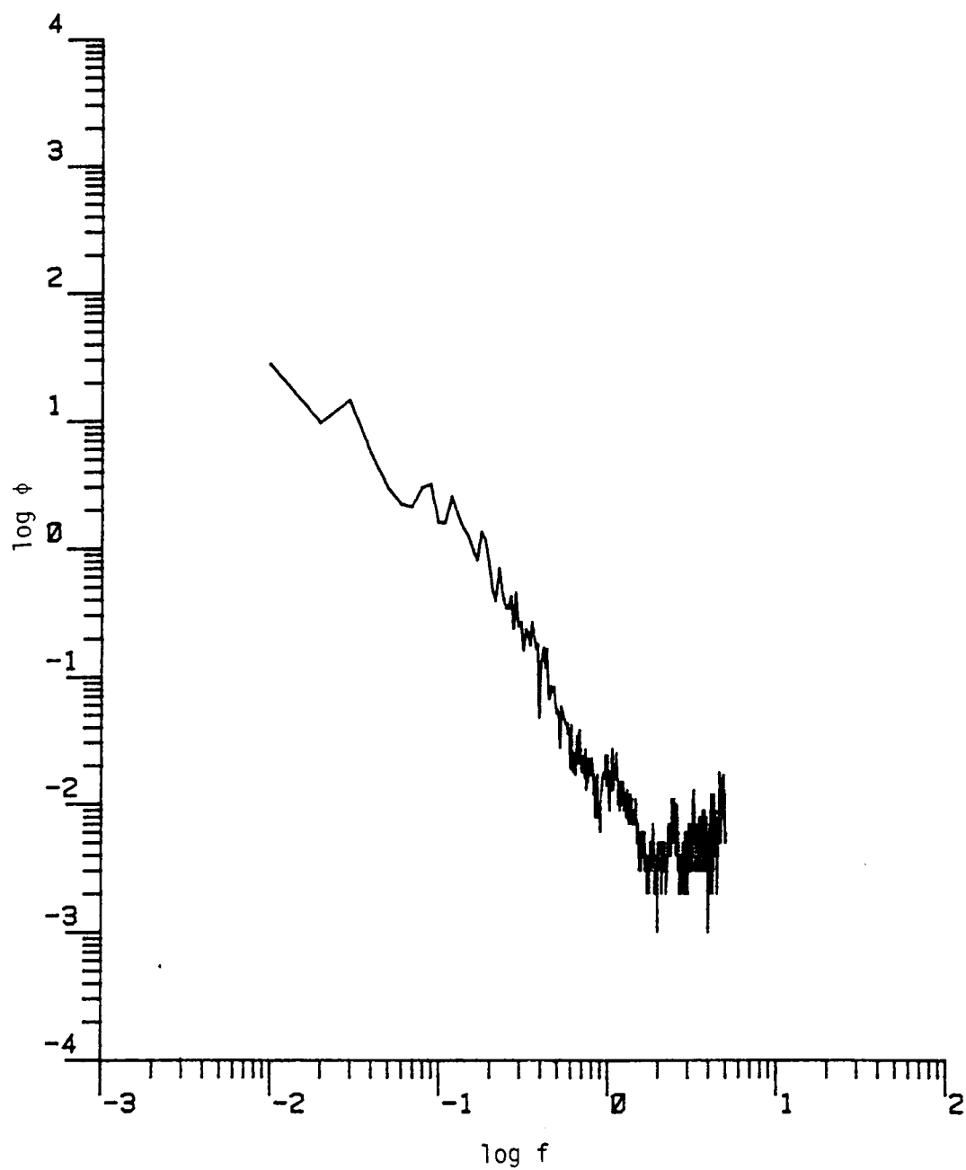
Figure D.41. The longitudinal power spectrum (Run #8624, T3L1, Component 1).
