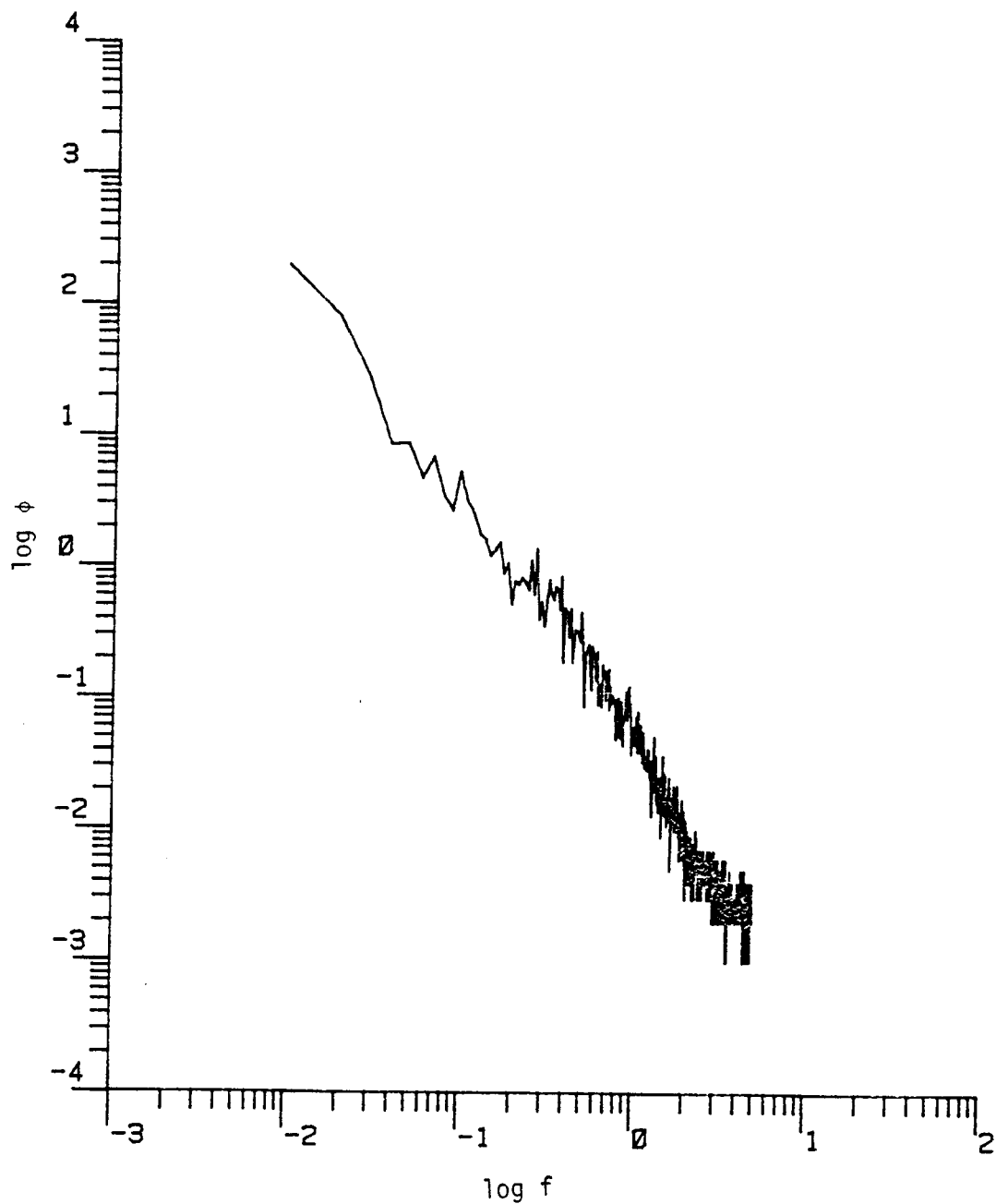
Figure D.12. The longitudinal power spectrum (Run #8623, T3L4, Component 1).
