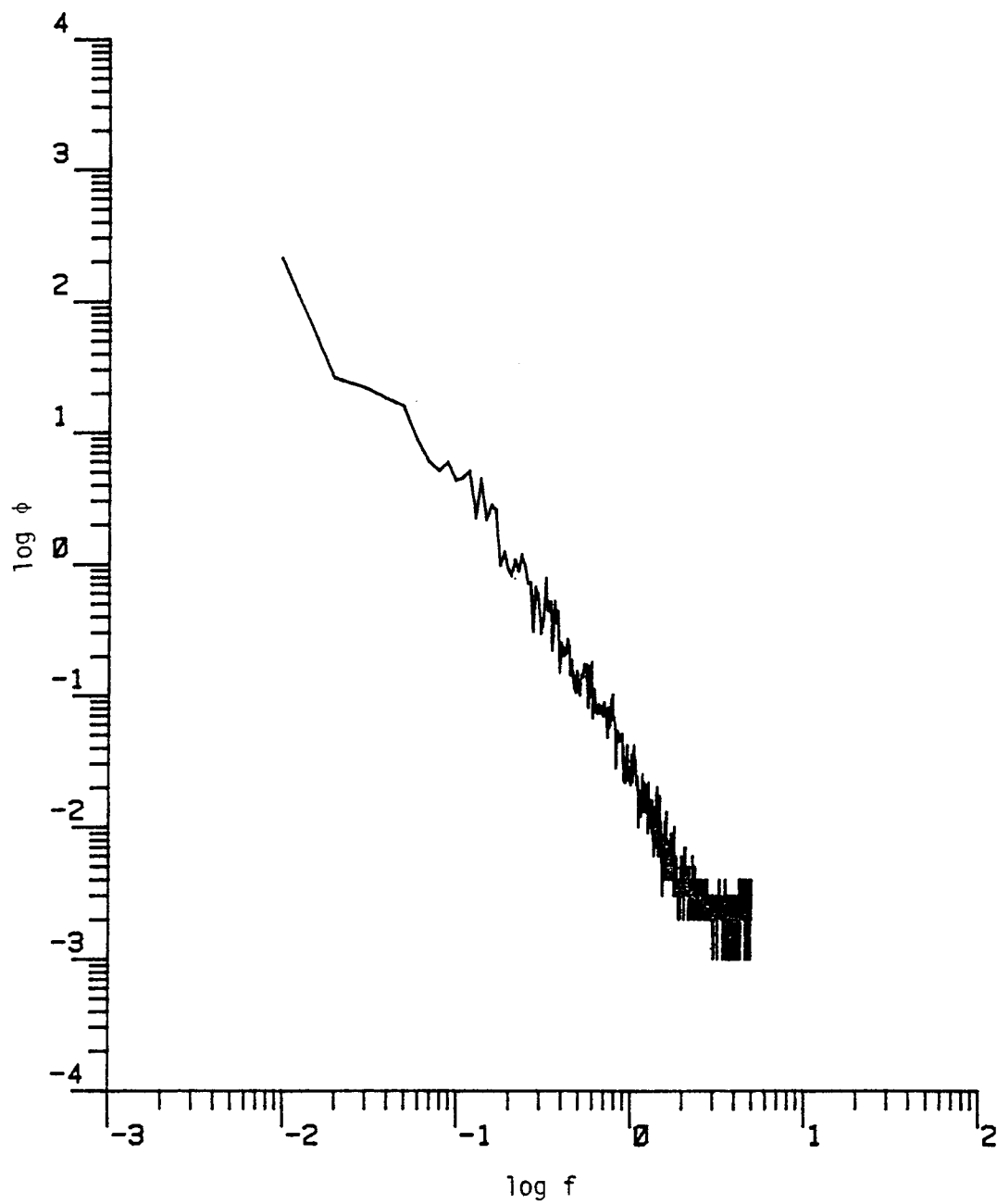
Figure D.46. The longitudinal power spectrum (Run #8624, T4L2, Component 1).
