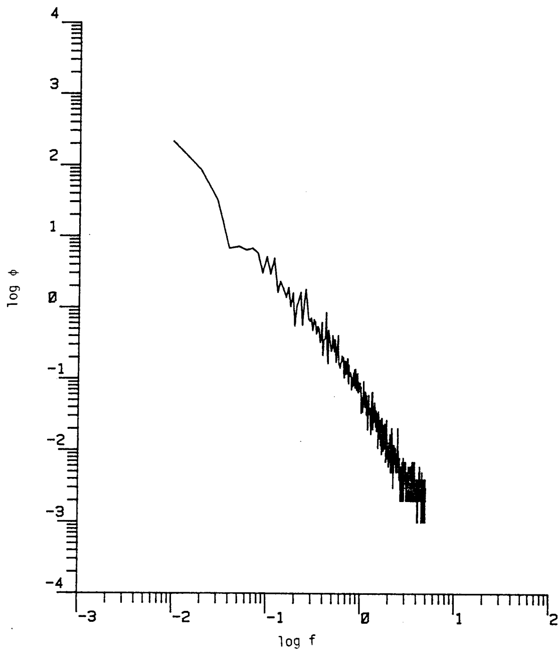
Figure D.11. The longitudinal power spectrum (Run #8623, T3L3, Component 1).
