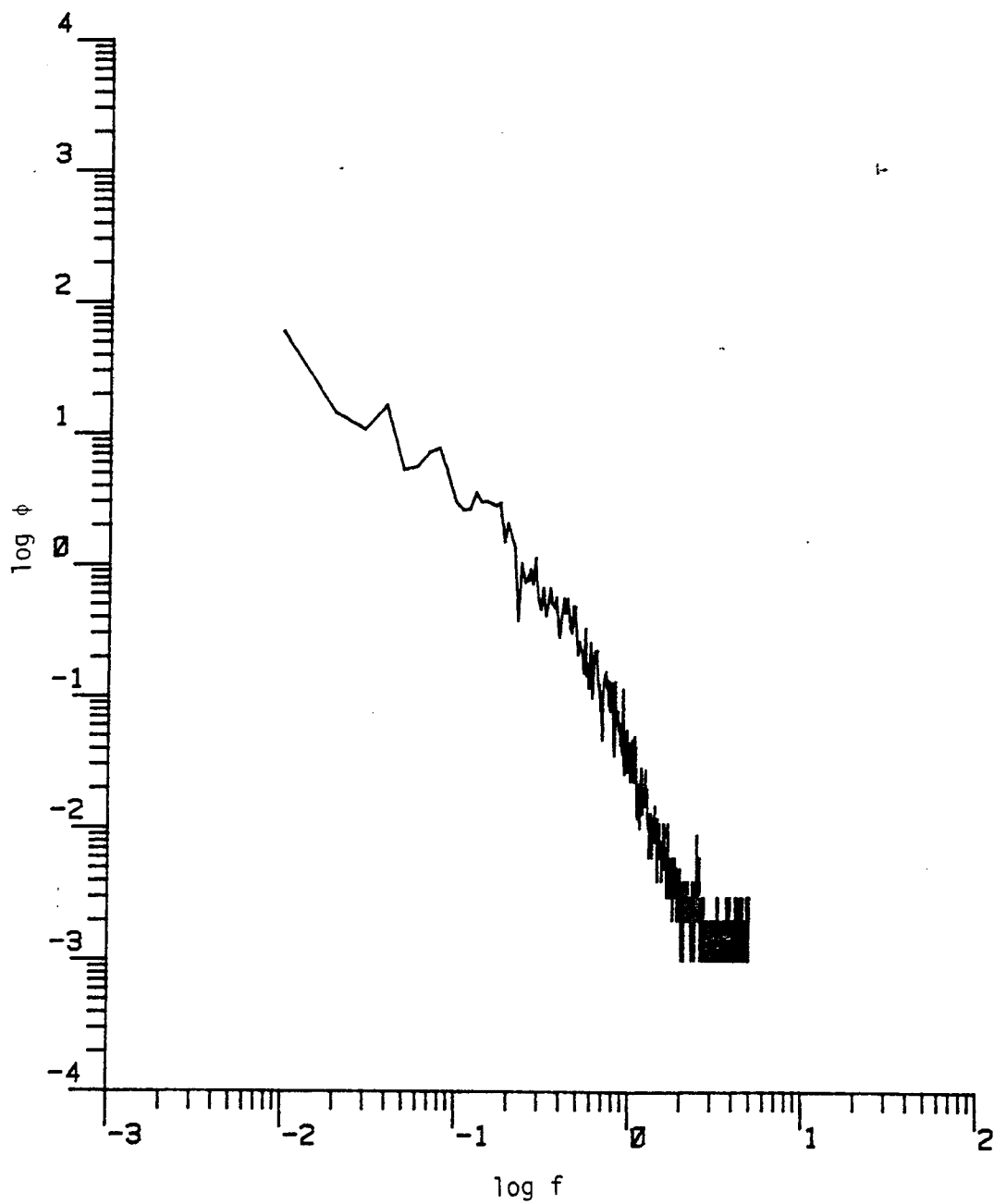
Figure D.45. The longitudinal power spectrum (Run #8624, T4L1, Component 1).
