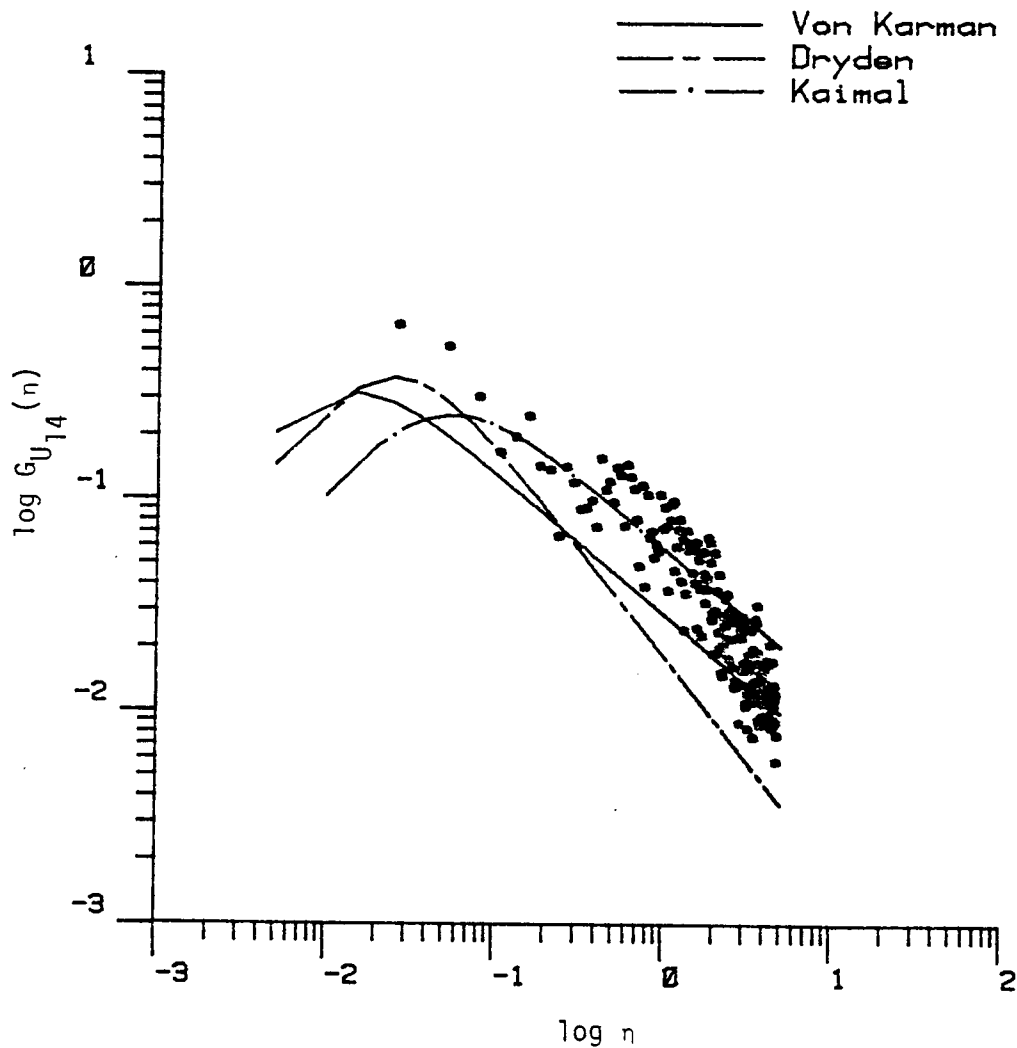
Figure 7.7. Comparison of longitudinal turbulence spectrum with three correlation models. (The length scale is calculated by Method 2, Chapter V, Run #8623).
