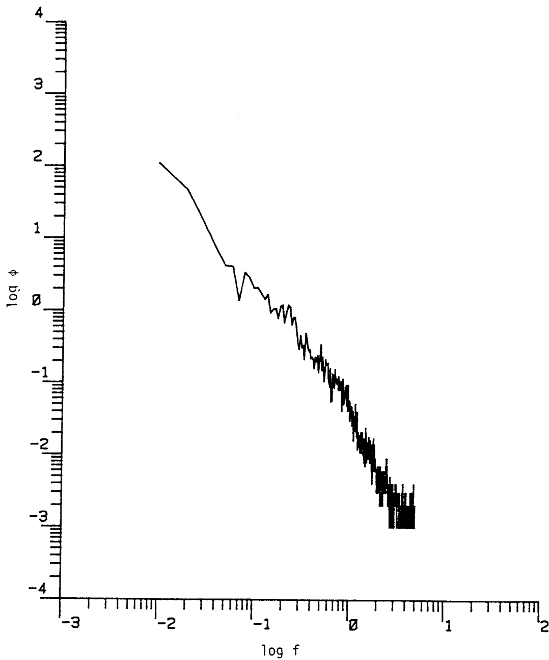
Figure D.22. The longitudinal power spectrum (Run #8623, S1L2, Component 1).
