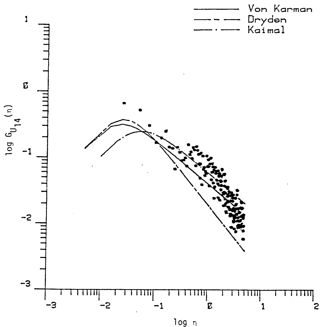
Figure 7.6. Comparison of longitudinal turbulence spectrum with three correlation models. (The length scale is calculated by Method 1, Chapter V, Run #8623).
