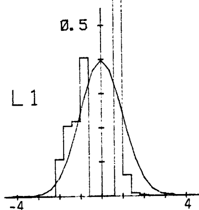
Figure C.53. Probability density function for vertical velocity component normalized with \sigma_{w_z} (Run #8624, S3, Component 3).
