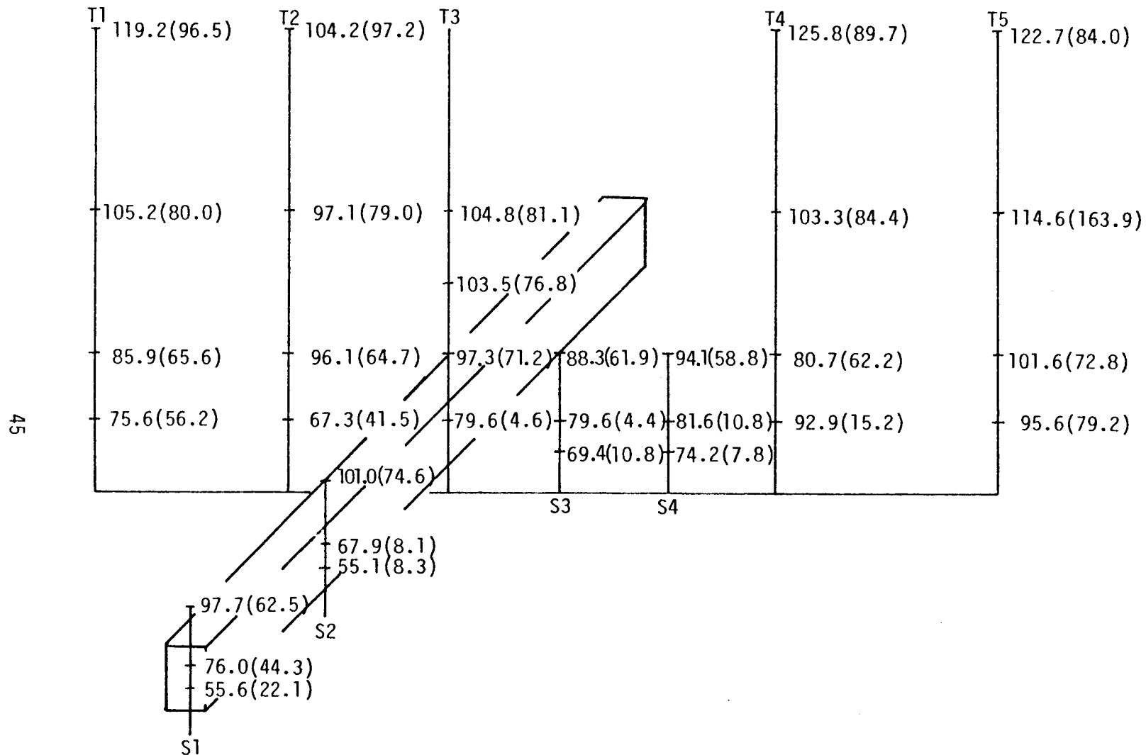
Figure 5.6. Spatial variation of the integral length scale in meters as computed by Method 3, Equation 5.7. (Component 1: Numbers not in parentheses, Run #8623, crosswind; numbers in parentheses, Run #8624, along wind).
