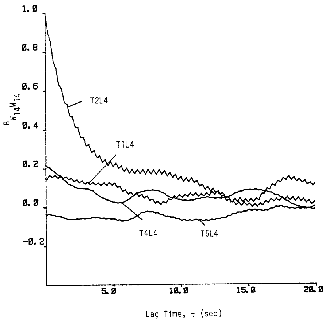
Figure E.6. Two-point horizontal space-time correlation relative to T2L4.
