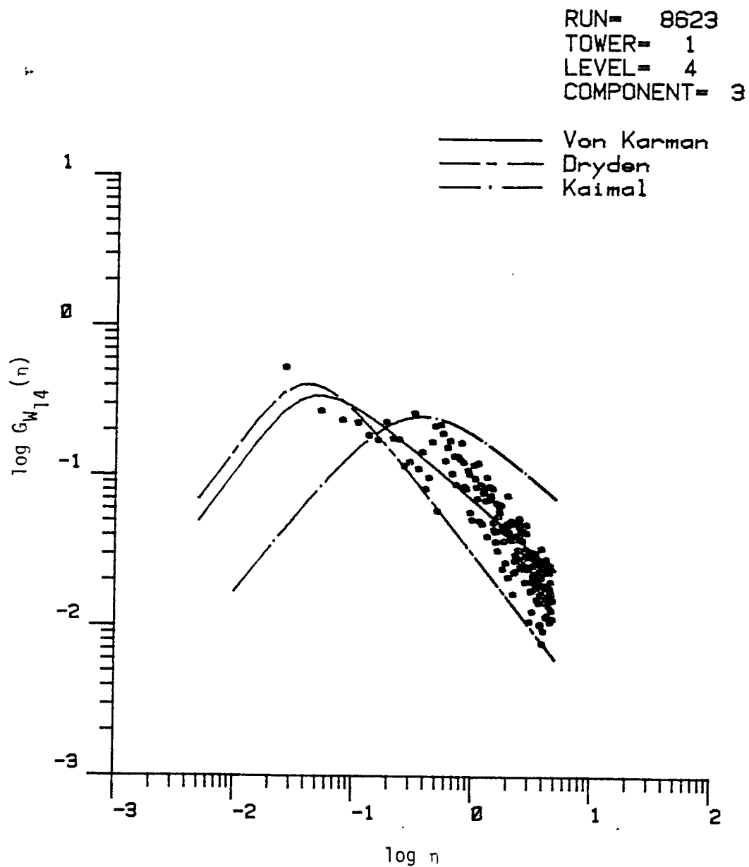
Figure 7.22. Comparison of vertical turbulence spectrum with three correlation models. (The length scale is calculated by Method 3, Chapter V, Run #8623).
