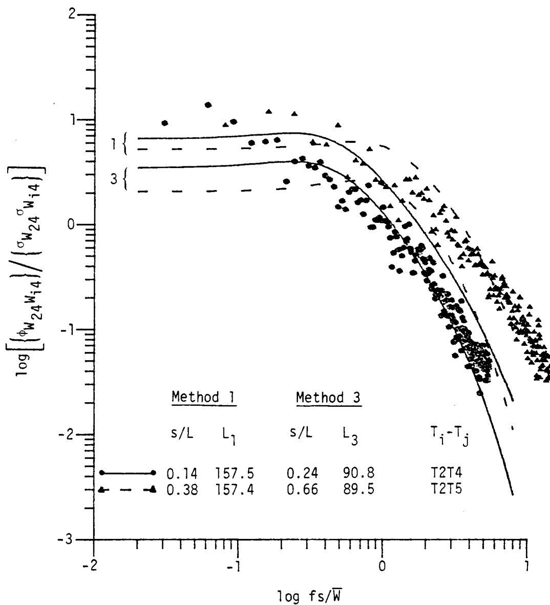
Figure 8.8. Comparison of computed two-point spatial spectra with the theoretical model of Houbolt and Sen (1972) (Run #8623, L4, Component 3).
