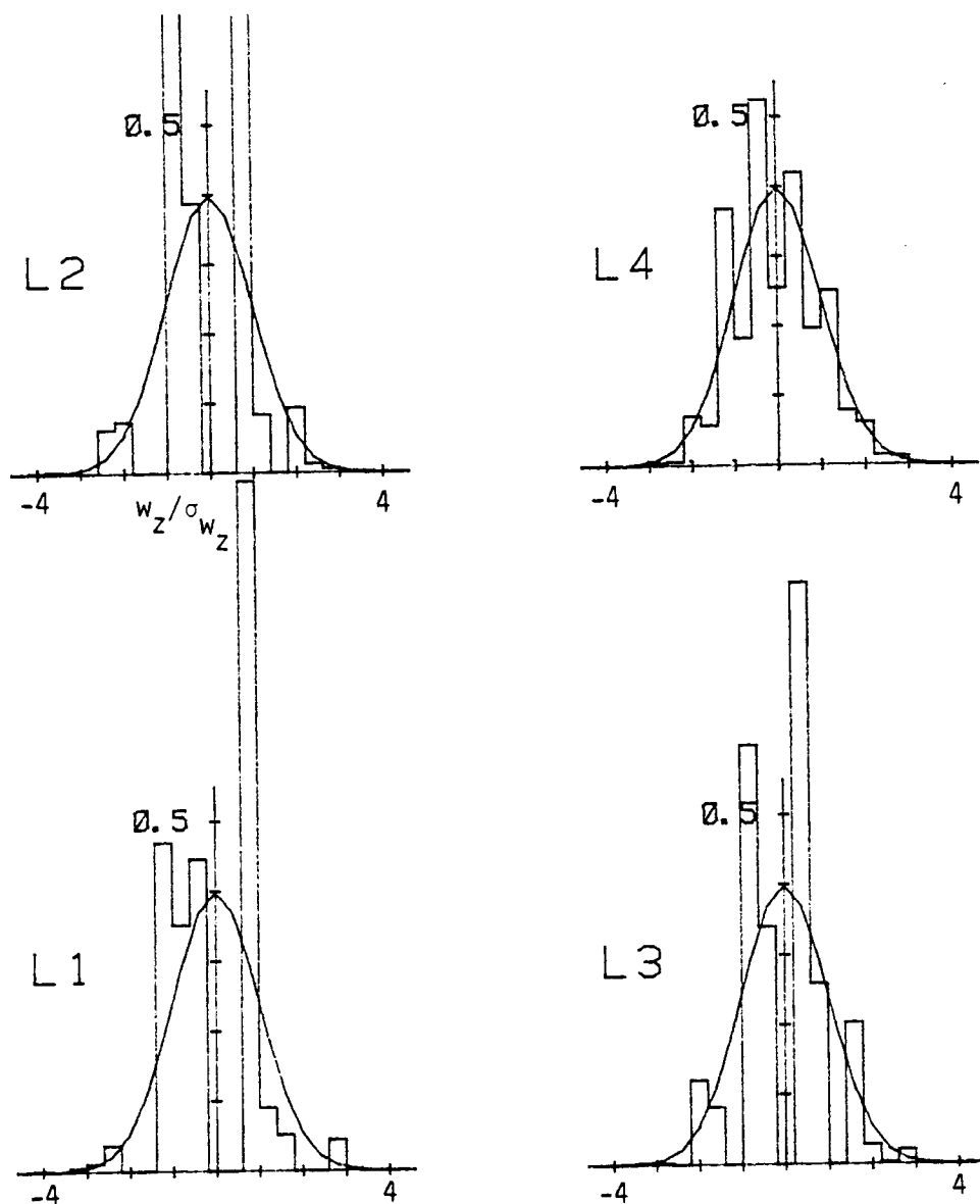
Figure C.40. Probability density function for vertical velocity component normalized with \sigma_{w_z} (Run #8623, T4, Component 3).
