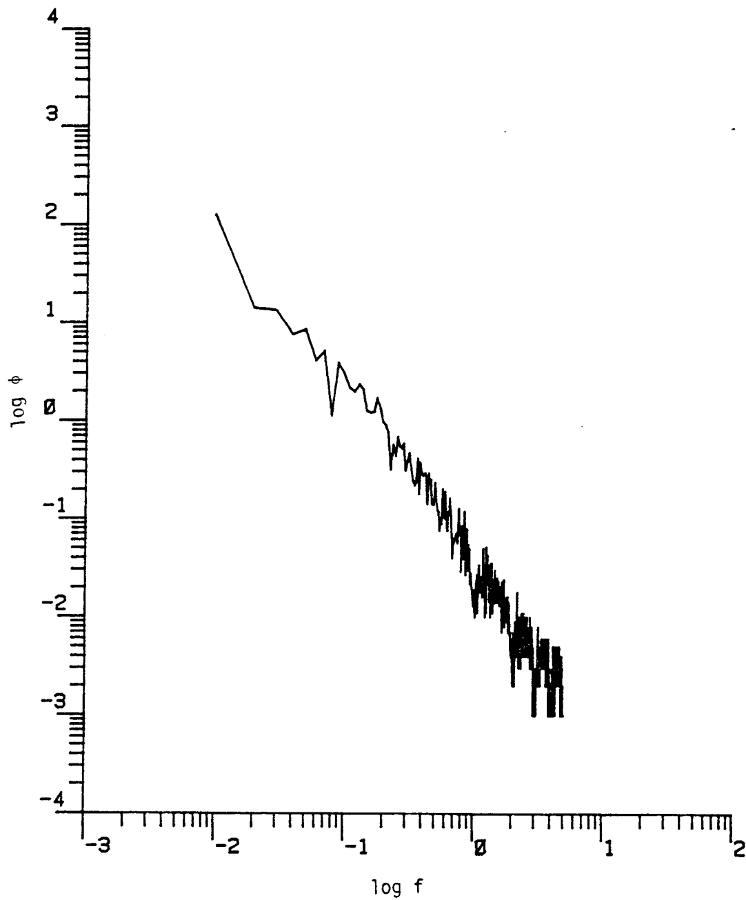
Figure D.61. The longitudinal power spectrum (Run #8624, S3L3, Component 1).
