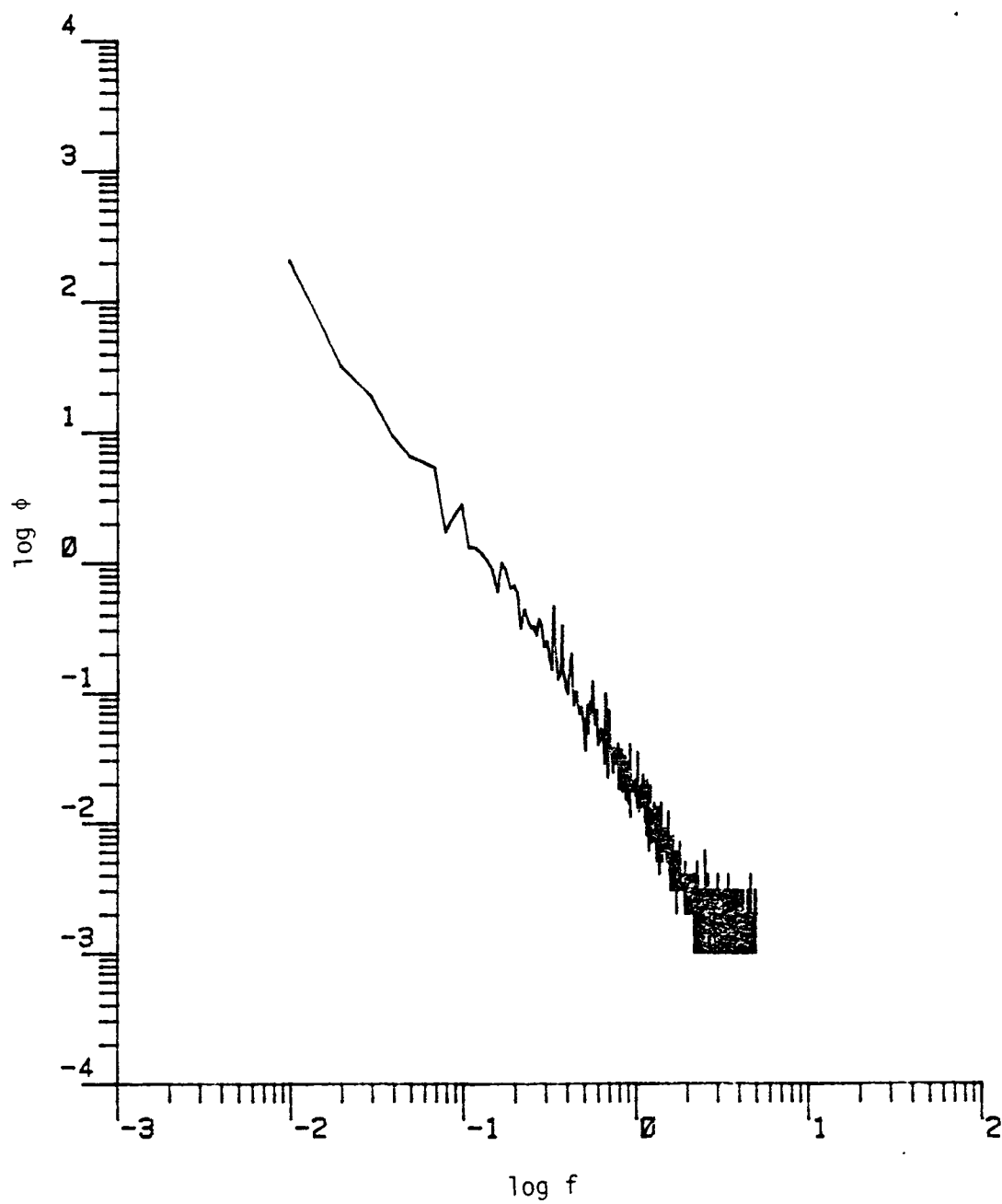
Figure D.36. The longitudinal power spectrum (Run #8624, T1L4, Component 1).
