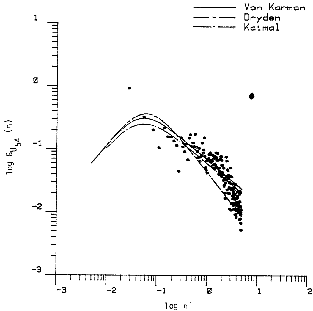
Figure 7.16. Comparison of longitudinal turbulence spectra with three analytical models. (The length scale is calculated by Method 4, T5).
