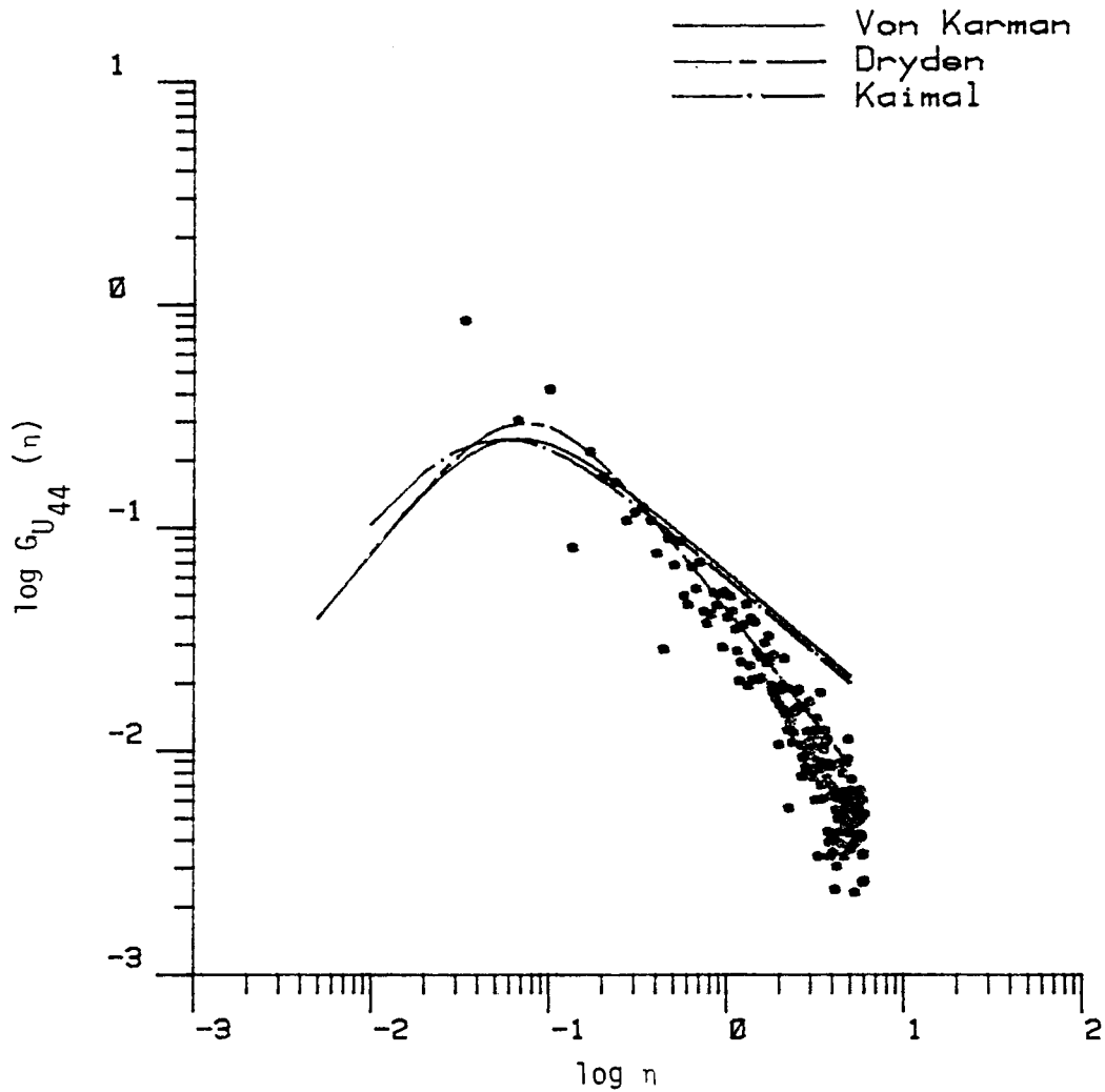
Figure 7.18. Comparison of longitudinal turbulence spectra with three analytical models. (The length scale is calculated by Method 4, T4).
