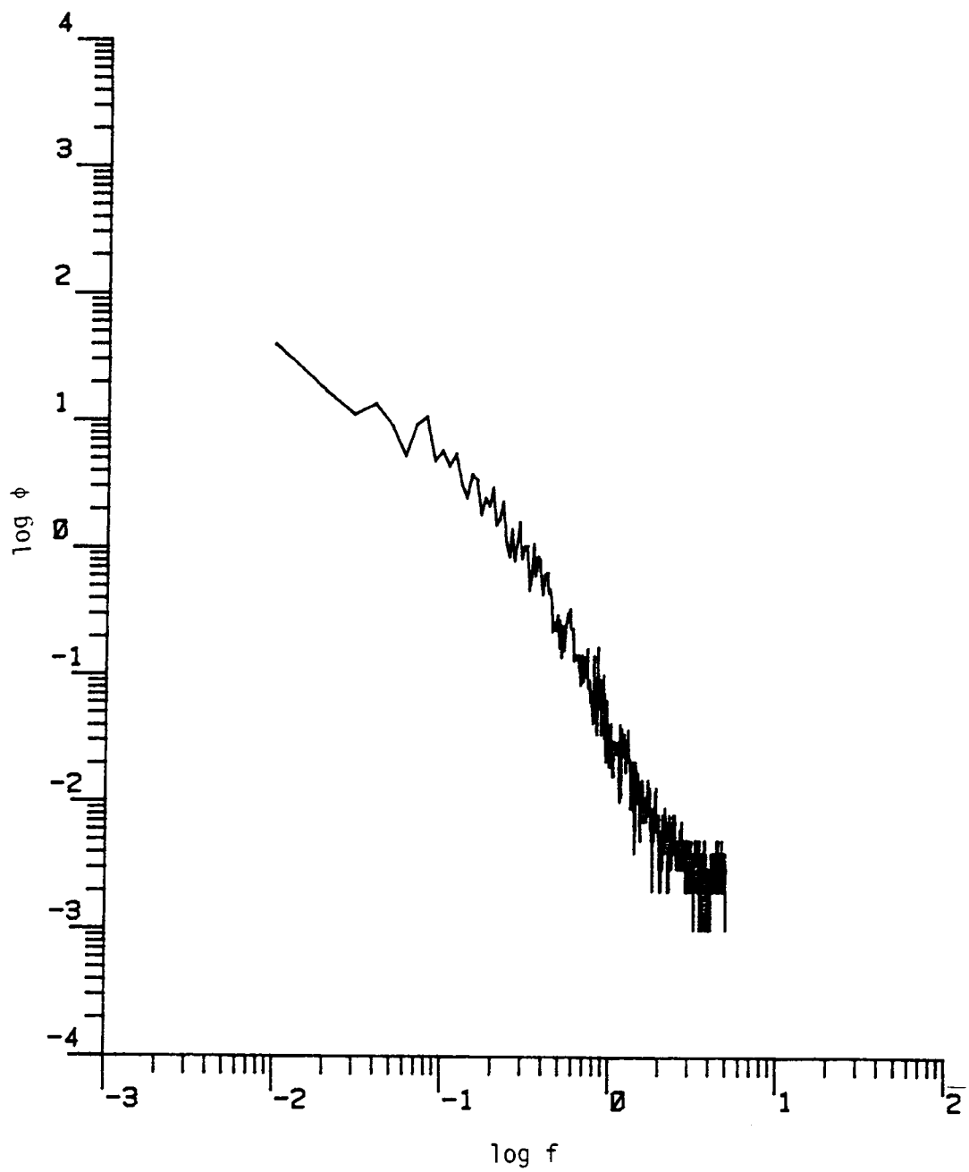
Figure D.63. The longitudinal power spectrum (Run #8624, S4L2, Component 1).
