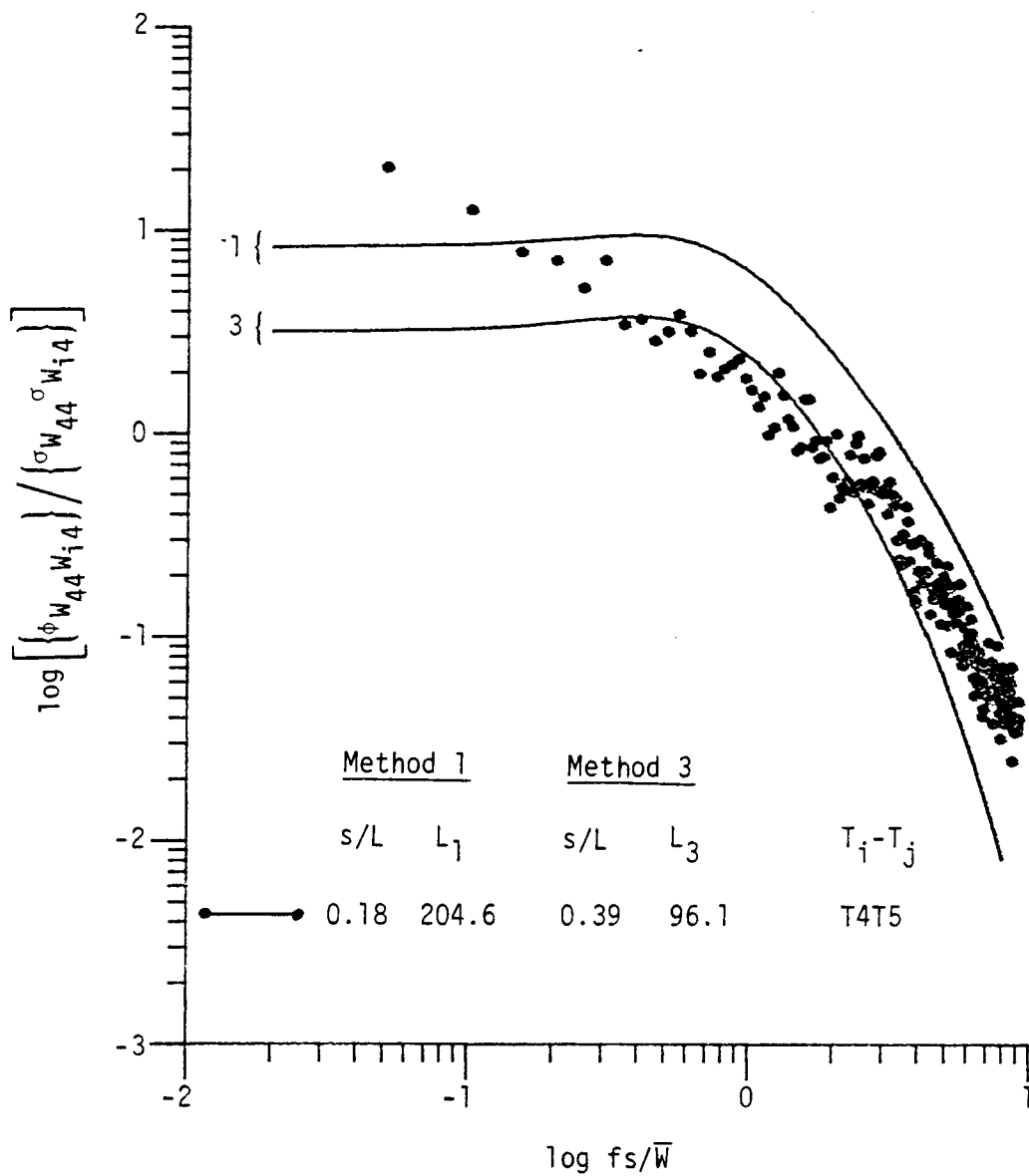
Figure 8.9. Comparison of computed two-point spatial spectra with the theoretical model of Houbolt and Sen (1972) (Run #8623, L4, Component 3).
