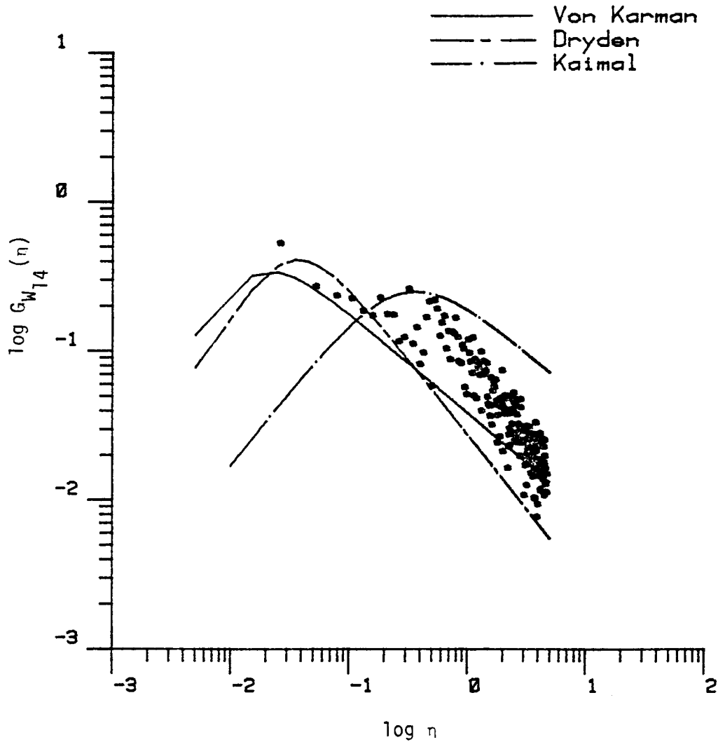
Figure 7.21. Comparison of vertical turbulence spectrum with three correlation models. (The length scale is calculated by Method 2, Chapter V, Run #8623).
