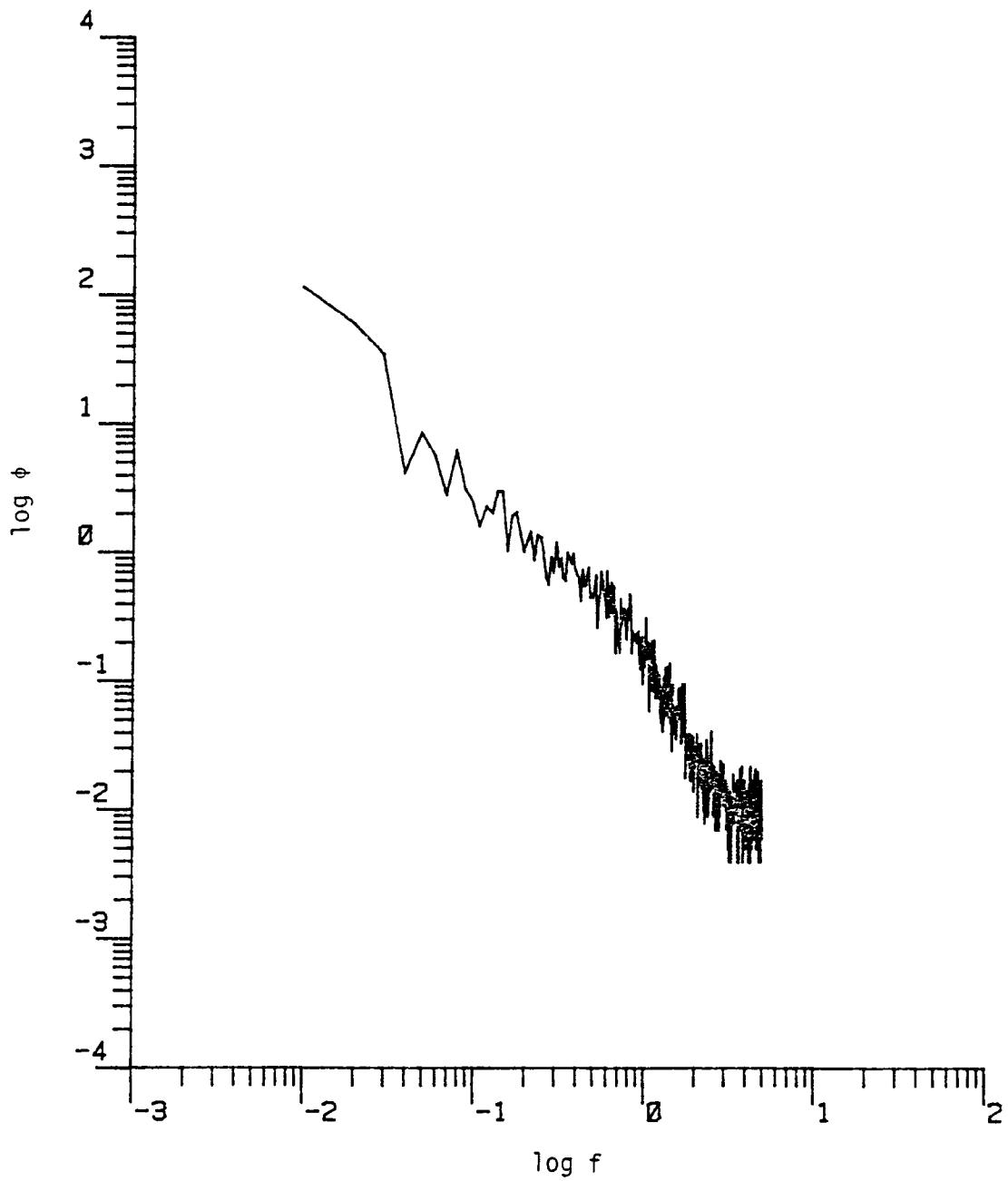
Figure D.5. The longitudinal power spectrum (Run #8623, T2L1, Component 1).
