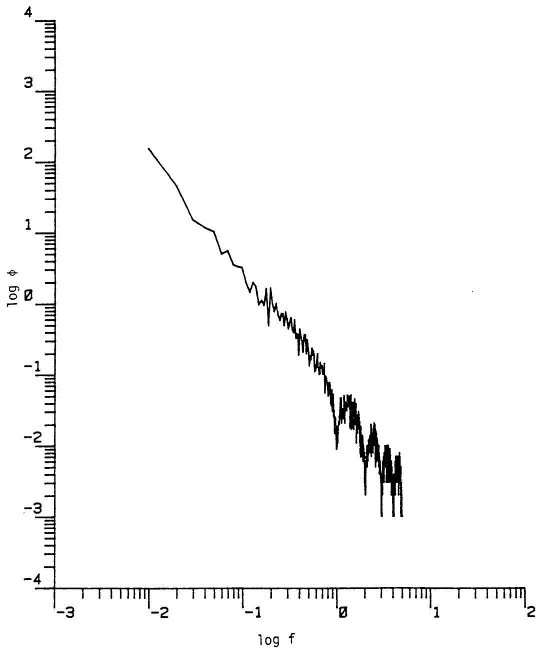
Figure D.29. The longitudinal power spectrum (Run #8623, S3L3, Component 1).
