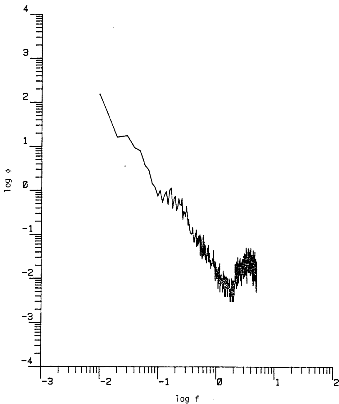
Figure D.39. The longitudinal power spectrum (Run #8624, T2L3, Component 1).
