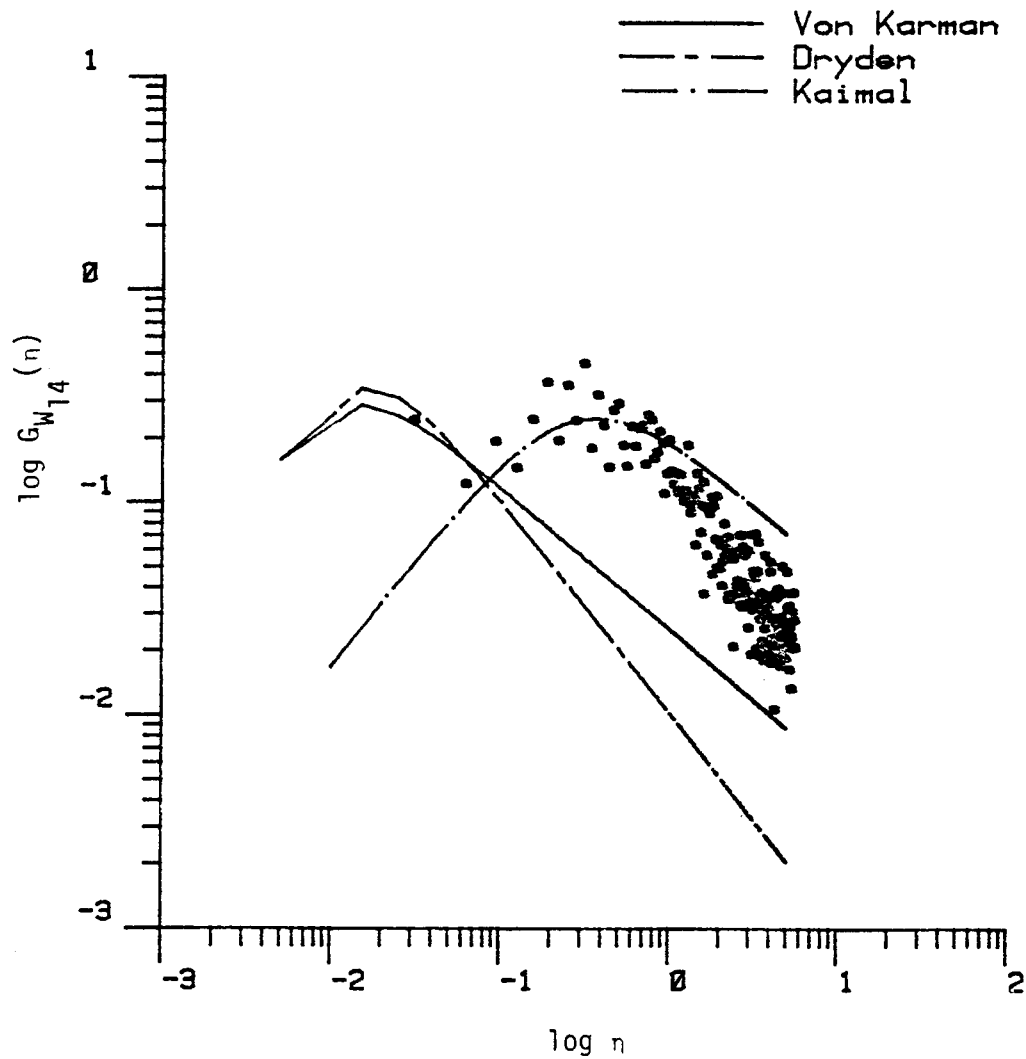
Figure 7.23. Comparison of vertical turbulence spectrum with three correlation models. (The length scale is calculated by Method 1, Chapter V, Run #8624).
