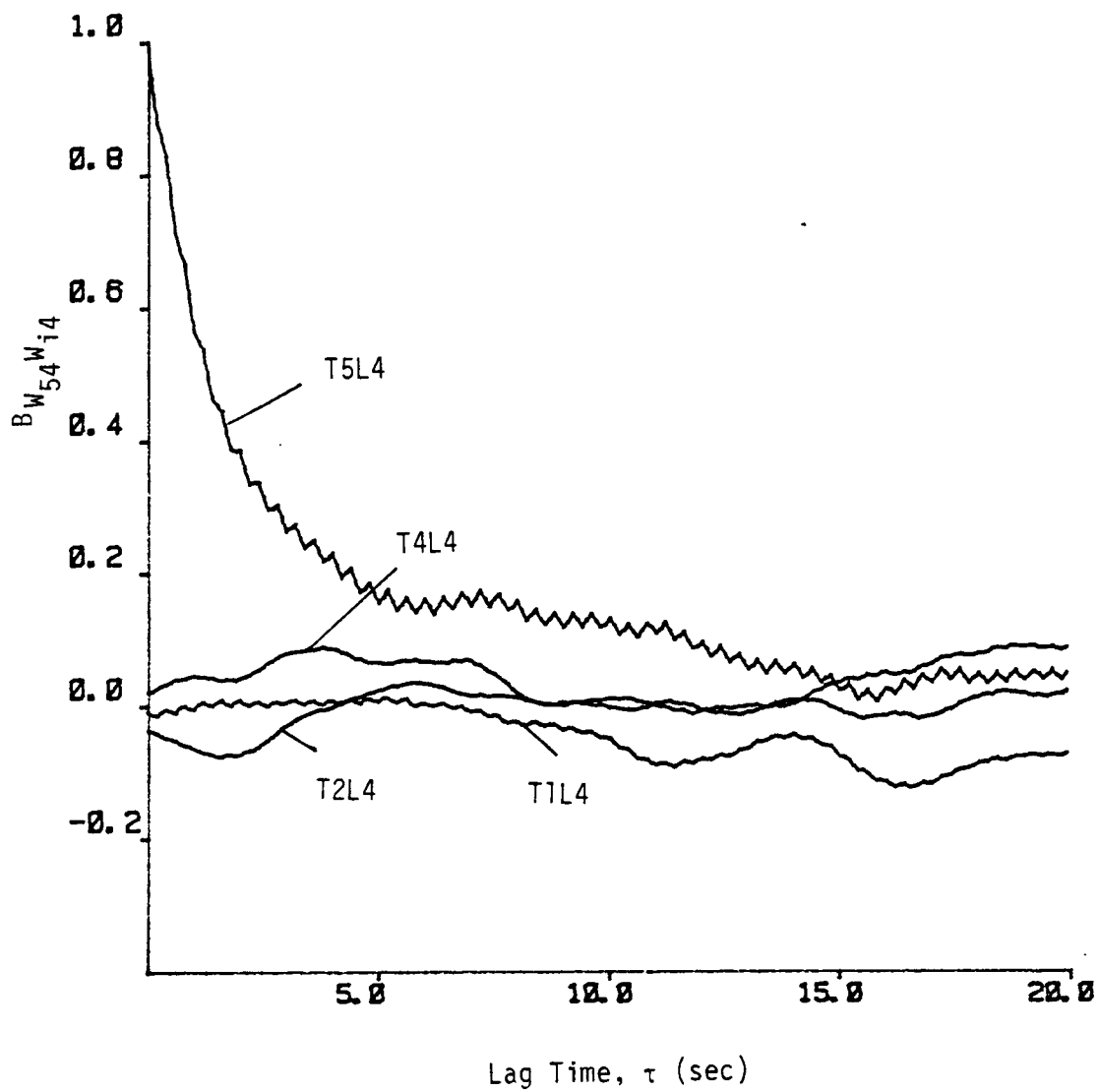
Figure E.8. Two-point horizontal space-time correlation relative to T5L4.
