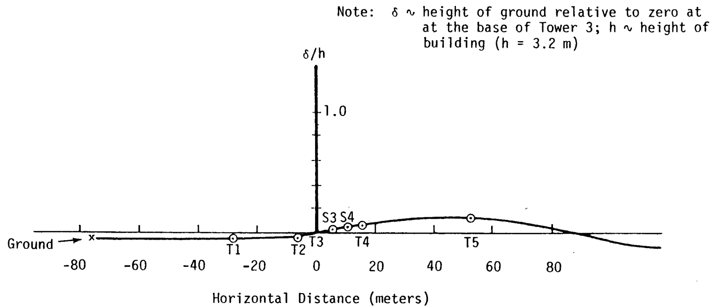
Figure 3.1. Cross-sectional contour of the eight-tower array. ◉ indicates the base of each tower x indicates ground level
