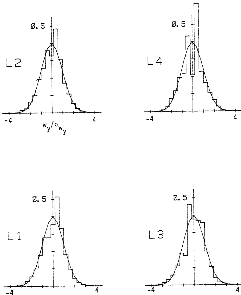
Figure C.19. Probability density function for lateral velocity component normalized with \sigma_{w_y} (Run #8623, T1, Component 2).
