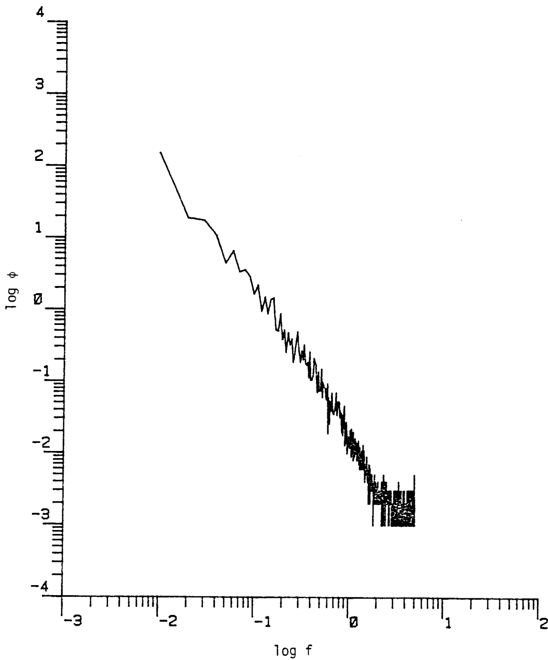
Figure D.35. The longitudinal power spectrum (Run #8624, T1L3, Component 1).
