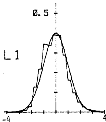
Figure C.6. Probability density function for longitudinal velocity component normalized with \sigma_{w_x} (Run #8623, S1, Component 1).
