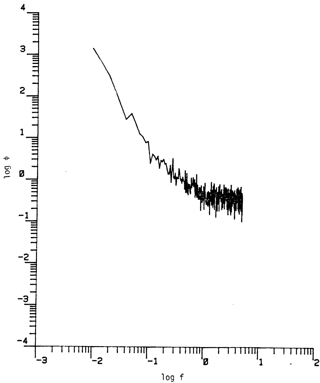
Figure D.23. The longitudinal power spectrum (Run #8623, S1L3, Component 1).
