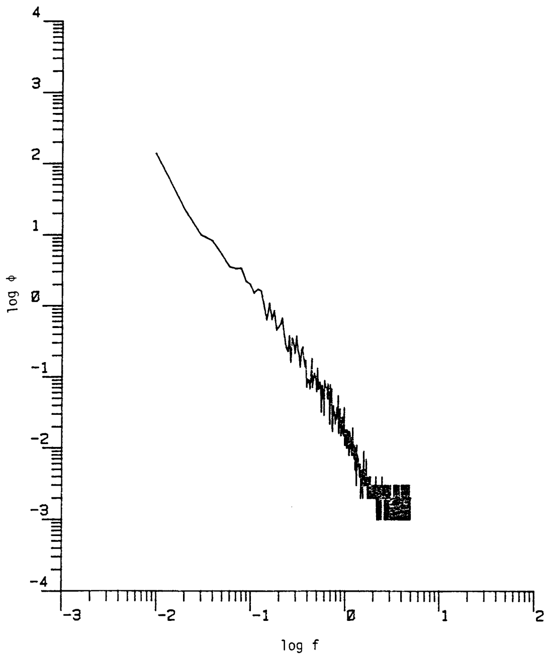
Figure D.49. The longitudinal power spectrum (Run #8624, T5L1, Component 1).
