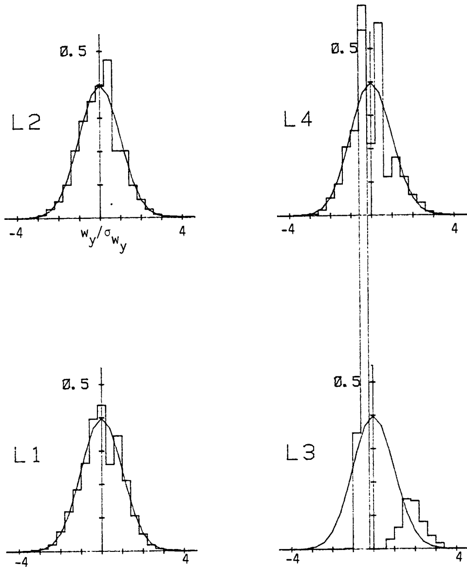
Figure C.32. Probability density function for lateral velocity component normalized with \sigma_{w_y} (Run #8624, T5, Component 2).
