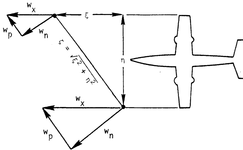
Figure 2.4. Illustration of coordinates and wind speed components.
