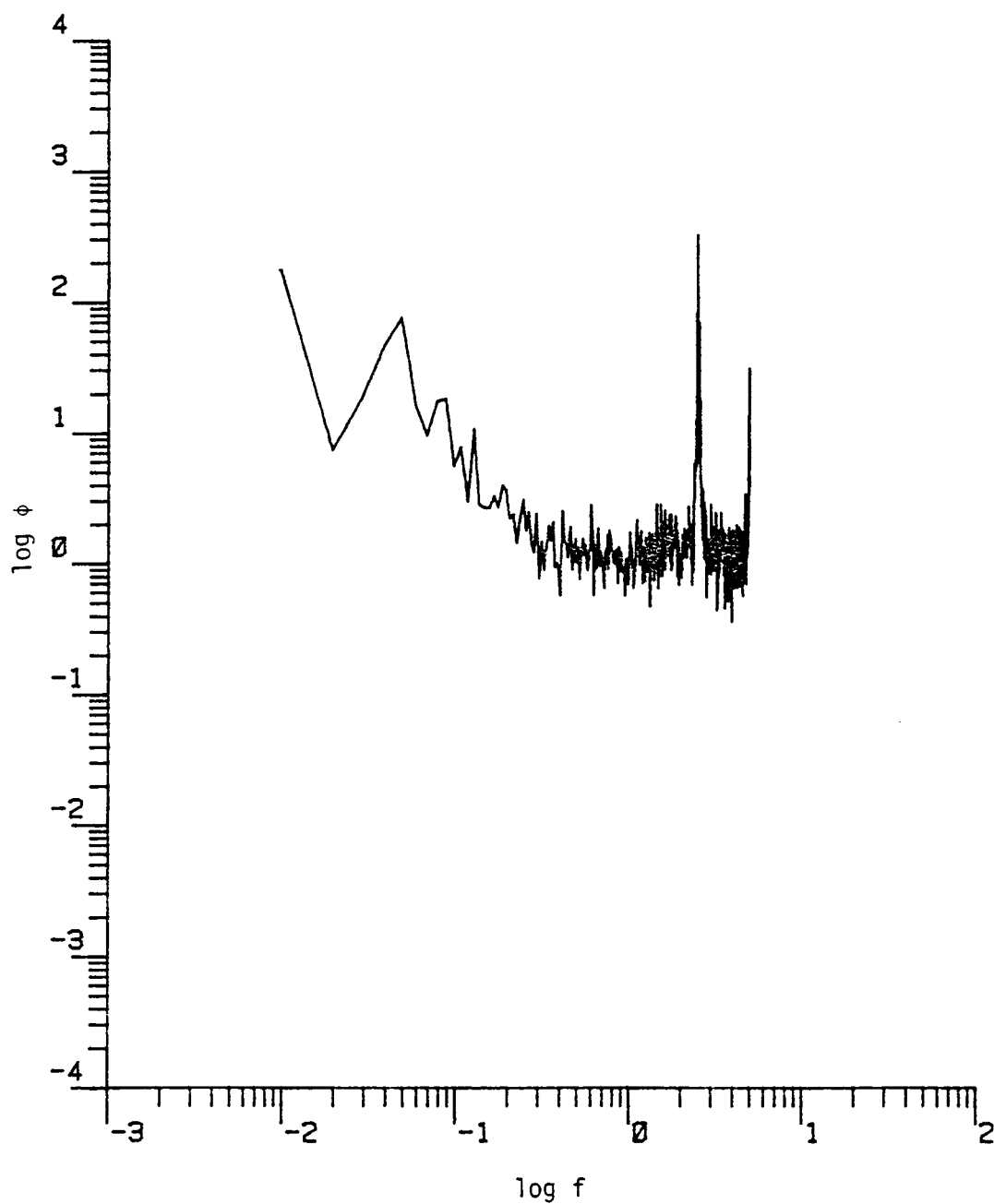
Figure D.51. The longitudinal power spectrum (Run #8624, T5L3, Component 1).
