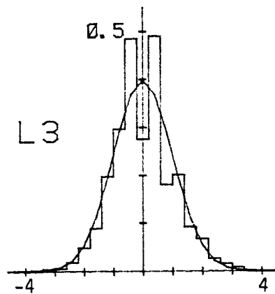
Figure C.28. Probability density function for lateral velocity component normalized with \sigma_{w_y} (Run #8624, T1, Component 2).
