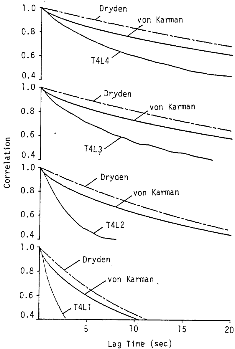
Figure 6.18. Comparison with von Karman and Dryden expressions for the longitudinal correlation (length scale L_1 , T4, Run #8624).
