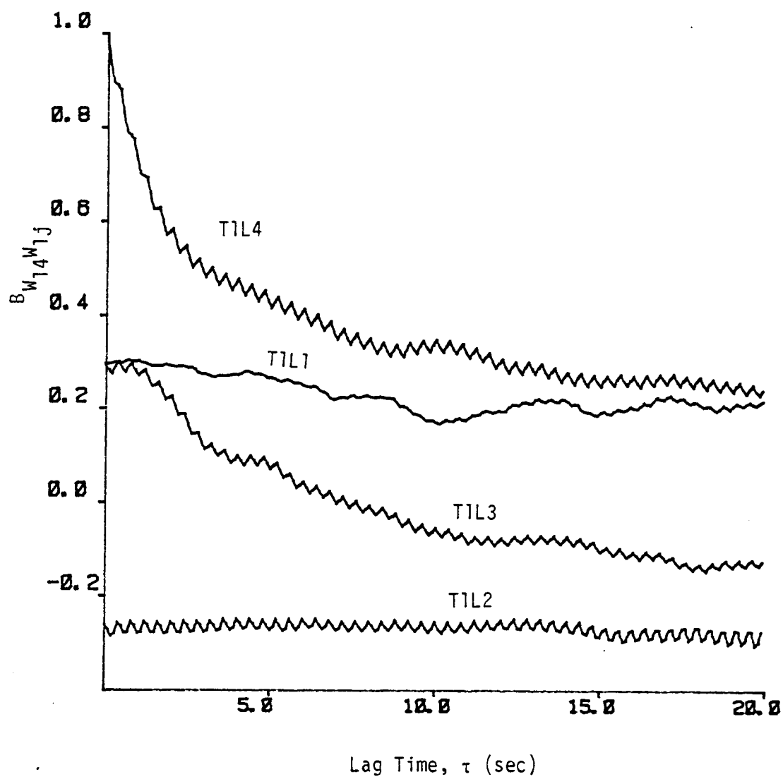
Figure E.1. Two-point vertical space-time correlation relative to T1L4.
