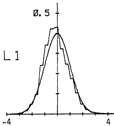
Figure C.1. Probability density function for longitudinal velocity component normalized with \sigma_{w_x} (Run #8623, T1, Component 1).
