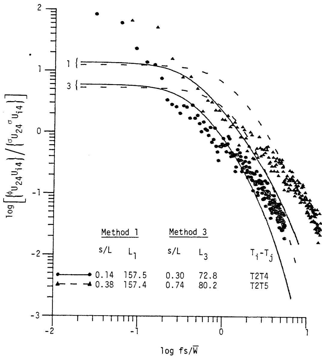
Figure 8.2. Comparison of computed two-point spatial spectra with the theoretical model of Houbolt and Sen (1972) (Run #8623, L4, Component 1).
