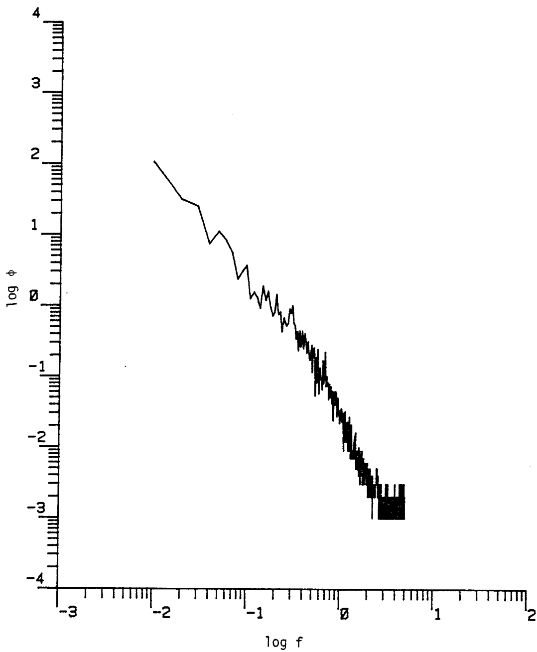
Figure D.54. The longitudinal power spectrum (Run #8624, S1L2, Component 1).
