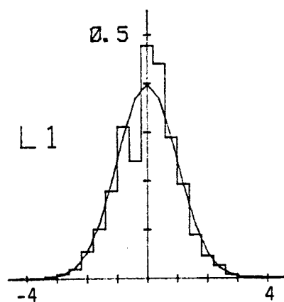
Figure C.26. Probability density function for lateral velocity component normalized with \sigma_{w_y} (Run #8623, S3, Component 2).
