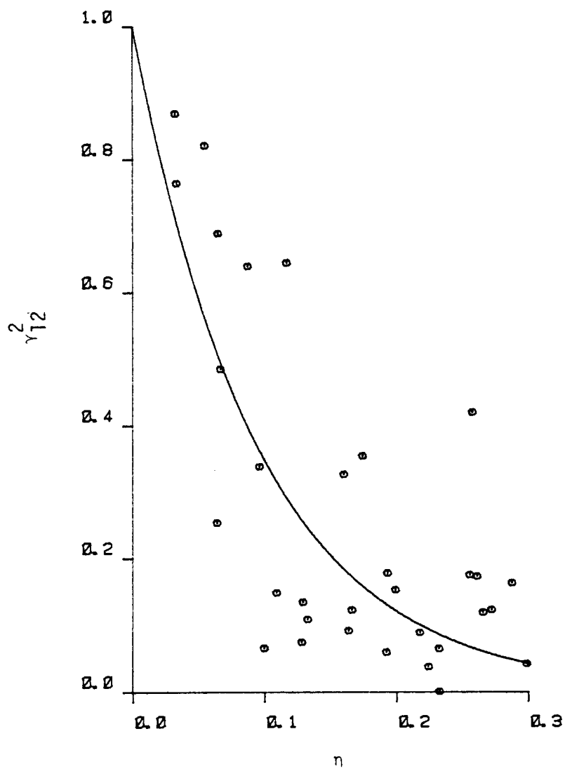
Figure 8.15. The lateral coherence \gamma_{12}^2 for the longitudinal velocity component at the 12-m level.
