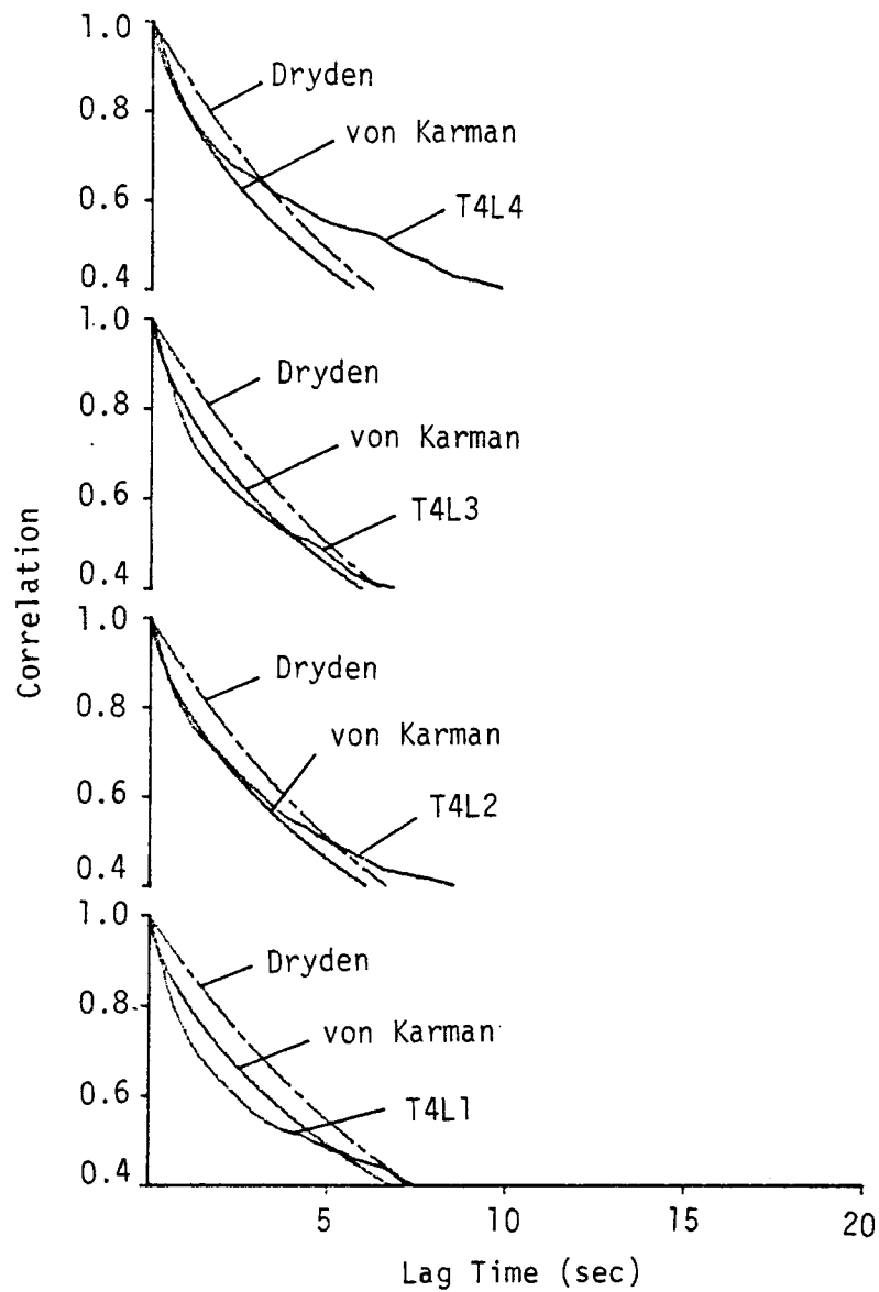
Figure 6.21. Comparison with von Karman and Dryden expressions for the longitudinal correlation (length scale L_4 , T4, Run #8623).
