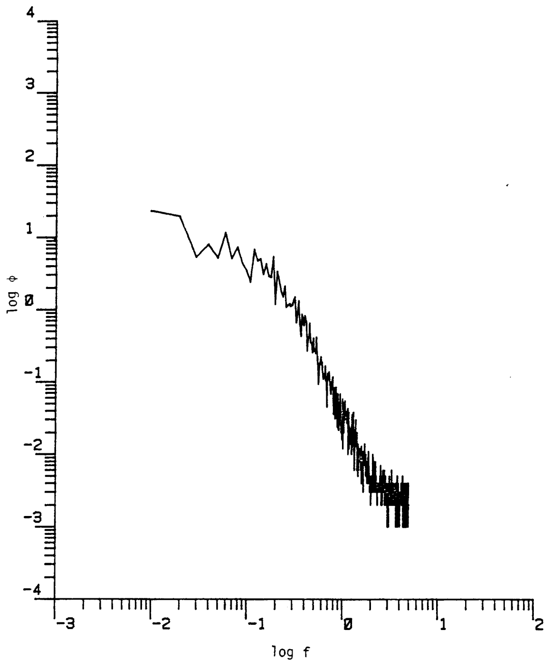
Figure D.60. The longitudinal power spectrum (Run #8624, S3L2, Component 1).
