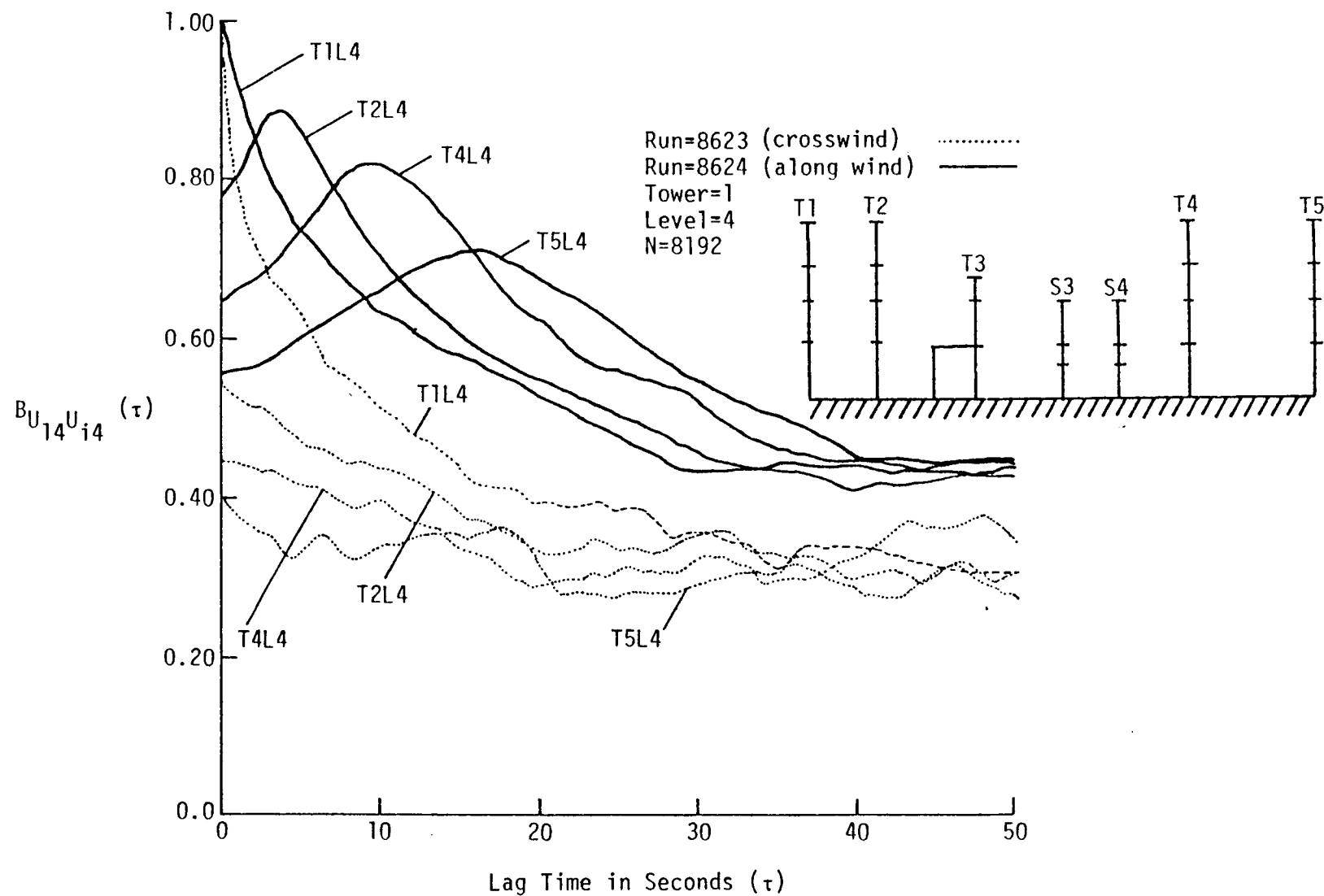
Figure 6.6. Two-point horizontal space-time correlation relative to T1L4.
