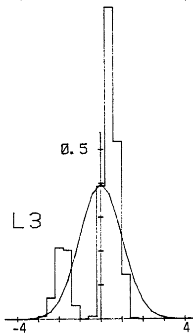
Figure C.14. Probability density function for longitudinal velocity component normalized with \sigma_{w_x} (Run #8624, T5, Component 1).
