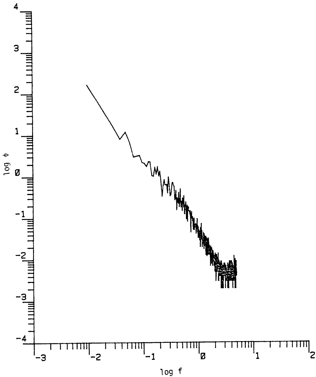
Figure D.19. The longitudinal power spectrum (Run #8623, T5L3, Component 1).
