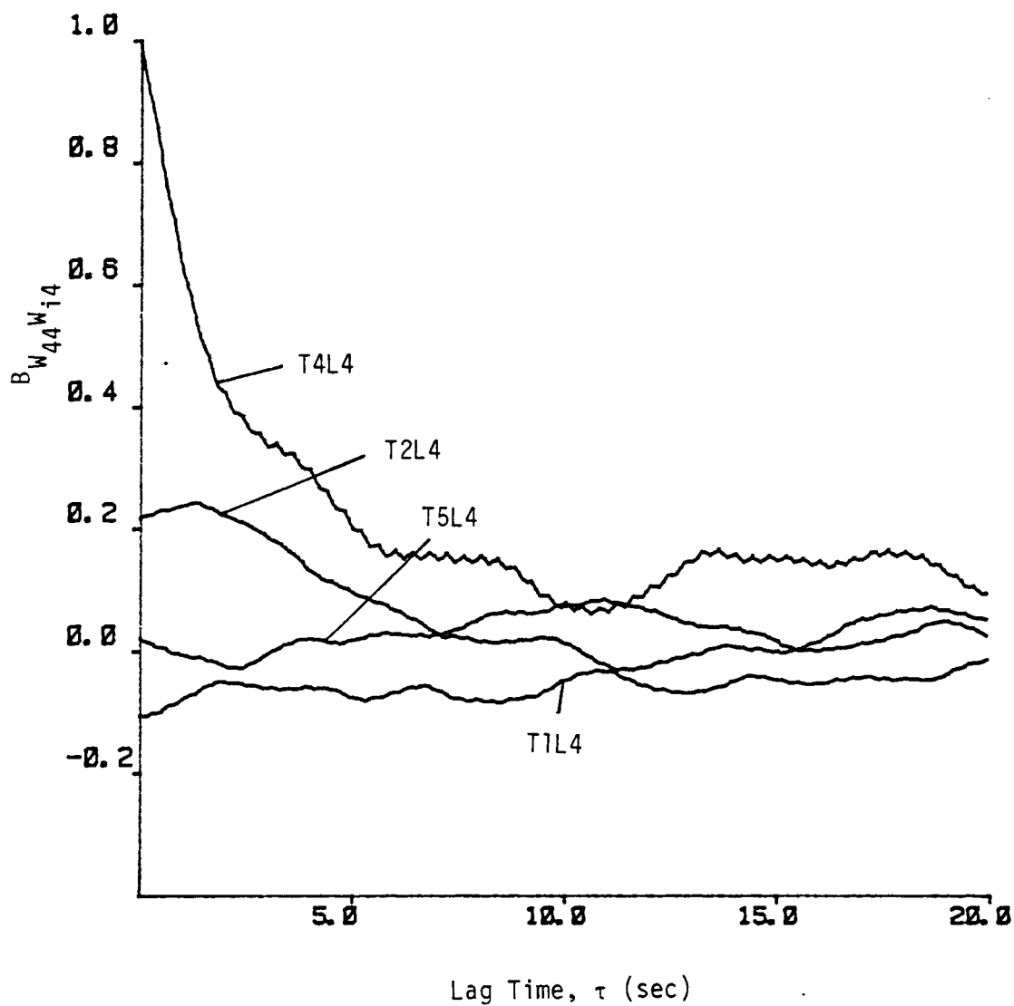
Figure E.7. Two-point horizontal space-time correlation relative to T4L4.
