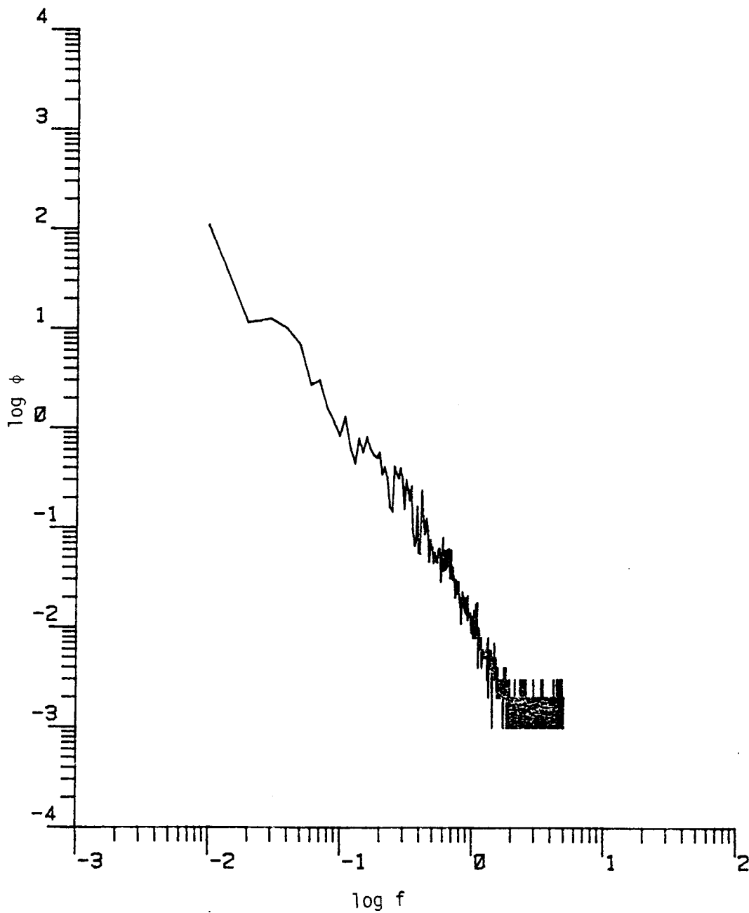
Figure D.33. The longitudinal power spectrum (Run #8624, T1L1, Component 1).
