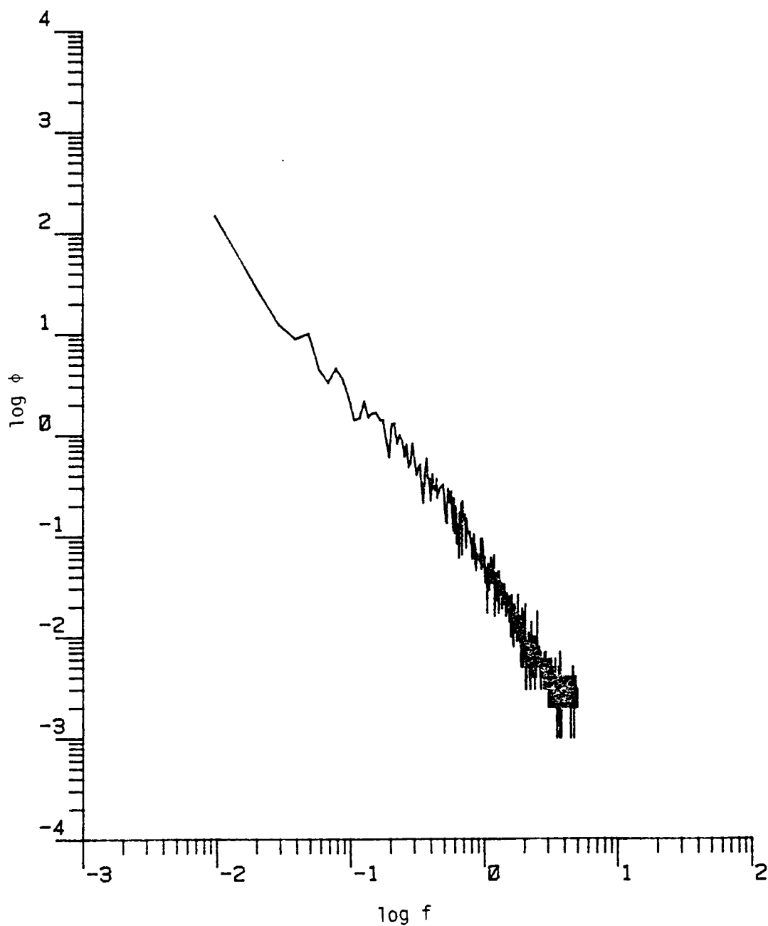
Figure D.18. The longitudinal power spectrum (Run #8623, T5L2, Component 1).
