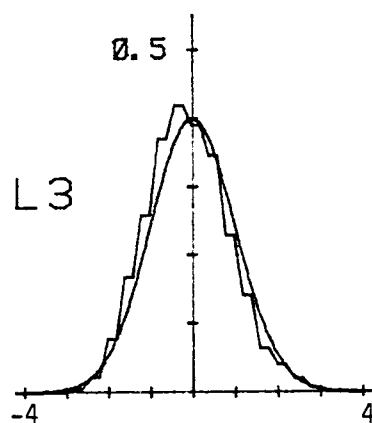
Figure C.9. Probability density function for longitudinal velocity component normalized with \sigma_{w_x} (Run #8623, S4, Component 1).
