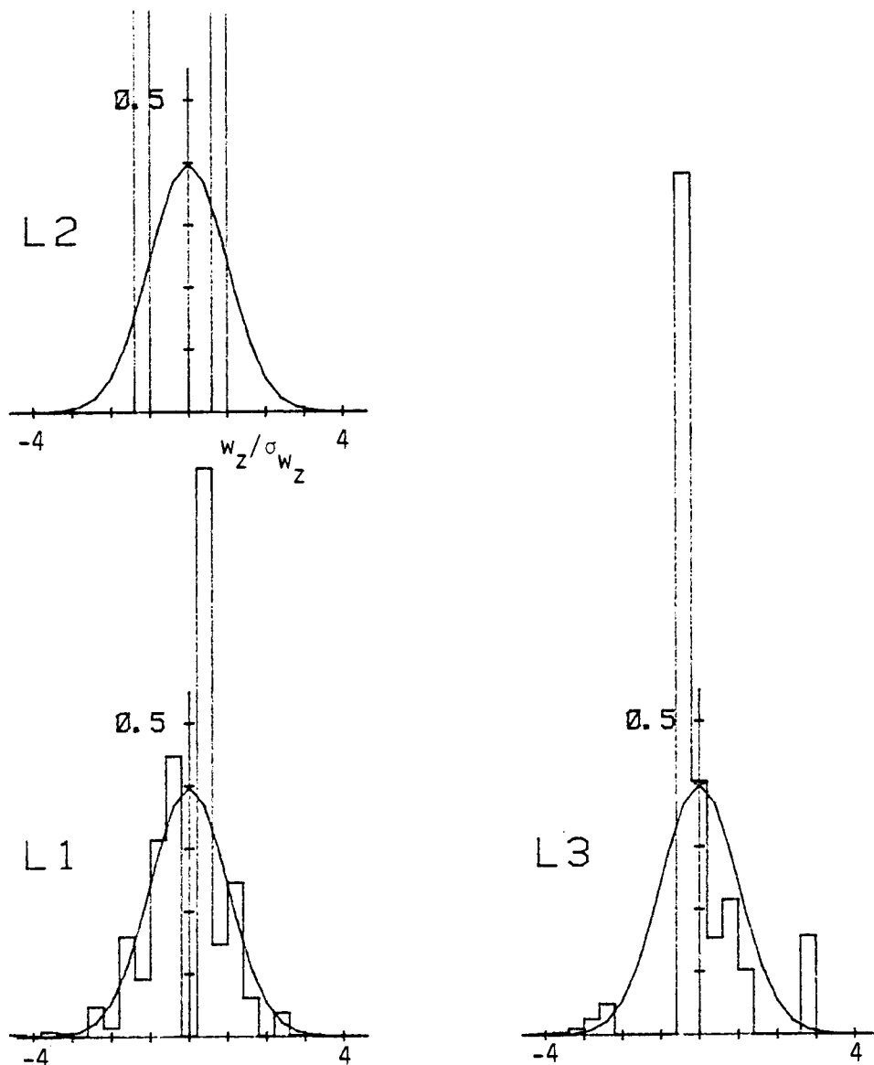
Figure C.54. Probability density function for vertical velocity component normalized with \sigma_{w_z} (Run #8624, S4, Component 3).
