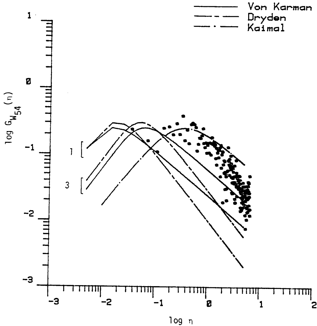
Figure 7.31. Comparison of vertical turbulence spectrum with three Correlation models. (The length scale is calculated by Methods 1 and 3, Chapter V, T5, Run #8624).
