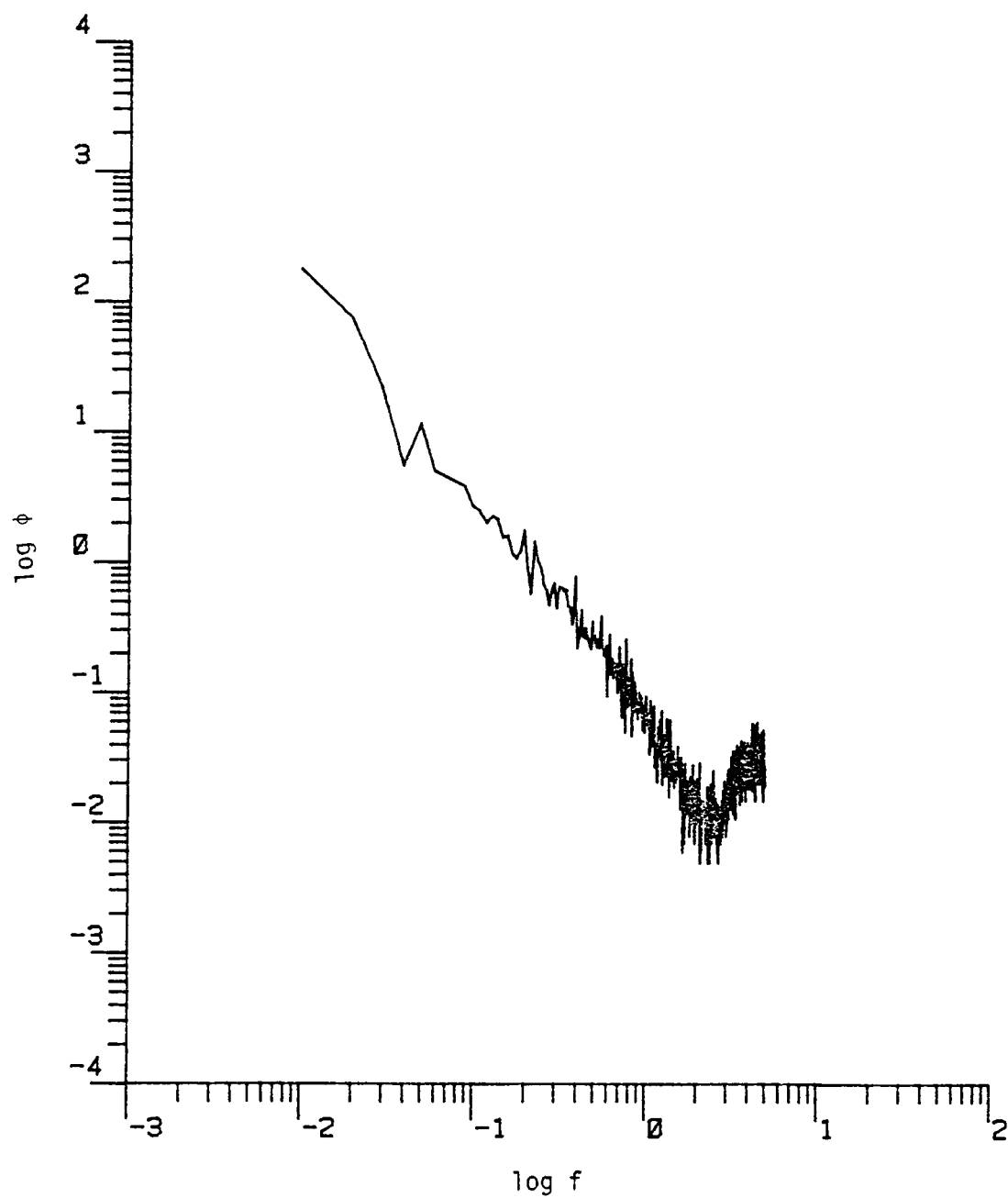
Figure D.7. The longitudinal power spectrum (Run #8623, T2L3, Component 1).
