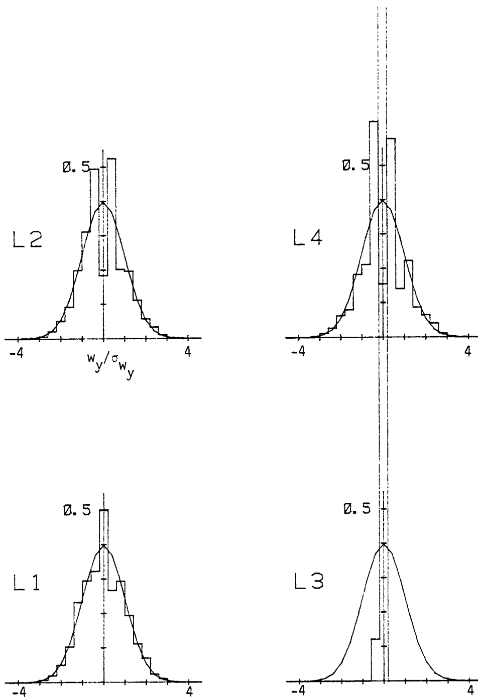
Figure C.23. Probability density function for lateral velocity component normalized with \sigma_{w_y} (Run #8623, T5, Component 2).
