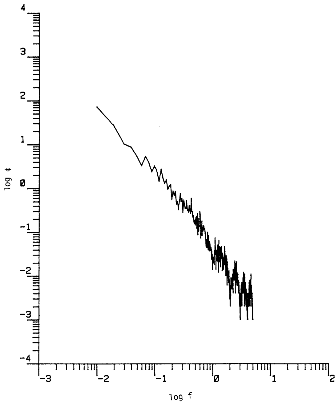
Figure D.27. The longitudinal power spectrum (Run #8623, S3L1, Component 1).
