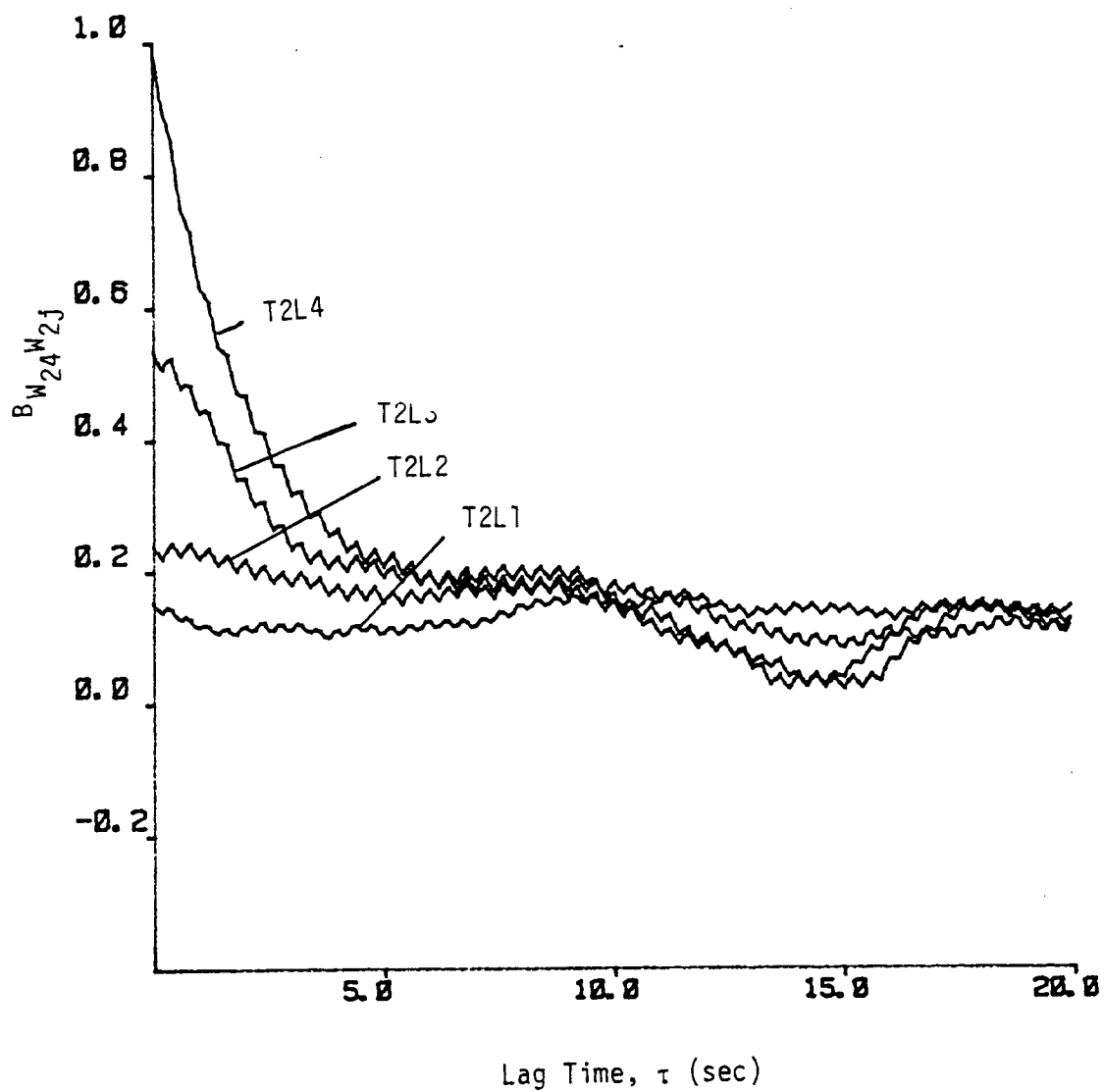
Figure E.2. Two-point vertical space-time correlation relative to T2L4.
