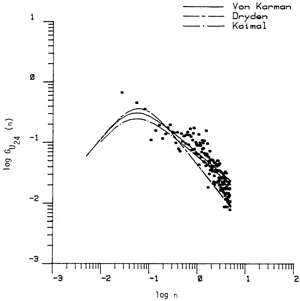
Figure 7.14. Comparison of longitudinal turbulence spectra with three analytical models. (The length scale is calculated by Method 4, T2).
