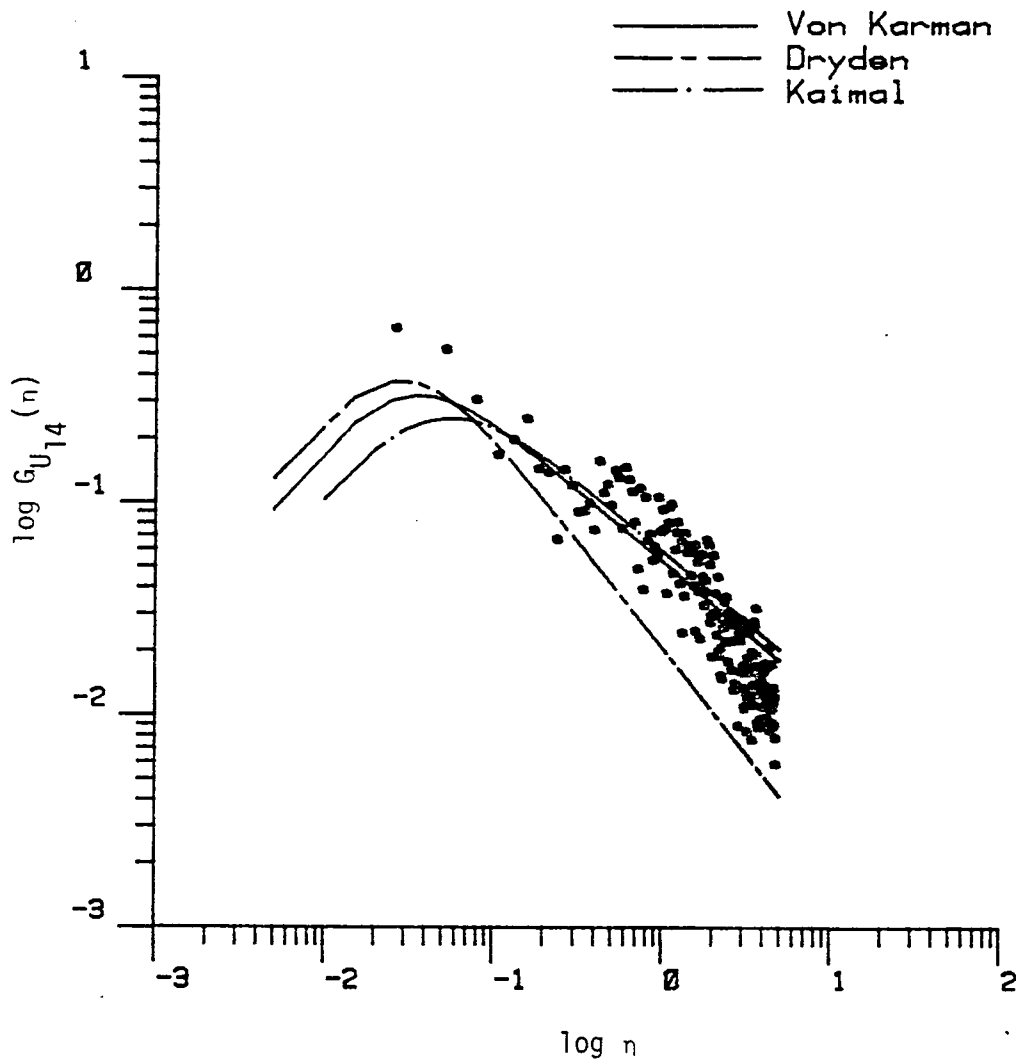
Figure 7.8. Comparison of longitudinal turbulence spectrum with three correlation models. (The length scale is calculated by Method 3, Chapter V, Run #8623).
