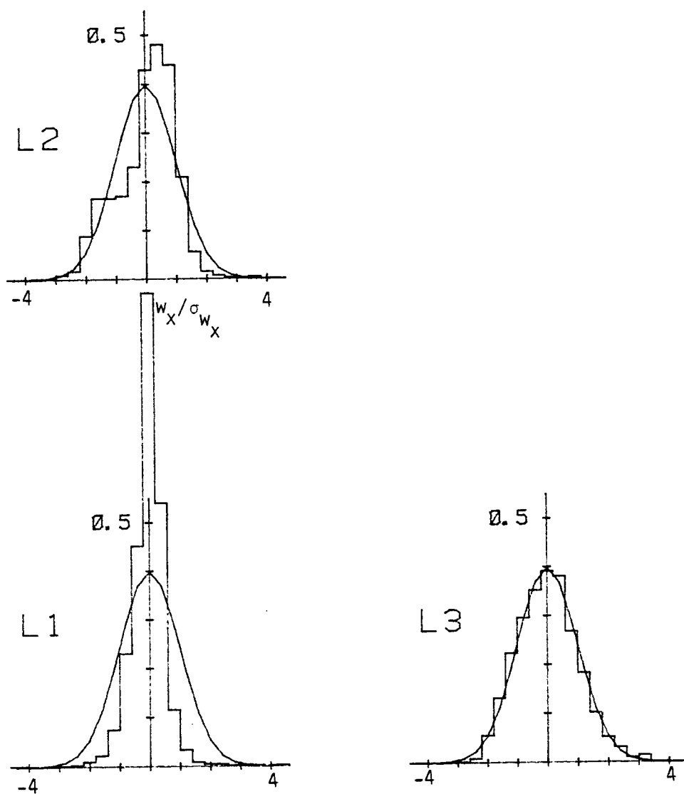
Figure C.16. Probability density function for longitudinal velocity component normalized with \sigma_{w_x} (Run #8624, S2, Component 1).
