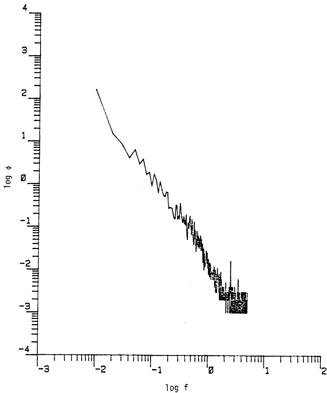
Figure D.44. The longitudinal power spectrum (Run #8624, T3L4, Component 1).
