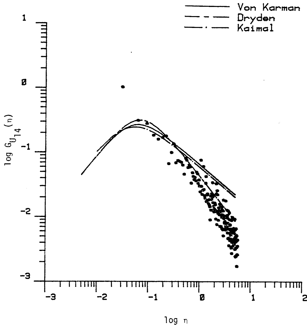
Figure 7.13. Comparison of longitudinal turbulence spectrum with three correlation models. (The length scale is calculated by Method 4, Chapter V, Run #8624).
