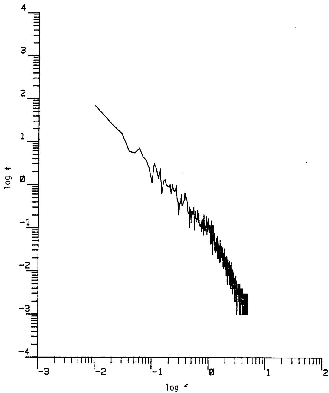
Figure D.9. The longitudinal power spectrum (Run #8623, T3L1, Component 1).
