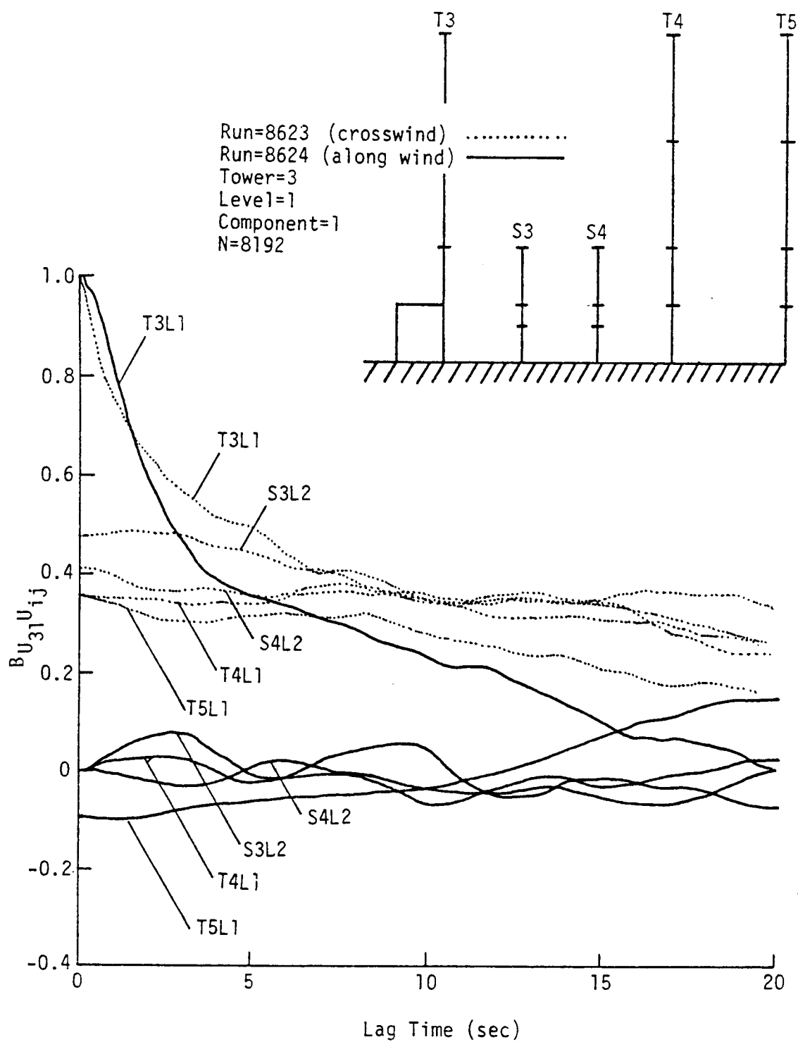
Figure 6.8. Two-point horizontal space-time correlation in the wake region relative to T3L1.
