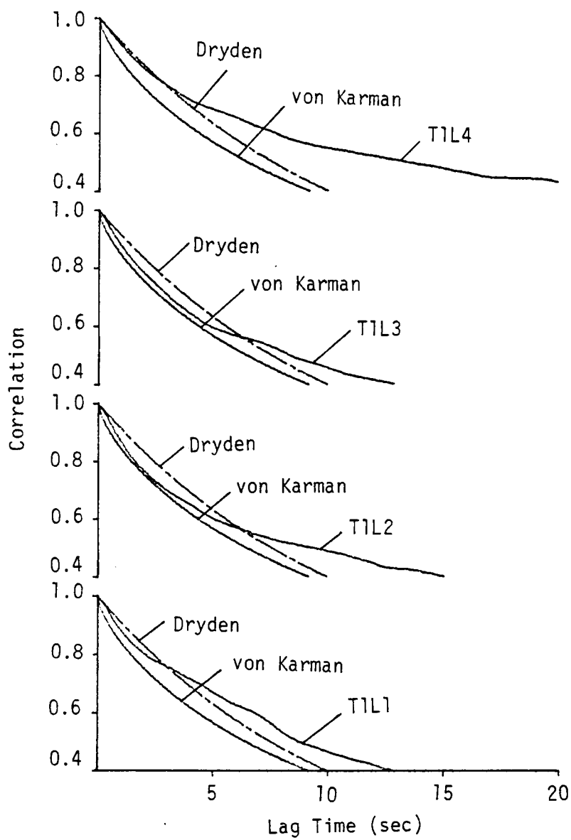
Figure 6.22. Comparison with von Karman and Dryden expressions for the longitudinal correlation (length scale L_4 , T1, Run #8624).
