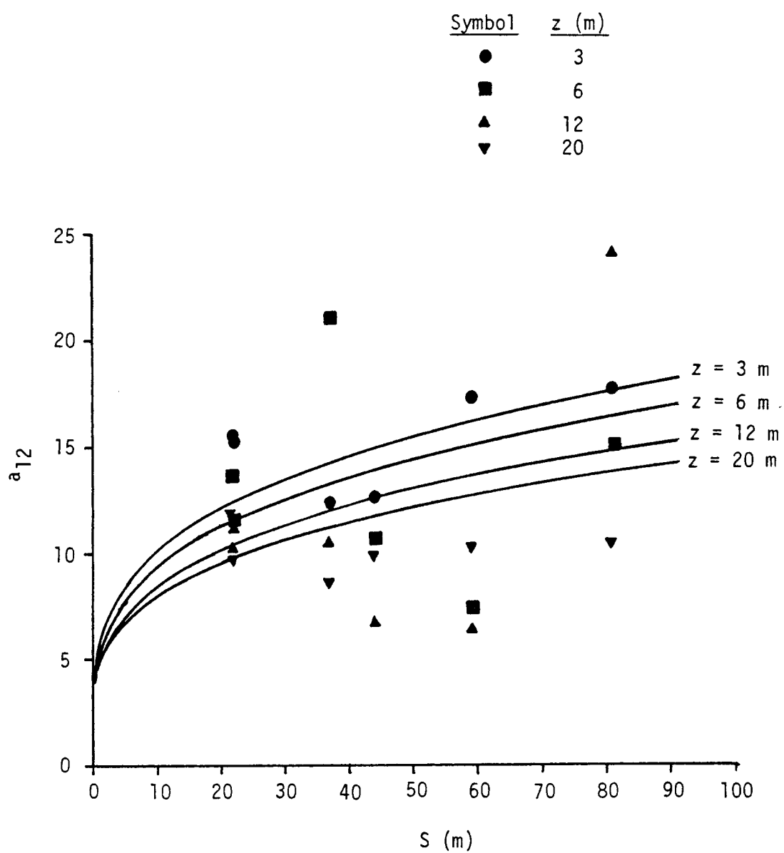
Figure 8.17. Comparison of the decay parameter a_{12} with Equation 8.16.
