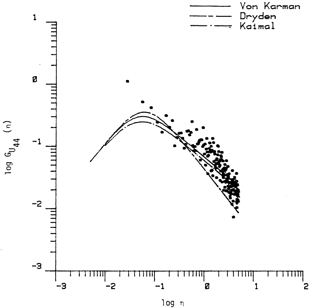
Figure 7.15. Comparison of longitudinal turbulence spectra with three analytical models. (The length scale is calculated by Method 4, T4).
