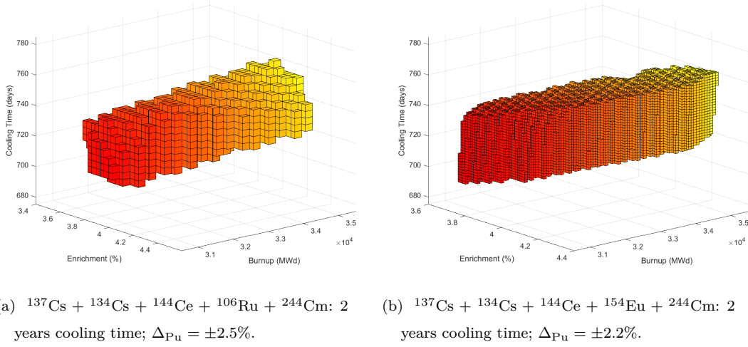
Figure 10: Degeneracy spaces for gamma-based burnup indicators, combined with gross neutron counting from ^{244}\text{Cm} ; 2-years post-discharge. \sigma_\gamma = 5\% , \sigma_{244} = 10\% .
