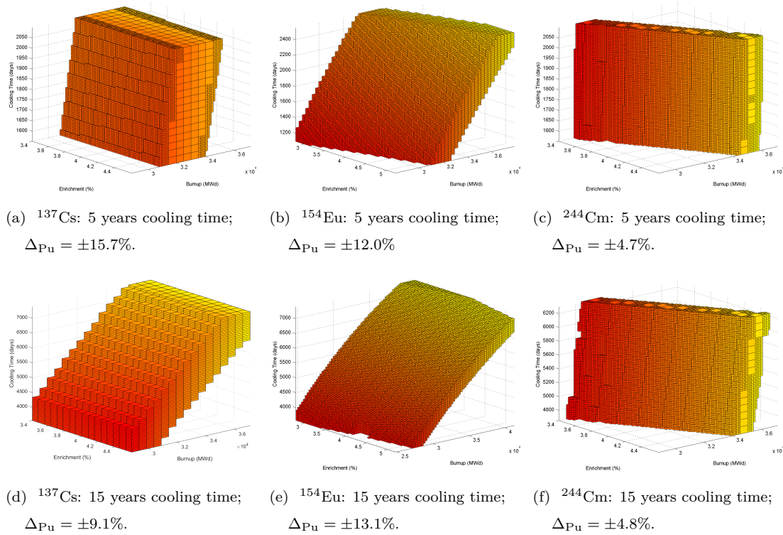
Figure 5: Degeneracy space for longer-lived burnup indicators: ^{137}\text{Cs} ( \tau_{1/2} = 30.17 \text{ y} ), ^{154}\text{Eu} ( \tau_{1/2} = 8.59 \text{ y} ), and ^{244}\text{Cm} ( \tau_{1/2} = 18.103 \text{ y} ); \sigma_{137} = \sigma_{154} = 5\% ; \sigma_{244} = 10\% .
