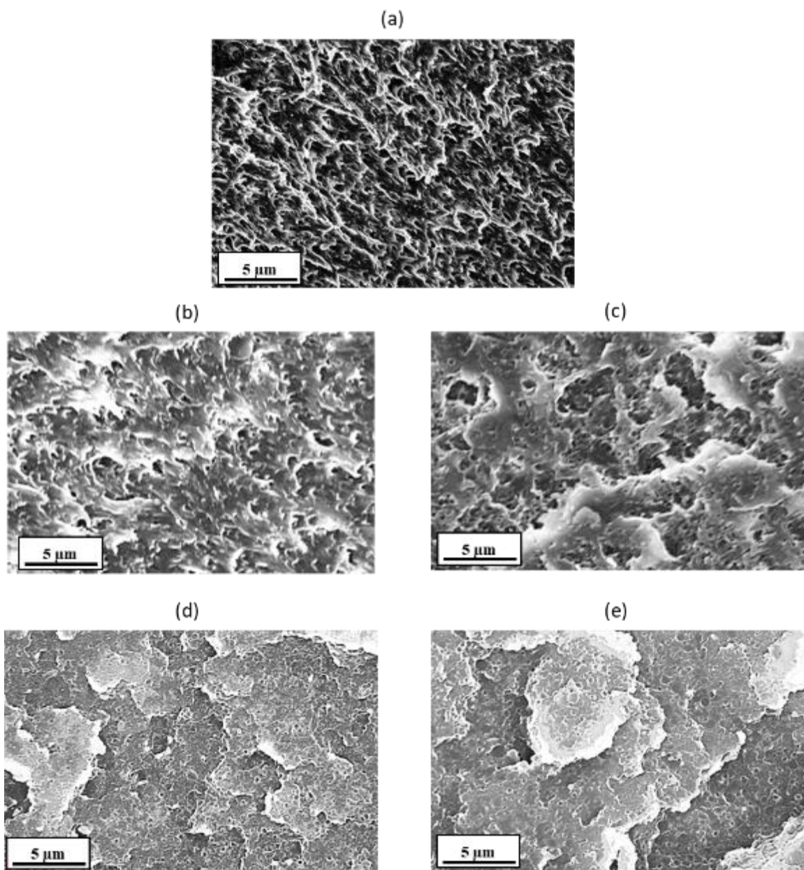
Figure A-1. Micrographs of tensile fractured surfaces; (a) neat ABS, (b) ABS/10% lignin, (c) ABS/10% lignin-PEO, (d) ABS/30% lignin, and (e) ABS/30% lignin-PEO.
