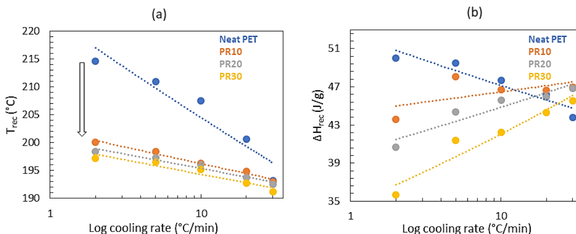
Figure 3-2. (a) Crystallization peak temperatures T_{\text{rec}} and (b) crystallization enthalpy \Delta H_{\text{rec}} as a function of log cooling rate.
