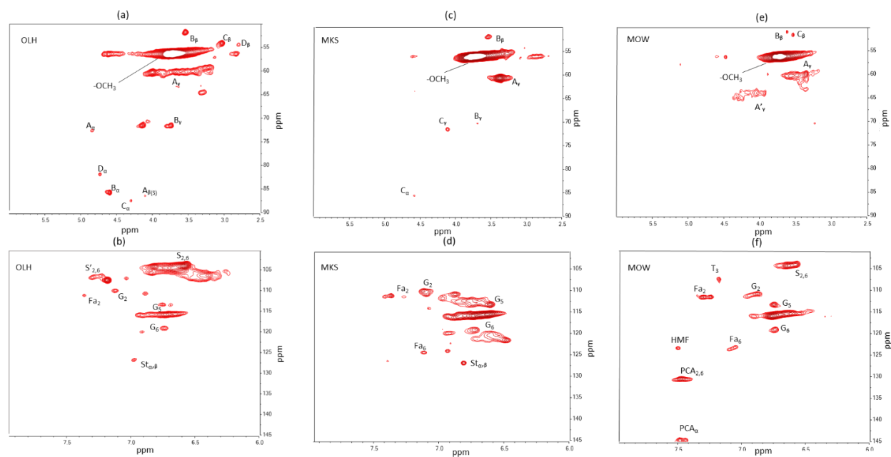
Figure 5-2. Oxygenated Aliphatic side chain ( \delta_C/\delta_H = 50-90/2.5-6 ) and aromatic ( \delta_C/\delta_H = 100-145/6-8 ) regions of 2D NMR heteronuclear single quantum coherence HSQC spectra of OLH, MKS, MOW lignins.
