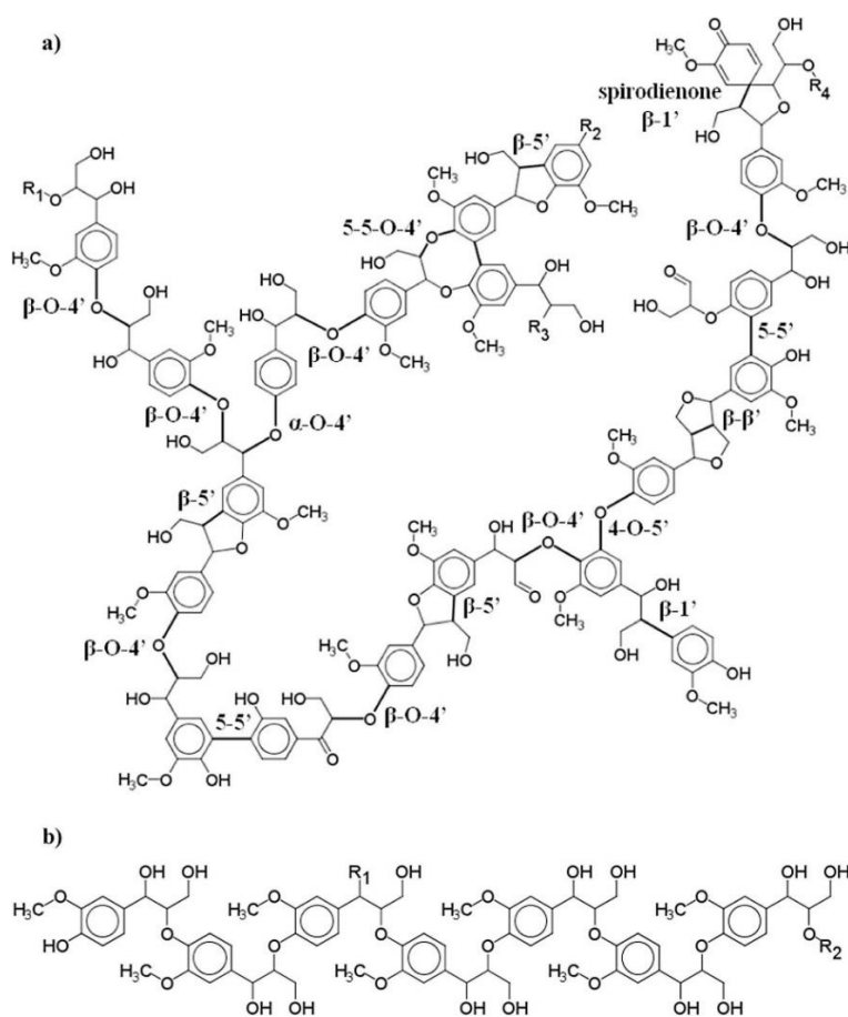
Figure 1-2. Empirical model structure of spruce lignin with two different structures: The random branching model (a), the linear lignin model (b) [3, 4].
