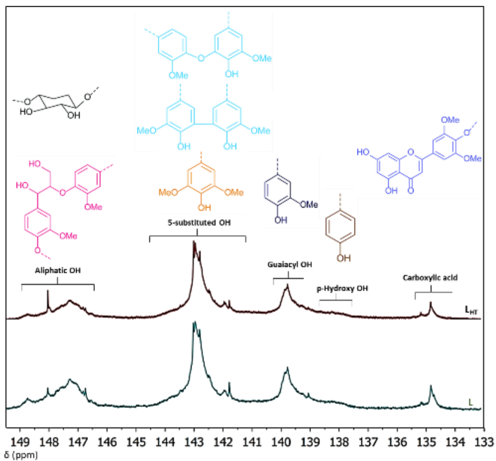
Figure 4-1. Functional groups identified by quantitative ^{31}\text{P} NMR measurements after phosphorylation of lignins L and L HT .
