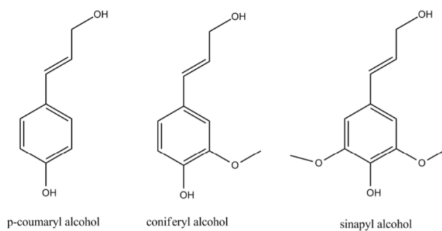
Figure 1-1. Phenylpropanoid monomers of lignin: p-coumaryl, coniferyl, and sinapyl alcohols [7].
