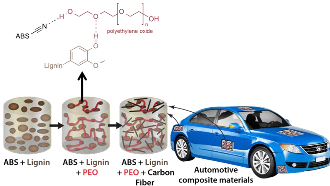
Figure 2-1. Schematic diagram of compositions of lignin-extended ABS resins and their fiber-reinforced composites created from a blend modified with poly(ethylene oxide).
