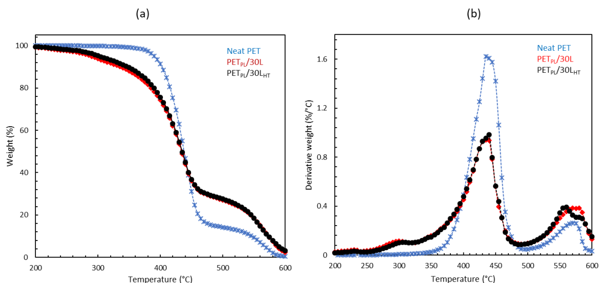
Figure C-5. Thermal decomposition of PET and it lignin derived blends at 30 wt.% lignin contents in oxidative atmosphere at 20°C/min.
