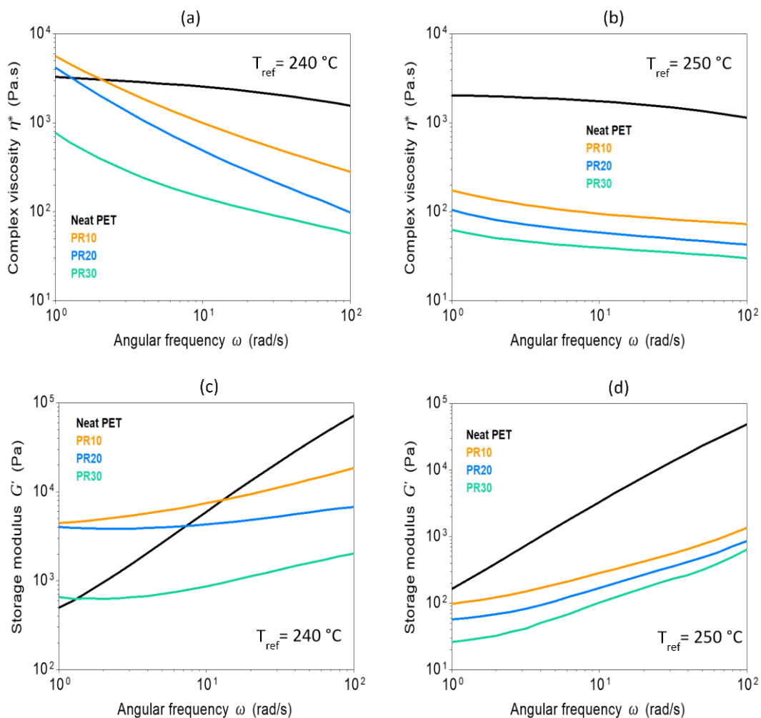
Figure 3-3. Frequency-dependent complex viscosity \eta^* at T_{ref} = 240\text{ °C} (a) and 250\text{ °C} (b) and Frequency-dependent storage modulus G' at T_{ref} = 240\text{ °C} (c) and 250\text{ °C} (d) of recycled PET and its TOFA plasticized derivatives.
