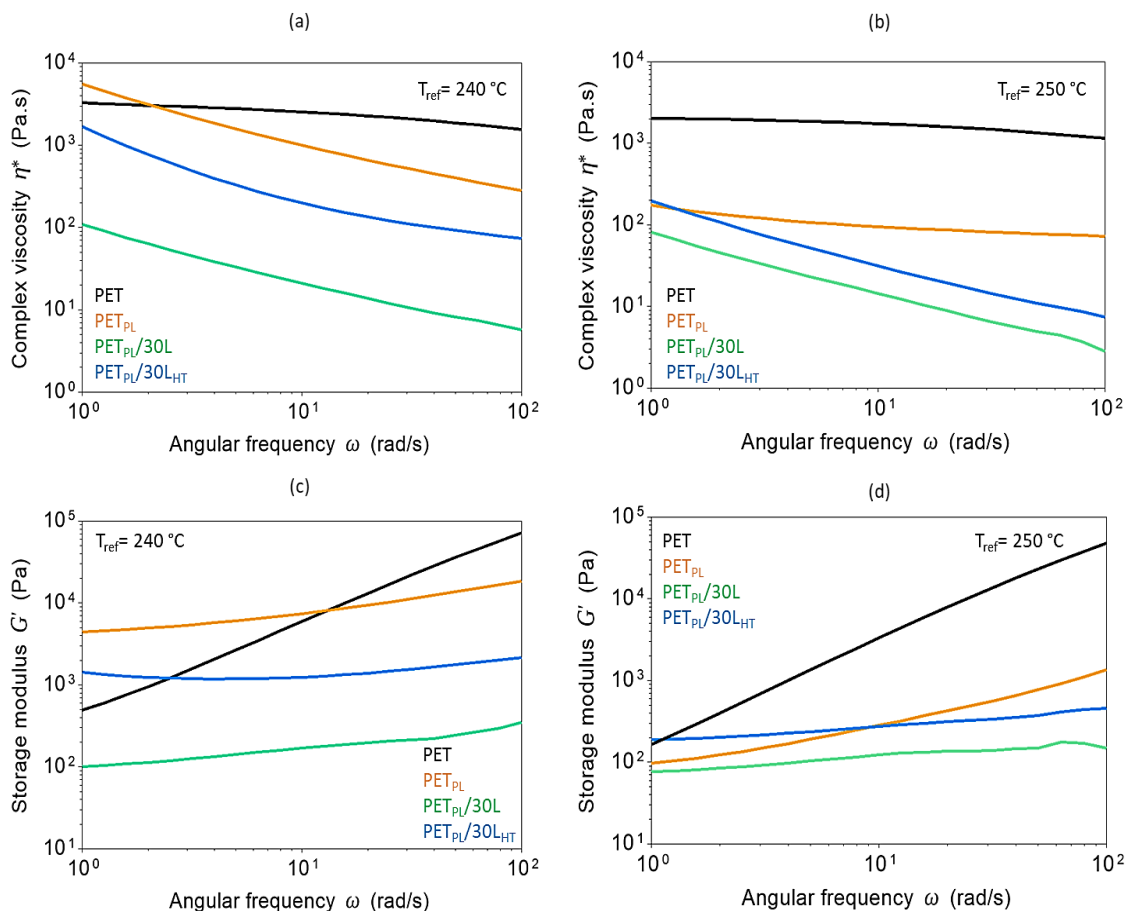
Figure 4-6. Frequency-dependent complex viscosity ( \eta^* ) at T_{ref} = 240 °C (a) and 250 °C (b) and Frequency-dependent storage modulus ( G' ) at T_{ref} = 240 °C (c) and 250 °C (d) of recycled PET, its plasticized resin (PET PL ), and its lignin-derived blends (PET PL /30L and PET PL /30L HT ).
