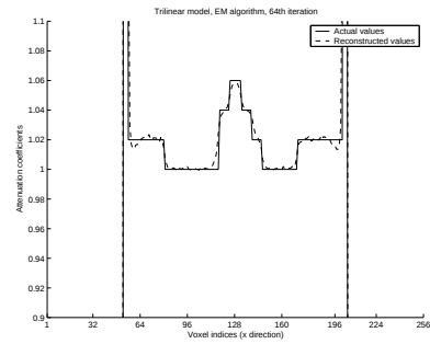
(c) Trilinear/EM
