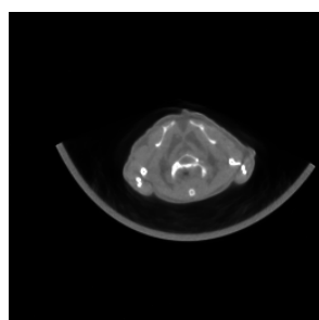
(c) Trilinear/EM
