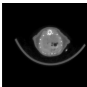
(a) Trilinear/SART
