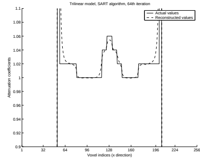
(a) Trilinear/SART
