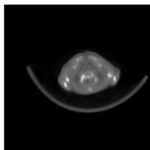
(e) Trilinear/FWLS
