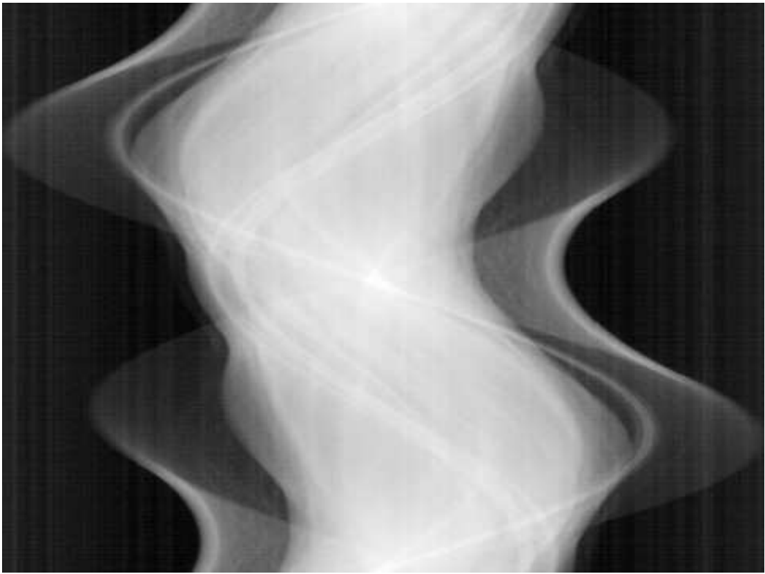
Figure 2.2. Fanbeam sinogram of a mouse
