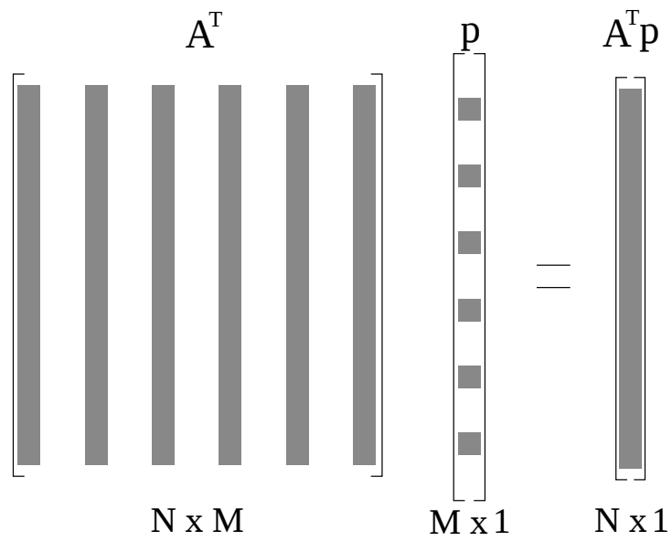
Figure 4.8. Partial backprojection
