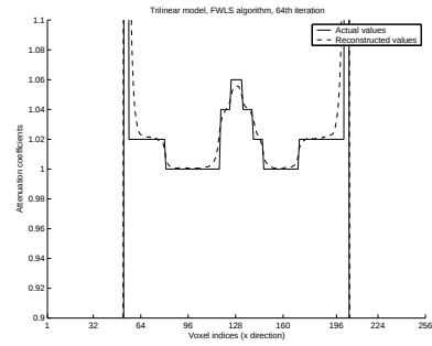
(e) Trilinear/FWLS
