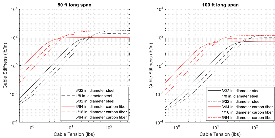
Figure 4.9 7x19 Steel vs. Carbon Fiber Cables
