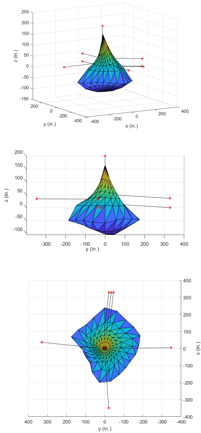
Figure 4.3 Workspace Boundary
