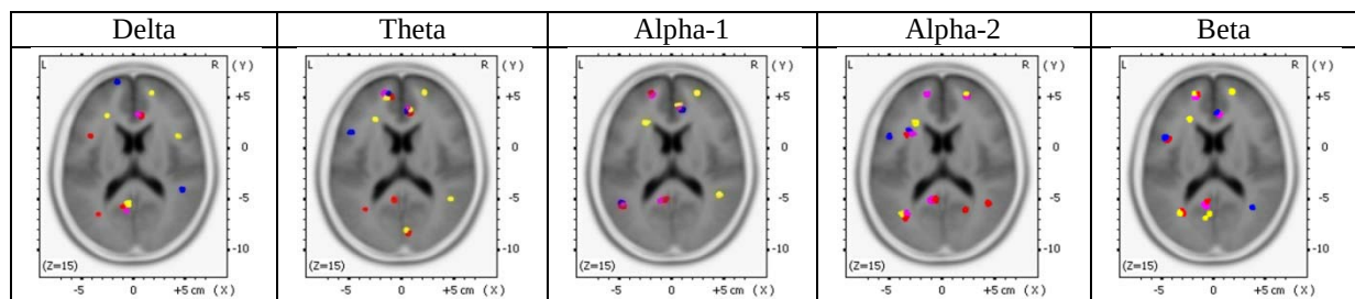
Figure 7: Regions of self-specific activation in each frequency domain. The images are a horizontal slice through the brain at z=15 . Regions are approximated for 2-D rendering. The blue regions in the image are those showing increased CSD during the SI condition. The yellow regions in the image are those showing increased CSD during the ES condition. The red regions in the image are those showing increased CSD during the BSI condition. The pink regions are those showing increased CSD during the TSCS condition.
