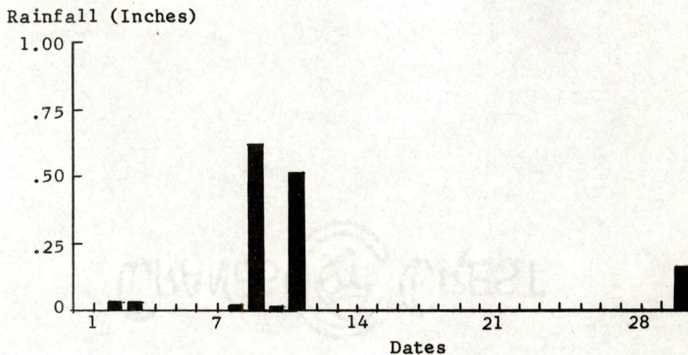
Figure 3-Inches of daily rainfall, U. S. Cotton Field Station, and daily maximum and minimum temperatures, U. S. Weather Bureau, Knoxville Airport, Knoxville, Tennessee, September 1959.
