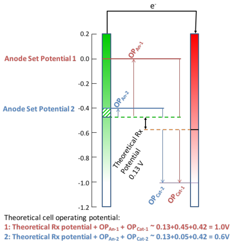
Figure 45: Theoretical overpotentials for 0 and -400 mV reactors operated with acetate as the substrate. (OP) indicates operating potential, (An) indicates anode, (Cat) indicates cathode. Voltage values are relative to Ag/AgCl reference electrode.
