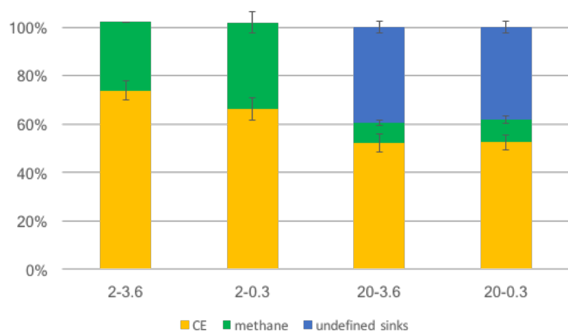
Figure 23: Electron balance across different operating conditions.
