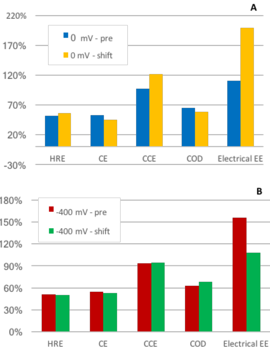
Figure 48: Efficiency values for pre and post potential (A) 0 mV reactor shifted to -400 mV and (B) -400 mV reactor shift to 0 MV.
