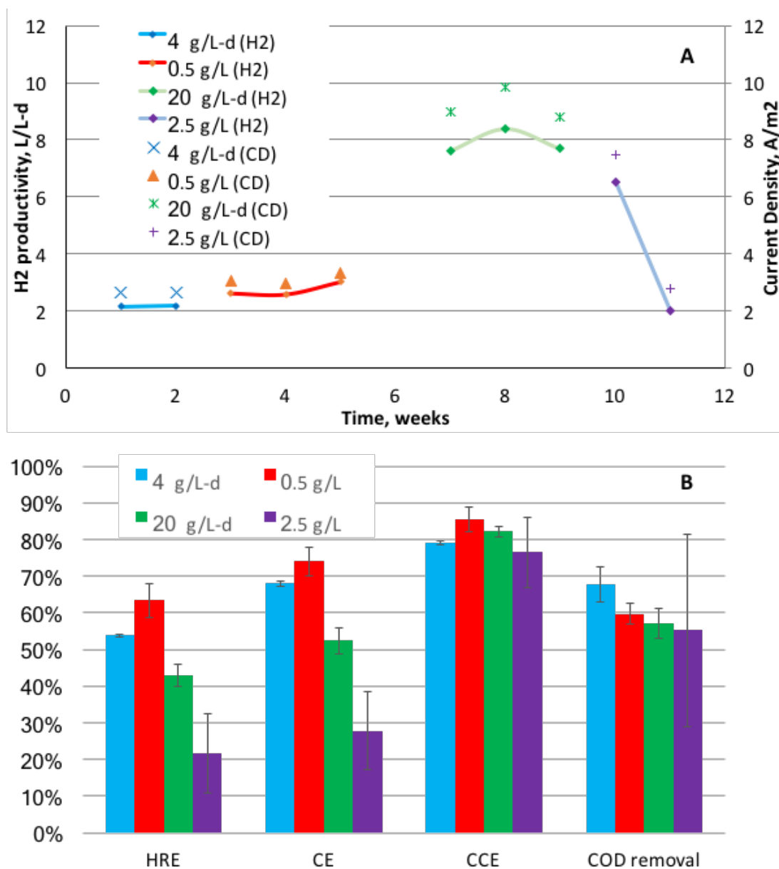
Figure 35: (A) MEC performance obtained under continuous and fed-batch mode of operation at various loading conditions. The units g/L-d in the legend refer to continuous mode of operation, while g/L refers to fed-batch mode of operation. (B) MEC efficiency and COD removal during continuous and fed-batch mode of operation. HRE: Hydrogen Recovery, CE: Anode Coulombic Efficiency, CCE: Cathode Conversion Efficiency.
