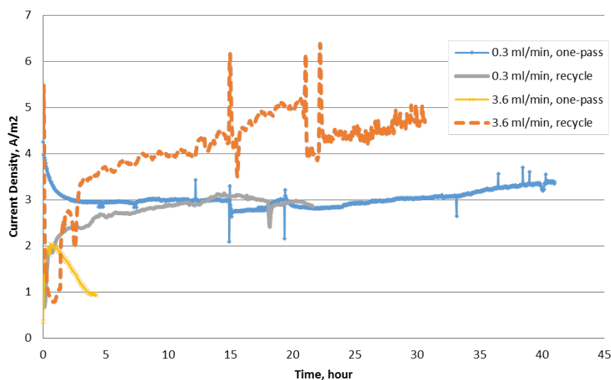
Figure 20: Comparison of current output across different flow rates during one-pass and recycle operation at 10 g/L-d.
