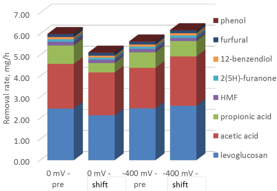
Figure 49: Individual compound removal during BOAP conversion before and after 48 hours of potential shift experiments.
