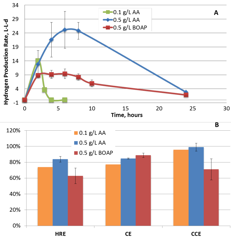
Figure 25: (A) Hydrogen productivity and (B) efficiency during batch experiments with BOAP and acetic acid as substrate.
