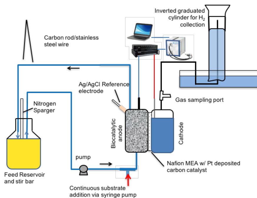
Figure 46: Schematic of MEC system
