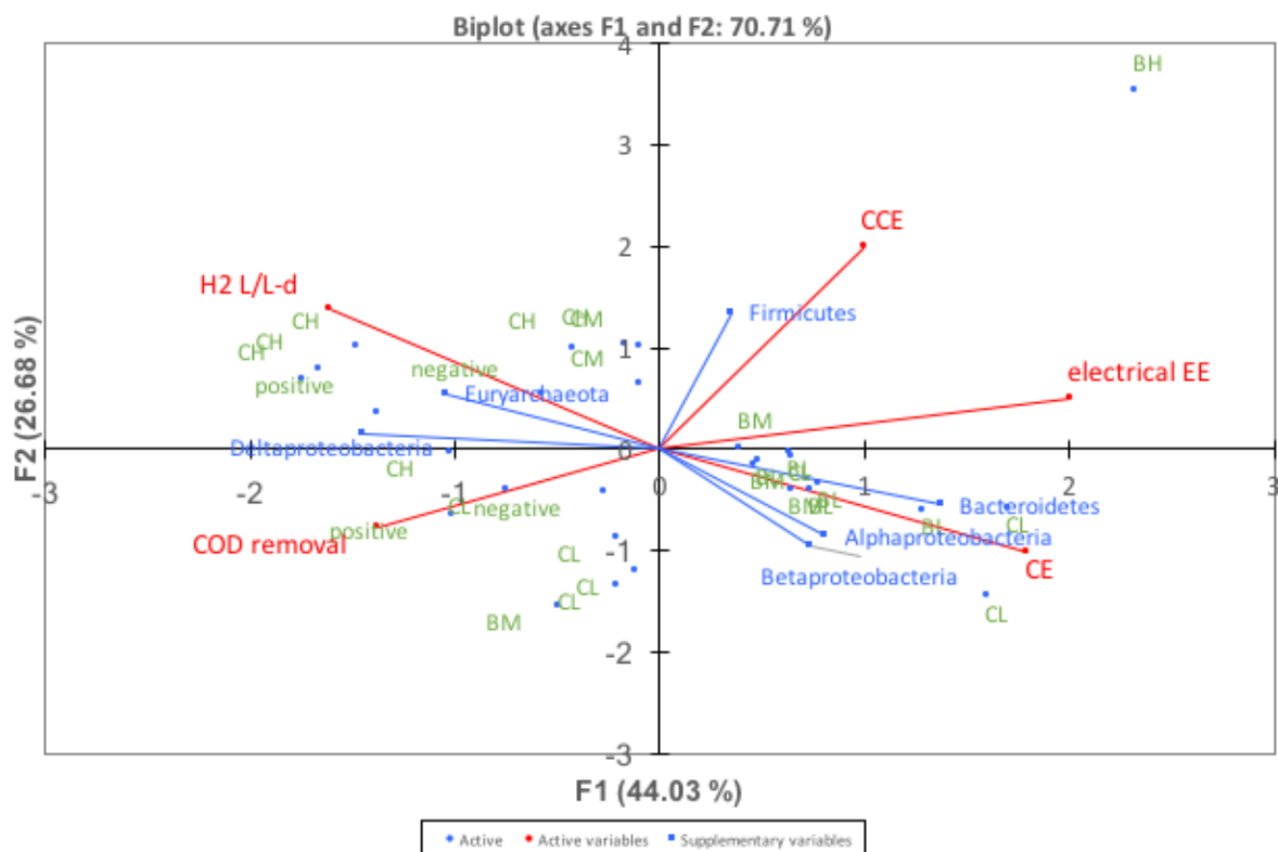
Figure 66: Canonical correspondence analysis (CCA) of all experimental conditions tested and the microbial taxa observed.
