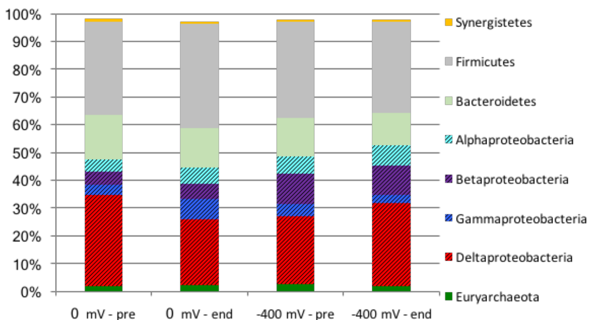
Figure 54: 16S rRNA analysis of microbial community pre-shift and after long-term exposure to opposite potential levels. (A) Phylum and Class level. (B) Individual OTUs displaying potential redox preferences.
