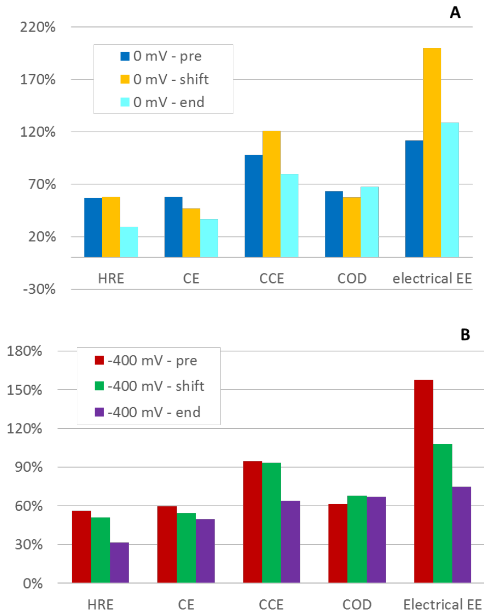
Figure 51: Efficiency values comparing pre-shift, post-shift, and end after long-term exposure to opposite potential levels.
